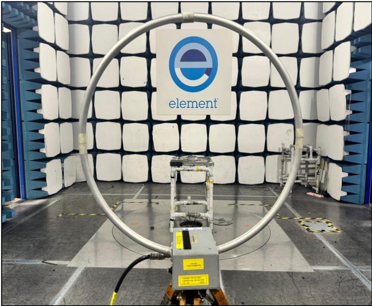
9kHz to 30MHz – Radiated
