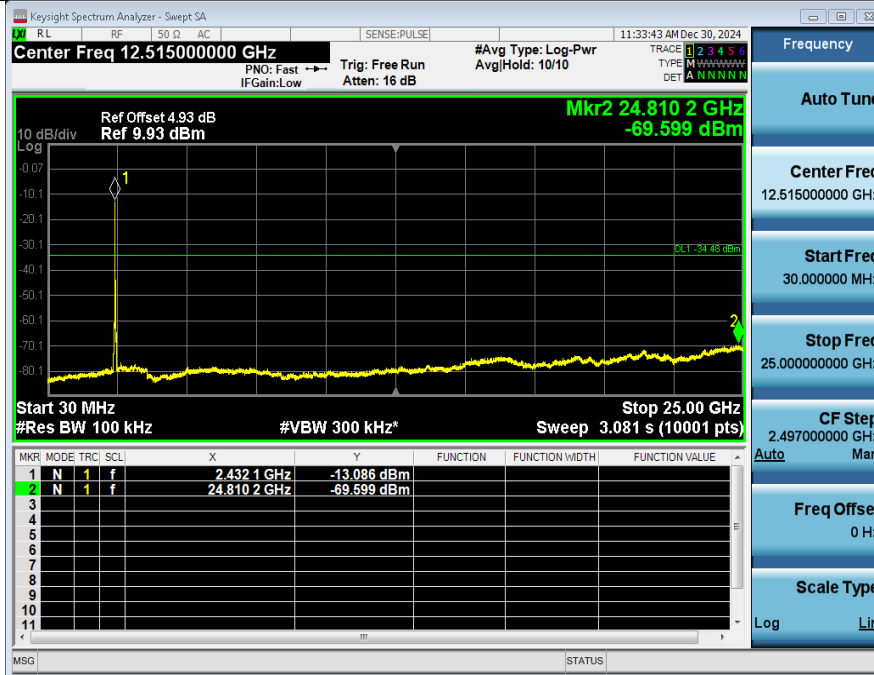
2_Spurious_Emission_NVNT_ANT1_802_11n(HT20)_2437
