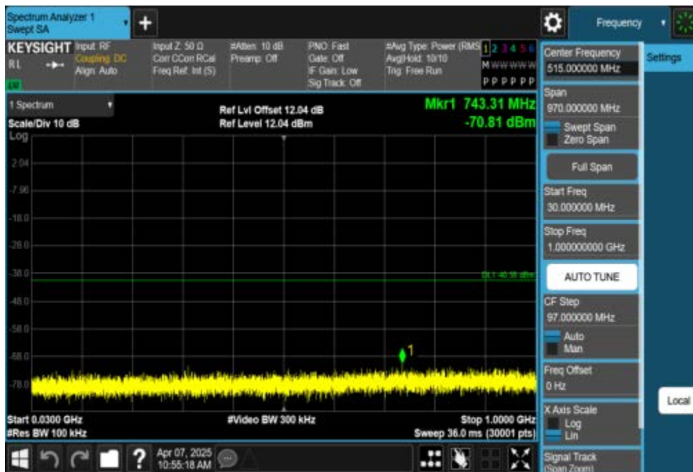
11N40SISO-Ant1-2422-30~1000-PASS
