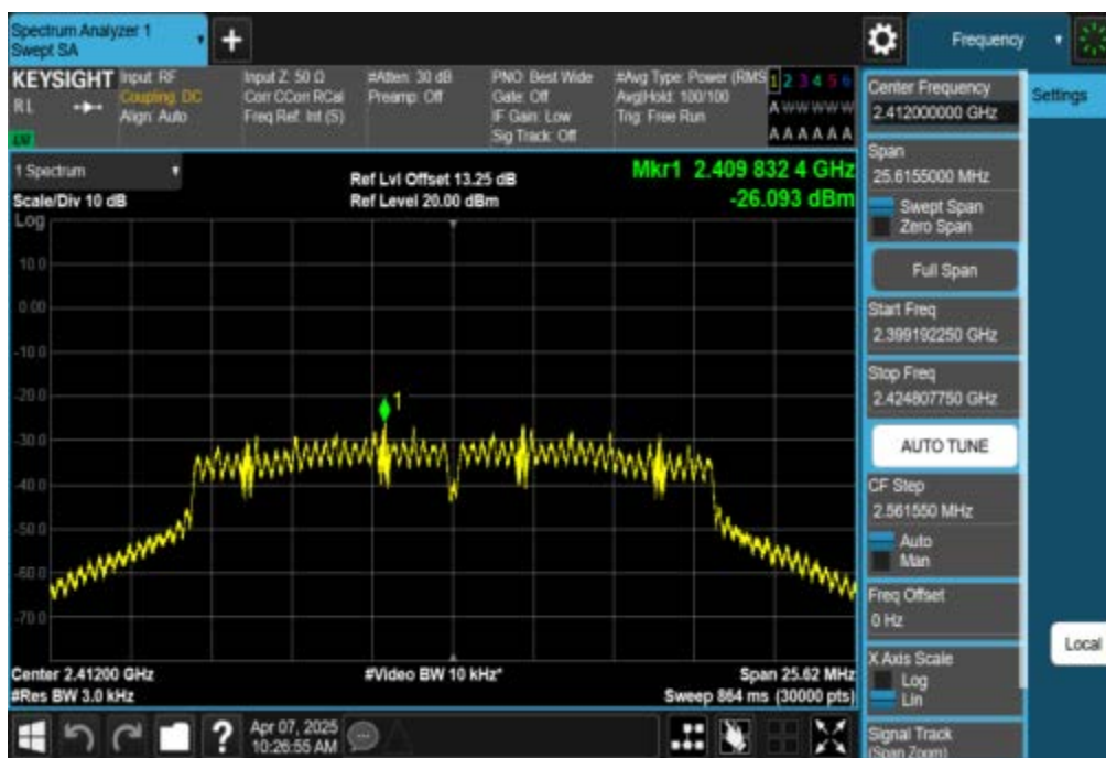
11G-Ant1-2412-PASS
