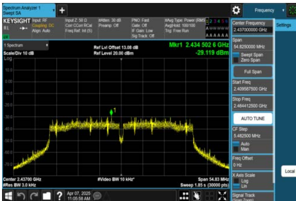
11N40SISO-Ant1-2437-PASS
