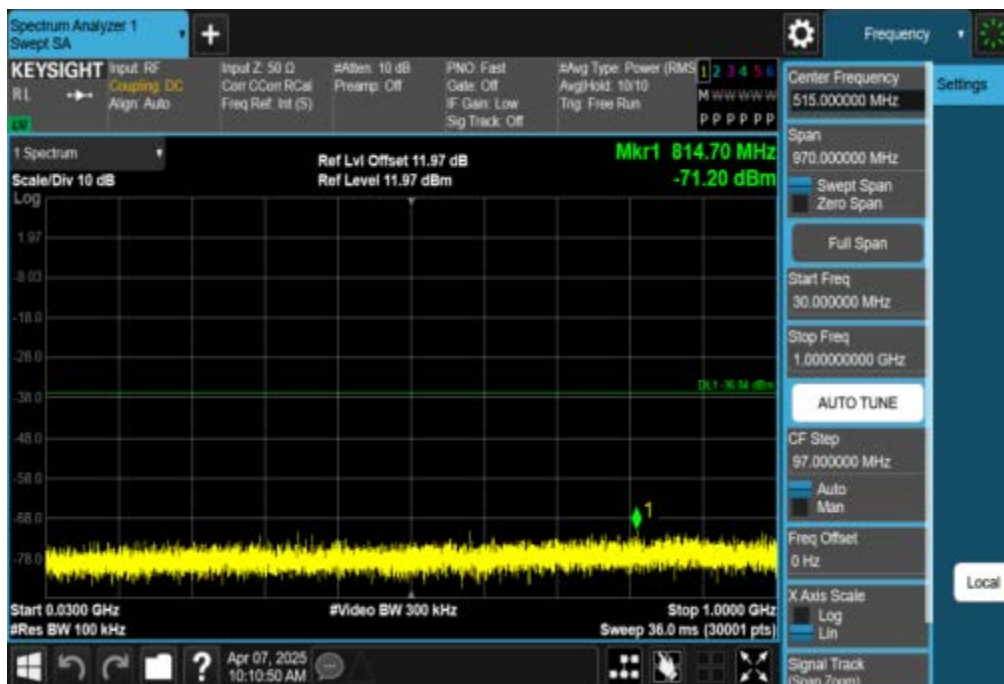
11B-Ant1-2462-30-1000-PASS
