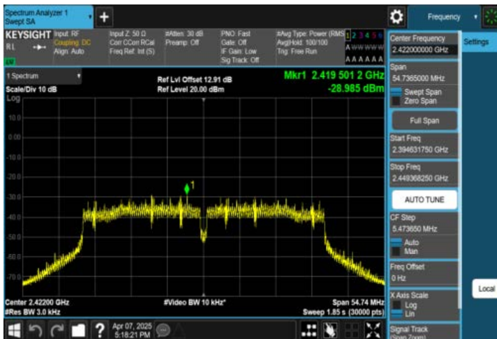
11N40SISO-Ant1-2422-PASS
