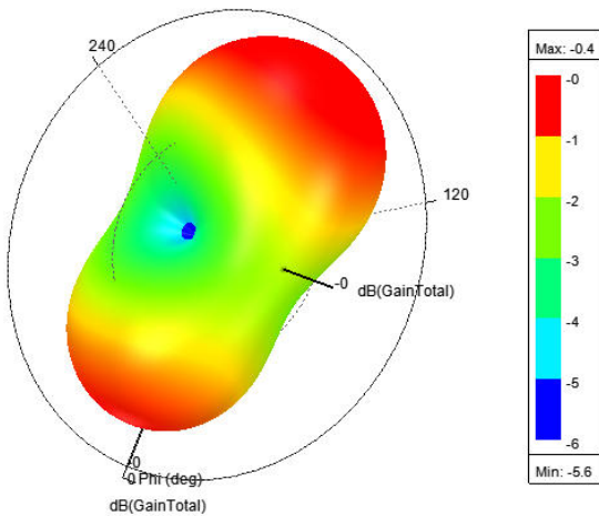
3D Gain Pattern (2450 MHz) unit:dBi
