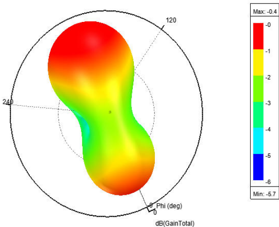
3D Gain Pattern (2500 MHz) unit:dBi
