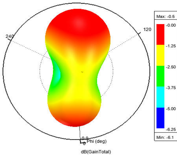
3D Gain Pattern (2500 MHz) unit:dBi
