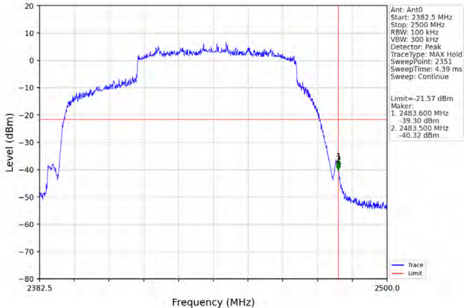
60M_HCH_2442.5MHz_Ant0_NTNV
