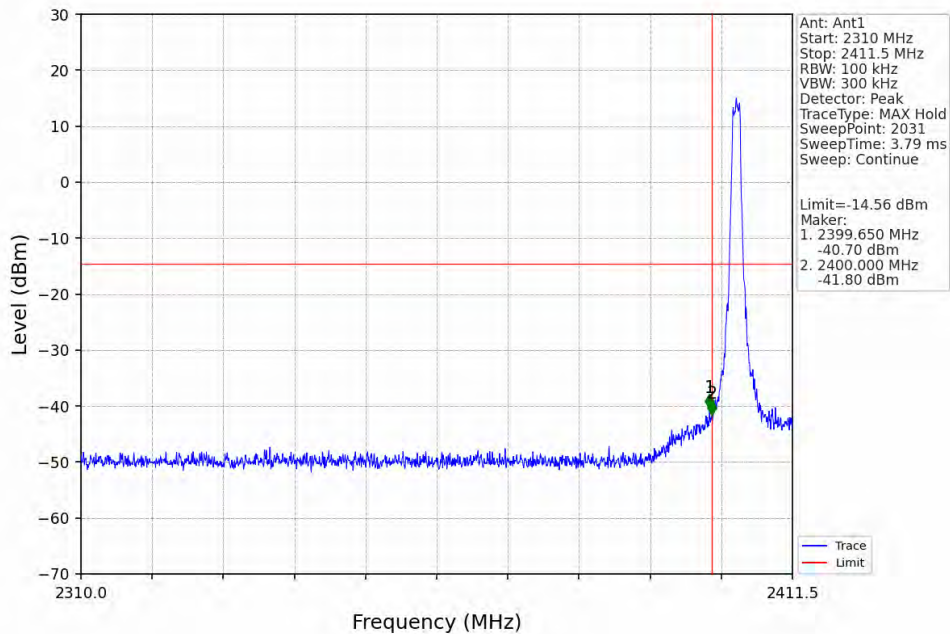
1.4M_LCH_2403.5MHz_Ant1_NTNV
