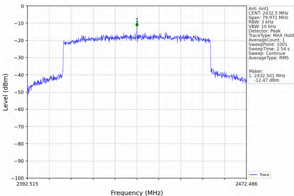
60M_LCH_2432.5MHz_Ant1_NTNV
