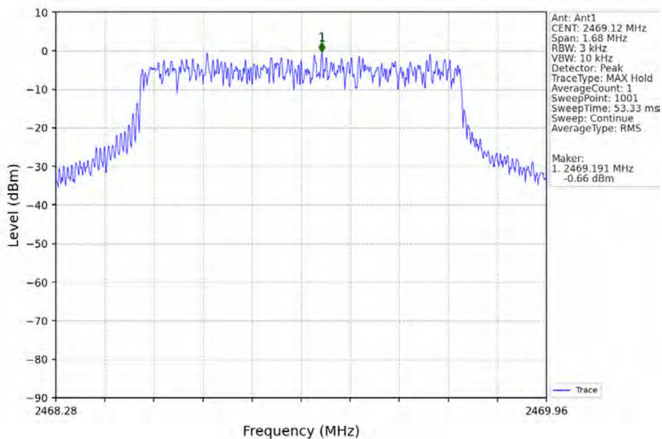
1.4M_HCH_2469.12MHz_Ant1_NTNV
