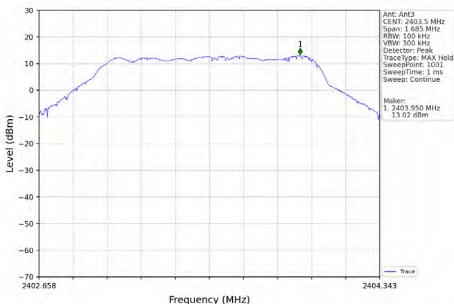
1.4M_LCH_2403.5MHz_Ant3_NTNV
