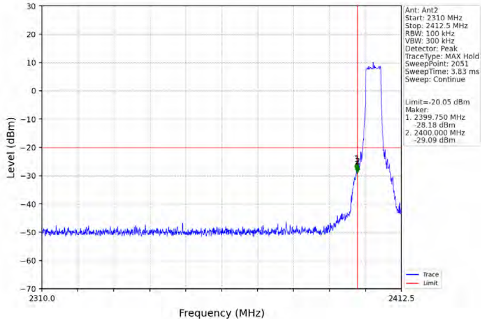
5M_LCH_2404.5MHz_Ant2_NTNV
