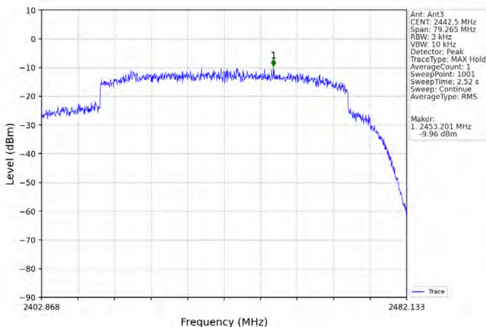
60M_HCH_2442.5MHz_Ant3_NTNV
