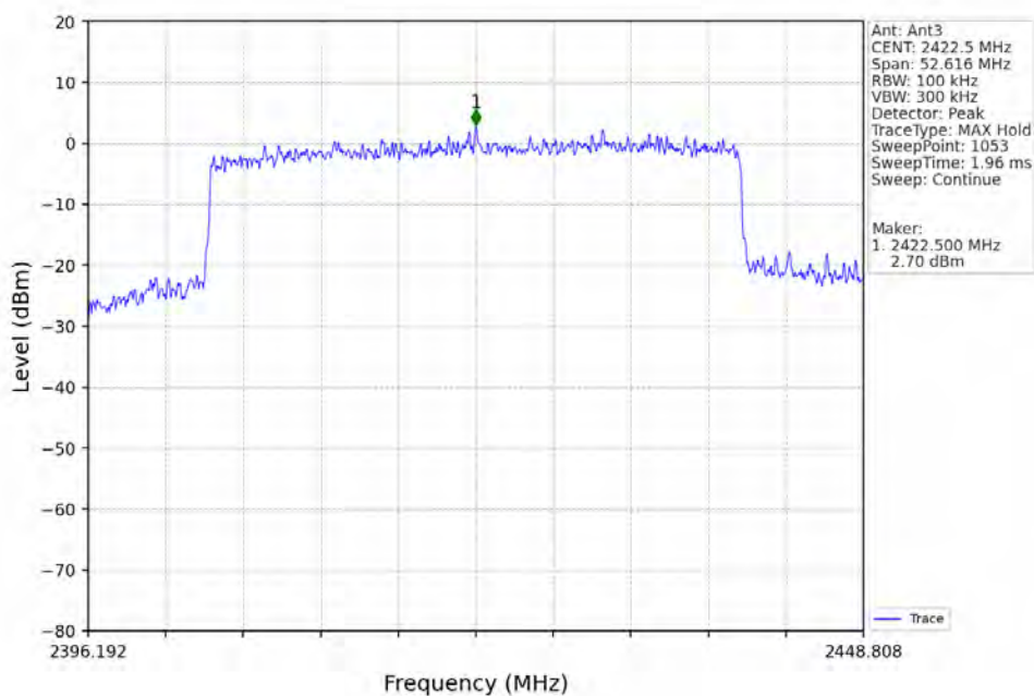
40M_LCH_2422.5MHz_Ant3_NTNV
