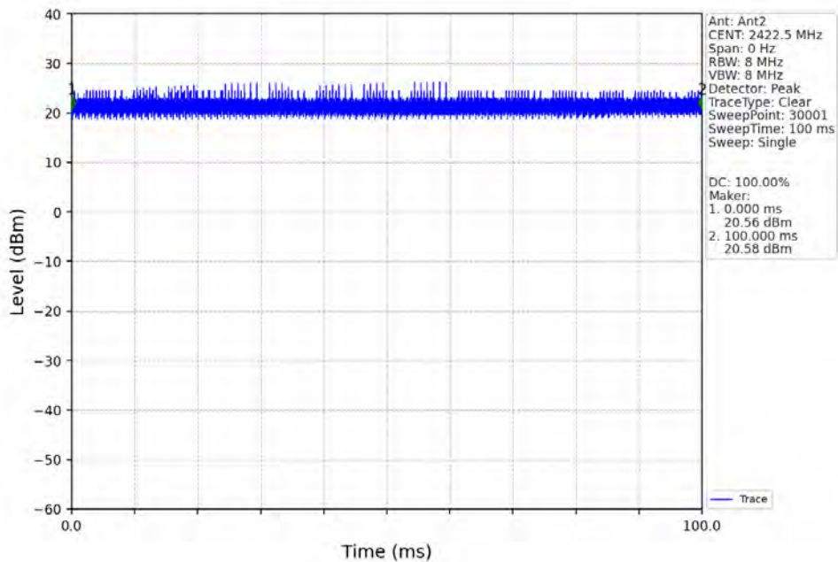
40M_LCH_2422.5MHz_Ant2_NTNV
