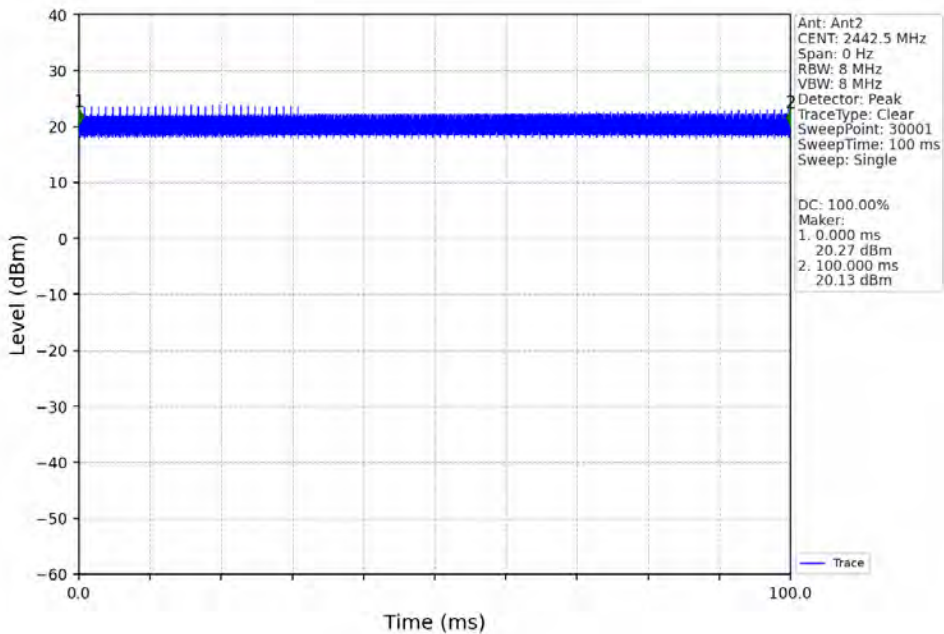
60M_HCH_2442.5MHz_Ant2_NTNV
