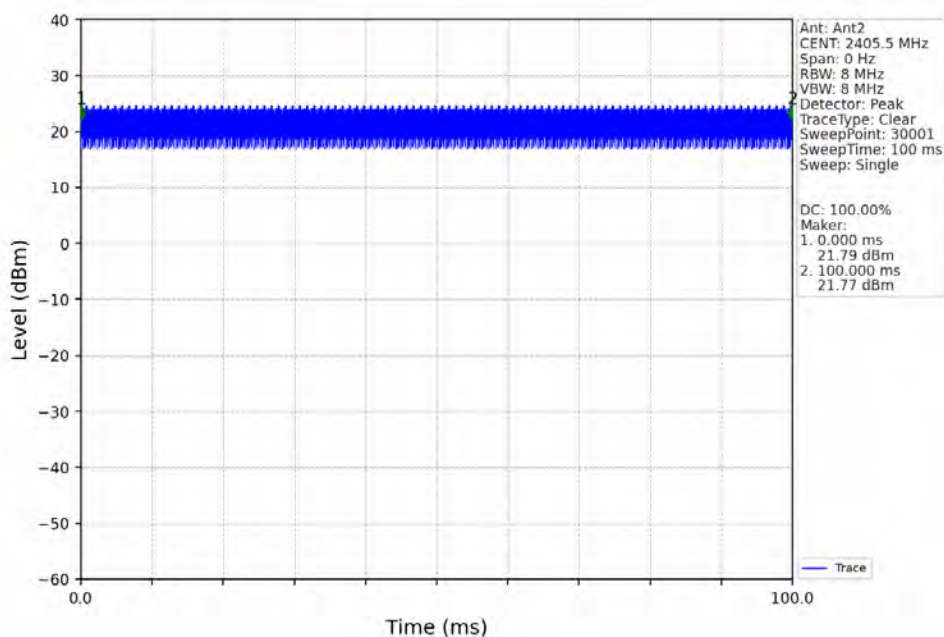
3M_LCH_2405.5MHz_Ant2_NTNV
