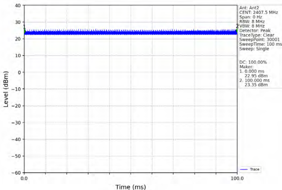
10M_LCH_2407.5MHz_Ant2_NTNV
