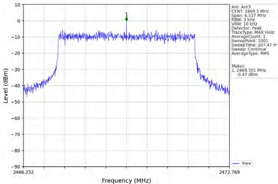
5M_HCH_2469.5MHz_Ant3_NTNV
