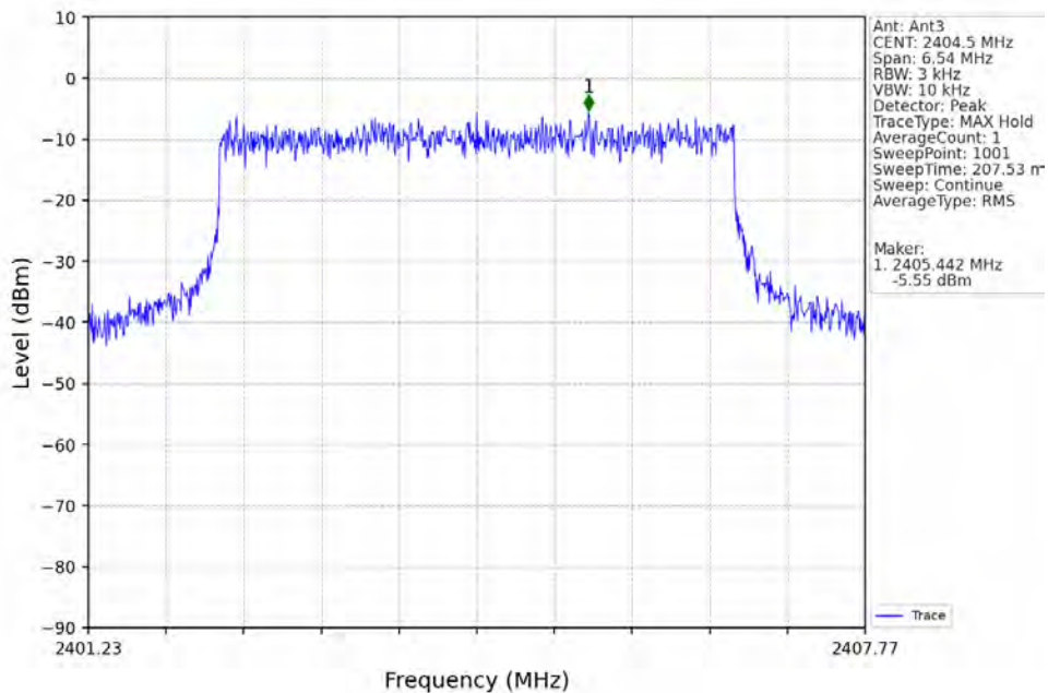
5M_LCH_2404.5MHz_Ant3_NTNV
