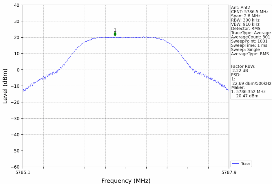
1.4M_MCH_5786.5MHz_MIMO_NTN
