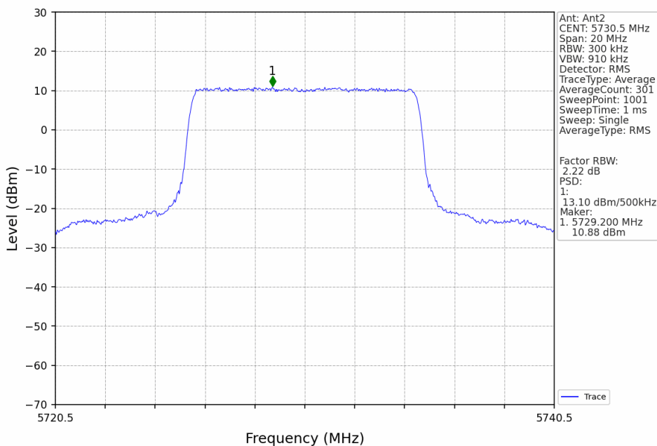
10M_LCH_5730.5MHz_MIMO_NTNV
