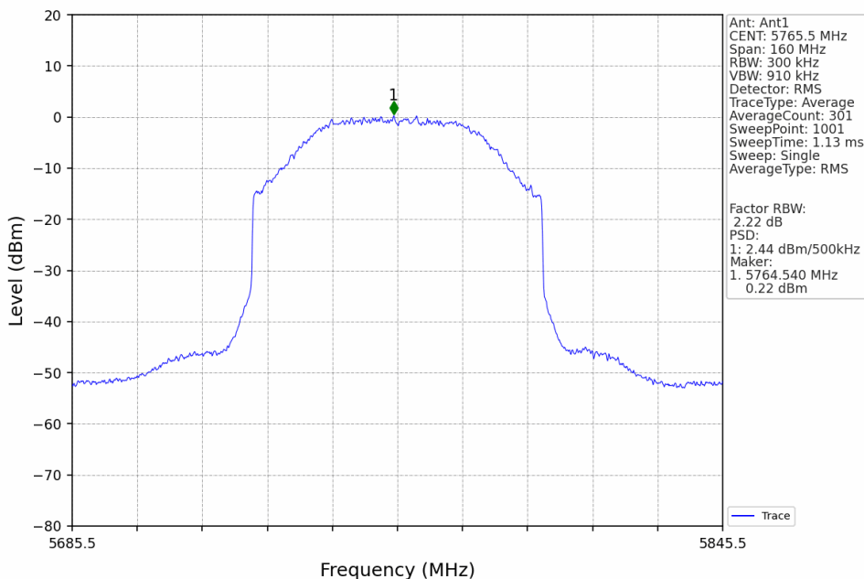
80M_LCH_5765.5MHz_Ant1_NTNV
