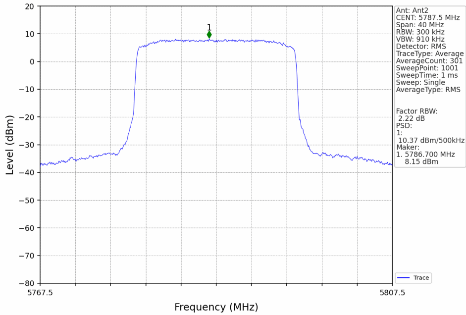
20M_MCH_5787.5MHz_MIMO_NTN
