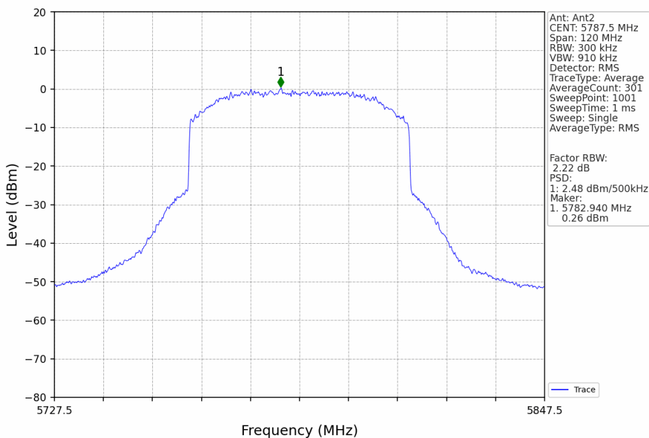
60M_MCH_5787.5MHz_MIMO_NTN
