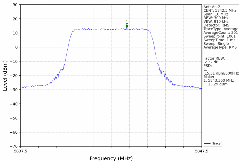
5M_HCH_5842.5MHz_Ant2_NTNV
