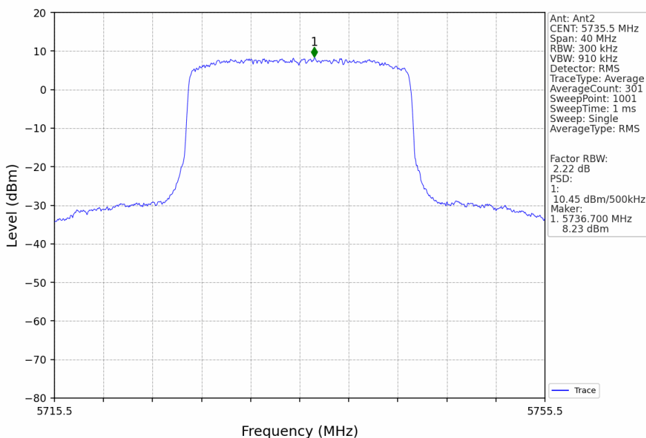
20M_LCH_5735.5MHz_Ant2_NTNV
