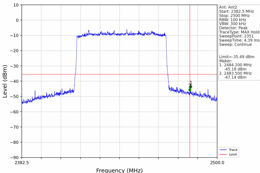
60M_HCH_2442.5MHz_Ant2_NTNV
