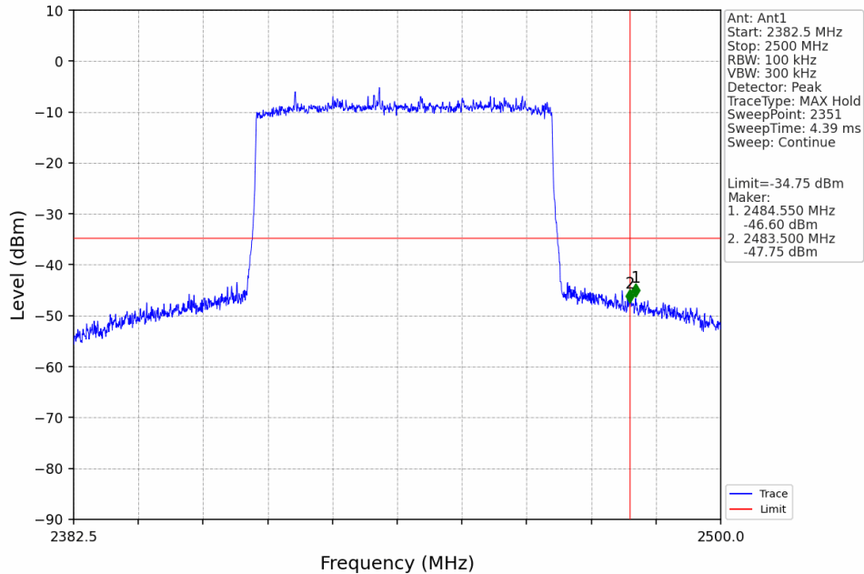
60M_HCH_2442.5MHz_Ant1_NTNV
