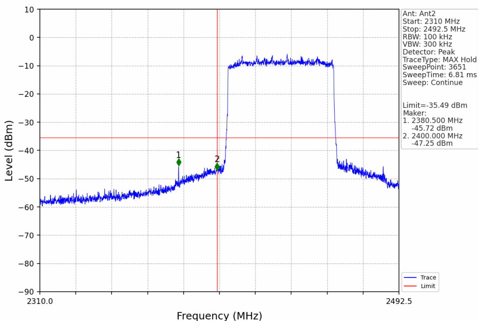
60M_LCH_2432.5MHz_Ant2_NTNV
