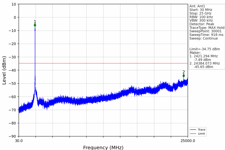
60M_LCH_2432.5MHz_Ant1_NTNV
