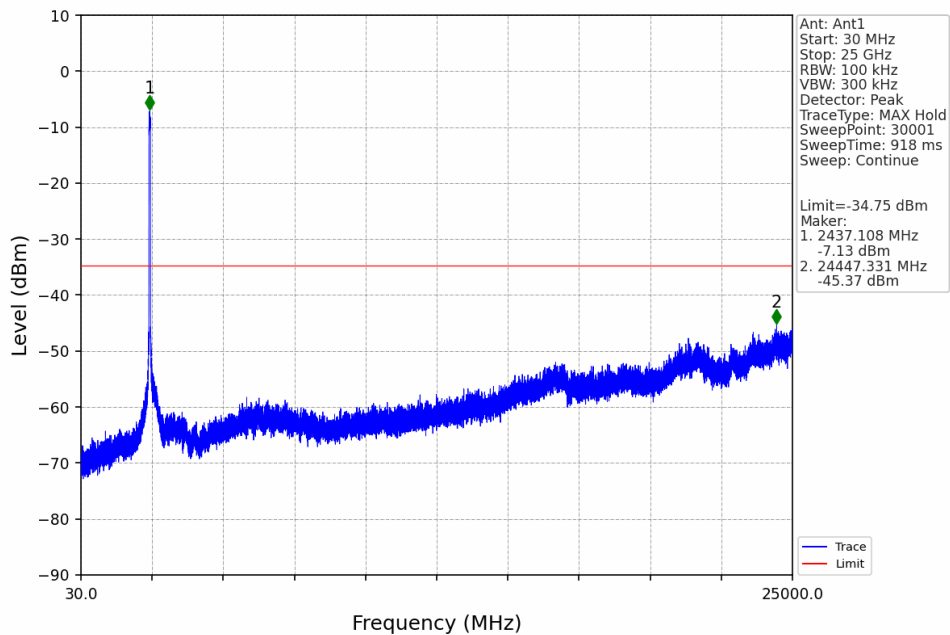
60M_HCH_2442.5MHz_Ant1_NTNV
