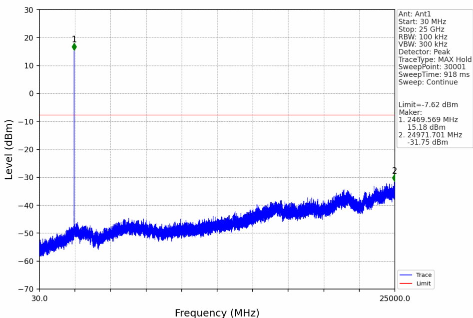
1.4M_HCH_2469.12MHz_Ant1_NTNV
