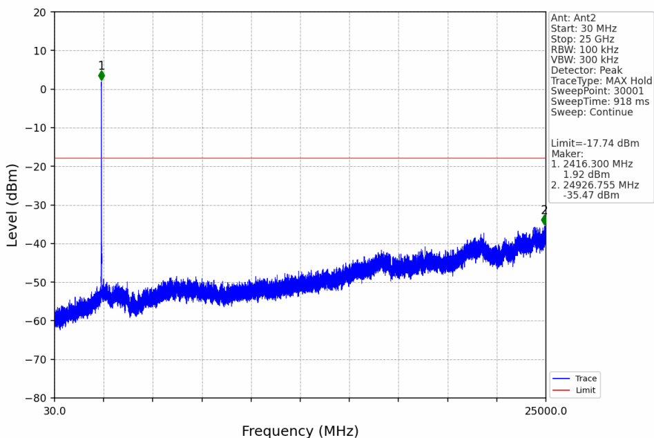
20M_LCH_2412.5MHz_Ant2_NTNV
