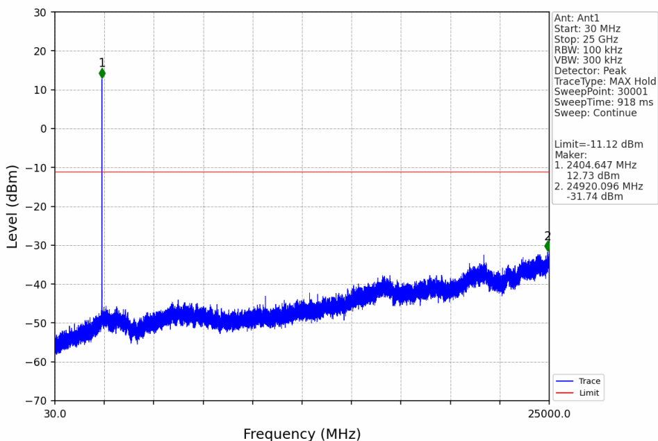
5M_LCH_2404.5MHz_Ant1_NTNV
