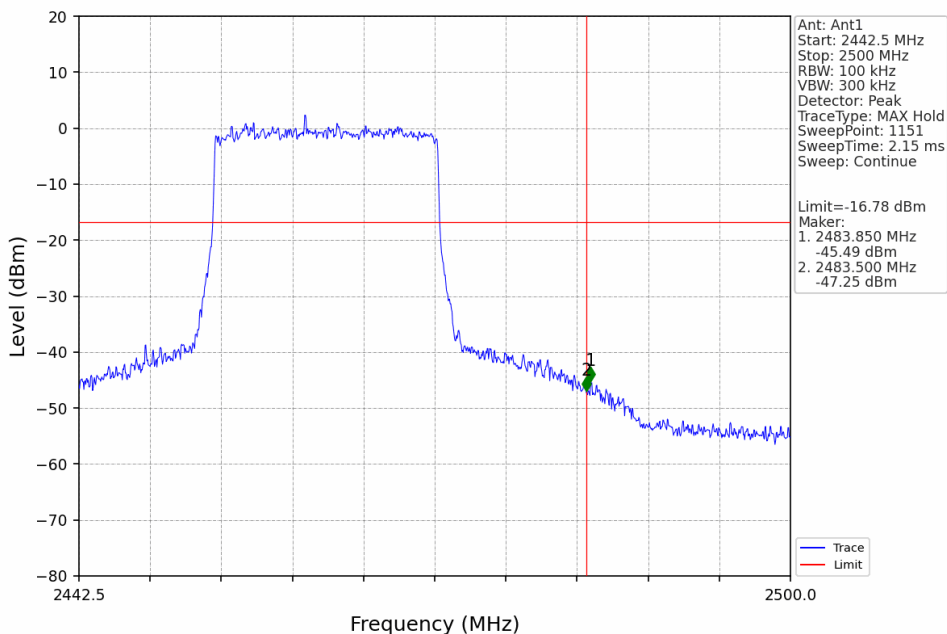
20M_HCH_2462.5MHz_Ant1_NTNV
