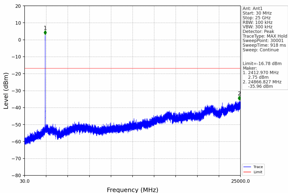
20M_LCH_2412.5MHz_Ant1_NTNV
