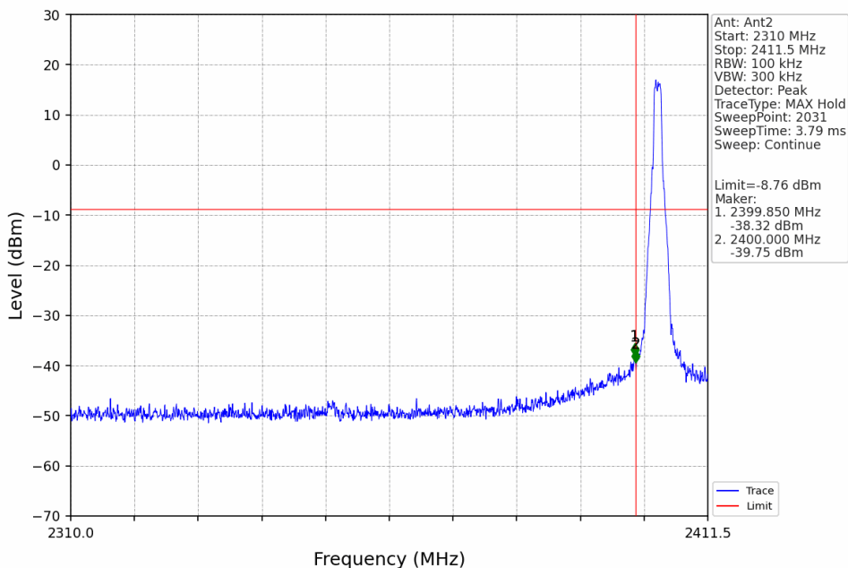
1.4M_LCH_2403.5MHz_Ant2_NTNV
