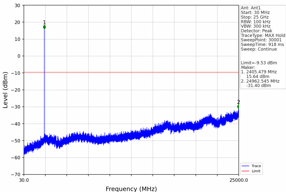
3M_LCH_2405.5MHz_Ant1_NTNV
