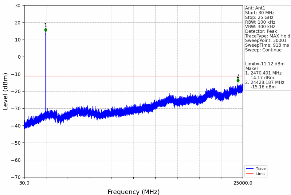
5M_HCH_2469.5MHz_Ant1_NTNV
