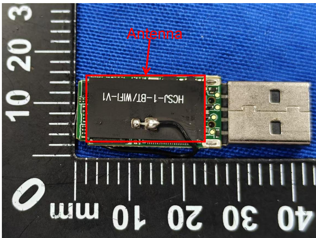
PCB view of unit (Model: C3020A; HVIN: C3020A)
