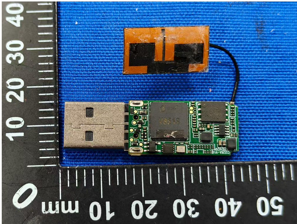
PCB view of unit (Model: U2; HVIN: U2)
