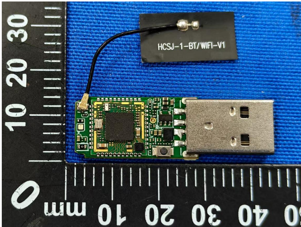
PCB view of unit (Model: U3; HVIN: U3)
