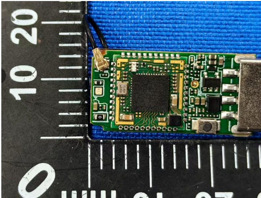
PCB view of unit (Model: C3020A; HVIN: C3020A)
