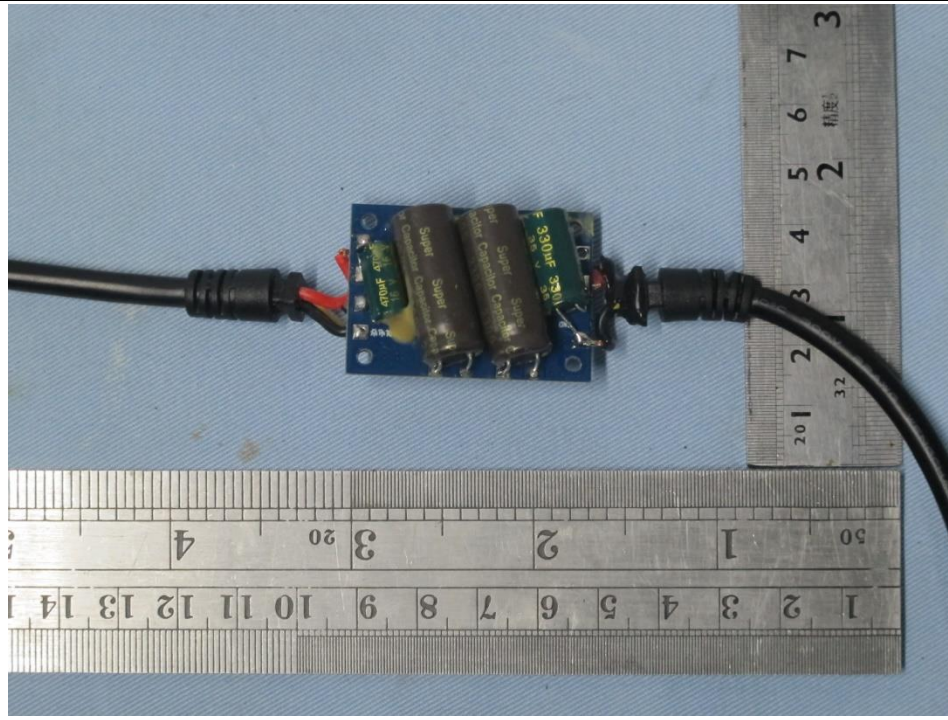
11. Front View of Power Box PCB
