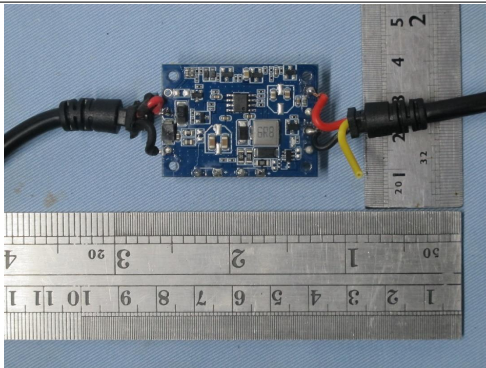
12. Rear View of Power Box PCB
