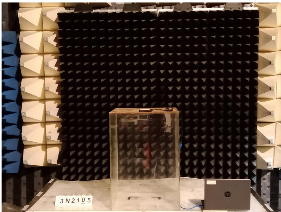
04. RADIATED BAND EDGE Rear View(1GHz above)
