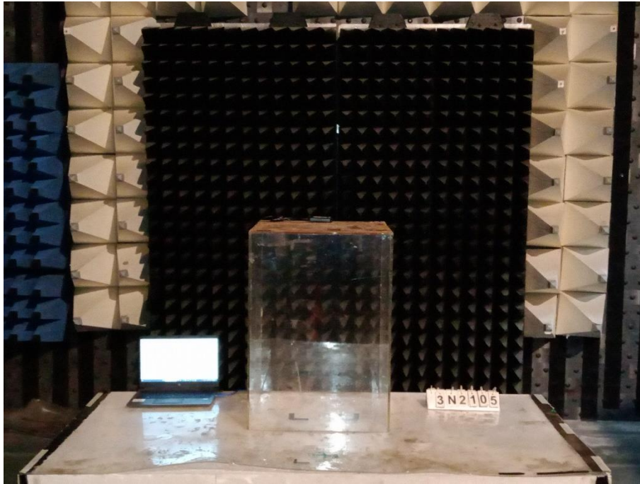
03. RADIATED BAND EDGE Front View(1GHz above)
