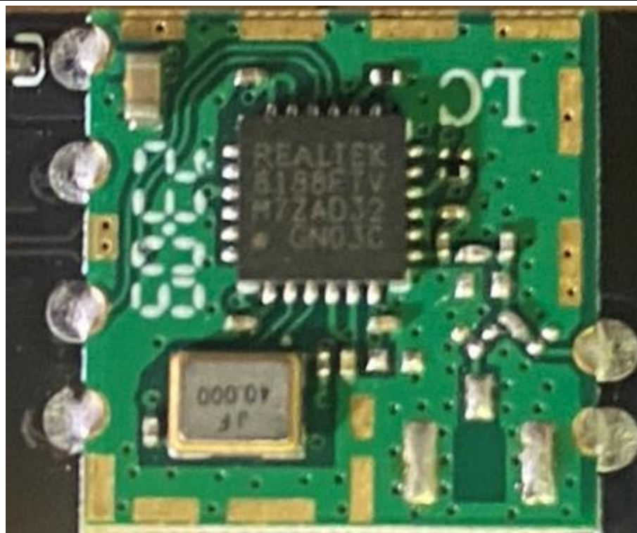
05. View of RFIC
