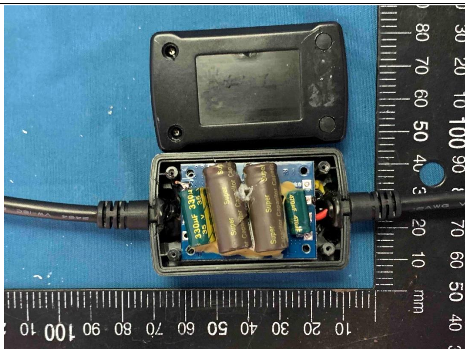
06. Inside View of Power Box
