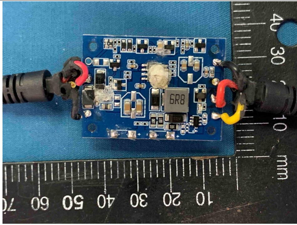
07. Front View of Power Box PCB
