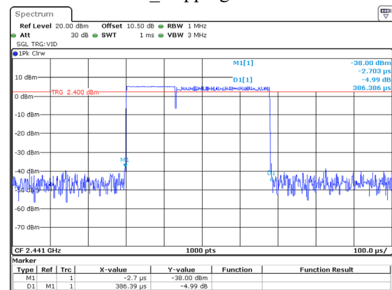
2DH1_Hopping 0.386ms
