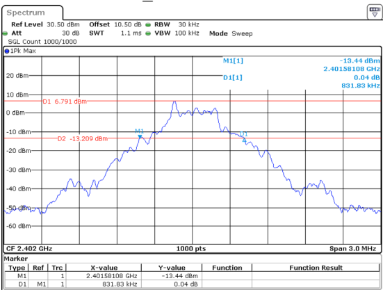
DH1_Low 0.832MHz
