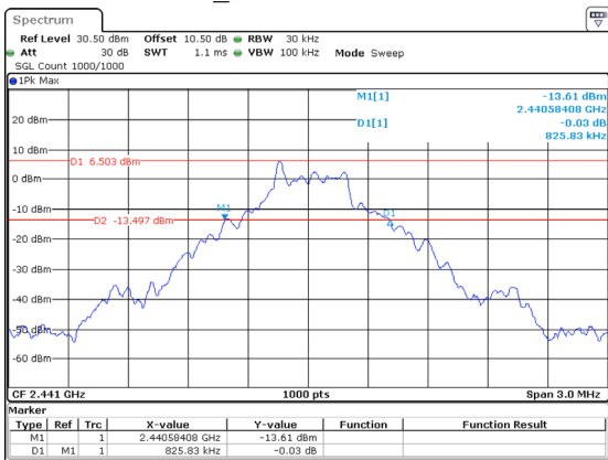
DH1_Middle 0.826MHz
