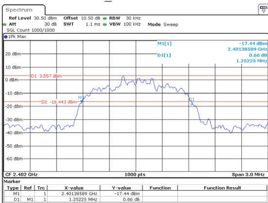
2DH1_Low 1.252MHz
