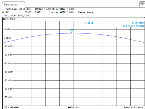
3DH1_High 5.76dBm
