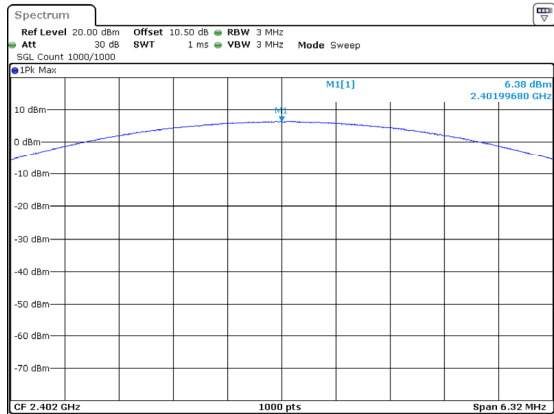
3DH1_Low 6.38dBm
