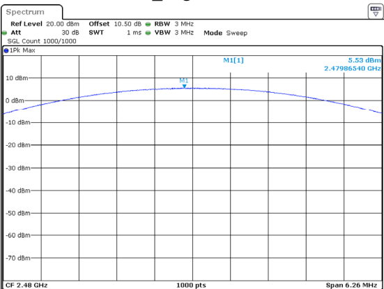
2DH1_High 5.53dBm
