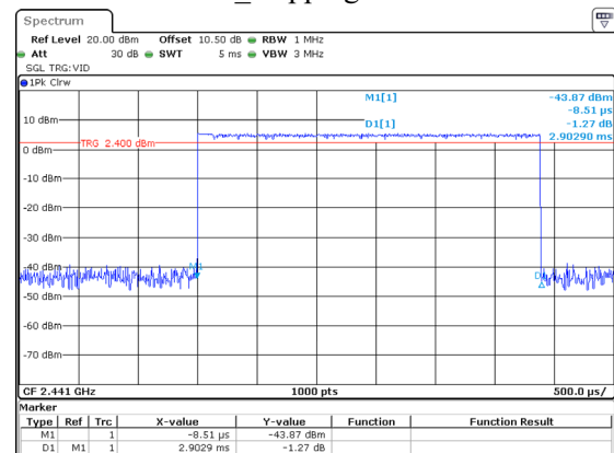
2DH5_Hopping 2.903ms
