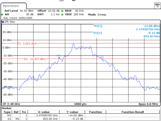
DH1_High 0.823MHz
