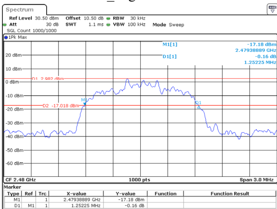
2DH1_High 1.252MHz
