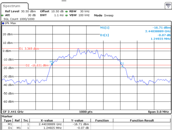
2DH1_Middle 1.249MHz
