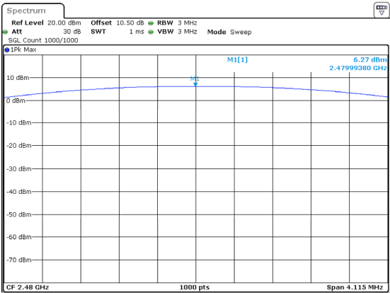
DH1_High 6.27dBm
