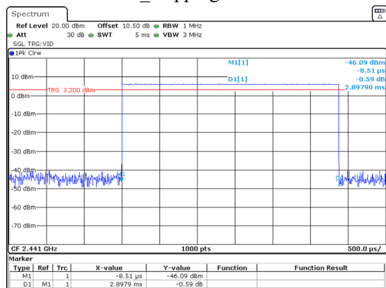
DH5_Hopping 2.898ms
