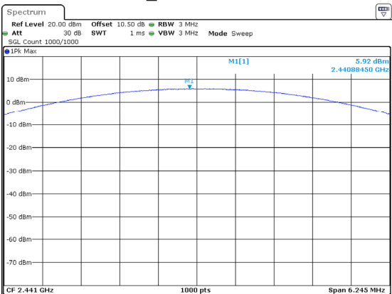
2DH1_Middle 5.92dBm
