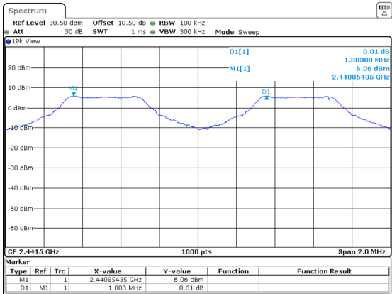
DH1_Middle 1.003MHz
