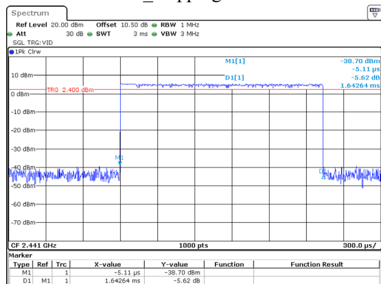
2DH3_Hopping 1.643ms
