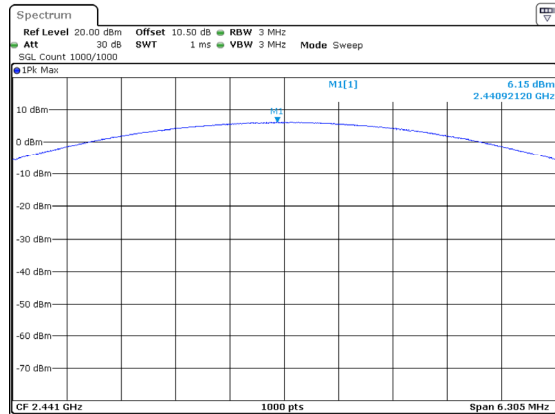
3DH1_Middle 6.15dBm
