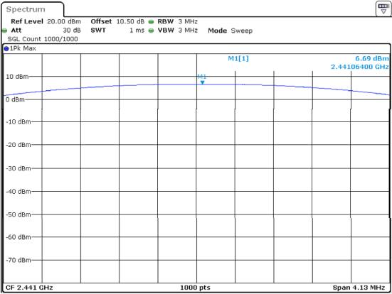
DH1_Middle 6.69dBm
