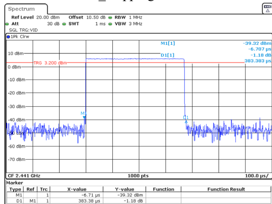
DH1_Hopping 0.383ms
