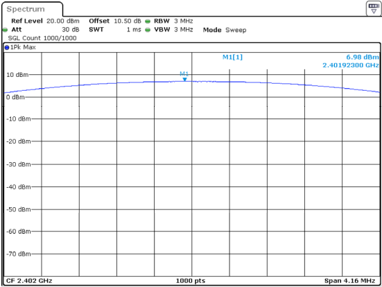
DH1_Low 6.98dBm
