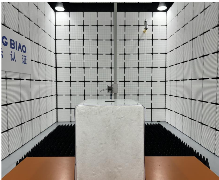
Radiated Emission Above 1GHz
