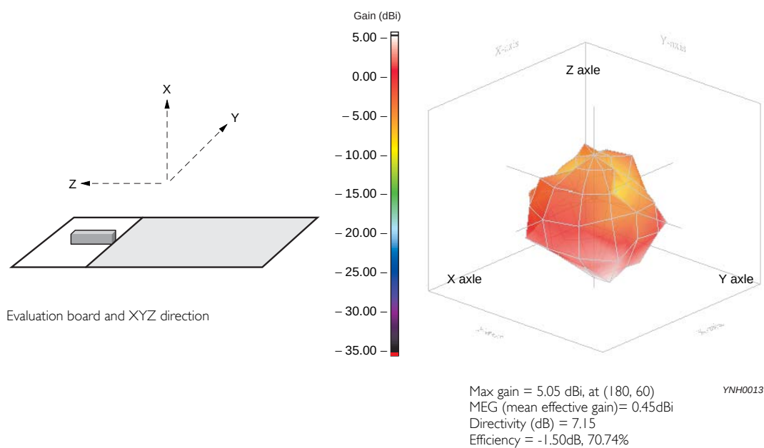
Fig. 5 Radiation pattern
