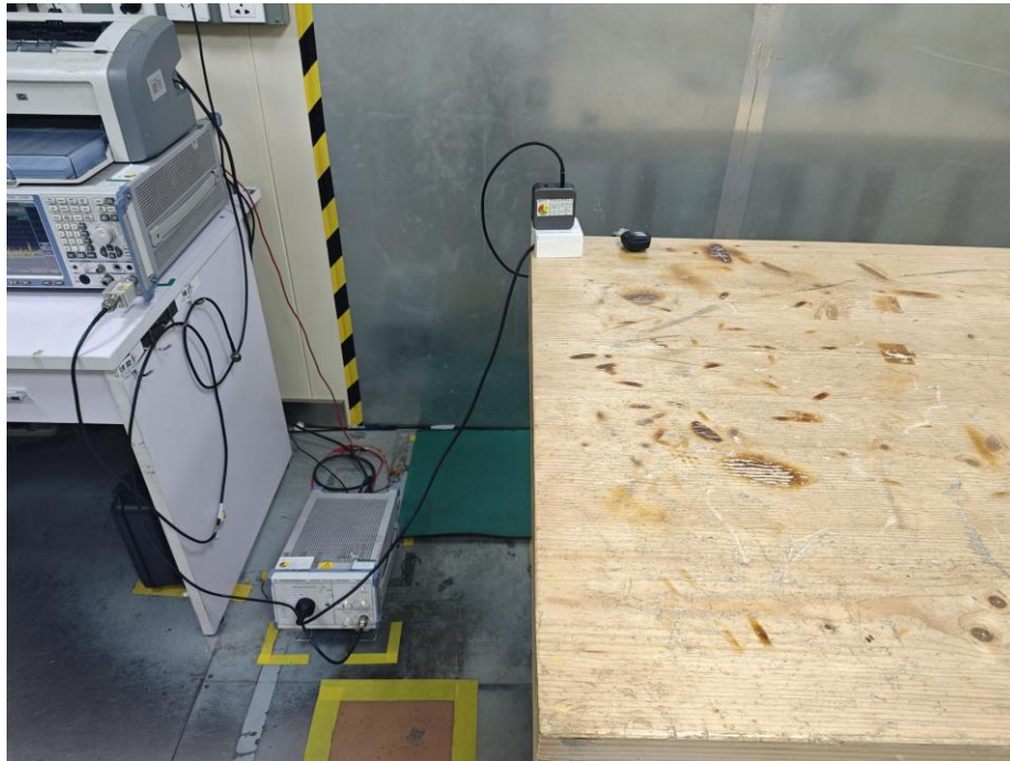
Conducted emissions
