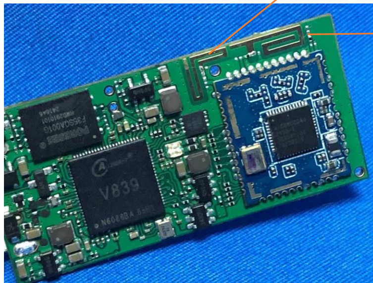
WIFI ANT
