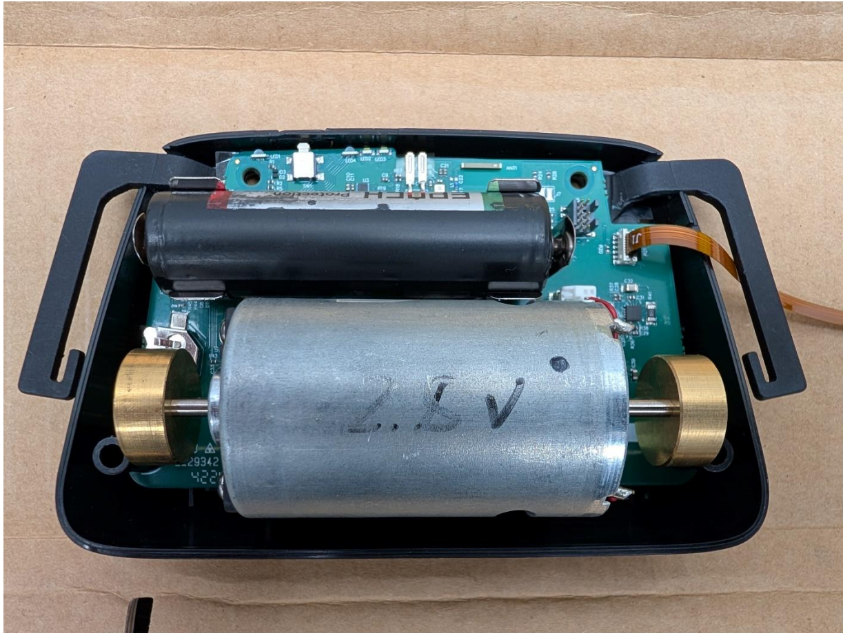
Close-Up of the MSP-09-2007 Vibration Pack
