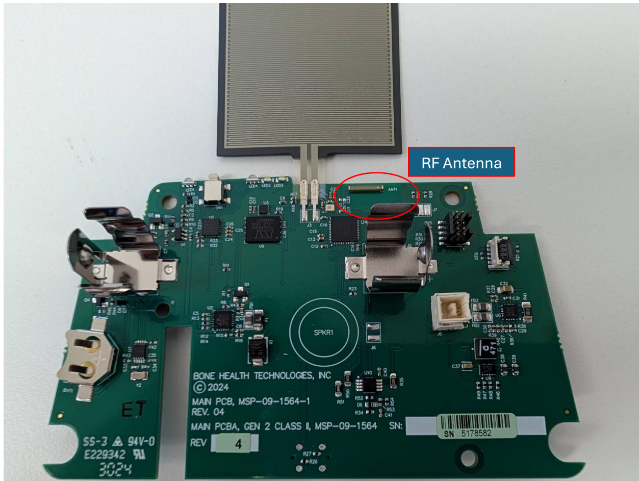
Front View of the MSP-09-1564 Main PCBA
