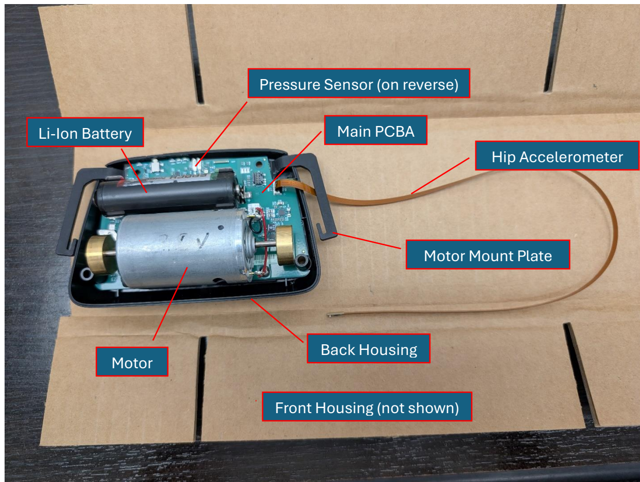
Open view of the MSP-09-2007 Vibration Pack
