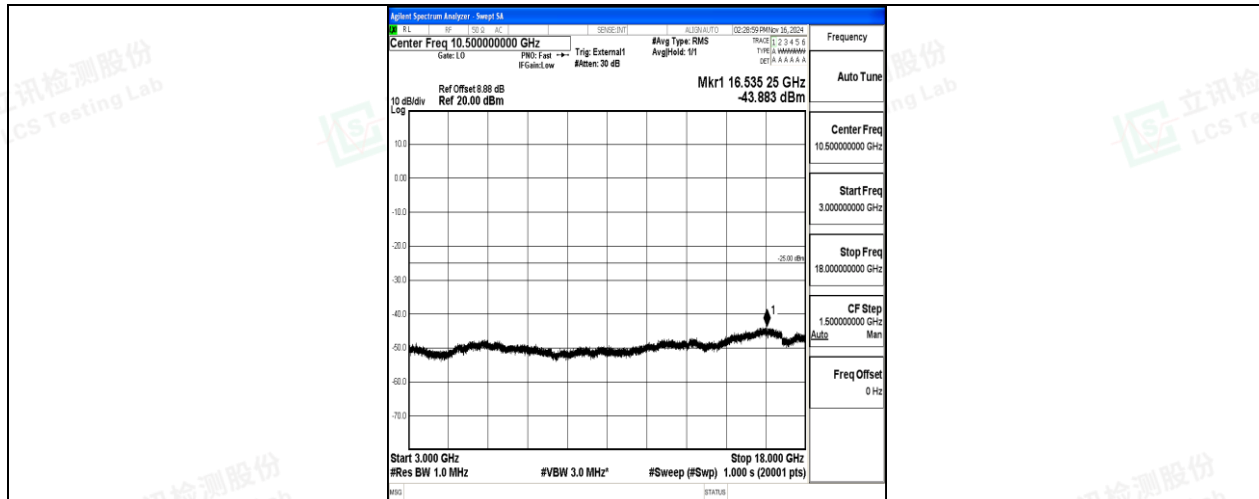
Band41-20MHz-16QAM-40620-1RB#0-3000~18000-PASS
