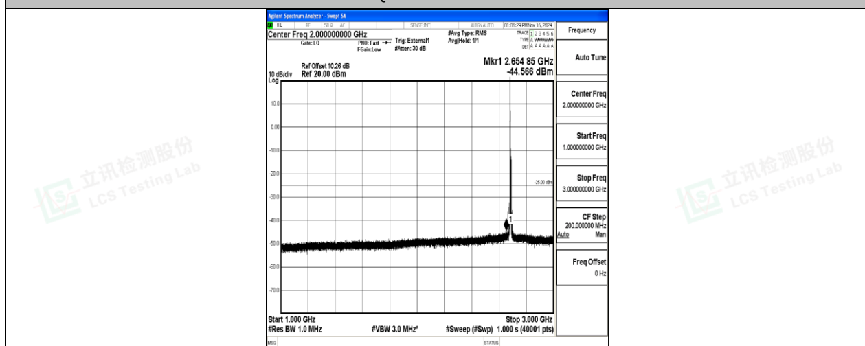
Band41-10MHz-16QAM-41540-1RB#0-1000~3000-PASS
