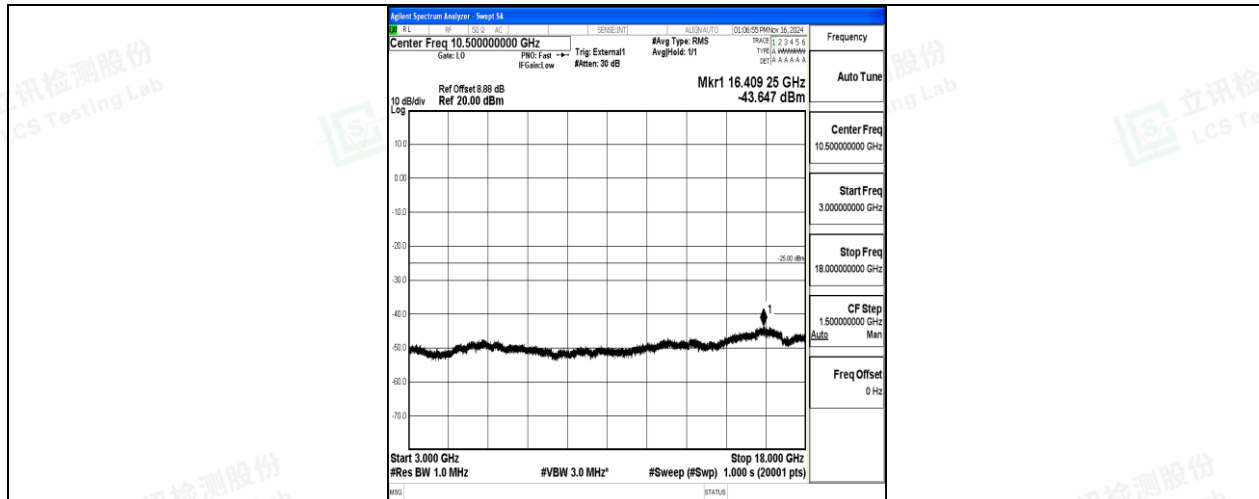
Band41-10MHz-16QAM-41540-1RB#0-3000~18000-PASS
