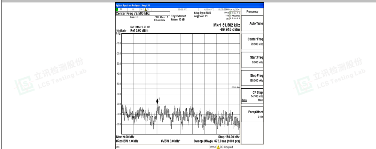
Band41-15MHz-16QAM-39725-1RB#0-0.009~0.15-PASS
