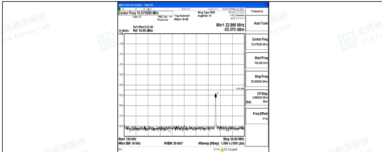
Band41-20MHz-QPSK-40620-1RB#0-0.15~30-PASS
