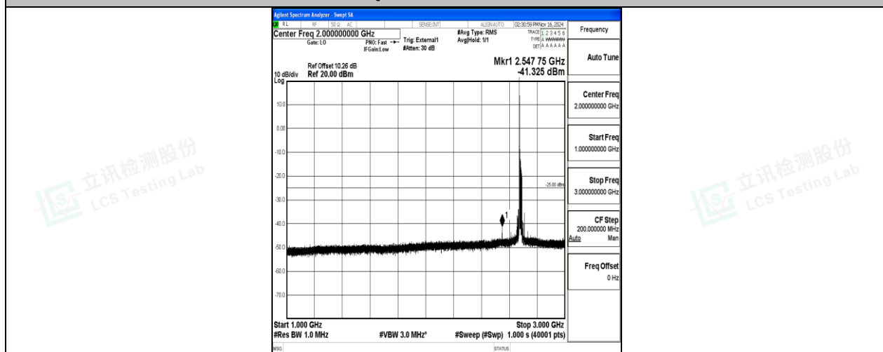
Band41-20MHz-QPSK-41490-1RB#0-1000~3000-PASS
