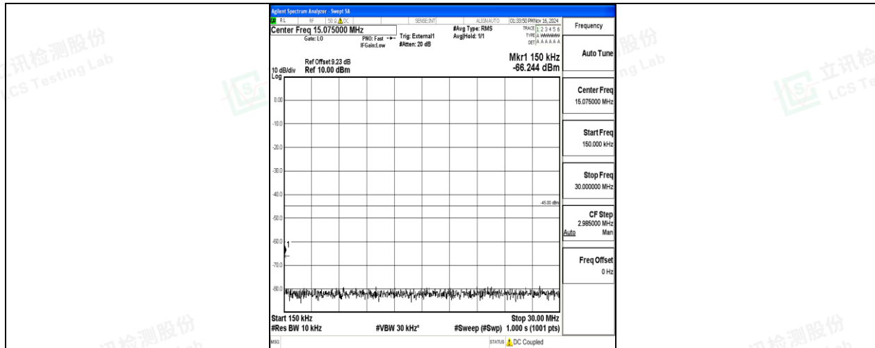
Band41-15MHz-QPSK-39725-1RB#0-0.15~30-PASS
