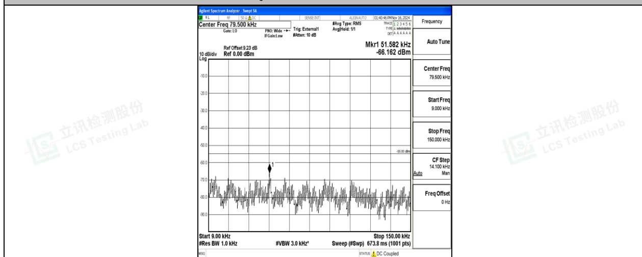
Band41-15MHz-16QAM-40620-1RB#0-0.009~0.15-PASS
