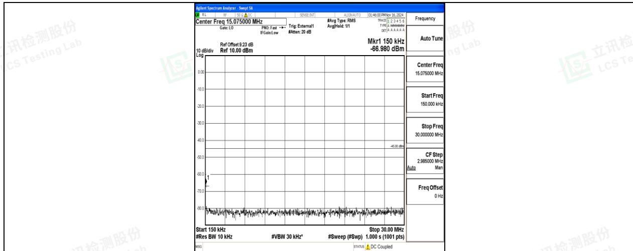
Band41-15MHz-16QAM-41515-1RB#0-0.15~30-PASS
