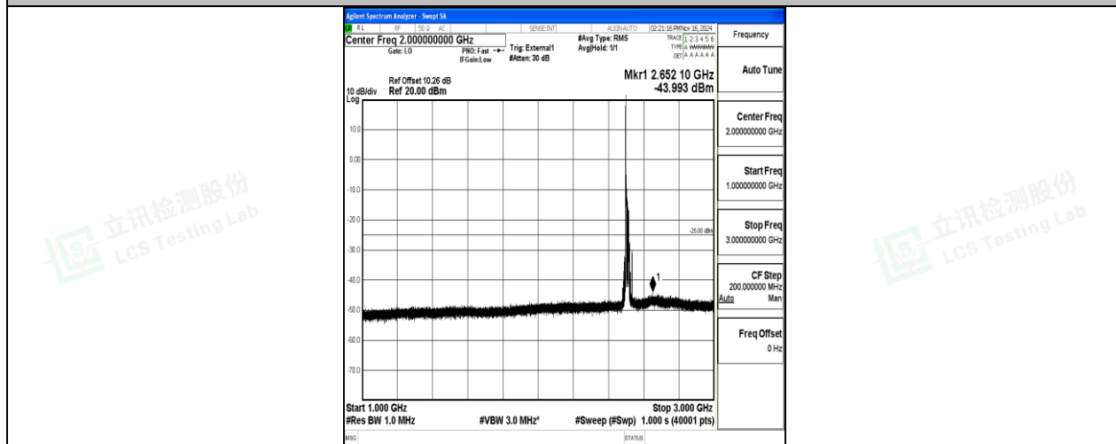
Band41-20MHz-QPSK-39750-1RB#0-1000~3000-PASS
