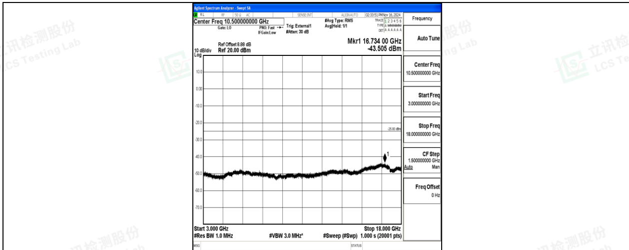
Band41-20MHz-16QAM-41490-1RB#0-3000~18000-PASS
