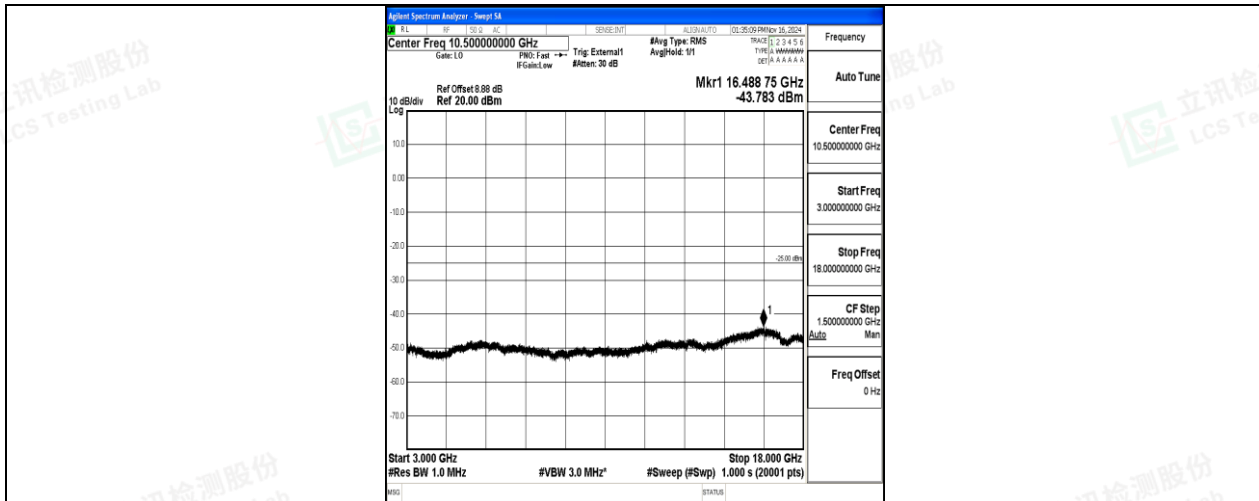
Band41-15MHz-QPSK-39725-1RB#0-3000~18000-PASS
