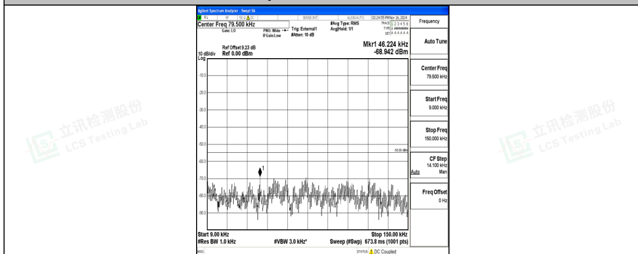
Band41-20MHz-QPSK-40620-1RB#0-0.009~0.15-PASS
