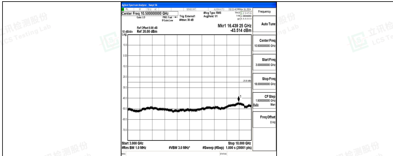
Band41-20MHz-QPSK-39750-1RB#0-3000~18000-PASS
