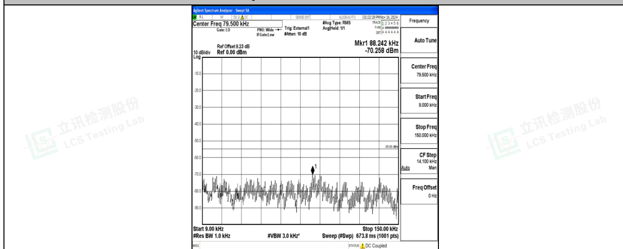
Band41-20MHz-16QAM-39750-1RB#0-0.009~0.15-PASS
