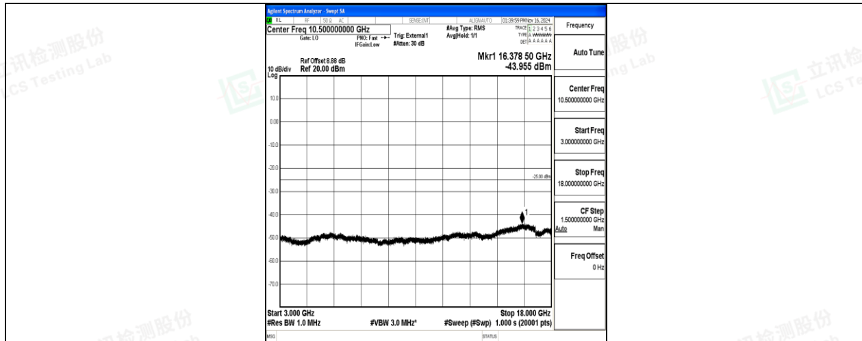
Band41-15MHz-QPSK-40620-1RB#0-3000~18000-PASS
