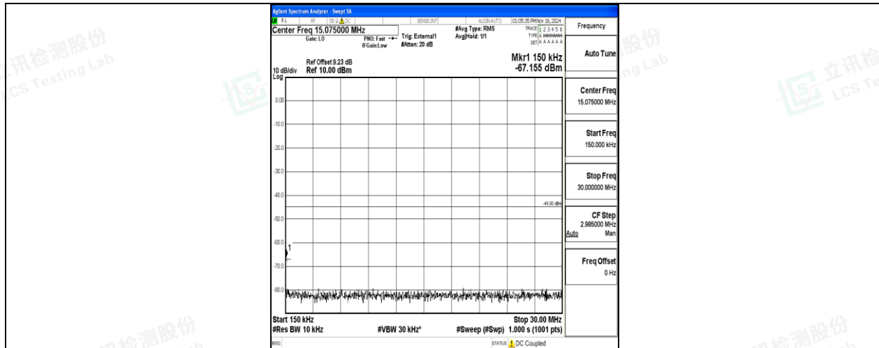
Band41-10MHz-16QAM-41540-1RB#0-0.15~30-PASS
