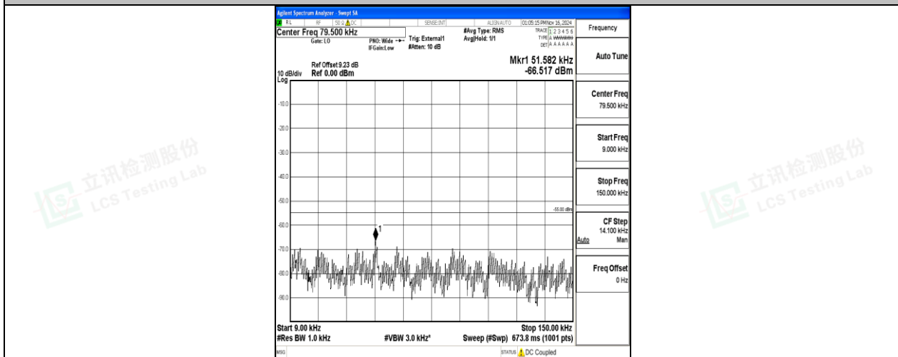
Band41-10MHz-16QAM-41540-1RB#0-0.009~0.15-PASS
