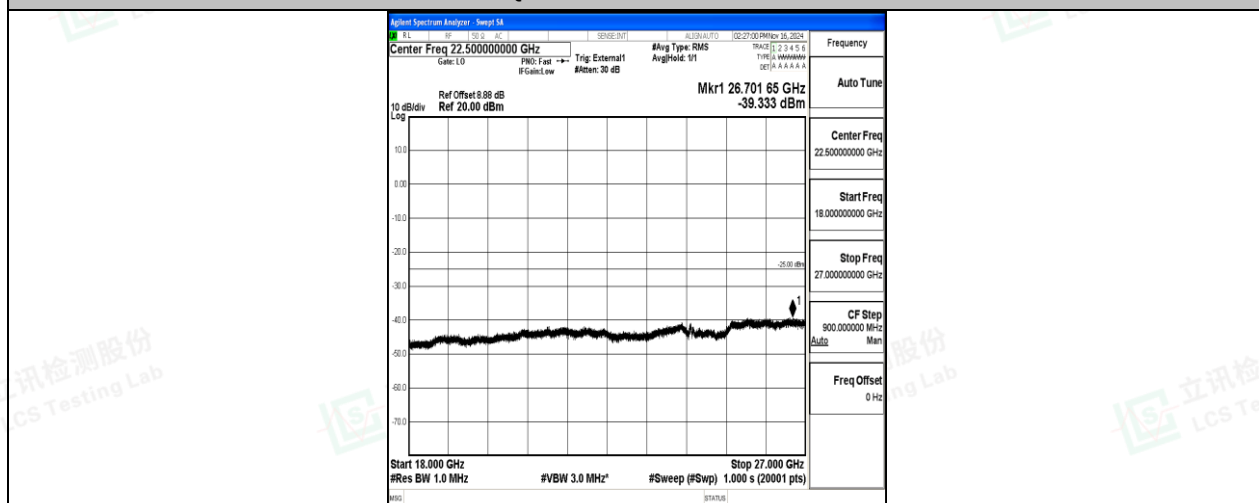
Band41-20MHz-QPSK-40620-1RB#0-18000~27000-PASS
