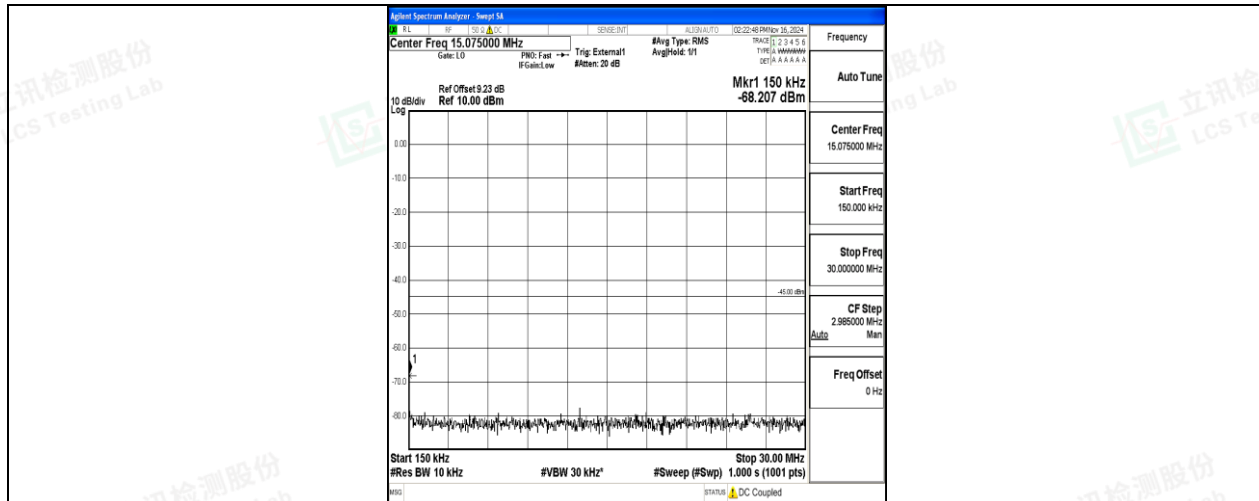
Band41-20MHz-16QAM-39750-1RB#0-0.15~30-PASS
