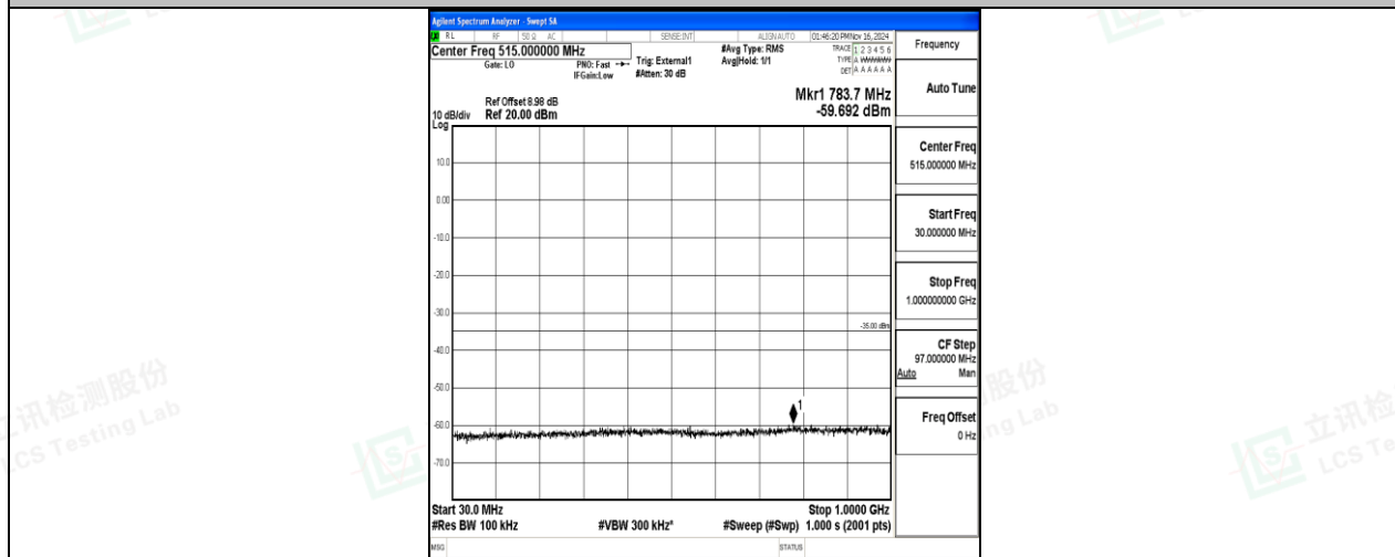
Band41-15MHz-16QAM-41515-1RB#0-30~1000-PASS
