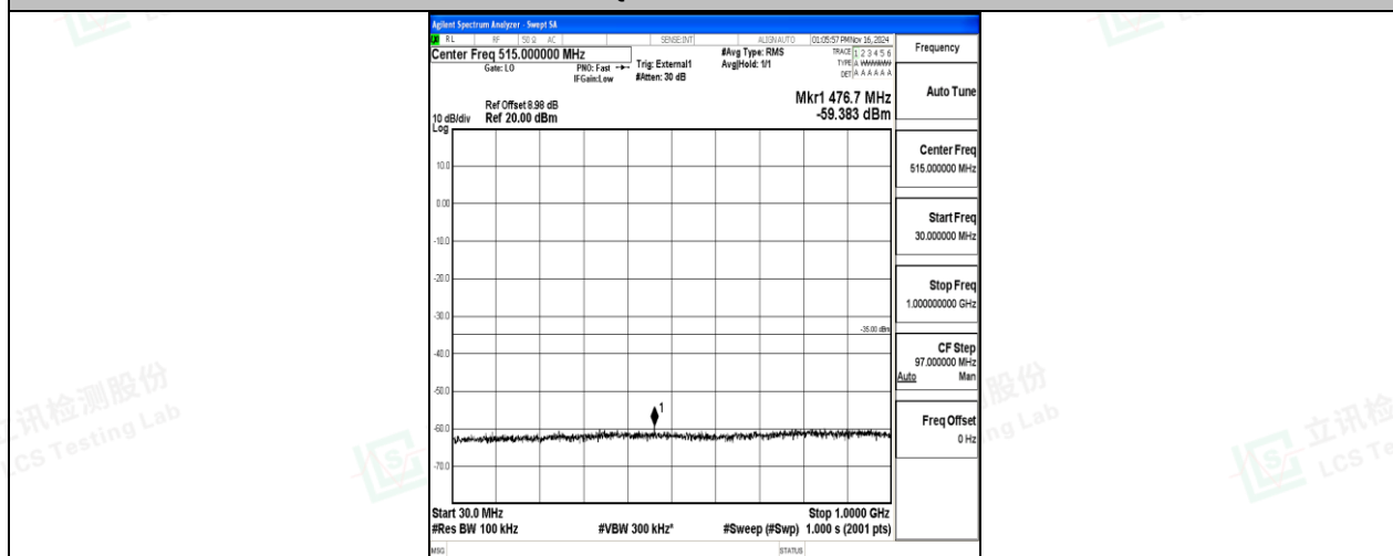
Band41-10MHz-16QAM-41540-1RB#0-30~1000-PASS
