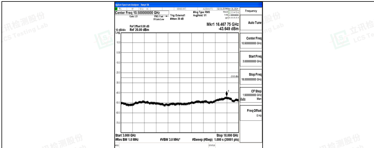
Band41-20MHz-QPSK-41490-1RB#0-3000~18000-PASS
