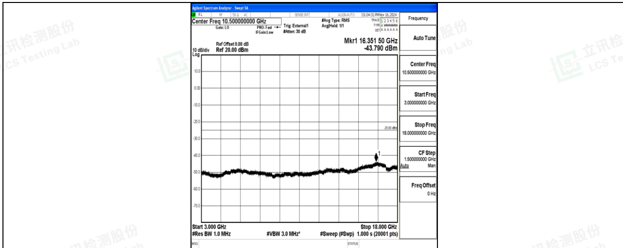
Band41-10MHz-QPSK-41540-1RB#0-3000~18000-PASS
