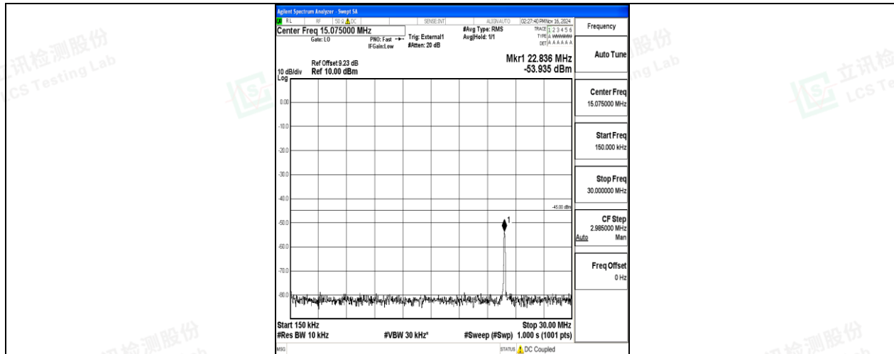
Band41-20MHz-16QAM-40620-1RB#0-0.15~30-PASS
