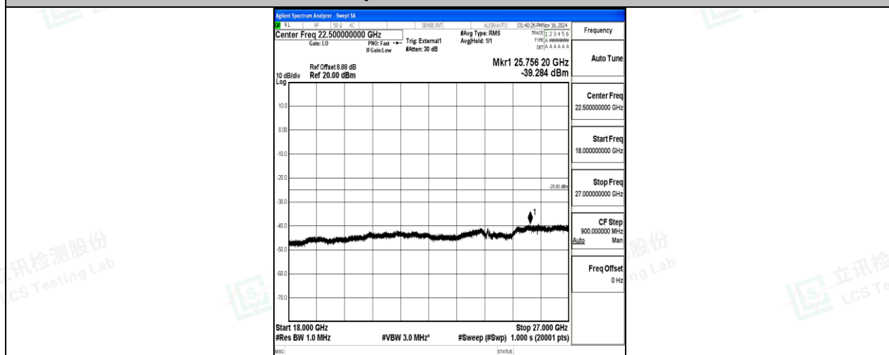
Band41-15MHz-QPSK-40620-1RB#0-18000~27000-PASS
