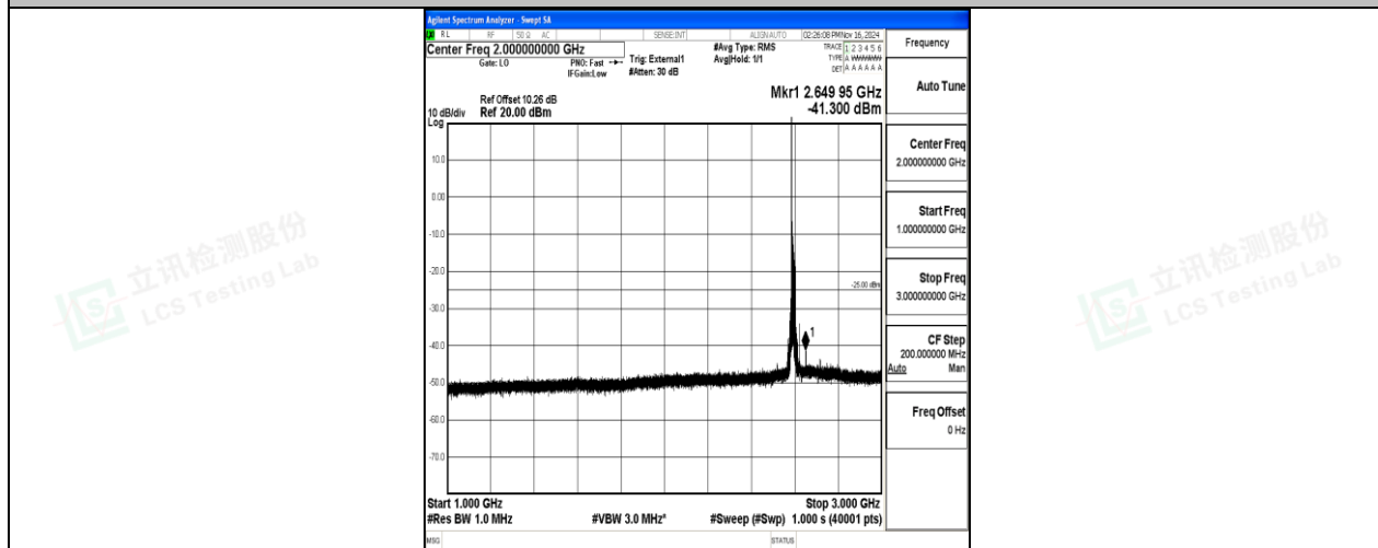
Band41-20MHz-QPSK-40620-1RB#0-1000~3000-PASS
