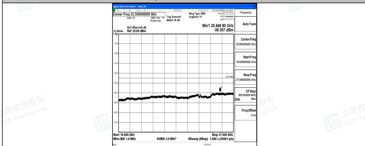
Band41-20MHz-16QAM-40620-1RB#0-18000~27000-PASS
