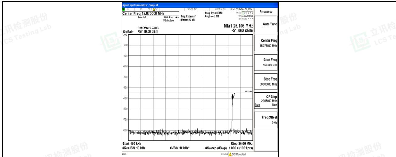
Band41-15MHz-16QAM-40620-1RB#0-0.15~30-PASS
