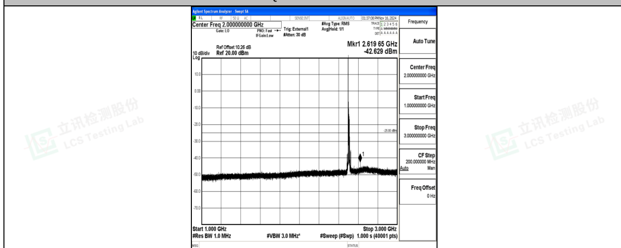
Band41-15MHz-16QAM-39725-1RB#0-1000~3000-PASS
