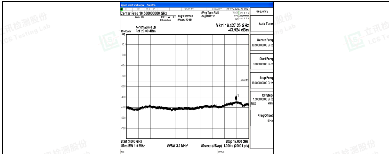
Band41-15MHz-16QAM-39725-1RB#0-3000~18000-PASS
