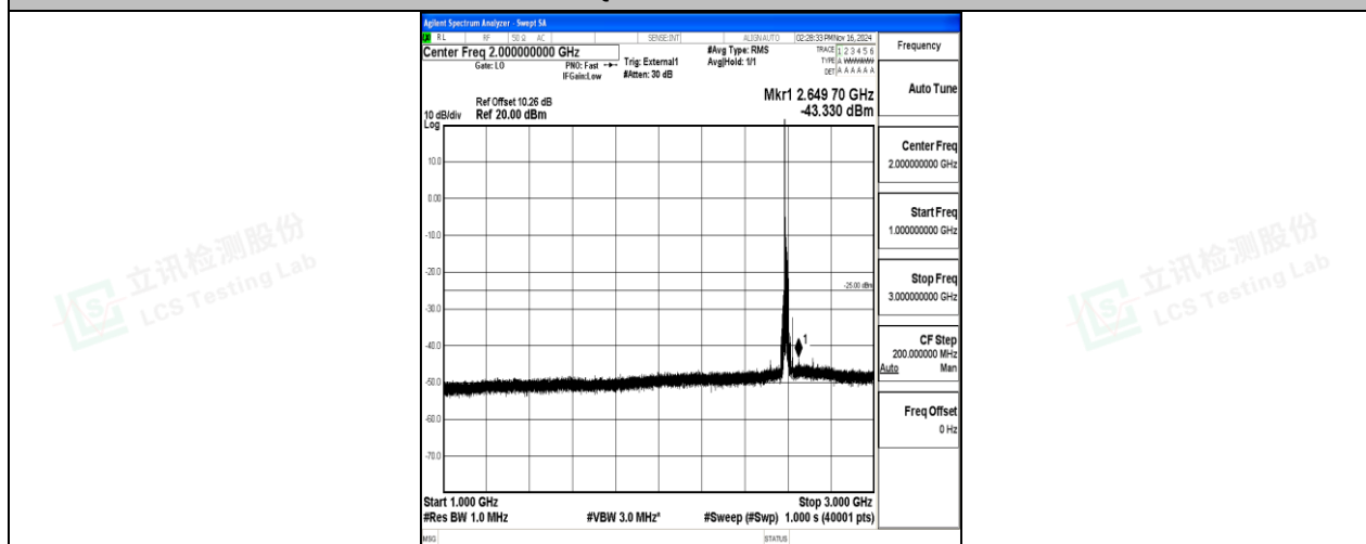
Band41-20MHz-16QAM-40620-1RB#0-1000~3000-PASS
