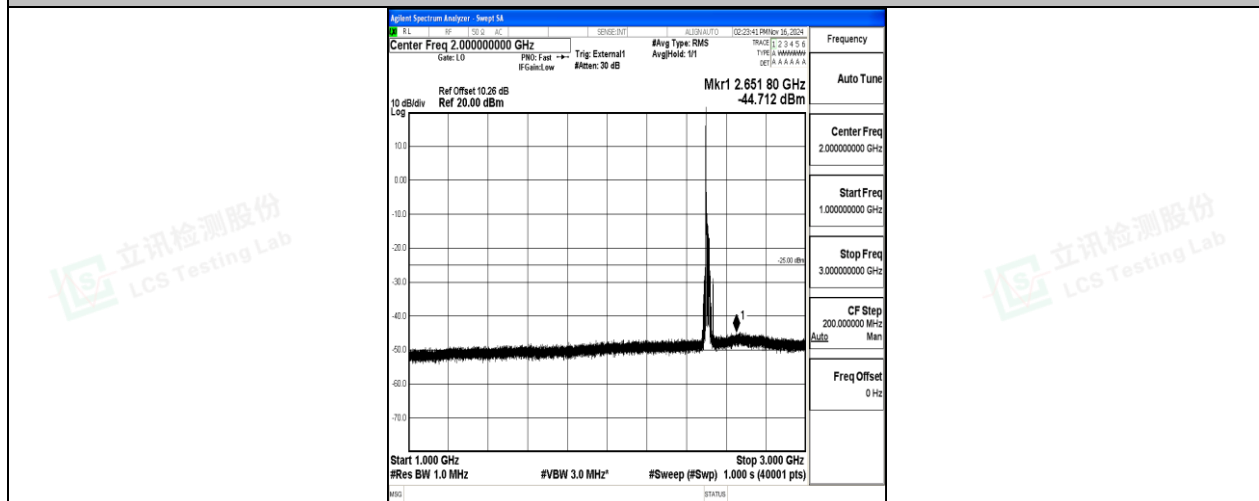
Band41-20MHz-16QAM-39750-1RB#0-1000~3000-PASS
