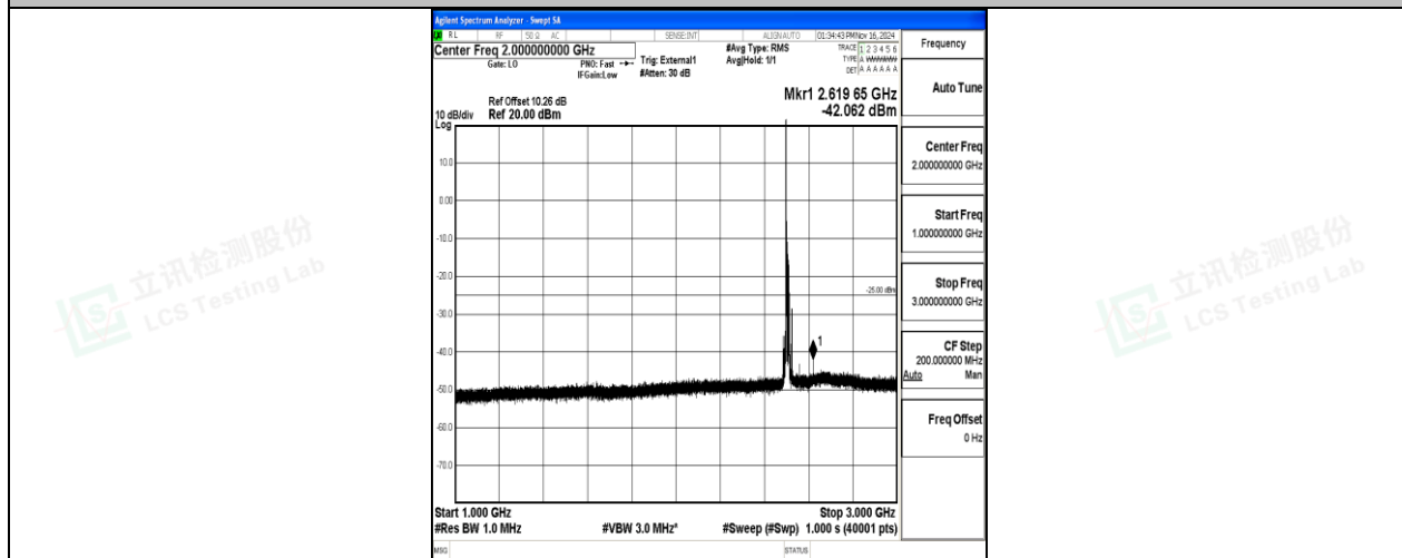
Band41-15MHz-QPSK-39725-1RB#0-1000~3000-PASS
