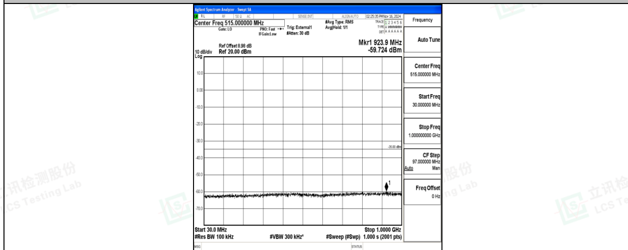
Band41-20MHz-QPSK-40620-1RB#0-30~1000-PASS
