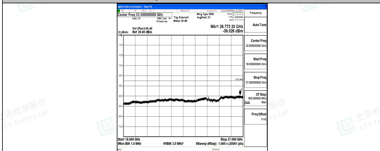
Band41-20MHz-QPSK-39750-1RB#0-18000~27000-PASS
