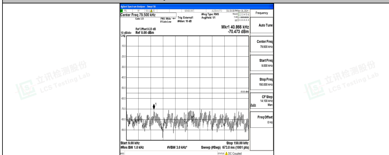
Band41-15MHz-QPSK-39725-1RB#0-0.009~0.15-PASS
