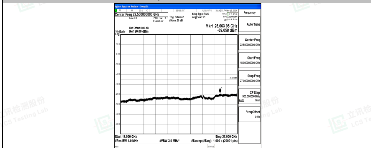
Band41-15MHz-16QAM-40620-1RB#0-18000~27000-PASS
