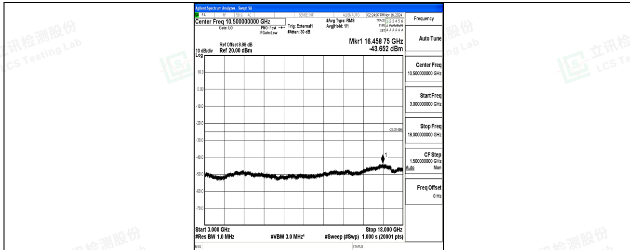
Band41-20MHz-16QAM-39750-1RB#0-3000~18000-PASS
