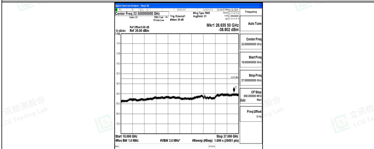
Band41-10MHz-QPSK-41540-1RB#0-18000~27000-PASS
