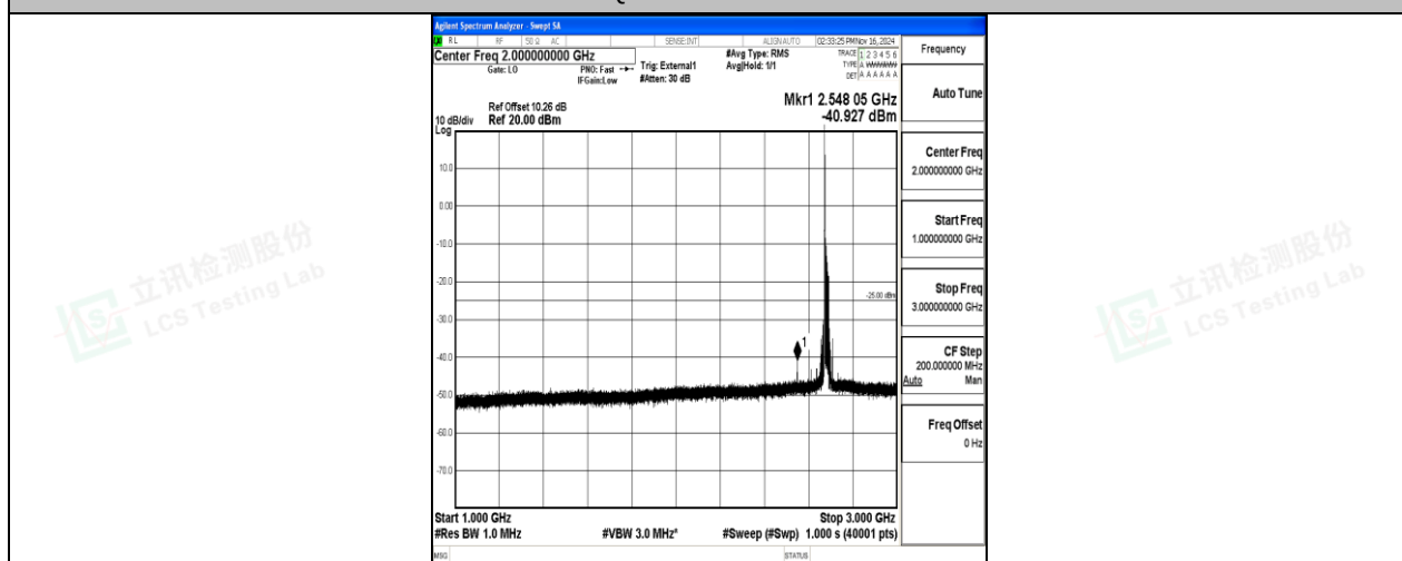
Band41-20MHz-16QAM-41490-1RB#0-1000~3000-PASS
