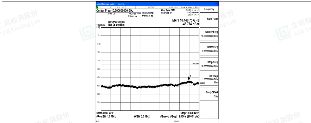
Band41-15MHz-QPSK-41515-1RB#0-3000~18000-PASS
