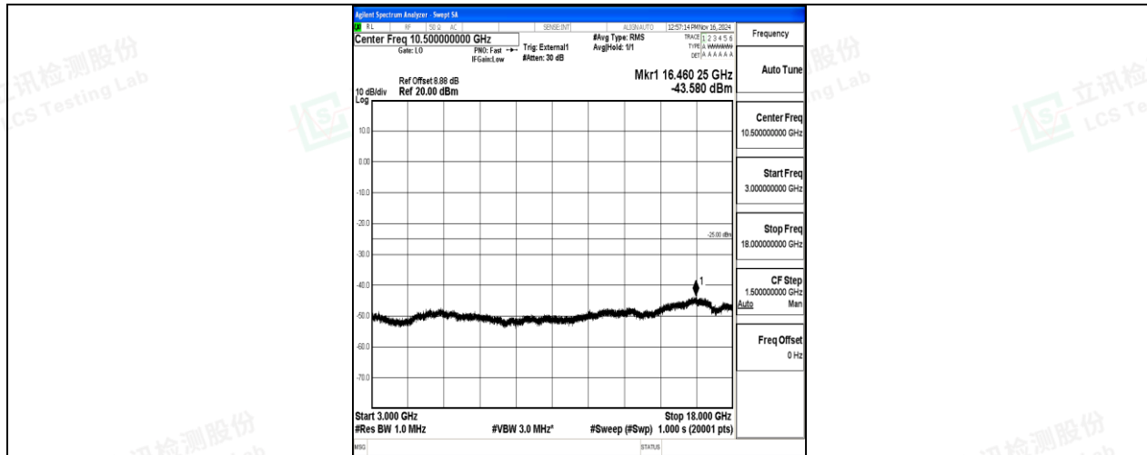
Band41-10MHz-16QAM-39700-1RB#0-3000~18000-PASS
