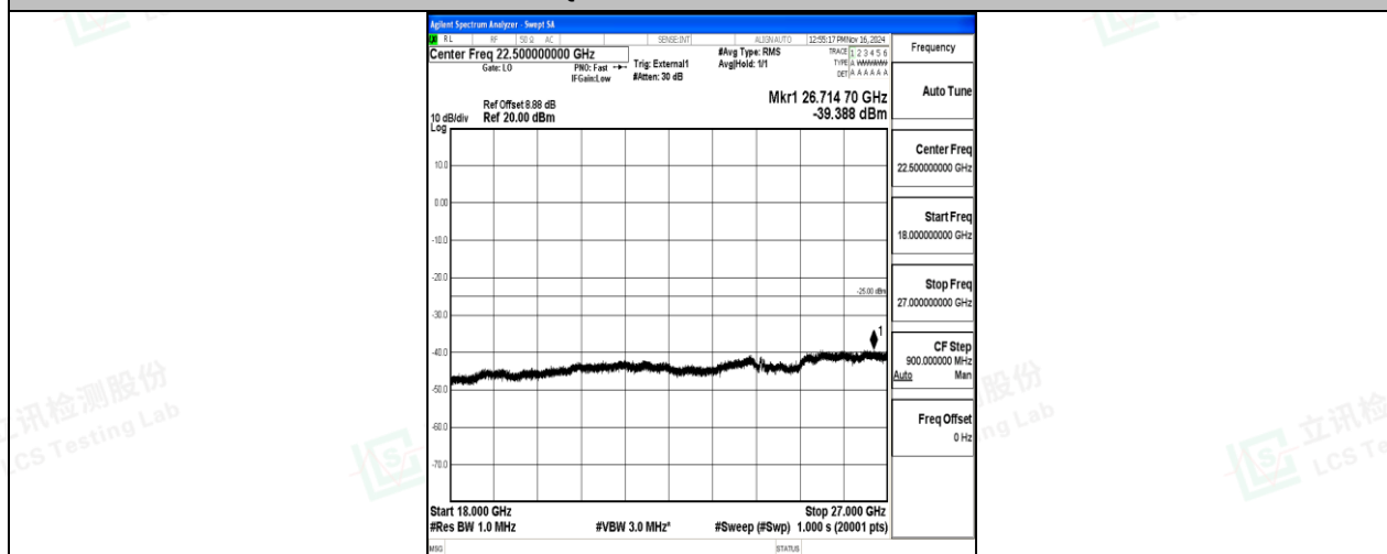
Band41-10MHz-QPSK-39700-1RB#0-18000~27000-PASS
