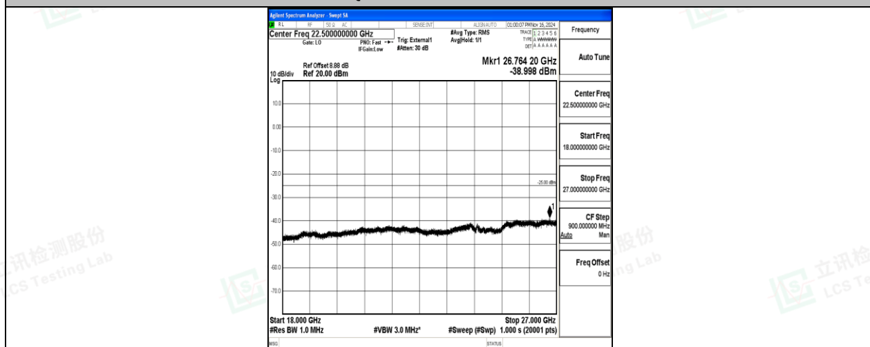
Band41-10MHz-QPSK-40620-1RB#0-18000~27000-PASS
