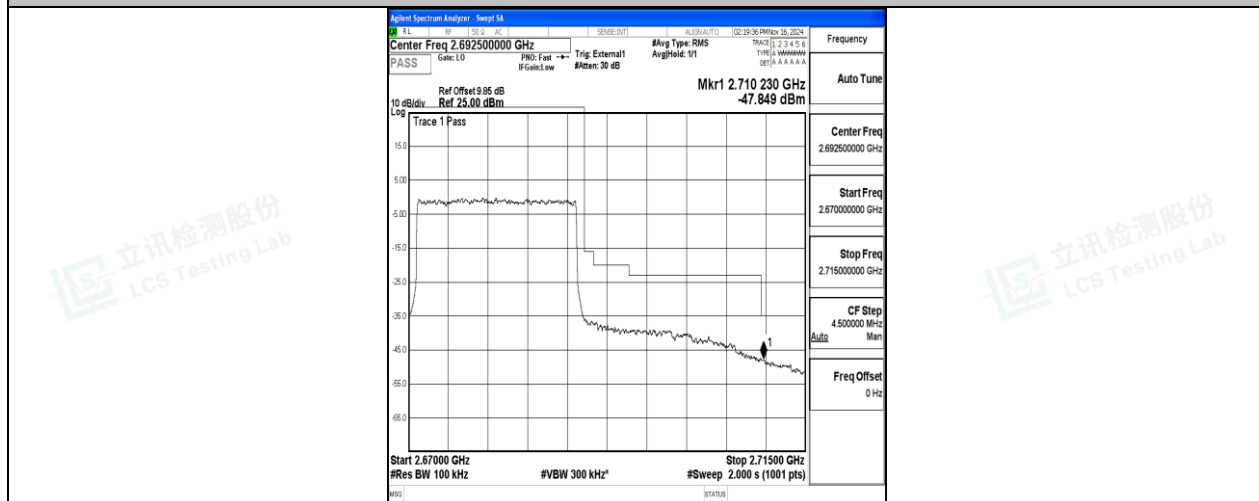
Band41-20MHz-16QAM-41490-100RB#0-PASS
