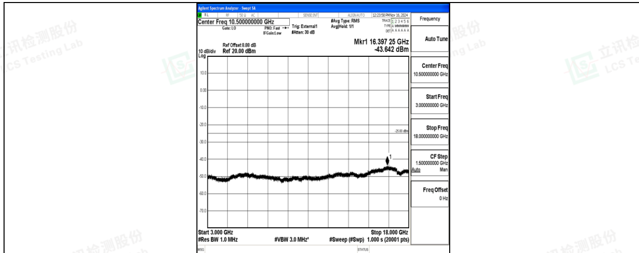
Band41-5MHz-16QAM-40620-1RB#0-3000~18000-PASS
