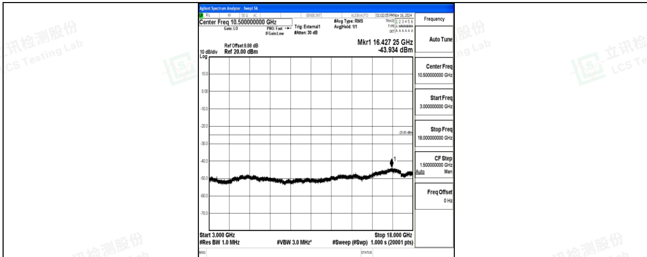
Band41-10MHz-16QAM-40620-1RB#0-3000~18000-PASS
