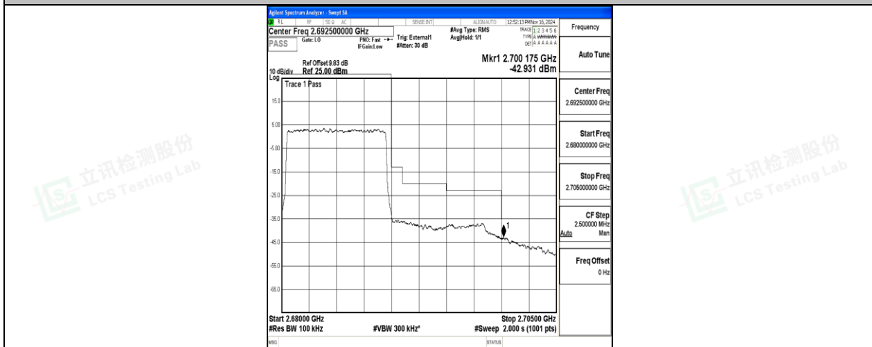
Band41-10MHz-QPSK-41540-50RB#0-PASS
