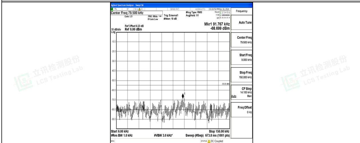
Band41-10MHz-QPSK-41540-1RB#0-0.009~0.15-PASS
