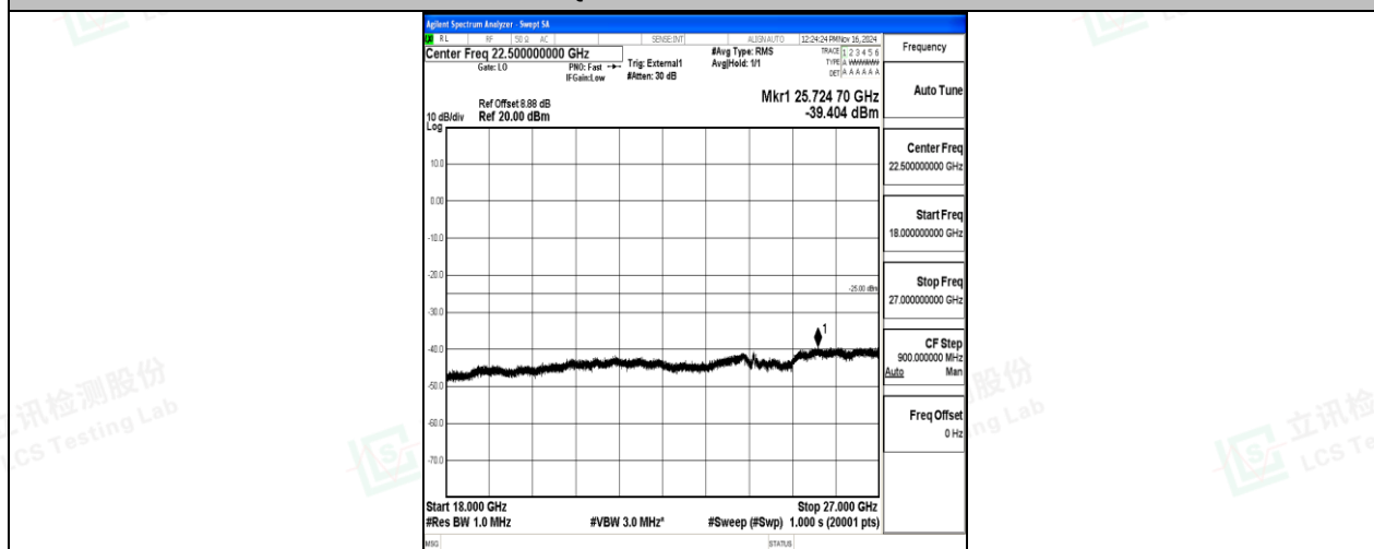
Band41-5MHz-16QAM-40620-1RB#0-18000~27000-PASS
