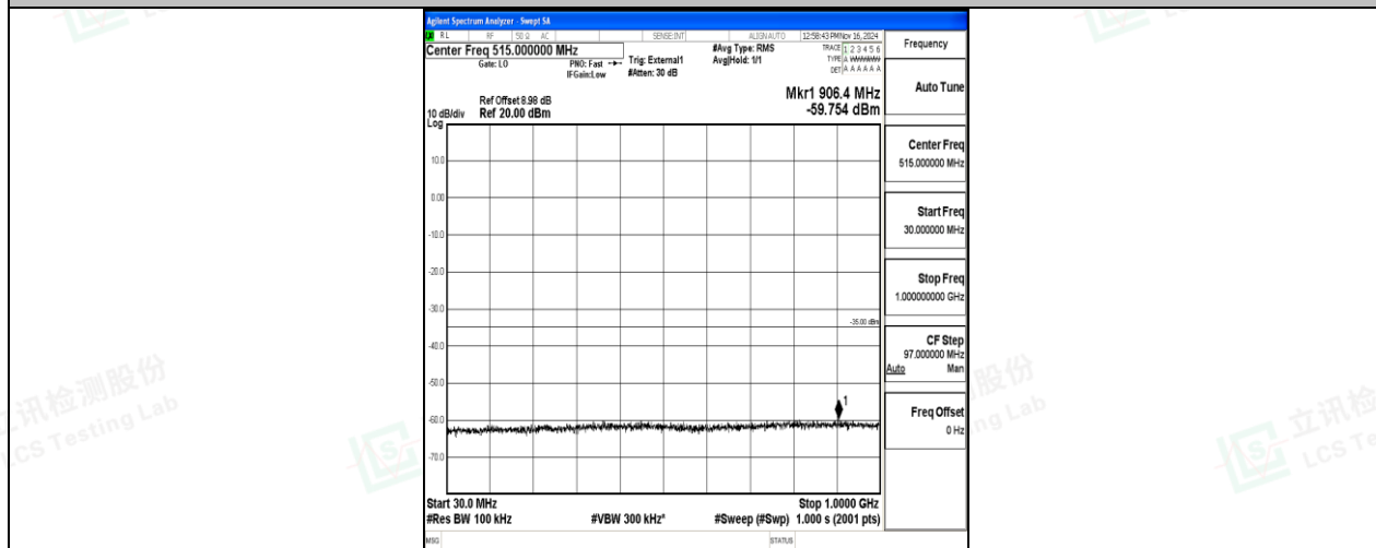
Band41-10MHz-QPSK-40620-1RB#0-30~1000-PASS
