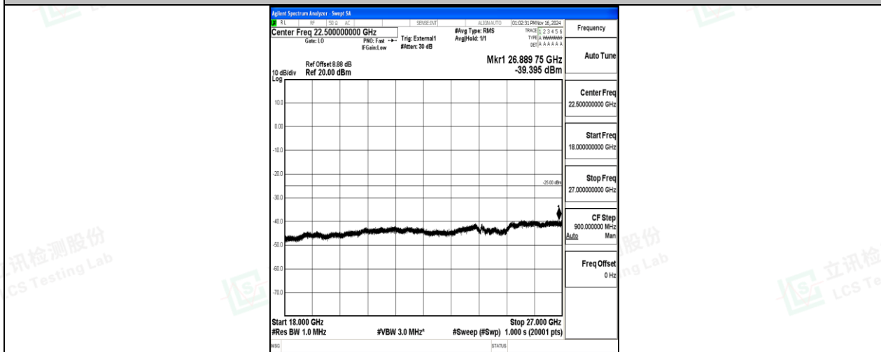
Band41-10MHz-16QAM-40620-1RB#0-18000~27000-PASS
