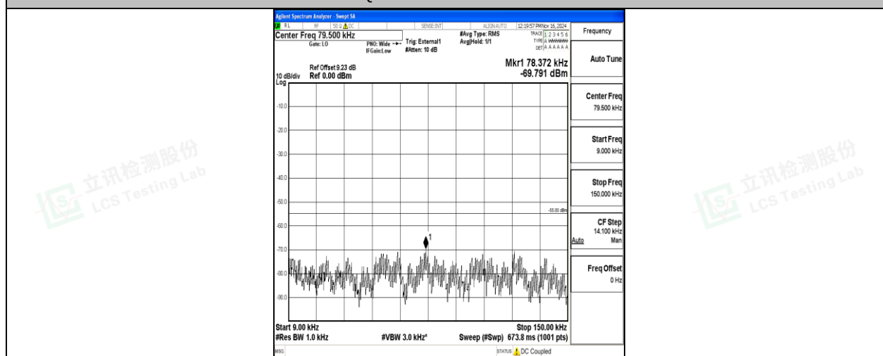
Band41-5MHz-OPSK-40620-1RB#0-0.009~0.15-PASS
