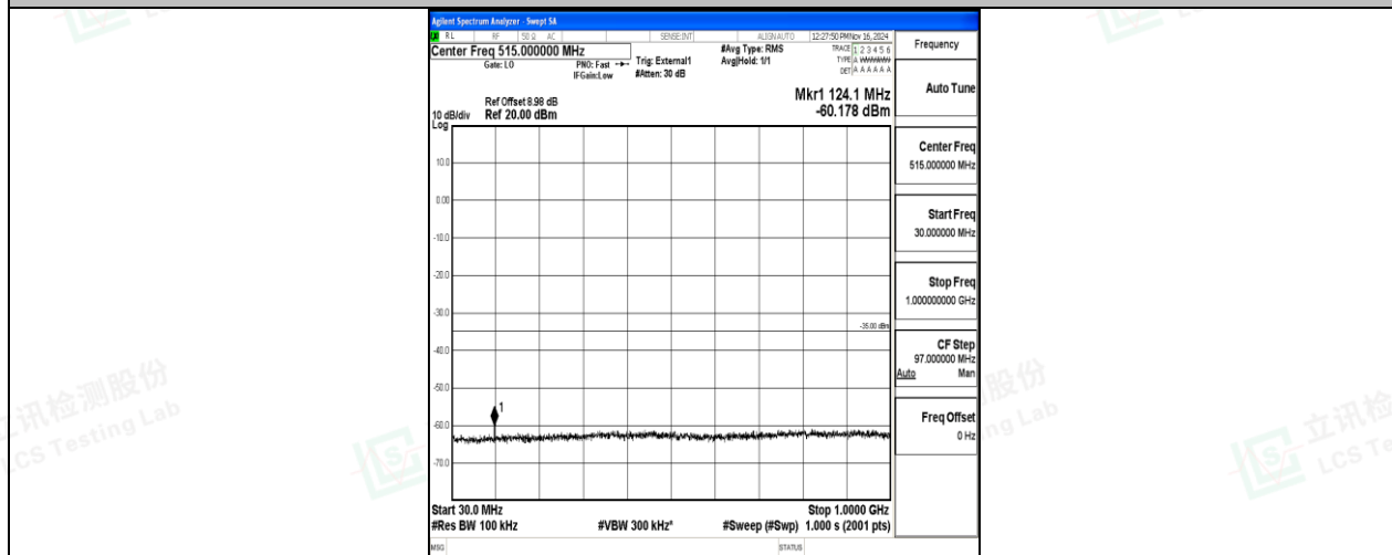
Band41-5MHz-16QAM-41565-1RB#0-30~1000-PASS
