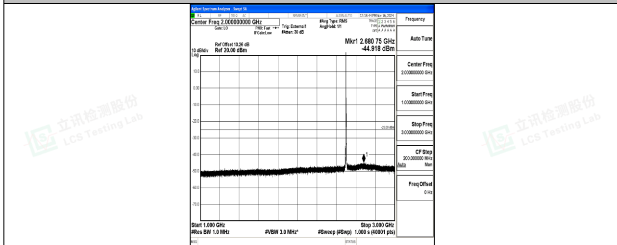
Band41-5MHz-16QAM-39675-1RB#0-1000~3000-PASS
