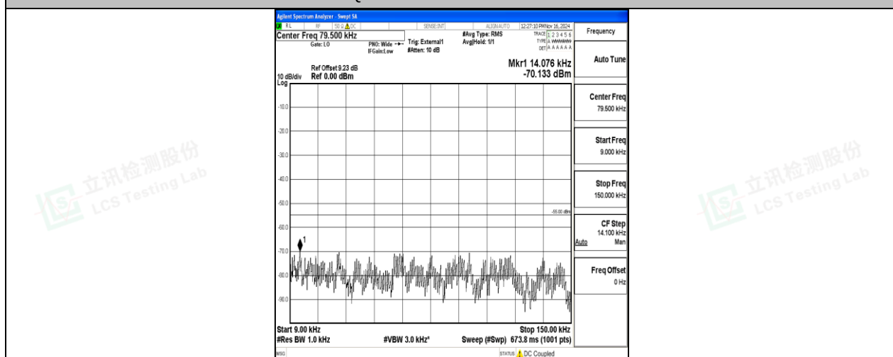
Band41-5MHz-16QAM-41565-1RB#0-0.009~0.15-PASS
