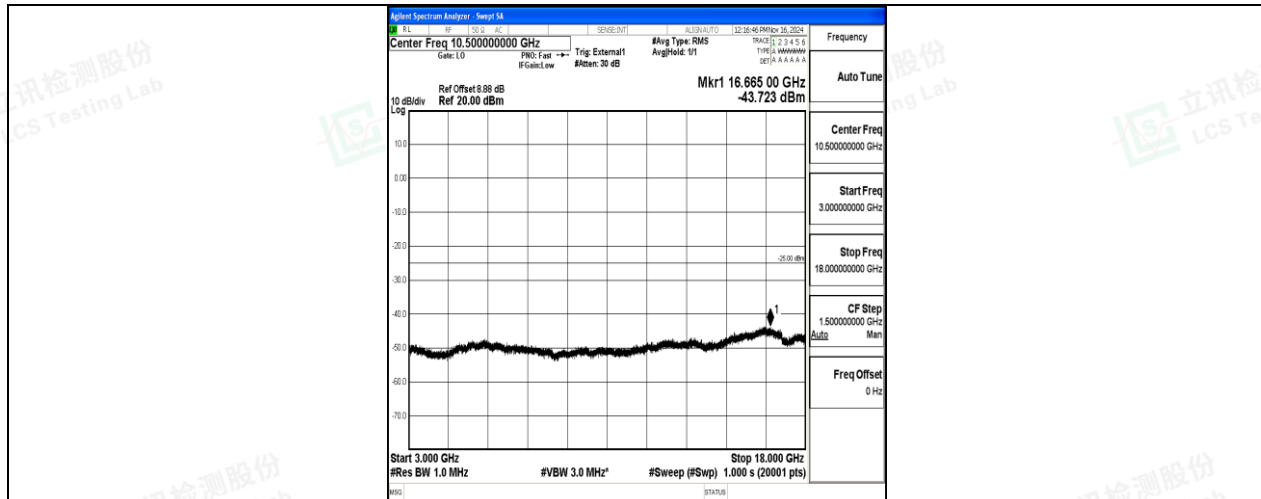
Band41-5MHz-QPSK-39675-1RB#0-3000~18000-PASS
