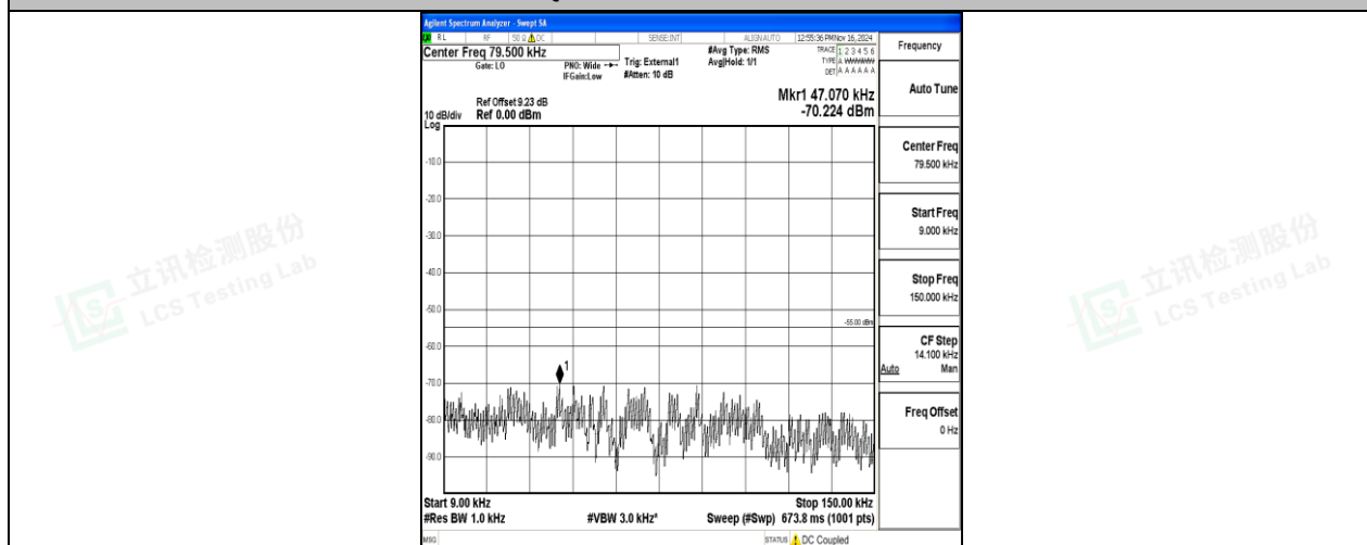
Band41-10MHz-16QAM-39700-1RB#0-0.009~0.15-PASS
