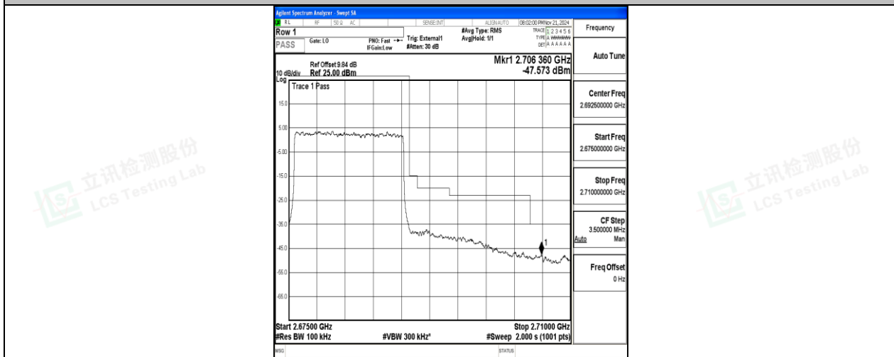
Band41-15MHz-16QAM-41515-75RB#0-PASS
