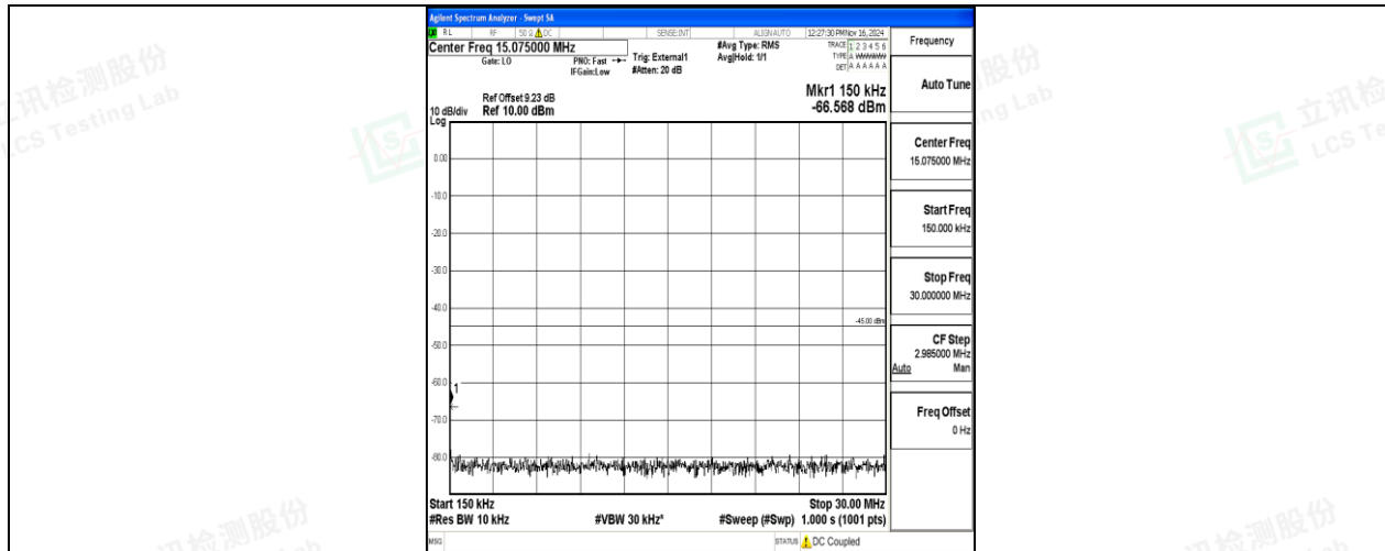
Band41-5MHz-16QAM-41565-1RB#0-0.15~30-PASS
