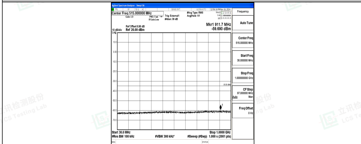
Band41-10MHz-16QAM-39700-1RB#0-30~1000-PASS
