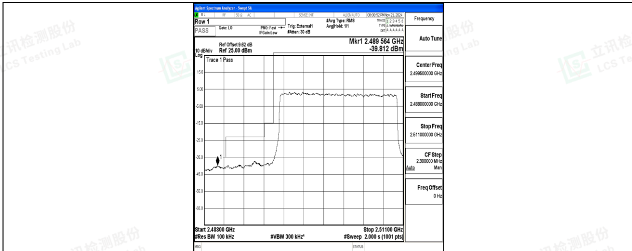
Band41-15MHz-16QAM-39725-75RB#0-PASS
