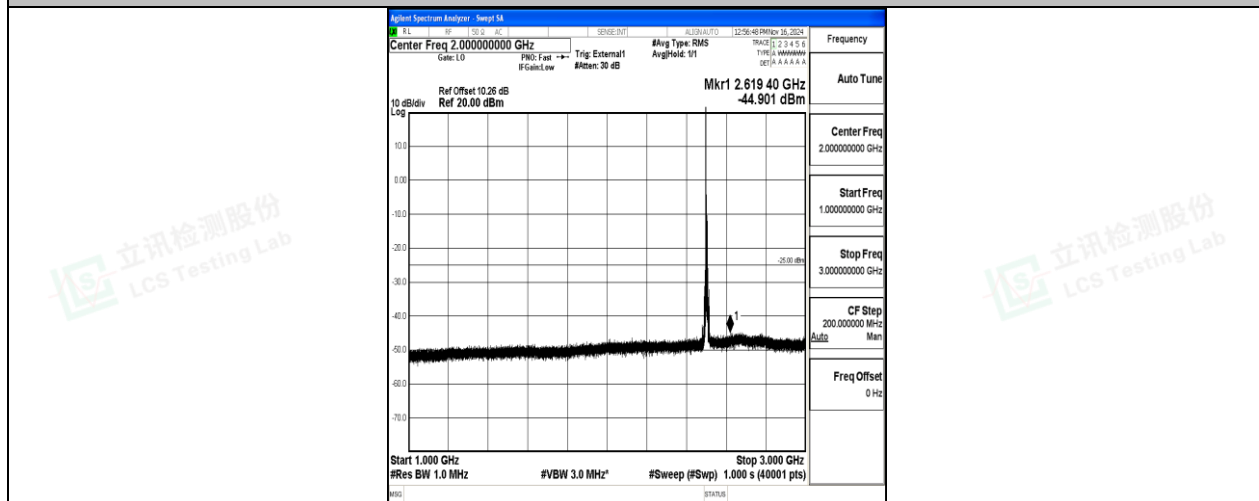
Band41-10MHz-16QAM-39700-1RB#0-1000~3000-PASS
