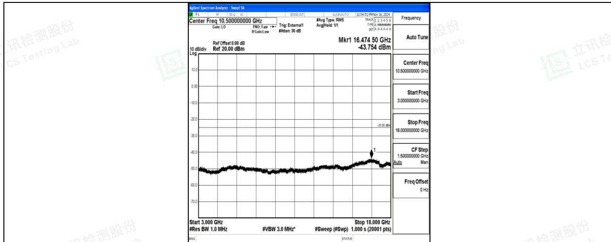
Band41-10MHz-QPSK-39700-1RB#0-3000~18000-PASS
