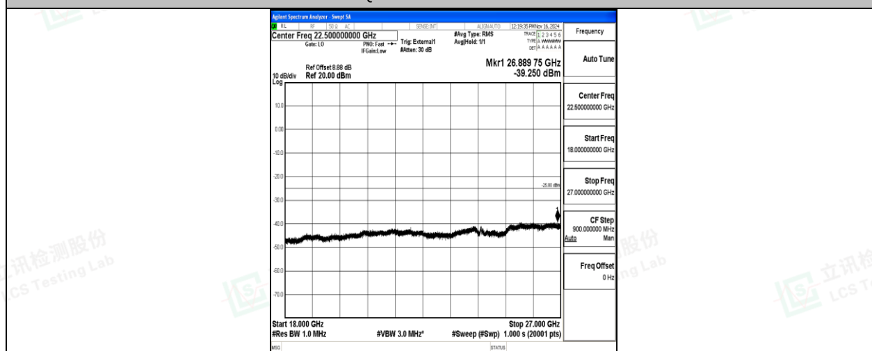
Band41-5MHz-16QAM-39675-1RB#0-18000~27000-PASS
