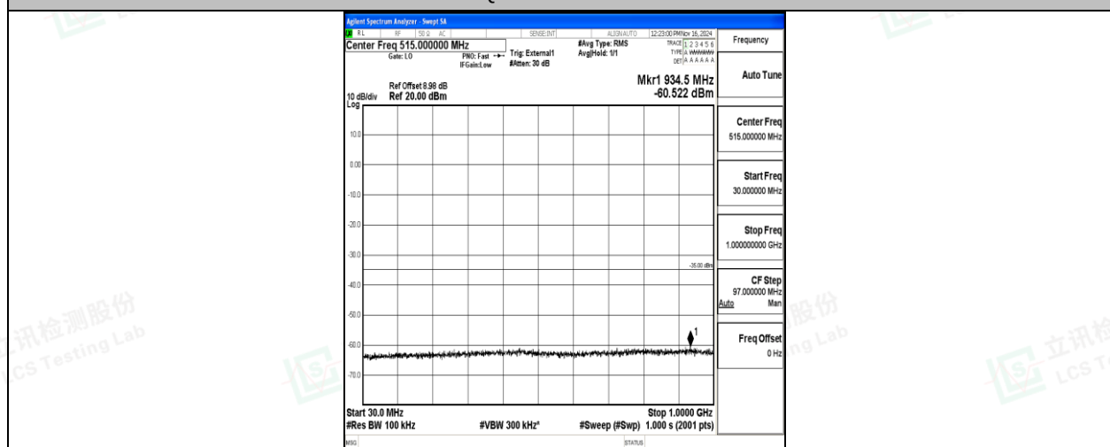
Band41-5MHz-16OAM-40620-1RB#0-30~1000-PASS
