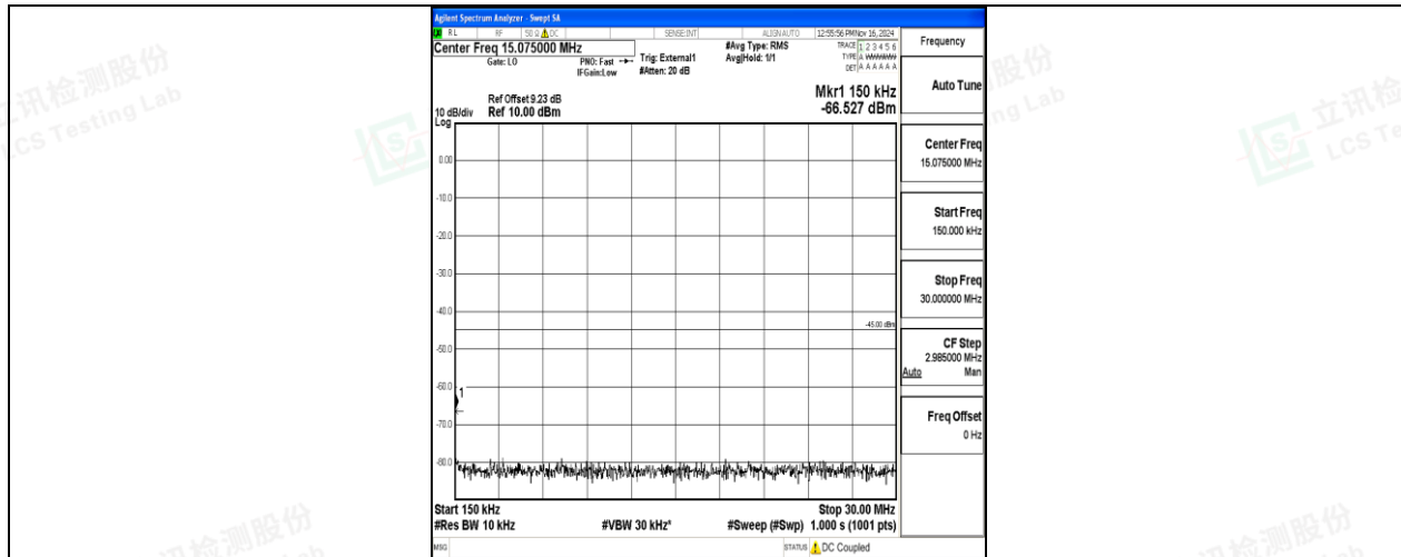
Band41-10MHz-16QAM-39700-1RB#0-0.15~30-PASS
