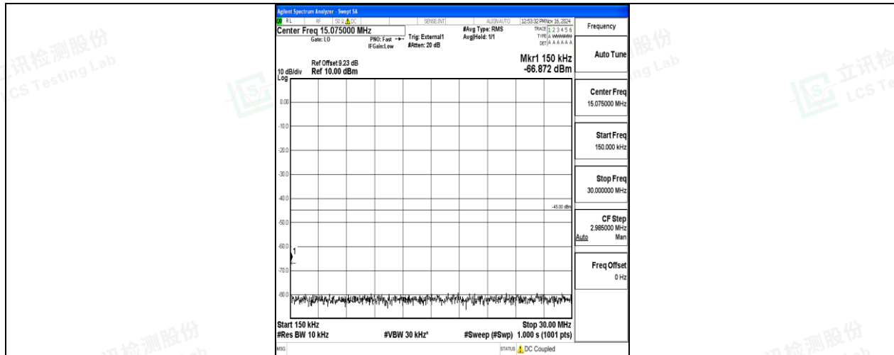
Band41-10MHz-QPSK-39700-1RB#0-0.15~30-PASS
