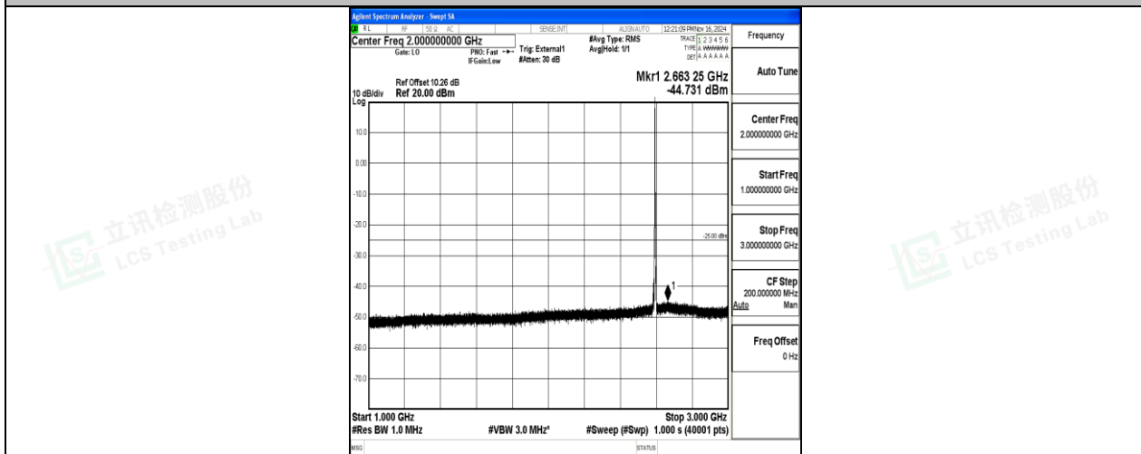
Band41-5MHz-QPSK-40620-1RB#0-1000~3000-PASS
