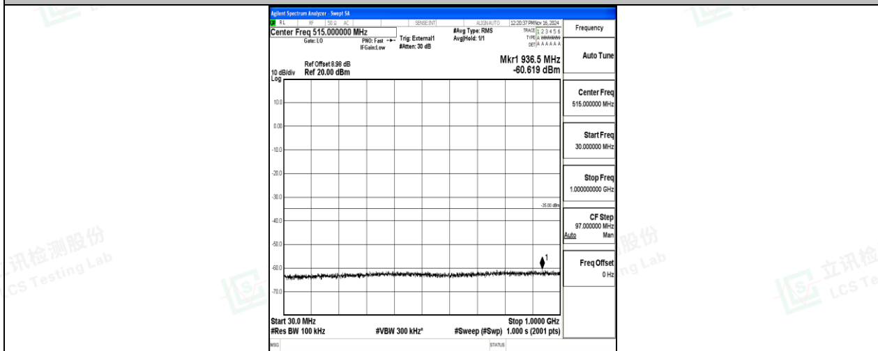
Band41-5MHz-QPSK-40620-1RB#0-30~1000-PASS
