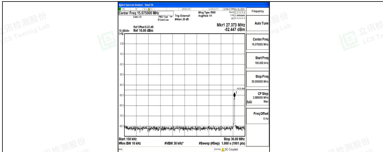
Band41-10MHz-QPSK-40620-1RB#0-0.15~30-PASS
