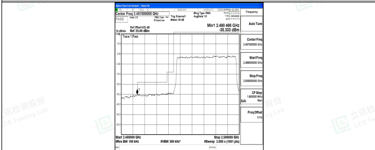
Band41-10MHz-16QAM-39700-50RB#0-PASS
