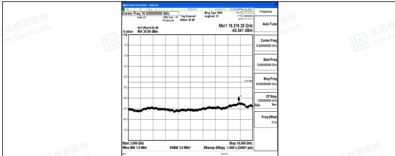
Band41-5MHz-QPSK-41565-1RB#0-3000~18000-PASS
