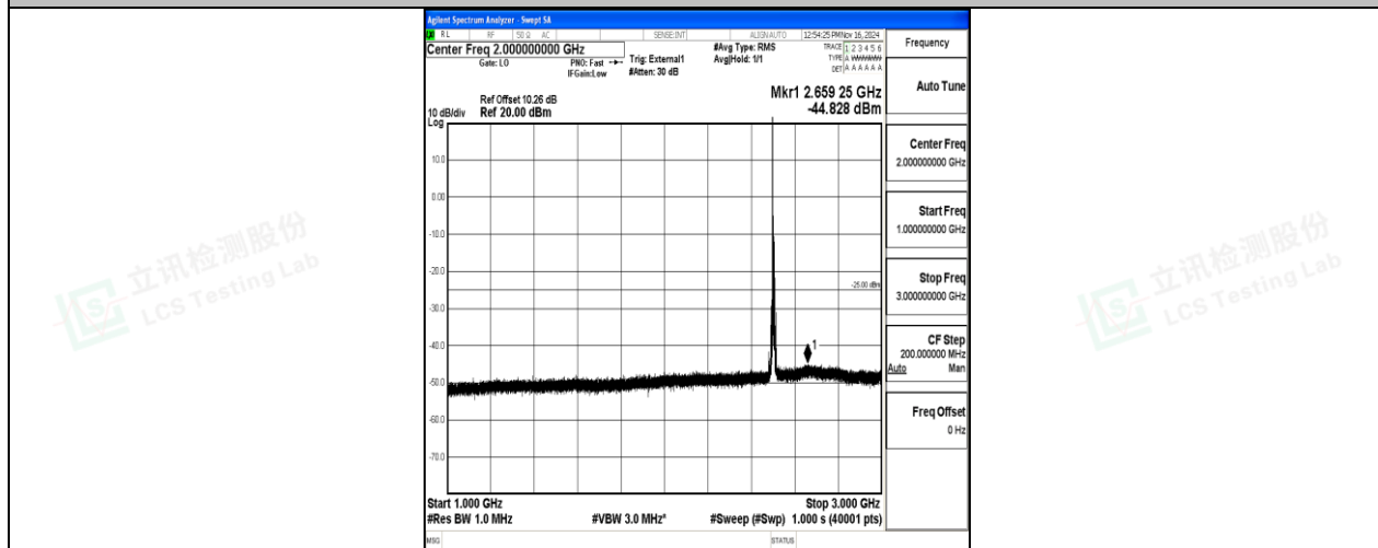
Band41-10MHz-QPSK-39700-1RB#0-1000~3000-PASS
