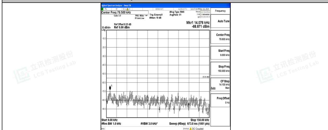
Band41-5MHz-16QAM-39675-1RB#0-0.009~0.15-PASS
