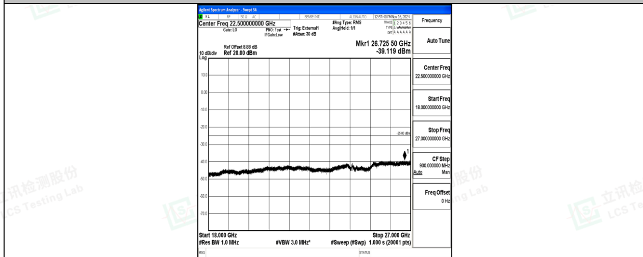
Band41-10MHz-16QAM-39700-1RB#0-18000~27000-PASS
