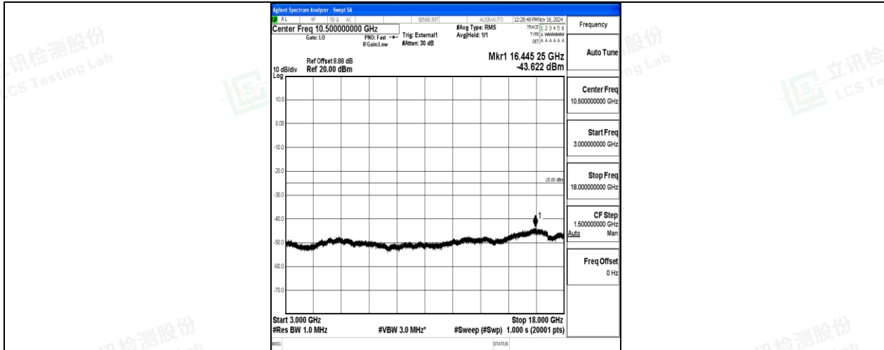
Band41-5MHz-16QAM-41565-1RB#0-3000~18000-PASS
