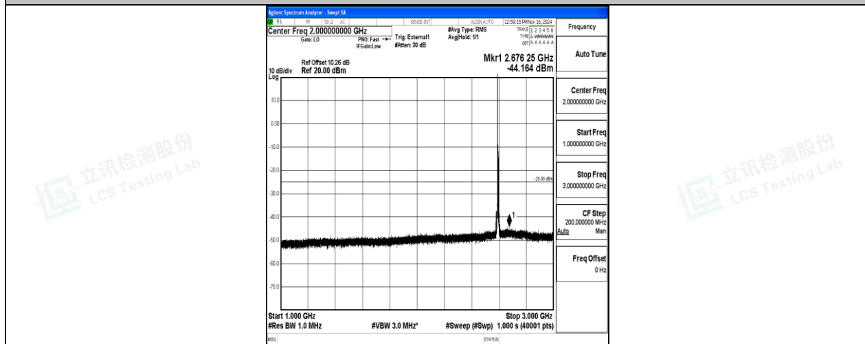
Band41-10MHz-QPSK-40620-1RB#0-1000~3000-PASS
