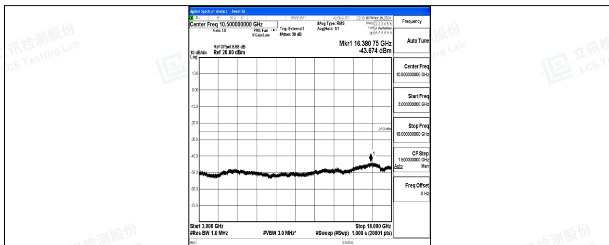
Band41-5MHz-16QAM-39675-1RB#0-3000~18000-PASS
