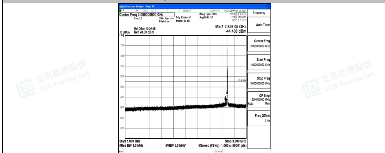
Band41-10MHz-QPSK-41540-1RB#0-1000~3000-PASS
