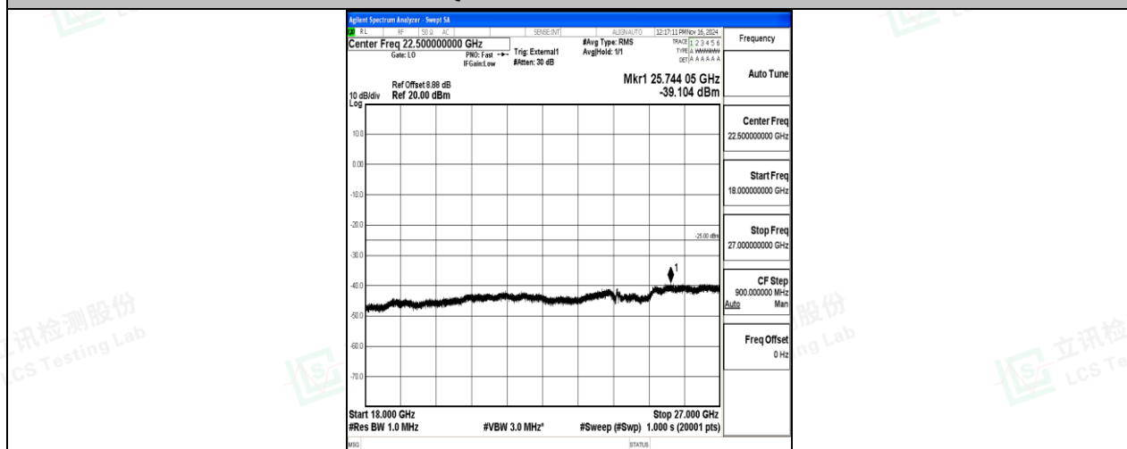
Band41-5MHz-QPSK-39675-1RB#0-18000~27000-PASS
