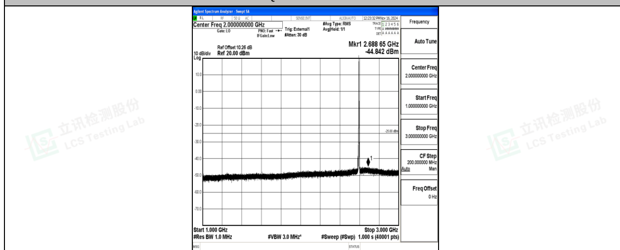
Band41-5MHz-16OAM-40620-1RB#0-1000~3000-PASS
