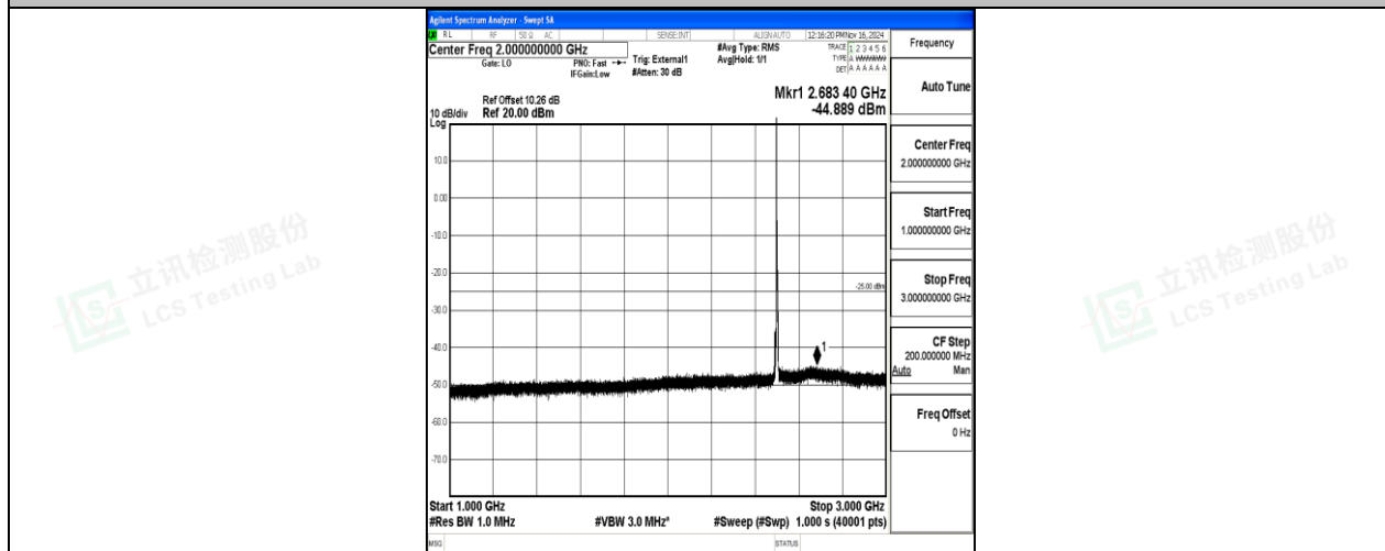
Band41-5MHz-QPSK-39675-1RB#0-1000~3000-PASS
