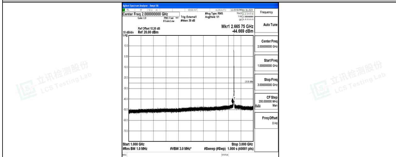
Band41-5MHz-QPSK-41565-1RB#0-1000~3000-PASS
