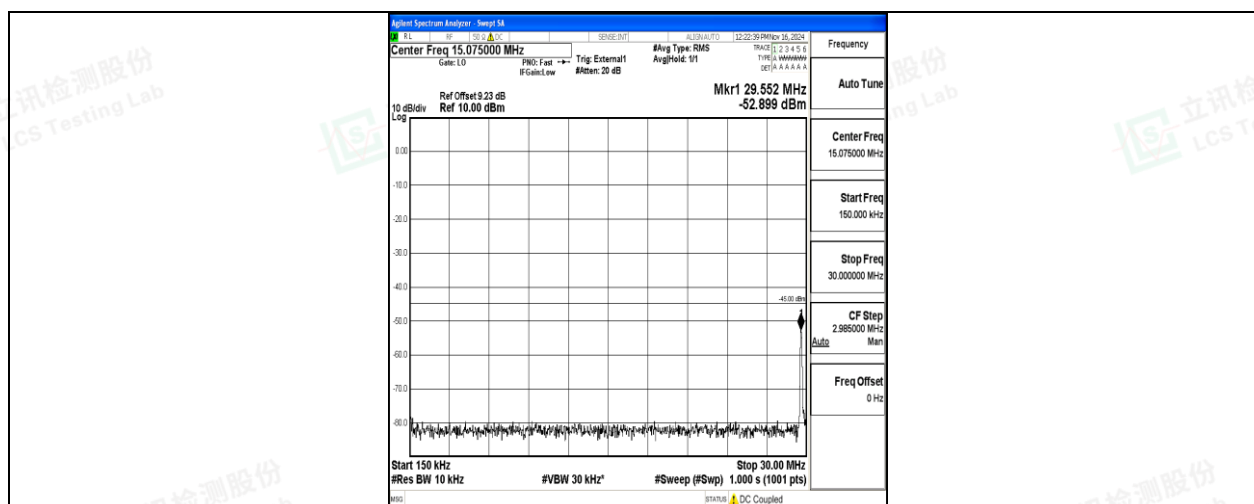
Band41-5MHz-16QAM-40620-1RB#0-0.15~30-PASS
