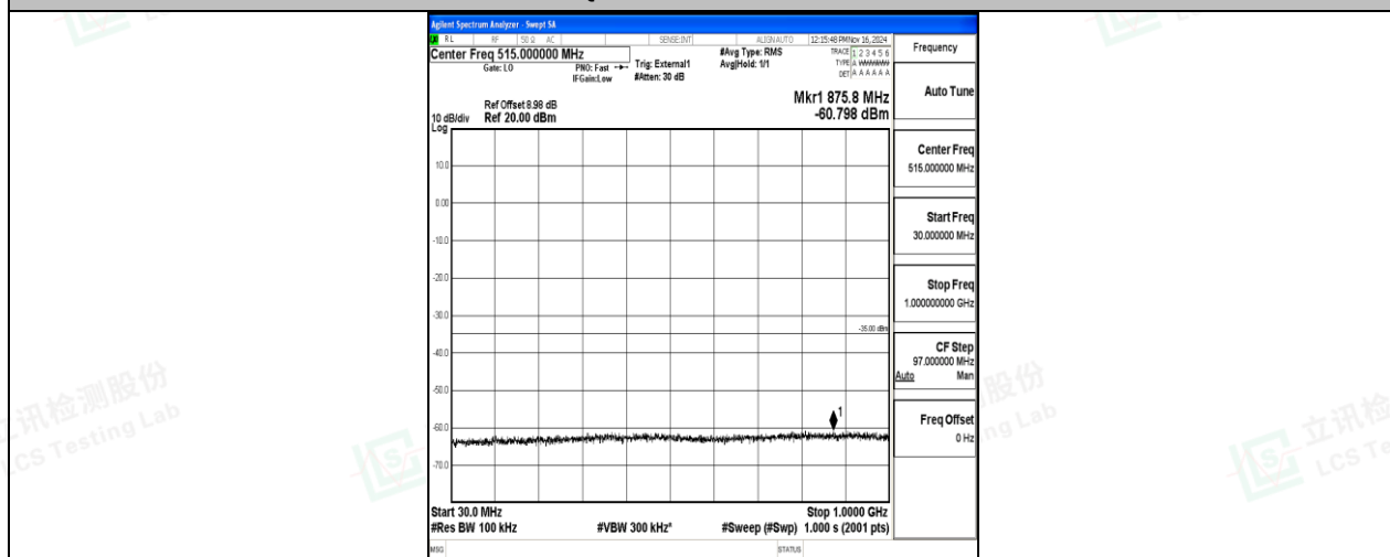
Band41-5MHz-QPSK-39675-1RB#0-30~1000-PASS
