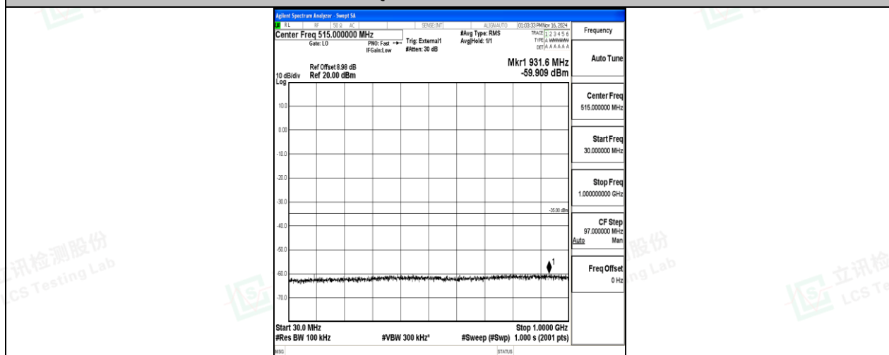
Band41-10MHz-QPSK-41540-1RB#0-30~1000-PASS
