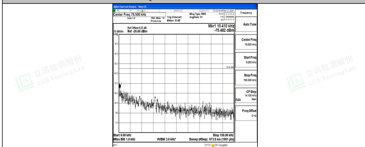
Band38-20MHz-QPSK-38150-100RB#0-0.009~0.15-PASS
