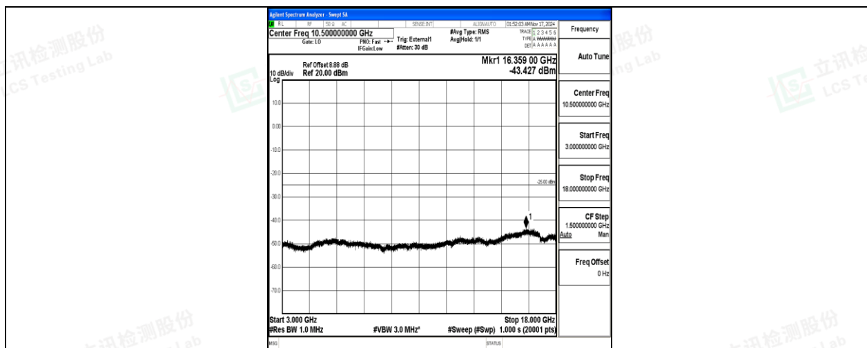
Band38-20MHz-16QAM-38000-100RB#0-3000~18000-PASS
