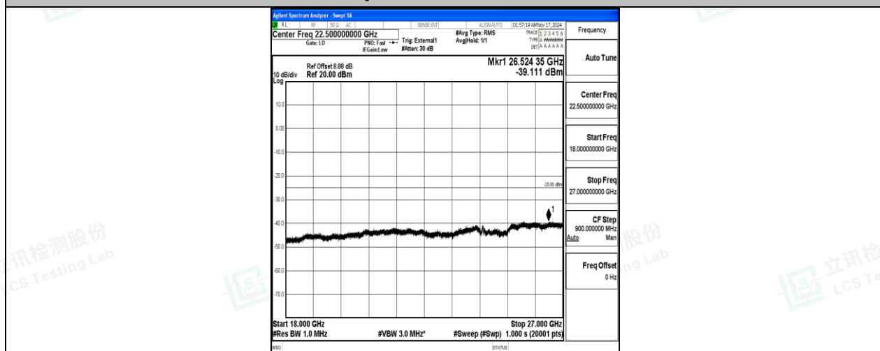
Band38-20MHz-16QAM-38150-100RB#0-18000~27000-PASS
