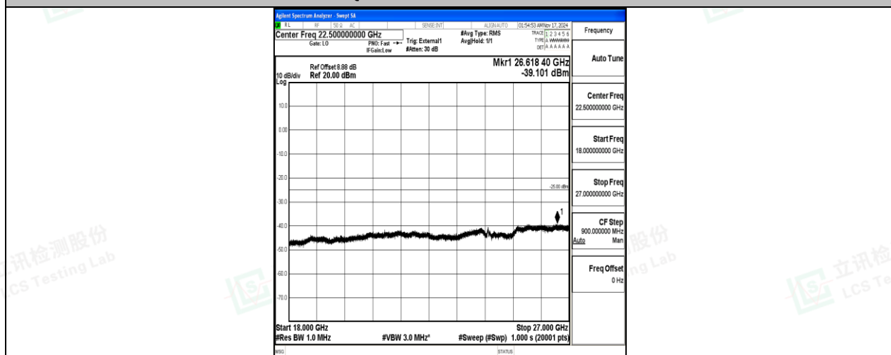
Band38-20MHz-QPSK-38150-100RB#0-18000~27000-PASS
