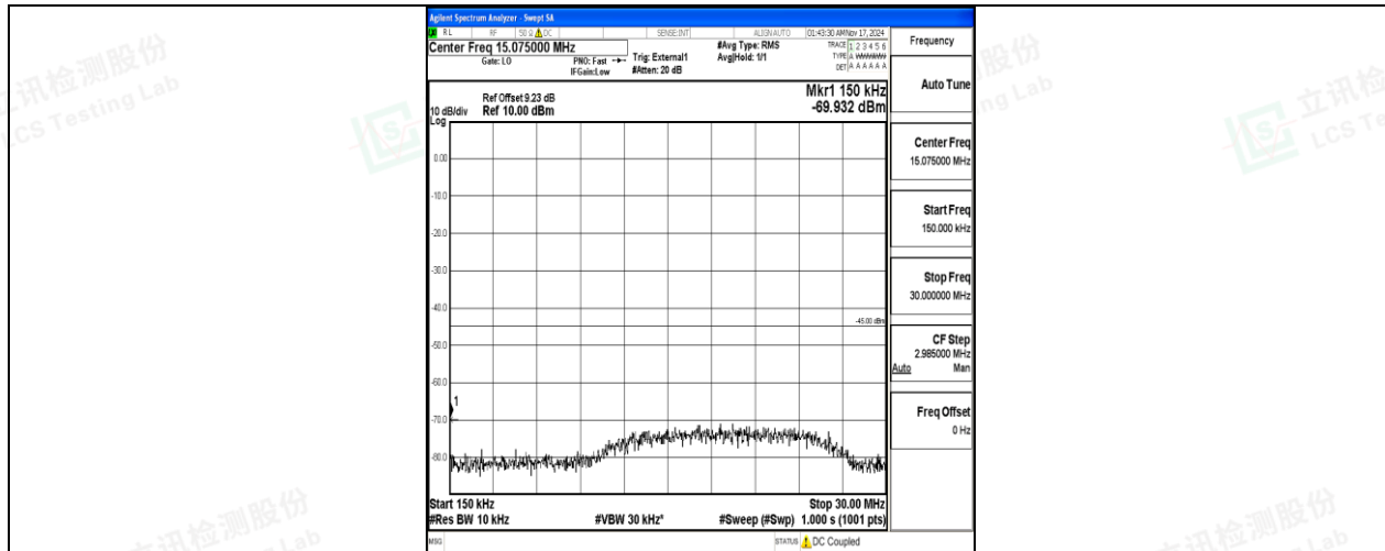
Band38-20MHz-QPSK-37850-100RB#0-0.15~30-PASS
