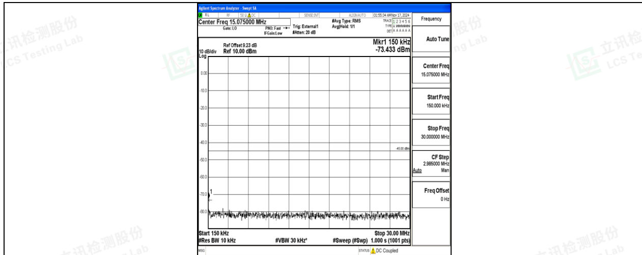
Band38-20MHz-16QAM-38150-100RB#0-0.15~30-PASS
