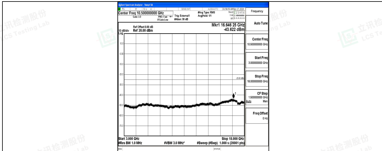
Band38-20MHz-16QAM-38150-100RB#0-3000~18000-PASS
