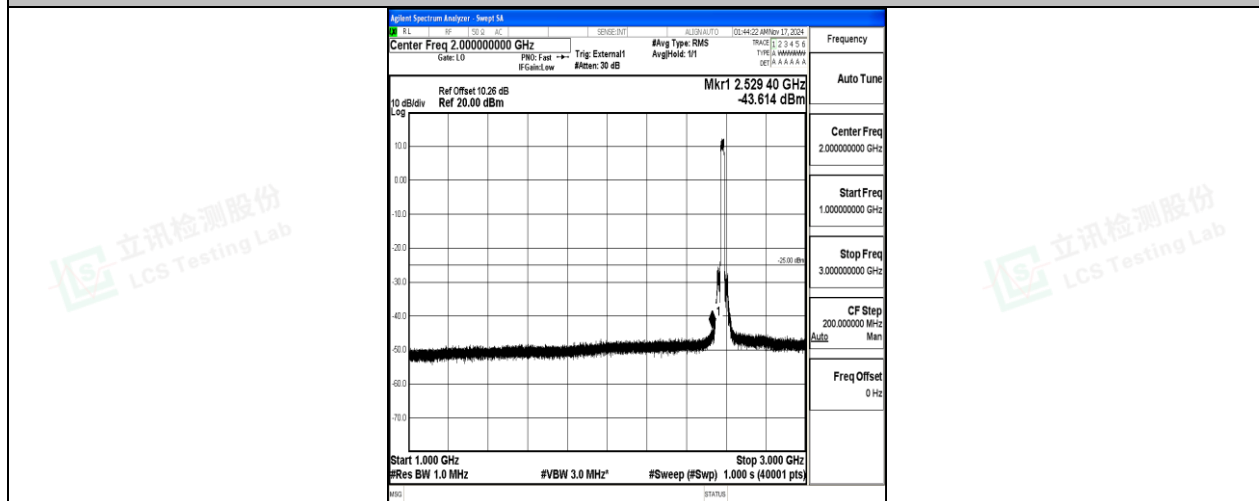
Band38-20MHz-QPSK-37850-100RB#0-1000~3000-PASS
