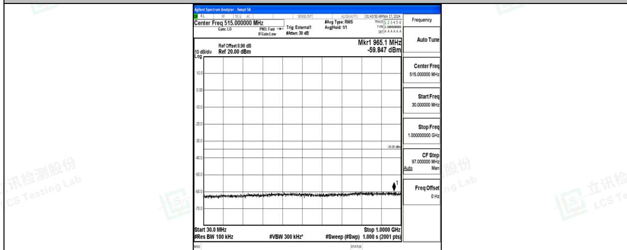
Band38-20MHz-QPSK-37850-100RB#0-30~1000-PASS
