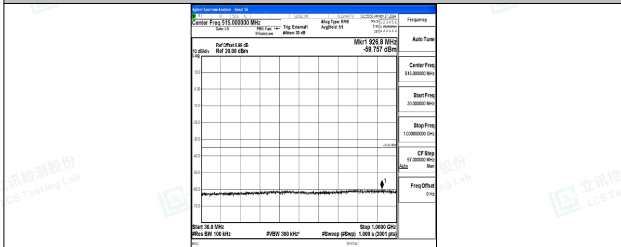
Band38-20MHz-16QAM-38150-100RB#0-30~1000-PASS
