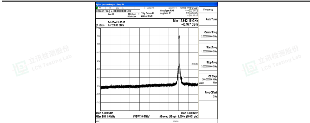
Band38-20MHz-16QAM-38150-100RB#0-1000~3000-PASS
