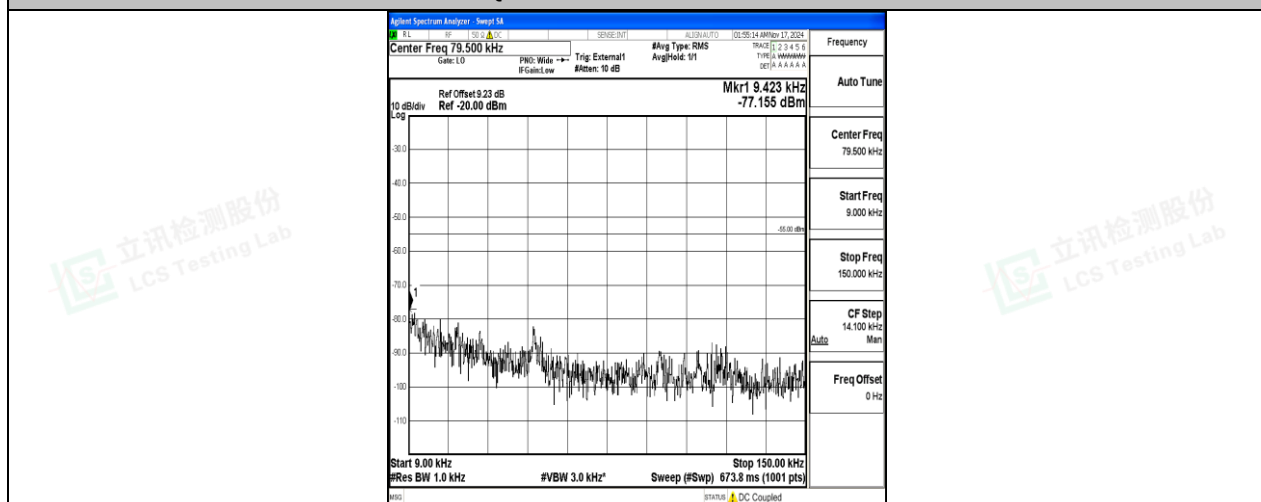
Band38-20MHz-16QAM-38150-100RB#0-0.009~0.15-PASS
