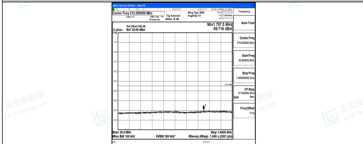
Band38-20MHz-16QAM-37850-100RB#0-30~1000-PASS
