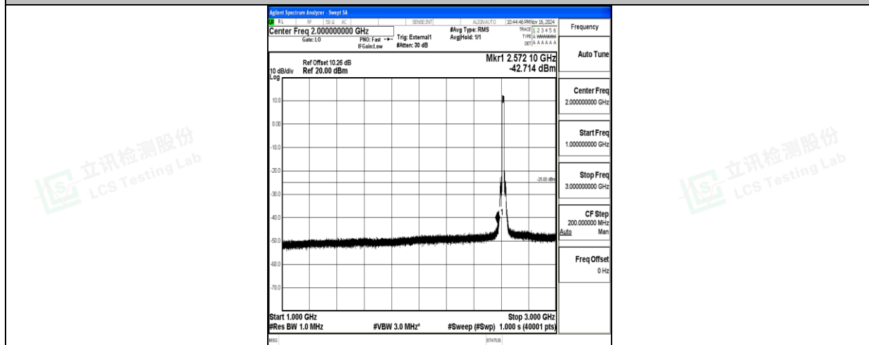
Band38-15MHz-QPSK-38175-75RB#0-1000~3000-PASS
