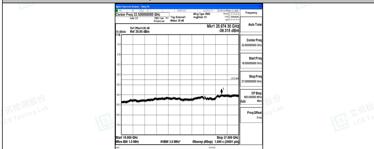
Band38-20MHz-QPSK-37850-100RB#0-18000~27000-PASS
