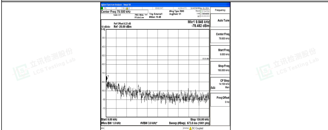
Band38-15MHz-16QAM-38175-75RB#0-0.009~0.15-PASS
