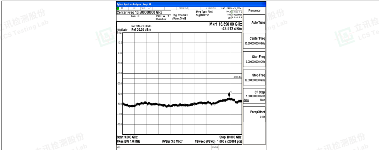
Band38-15MHz-QPSK-38175-75RB#0-3000~18000-PASS
