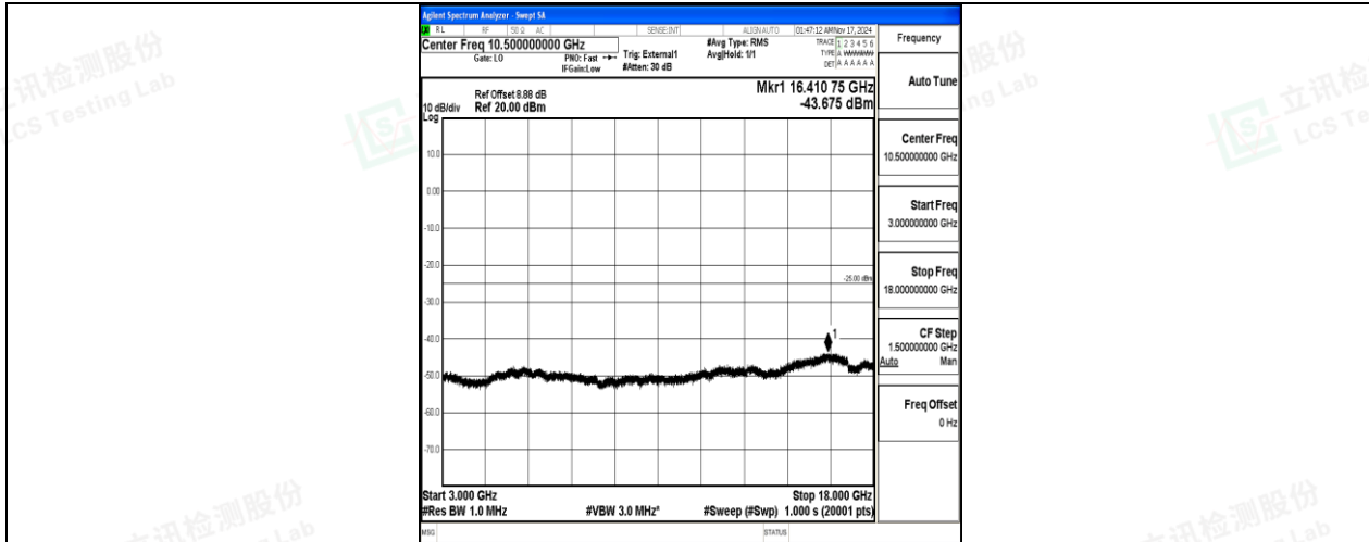
Band38-20MHz-16QAM-37850-100RB#0-3000~18000-PASS
