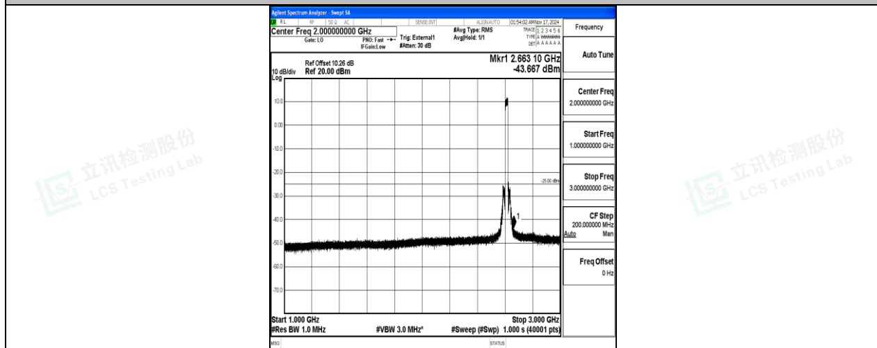
Band38-20MHz-QPSK-38150-100RB#0-1000~3000-PASS
