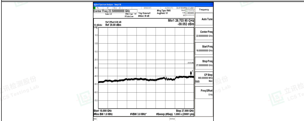
Band38-20MHz-16QAM-37850-100RB#0-18000~27000-PASS
