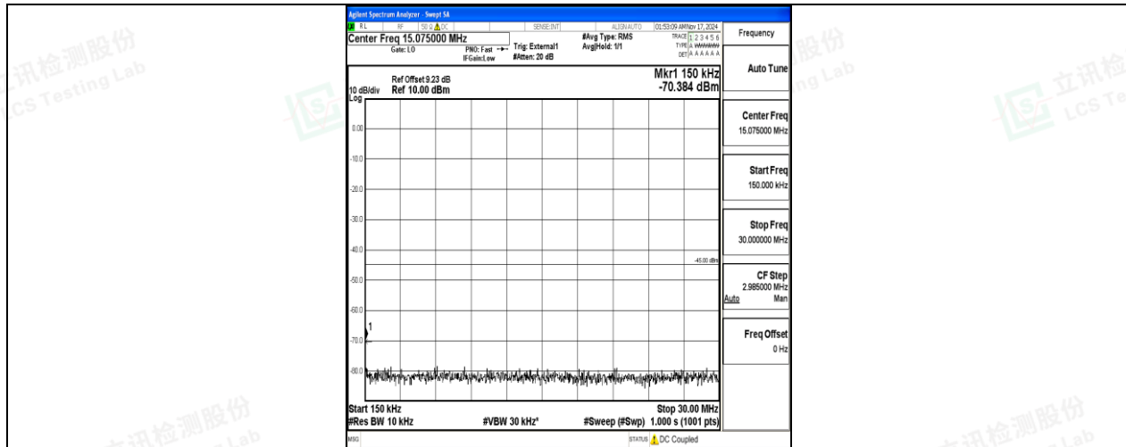
Band38-20MHz-QPSK-38150-100RB#0-0.15~30-PASS
