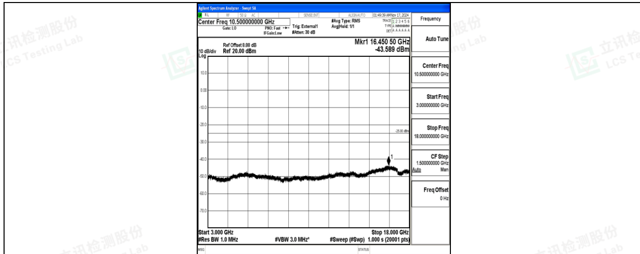
Band38-20MHz-QPSK-38000-100RB#0-3000~18000-PASS
