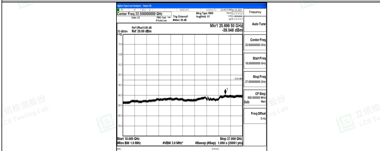
Band38-15MHz-QPSK-38175-75RB#0-18000~27000-PASS
