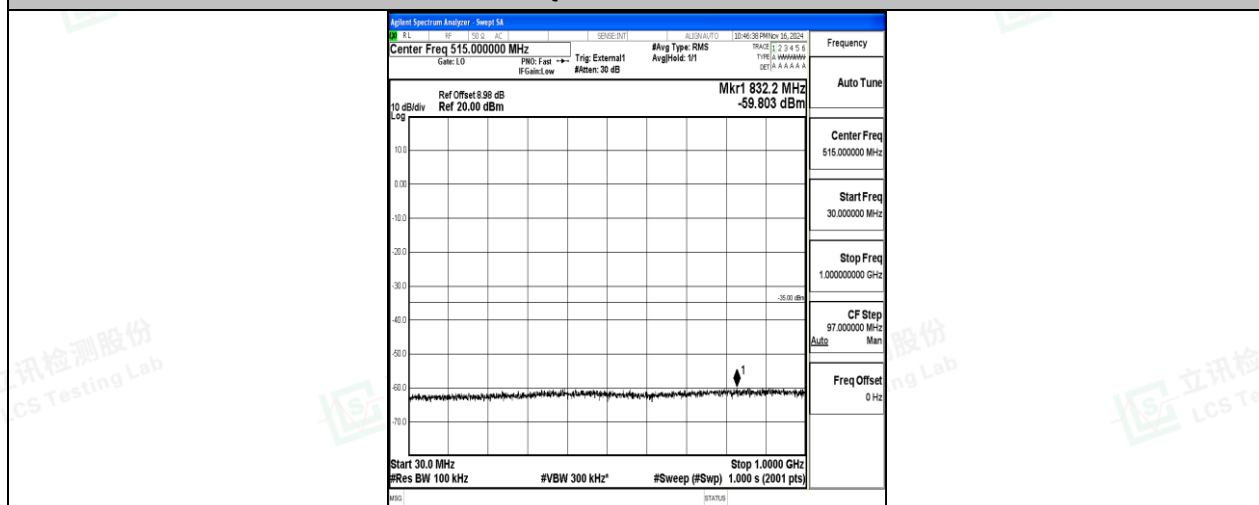
Band38-15MHz-16QAM-38175-75RB#0-30~1000-PASS
