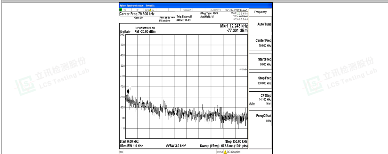
Band38-20MHz-QPSK-38000-100RB#0-0.009~0.15-PASS
