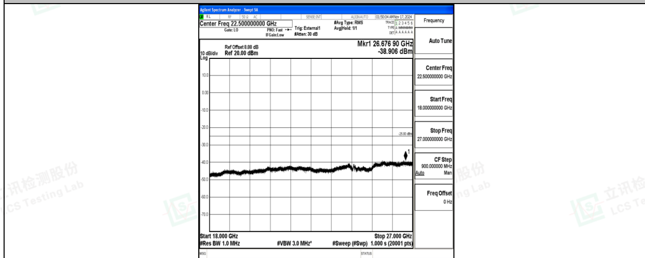
Band38-20MHz-QPSK-38000-100RB#0-18000~27000-PASS
