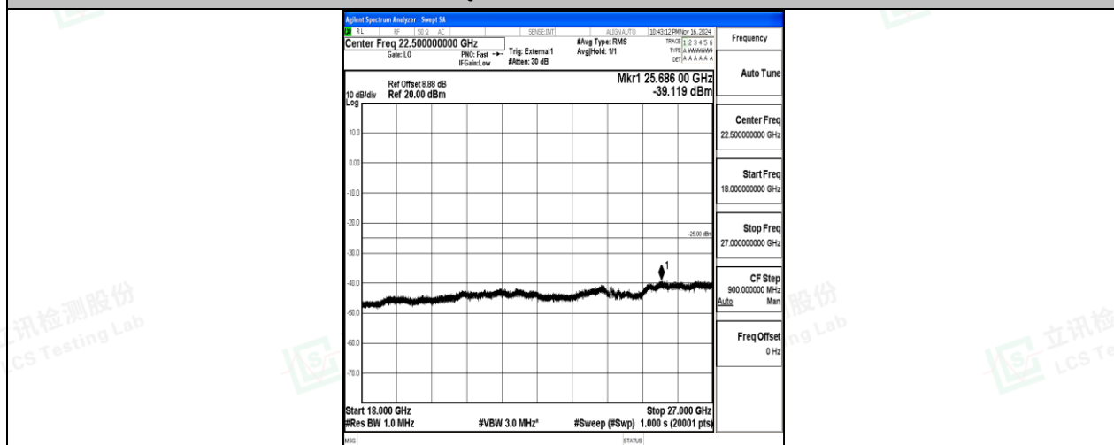
Band38-15MHz-16QAM-38000-75RB#0-18000~27000-PASS
