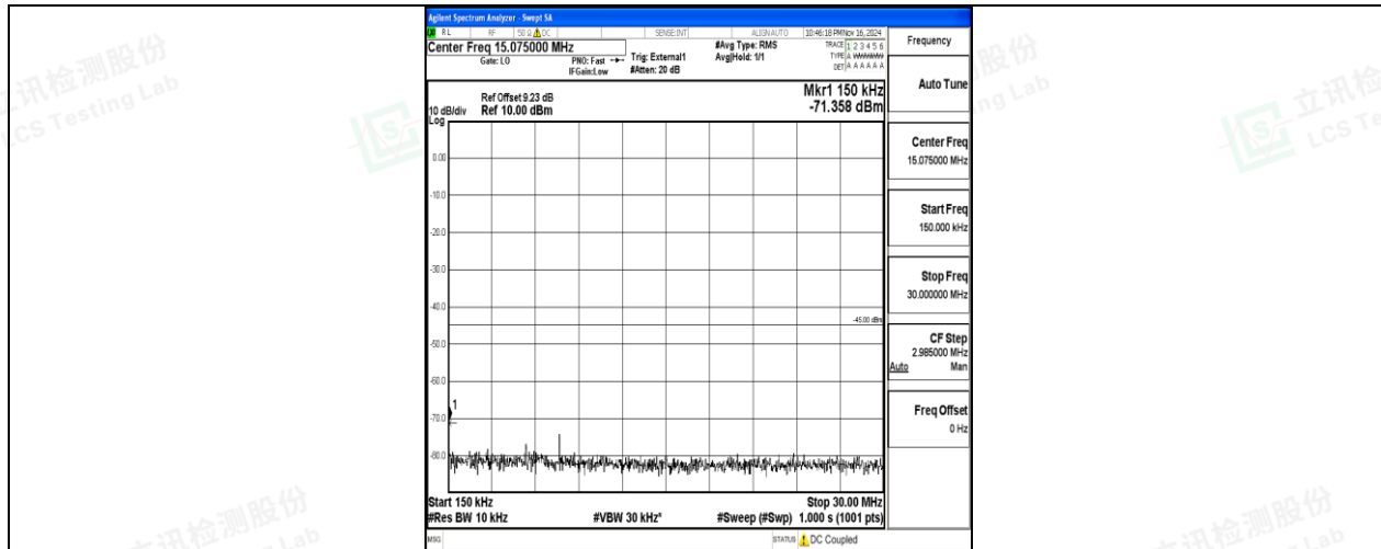
Band38-15MHz-16QAM-38175-75RB#0-0.15~30-PASS
