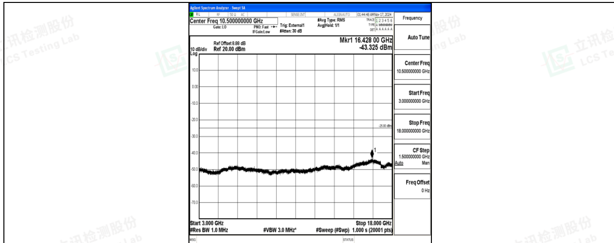
Band38-20MHz-QPSK-37850-100RB#0-3000~18000-PASS
