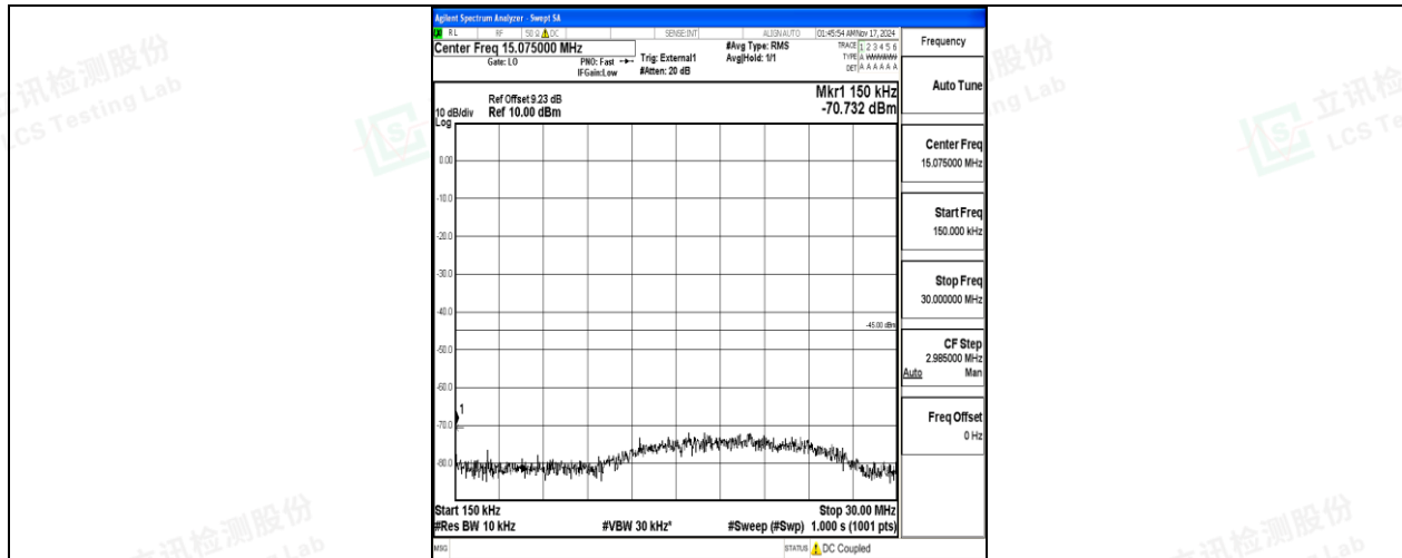
Band38-20MHz-16QAM-37850-100RB#0-0.15~30-PASS
