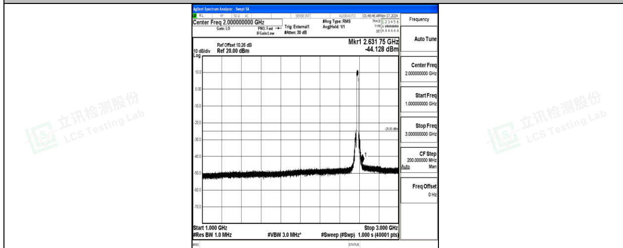
Band38-20MHz-16QAM-37850-100RB#0-1000~3000-PASS
