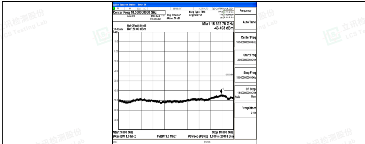
Band38-15MHz-16QAM-38000-75RB#0-3000~18000-PASS
