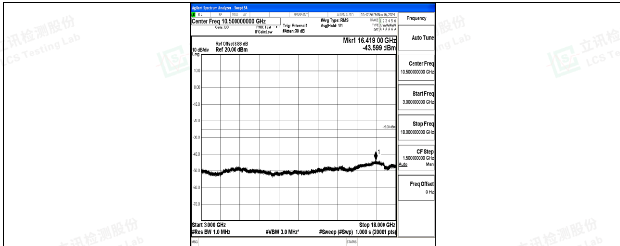
Band38-15MHz-16QAM-38175-75RB#0-3000~18000-PASS
