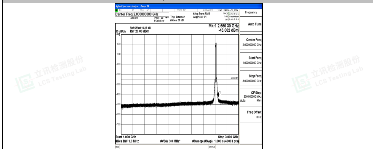
Band38-15MHz-16QAM-38175-75RB#0-1000~3000-PASS
