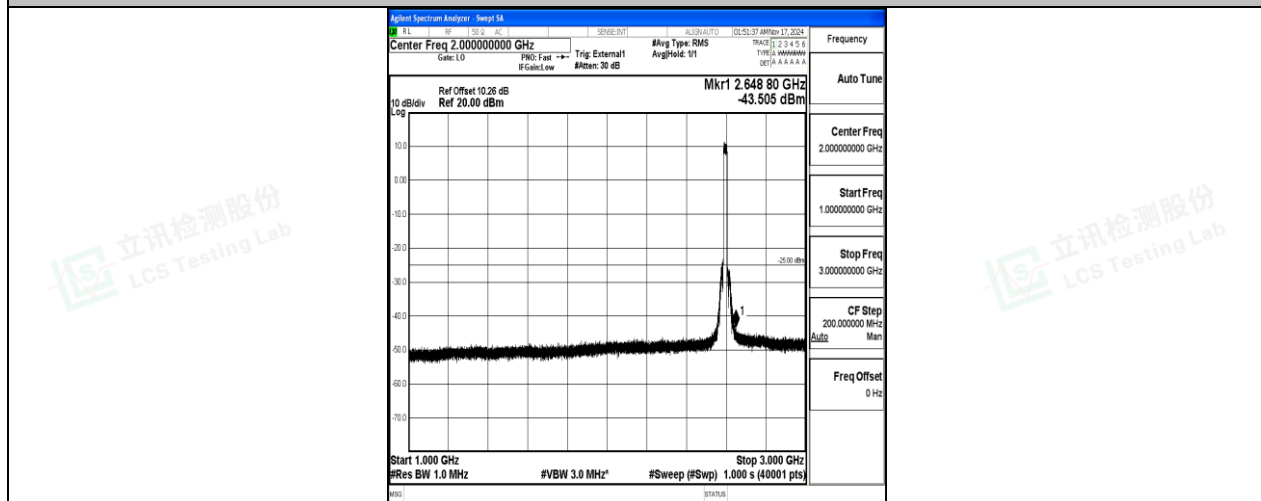
Band38-20MHz-16QAM-38000-100RB#0-1000~3000-PASS
