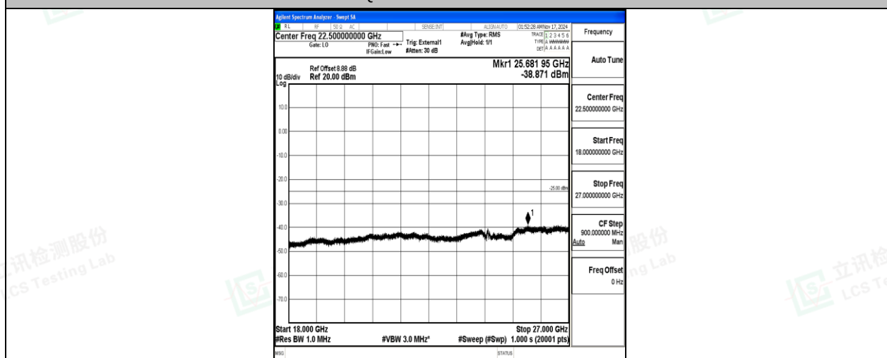
Band38-20MHz-16QAM-38000-100RB#0-18000~27000-PASS
