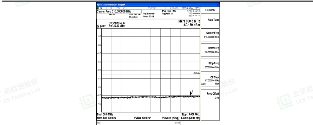
Band38-20MHz-QPSK-38150-100RB#0-30~1000-PASS
