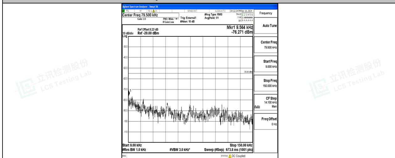
Band38-5MHz-16QAM-37775-25RB#0-0.009~0.15-PASS
