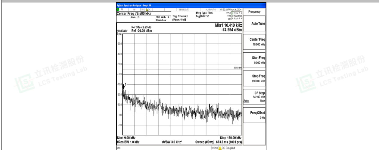
Band38-10MHz-QPSK-38200-50RB#0-0.009~0.15-PASS
