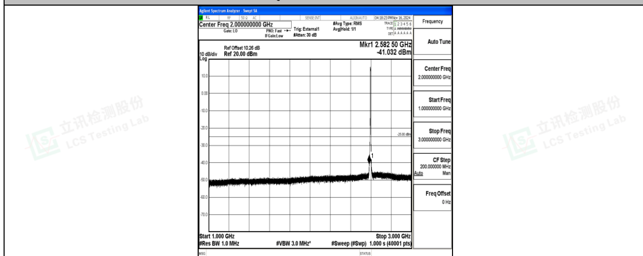
Band38-5MHz-16QAM-38000-25RB#0-1000~3000-PASS
