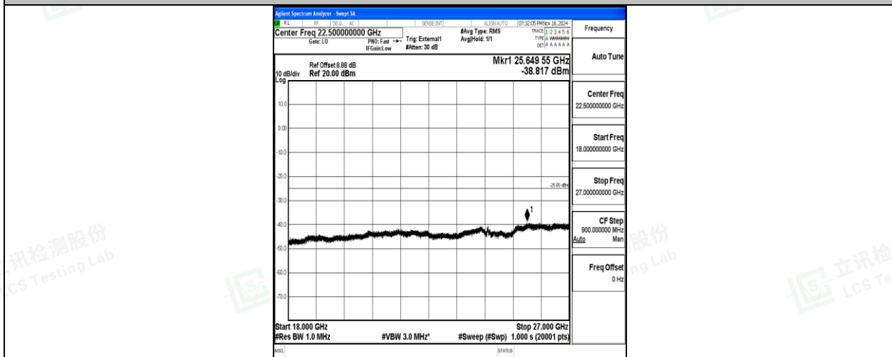
Band38-10MHz-16QAM-38000-50RB#0-18000~27000-PASS
