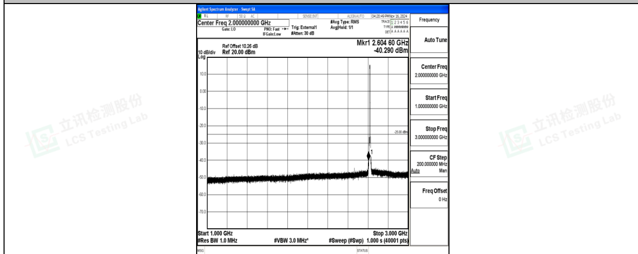
Band38-5MHz-QPSK-38225-25RB#0-1000~3000-PASS
