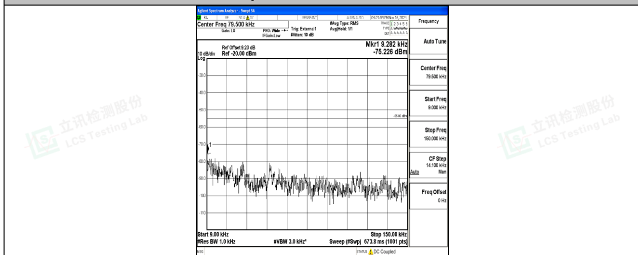
Band38-5MHz-16QAM-38225-25RB#0-0.009~0.15-PASS
