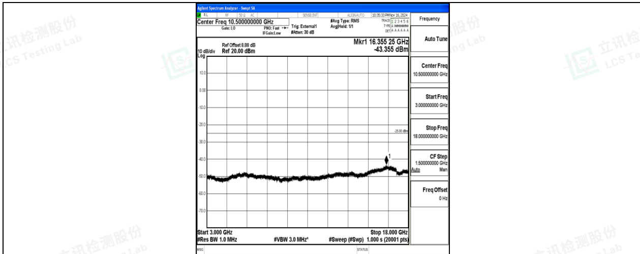
Band38-15MHz-QPSK-37825-75RB#0-3000~18000-PASS
