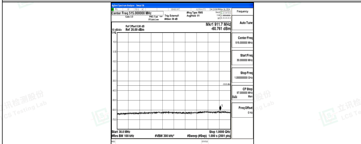
Band38-5MHz-16QAM-37775-25RB#0-30~1000-PASS
