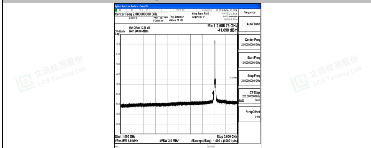
Band38-10MHz-QPSK-38200-50RB#0-1000~3000-PASS
