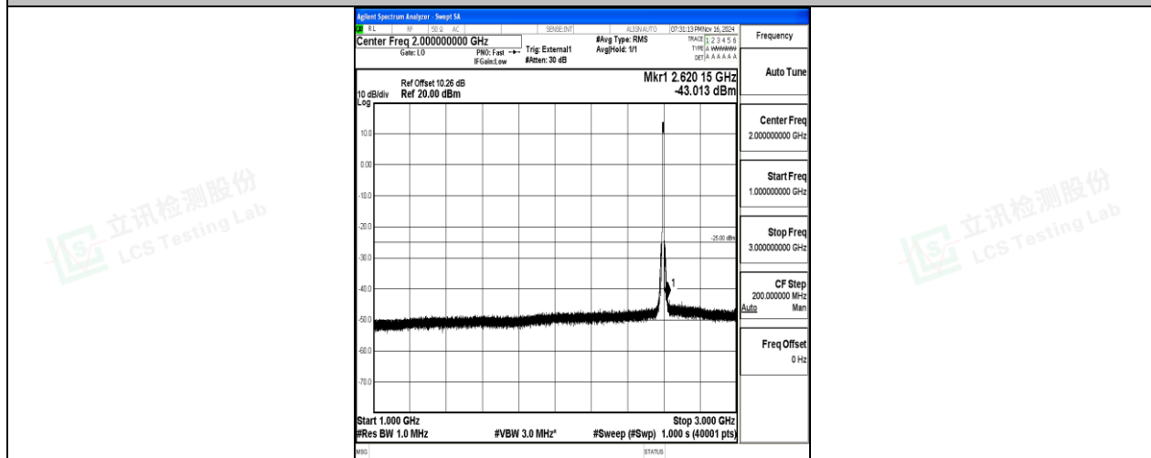
Band38-10MHz-16QAM-38000-50RB#0-1000~3000-PASS
