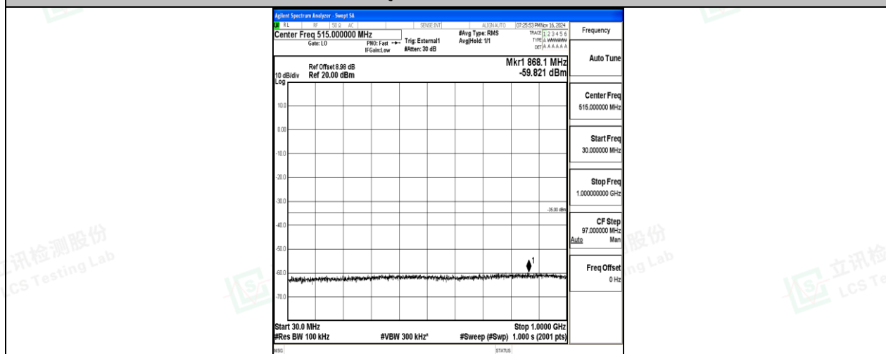
Band38-10MHz-16QAM-37800-50RB#0-30~1000-PASS
