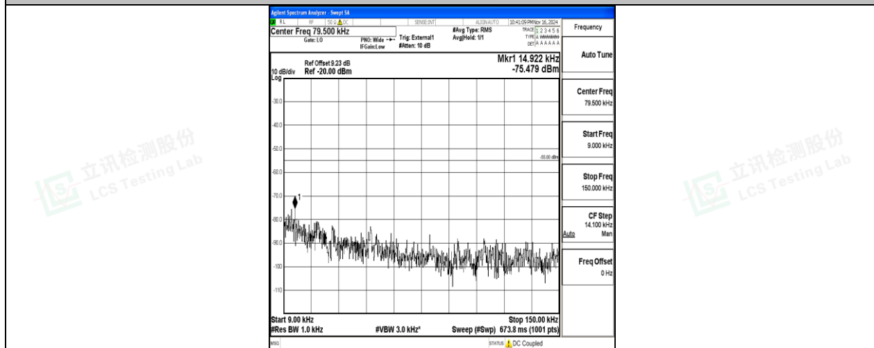
Band38-15MHz-16QAM-38000-75RB#0-0.009~0.15-PASS
