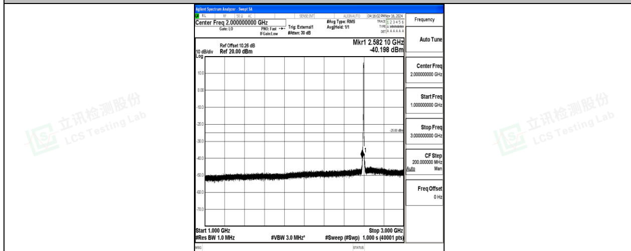
Band38-5MHz-QPSK-38000-25RB#0-1000~3000-PASS
