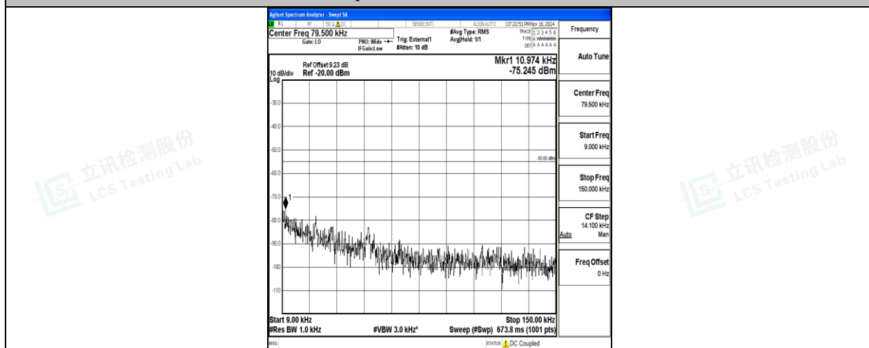
Band38-10MHz-QPSK-37800-50RB#0-0.009~0.15-PASS
