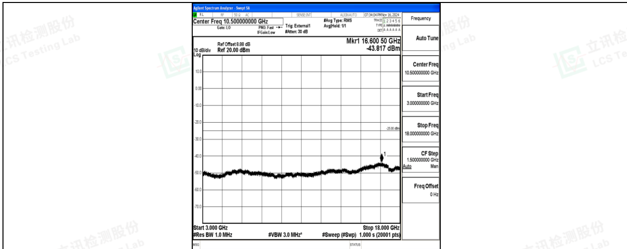
Band38-10MHz-QPSK-38200-50RB#0-3000~18000-PASS
