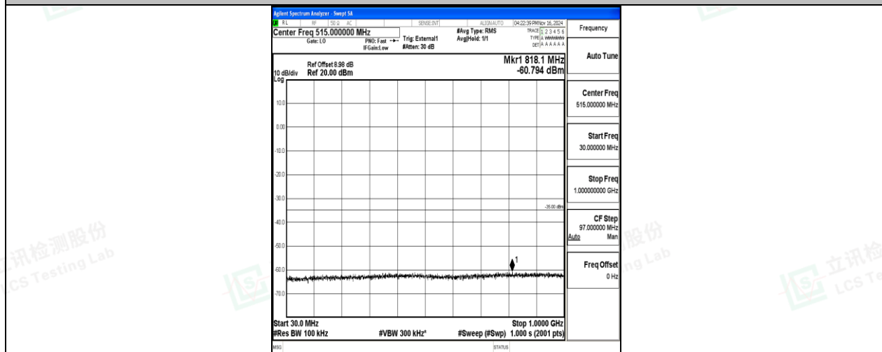
Band38-5MHz-16QAM-38225-25RB#0-30~1000-PASS
