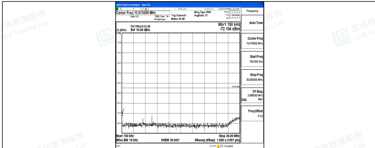
Band38-15MHz-QPSK-38000-75RB#0-0.15~30-PASS
