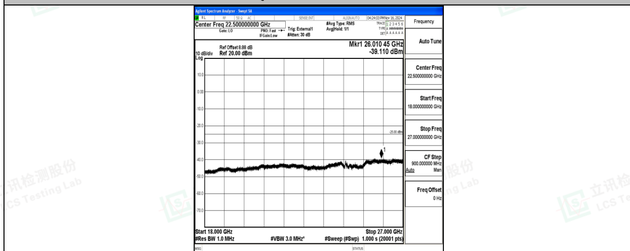
Band38-5MHz-16QAM-38225-25RB#0-18000~27000-PASS
