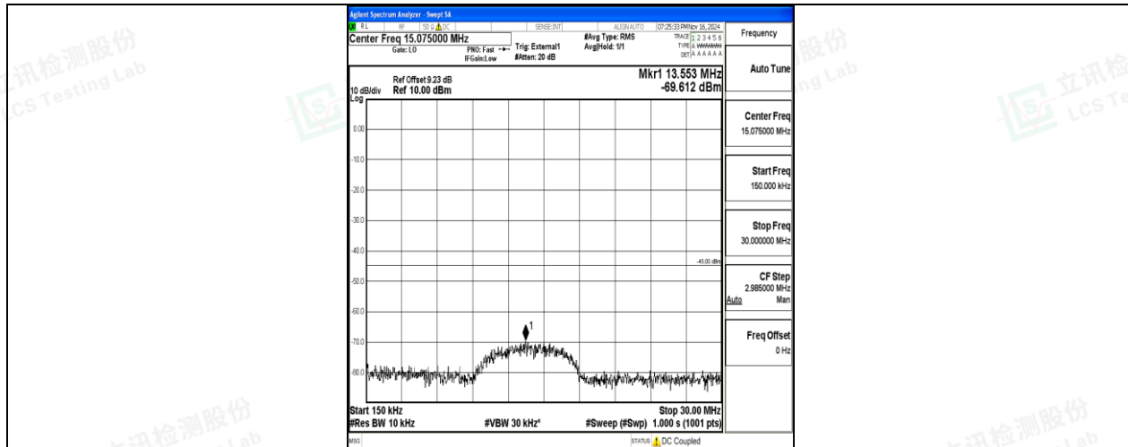
Band38-10MHz-16QAM-37800-50RB#0-0.15~30-PASS
