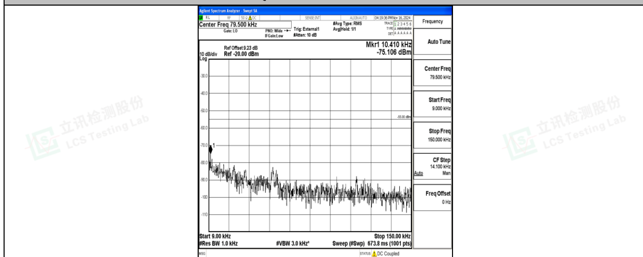
Band38-5MHz-QPSK-38225-25RB#0-0.009~0.15-PASS
