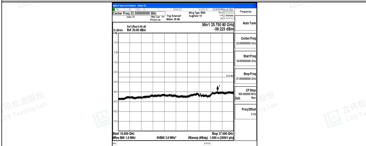
Band38-15MHz-QPSK-37825-75RB#0-18000~27000-PASS
