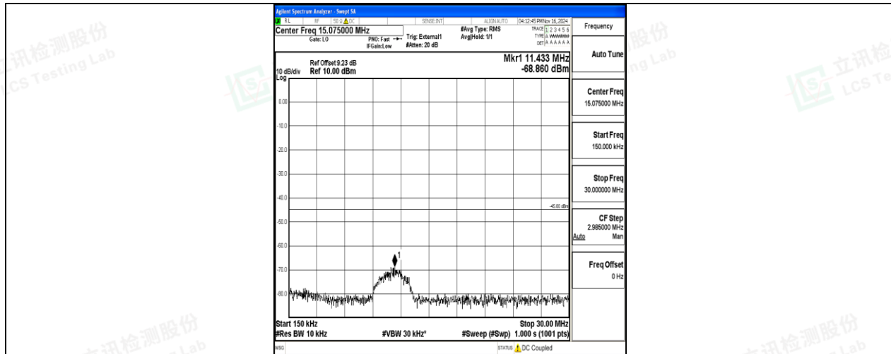
Band38-5MHz-16QAM-37775-25RB#0-0.15~30-PASS
