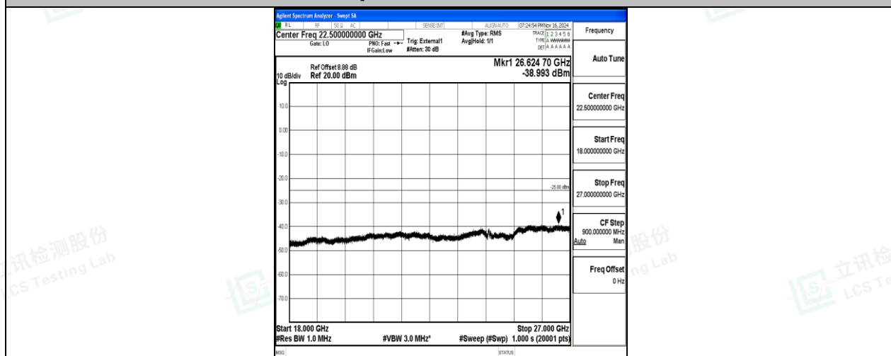
Band38-10MHz-QPSK-37800-50RB#0-18000~27000-PASS
