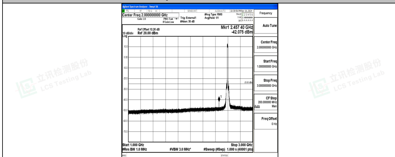
Band38-15MHz-QPSK-38000-75RB#0-1000~3000-PASS
