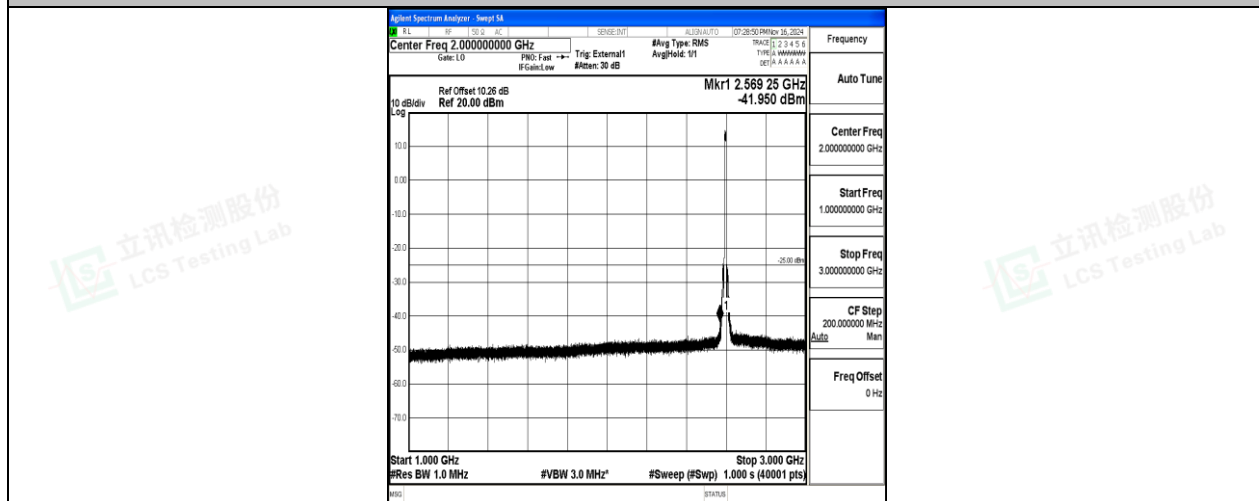
Band38-10MHz-QPSK-38000-50RB#0-1000~3000-PASS
