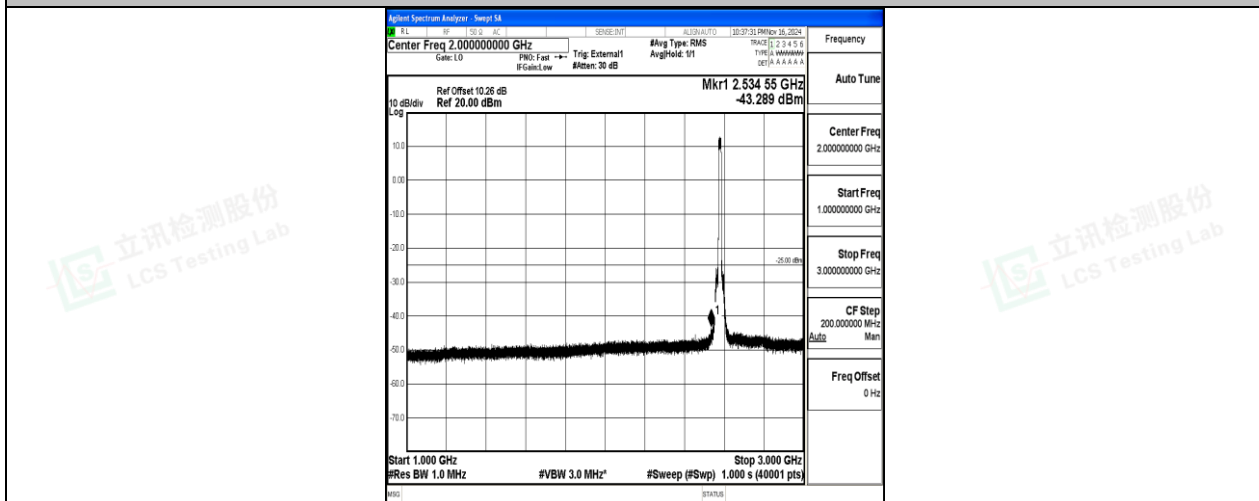
Band38-15MHz-16QAM-37825-75RB#0-1000~3000-PASS
