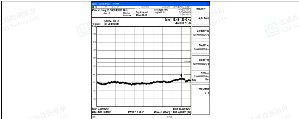
Band38-10MHz-QPSK-38000-50RB#0-3000~18000-PASS
