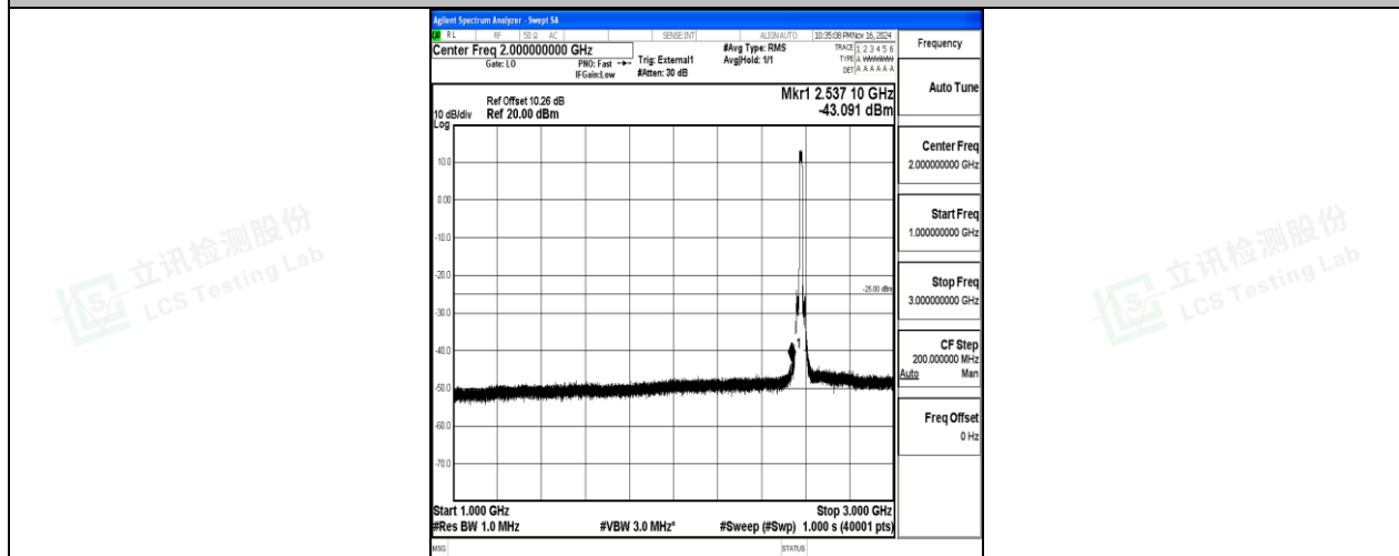
Band38-15MHz-QPSK-37825-75RB#0-1000~3000-PASS
