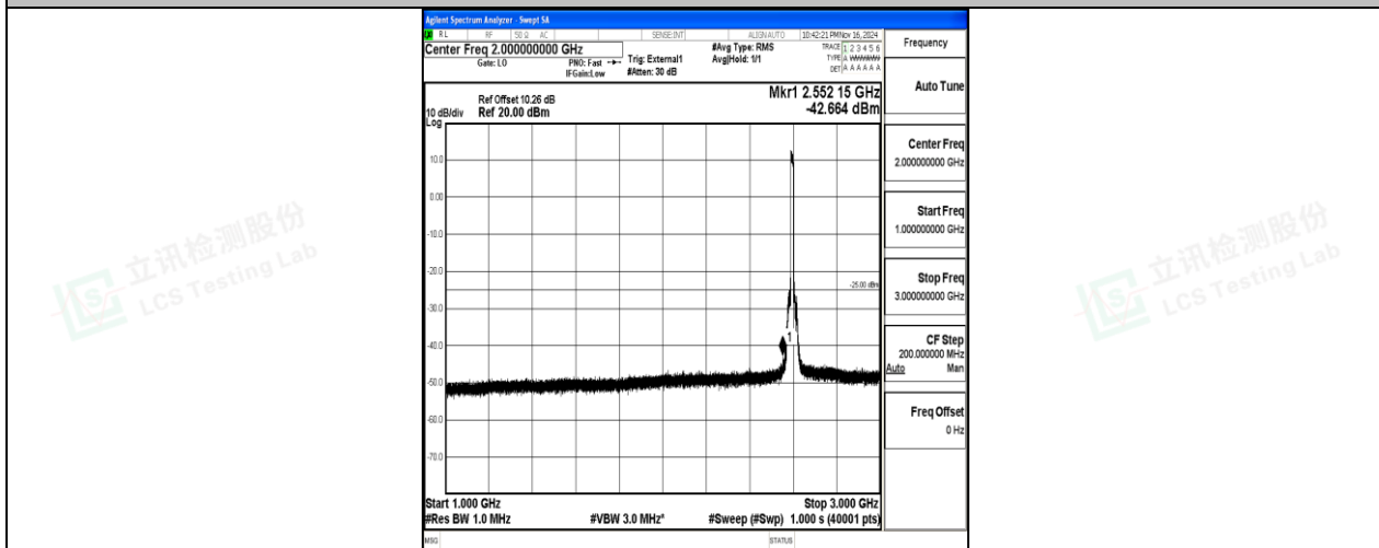
Band38-15MHz-16QAM-38000-75RB#0-1000~3000-PASS
