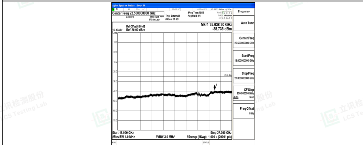
Band38-10MHz-16QAM-38200-50RB#0-18000~27000-PASS
