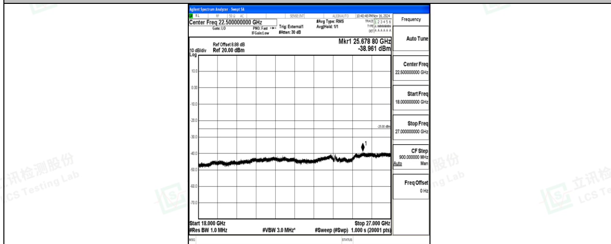
Band38-15MHz-QPSK-38000-75RB#0-18000~27000-PASS
