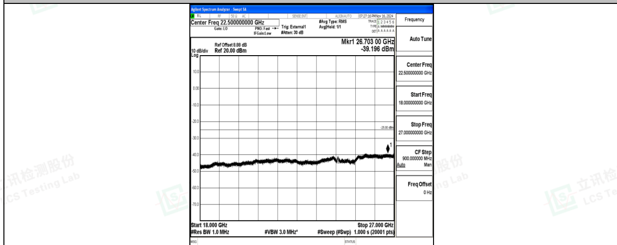
Band38-10MHz-16QAM-37800-50RB#0-18000~27000-PASS
