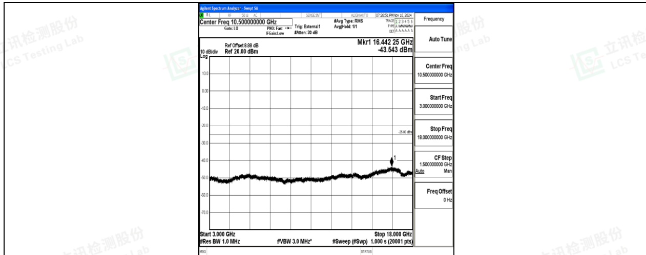
Band38-10MHz-16QAM-37800-50RB#0-3000~18000-PASS
