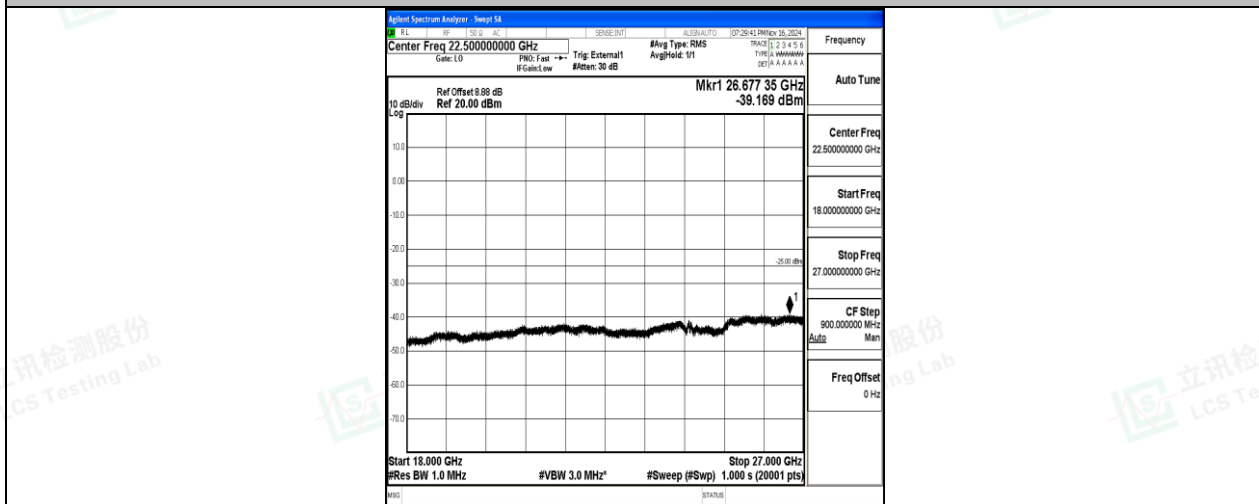
Band38-10MHz-QPSK-38000-50RB#0-18000~27000-PASS
