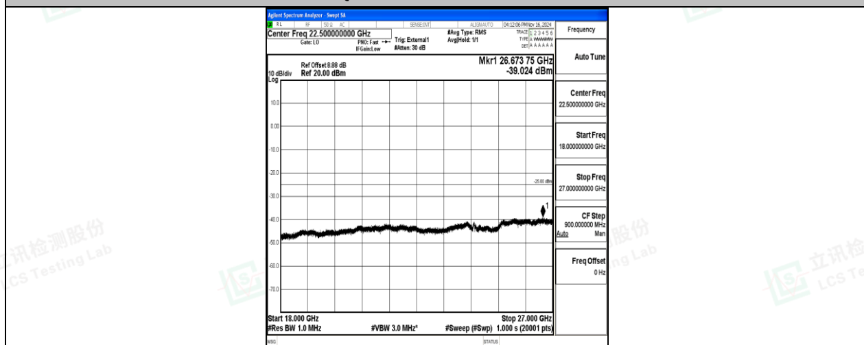
Band38-5MHz-QPSK-37775-25RB#0-18000~27000-PASS
