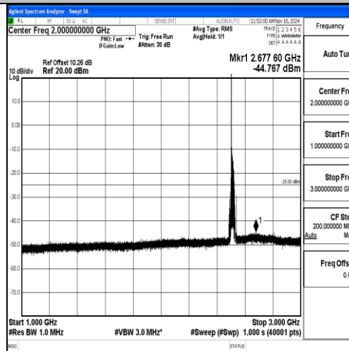
Band7-20MHz-16QAM-20850-1RB#0-1000~3000-PASS
