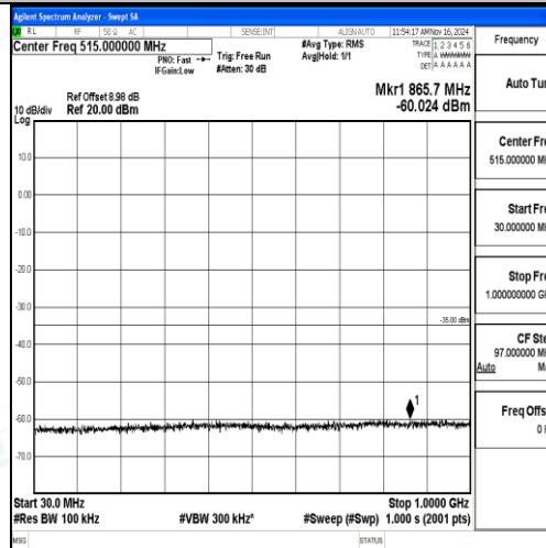
Band7-20MHz-16QAM-21100-1RB#0-30~1000-PASS
