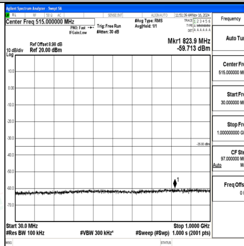
Band7-20MHz-16QAM-20850-1RB#0-0-30~1000-PASS
