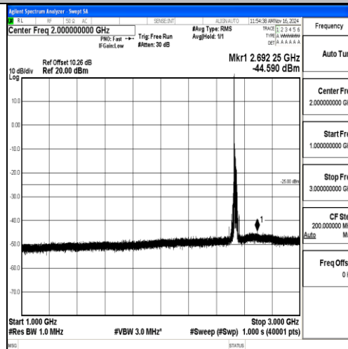
Band7-20MHz-16QAM-21100-1RB#0-1000~3000-PASS
