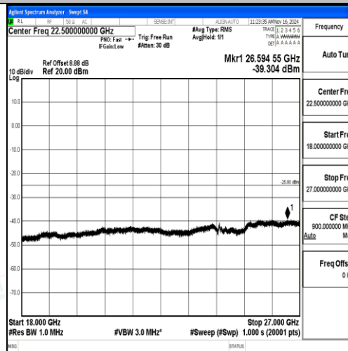
Band7-15MHz-QPSK-21375-1RB#0-18000~27000-PASS
