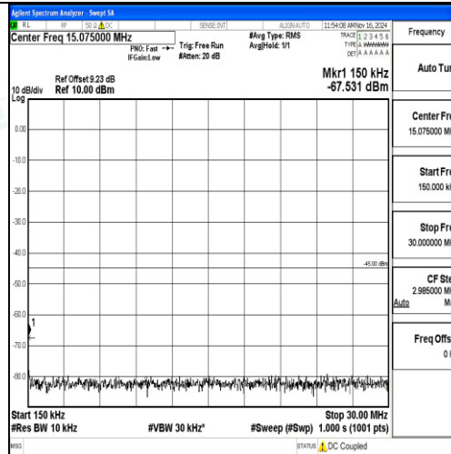
Band7-20MHz-16QAM-21100-1RB#0-0.15~30-PASS
