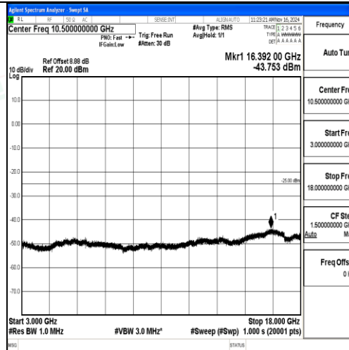
Band7-15MHz-QPSK-21375-1RB#0-3000~18000-PASS
