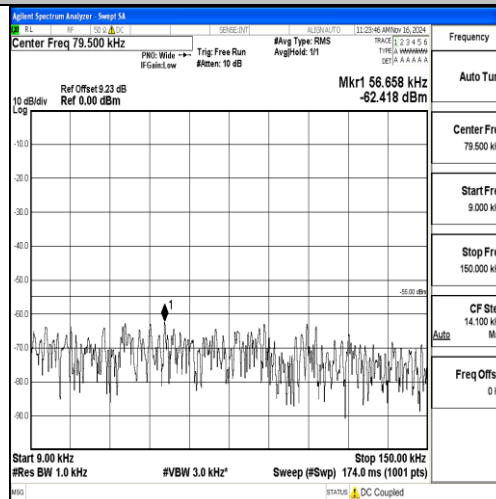
Band7-15MHz-16QAM-21375-1RB#0-0.009~0.15-PASS
