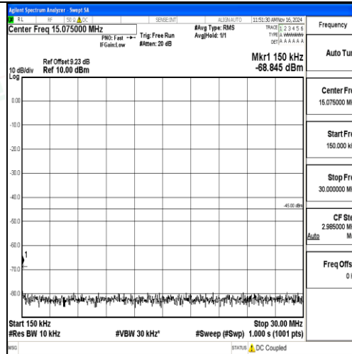
Band7-20MHz-16QAM-20850-1RB#0-0.15~30-PASS
