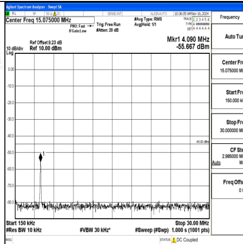
Band7-5MHz-16QAM-21425-1RB#0-0.15~30-PASS
