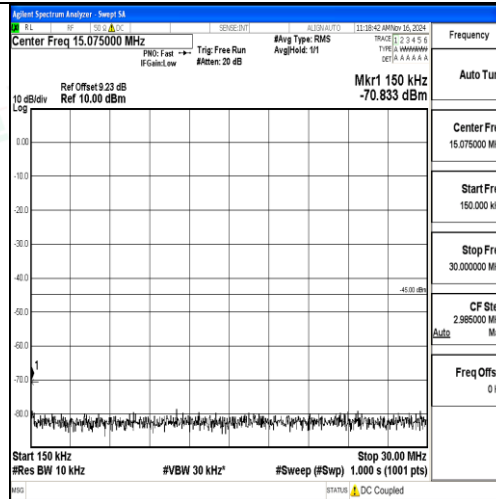
Band7-15MHz-16QAM-20825-1RB#0-0.15~30-PASS
