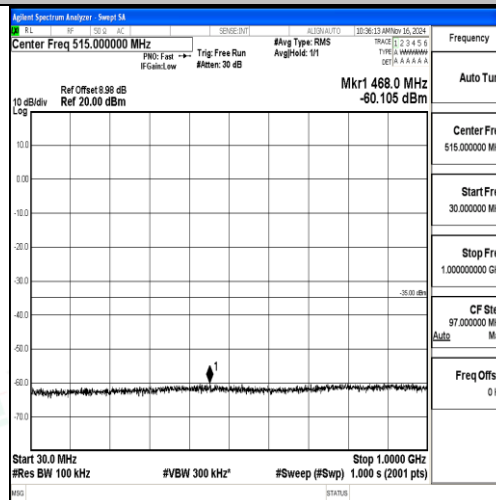
Band7-5MHz-16QAM-21425-1RB#0-30~1000-PASS
