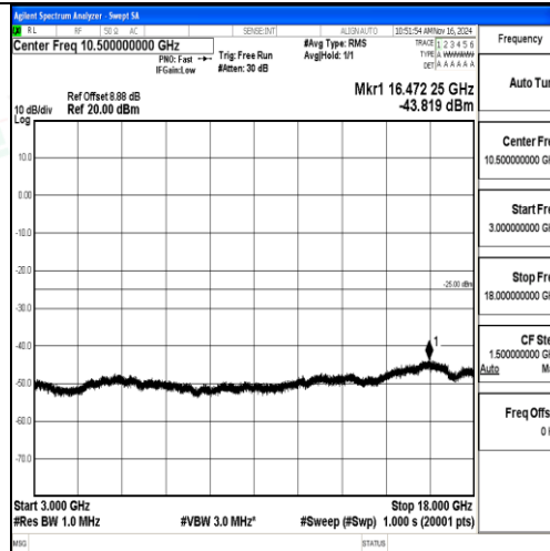
Band7-10MHz-QPSK-20800-1RB#0-3000~18000-PASS
