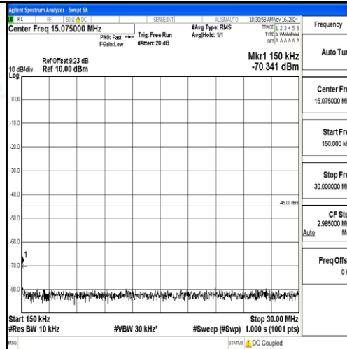
Band7-5MHz-16QAM-20775-1RB#0-0.15~30-PASS
