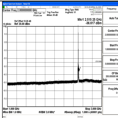
Band7-5MHz-16QAM-20775-1RB#0-1000~3000-PASS
