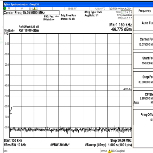
Band7-10MHz-16QAM-21100-1RB#0-0.15~30-PASS
