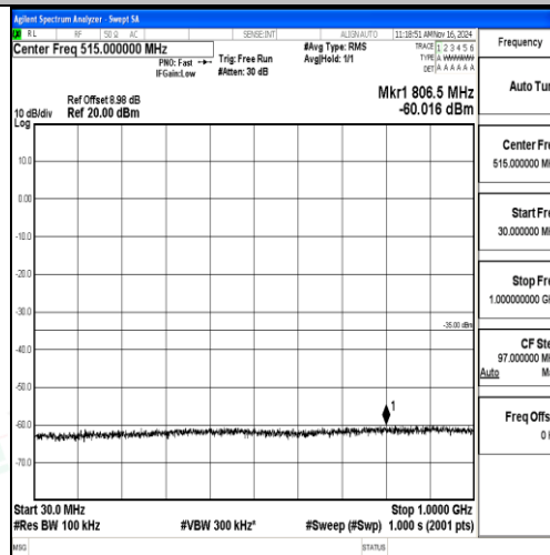
Band7-15MHz-16QAM-20825-1RB#0-30~1000-PASS
