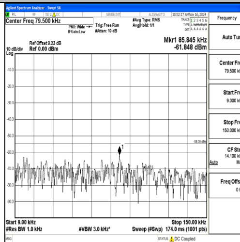
Band7-10MHz-16QAM-20800-1RB#0-0.009~0.15-PASS
