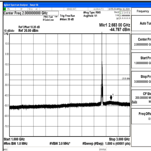
Band7-10MHz-16QAM-21100-1RB#0-1000~3000-PASS
