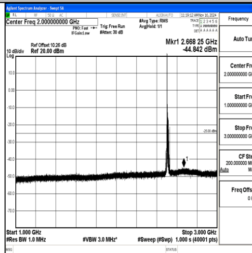
Band7-15MHz-16QAM-20825-1RB#0-1000~3000-PASS
