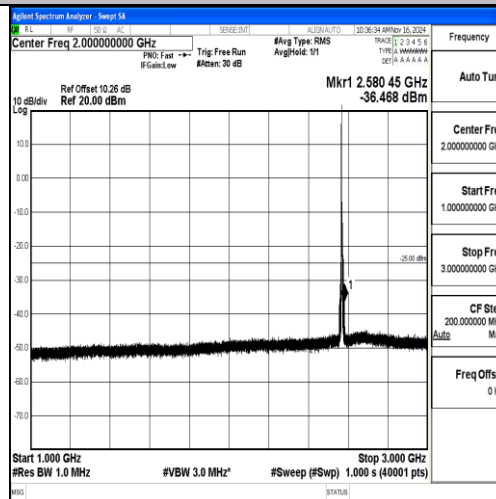
Band7-5MHz-16QAM-21425-1RB#0-1000~3000-PASS
