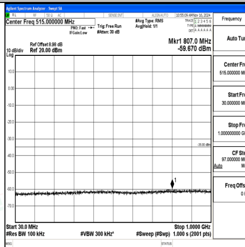
Band7-10MHz-16QAM-21100-1RB#0-0-30~1000-PASS
