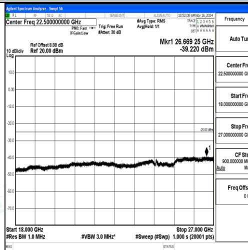
Band7-10MHz-QPSK-20800-1RB#0-18000~27000-PASS
