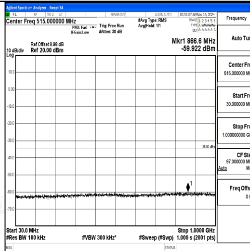
Band7-5MHz-16QAM-20775-1RB#0-30~1000-PASS
