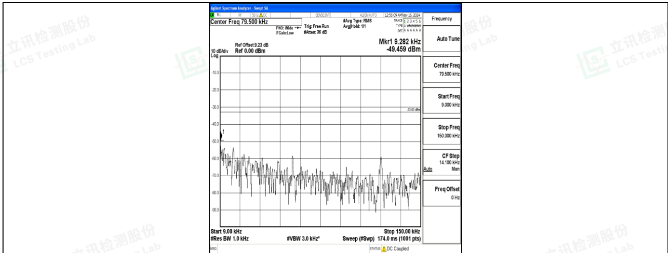
Band5-5MHz-QPSK-20425-1RB#0-0.009~0.15-PASS
