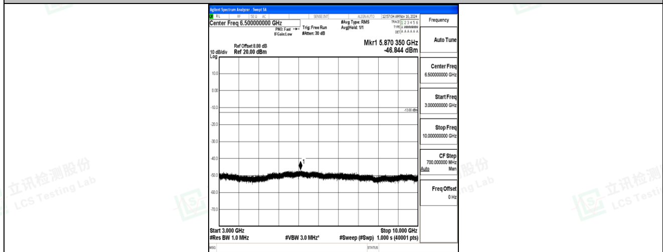
Band5-5MHz-QPSK-20425-1RB#0-3000~10000-PASS
