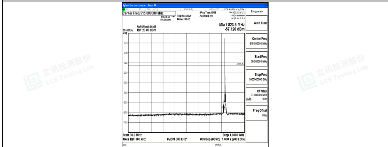
Band5-5MHz-16QAM-20525-1RB#0-30~1000-PASS
