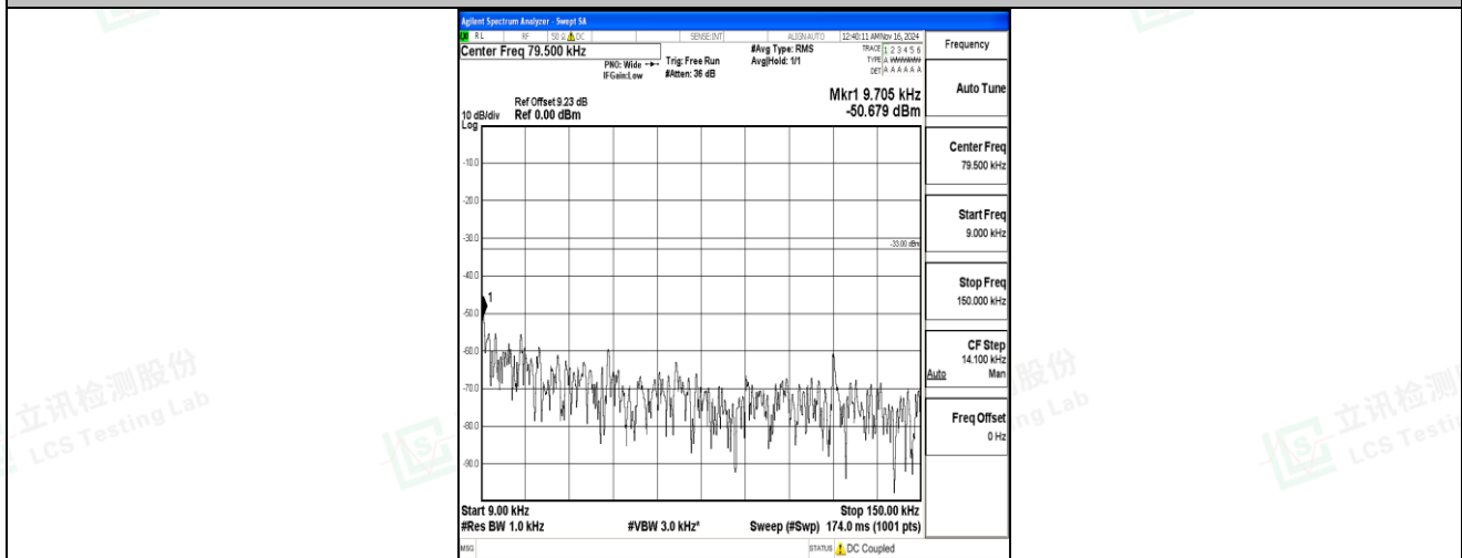
Band5-3MHz-16QAM-20635-1RB#0-0.009~0.15-PASS
