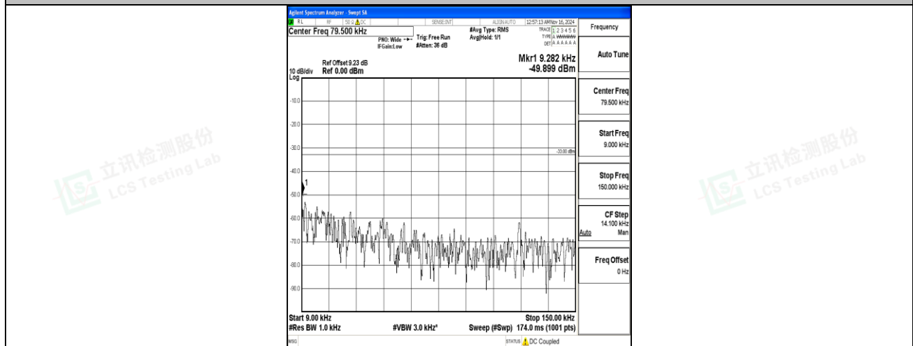
Band5-5MHz-16QAM-20425-1RB#0-0.009~0.15-PASS
