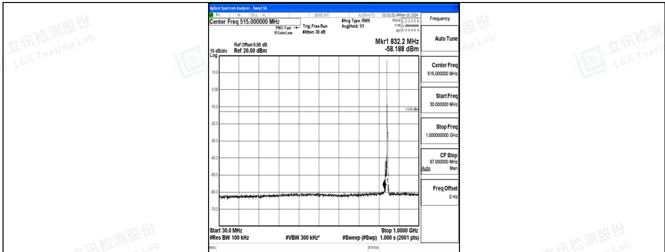
Band5-5MHz-16QAM-20625-1RB#0-30~1000-PASS
