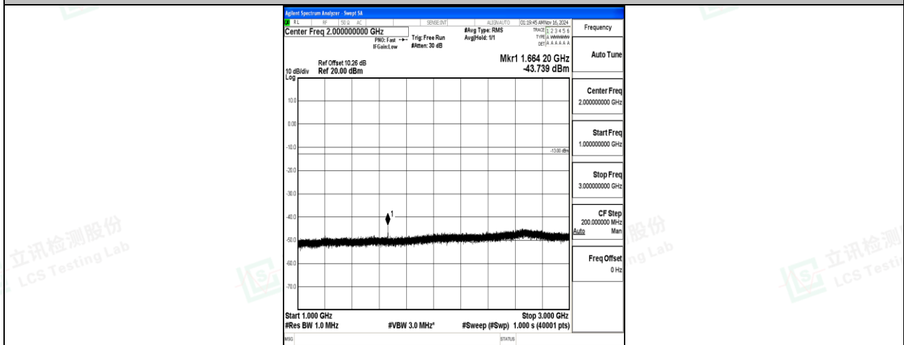
Band5-10MHz-QPSK-20525-1RB#0-1000~3000-PASS
