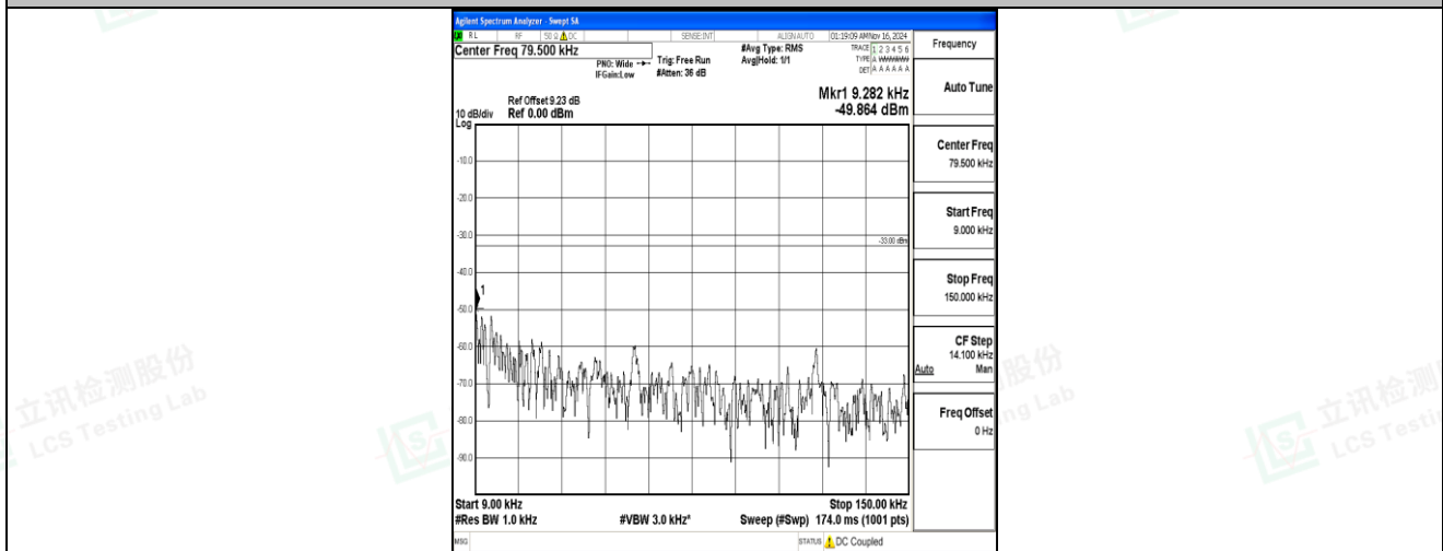
Band5-10MHz-QPSK-20525-1RB#0-0.009~0.15-PASS
