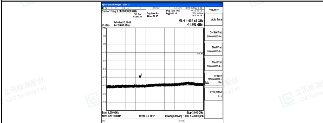
Band5-3MHz-16QAM-20635-1RB#0-1000~3000-PASS
