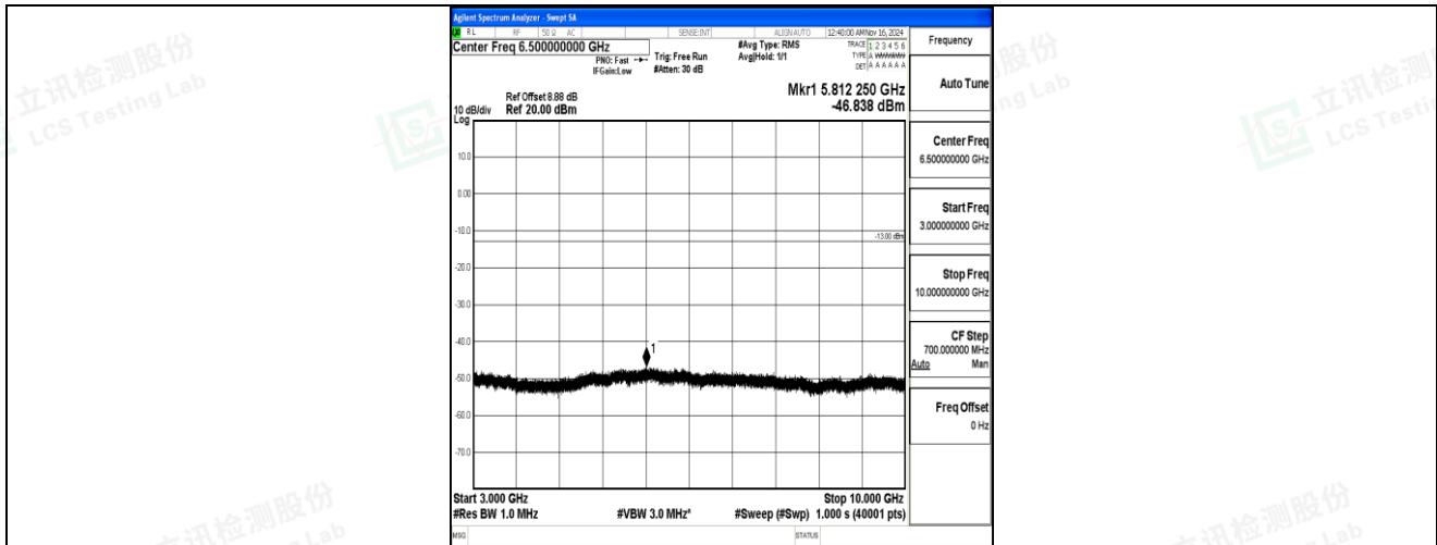
Band5-3MHz-QPSK-20635-1RB#0-3000~10000-PASS
