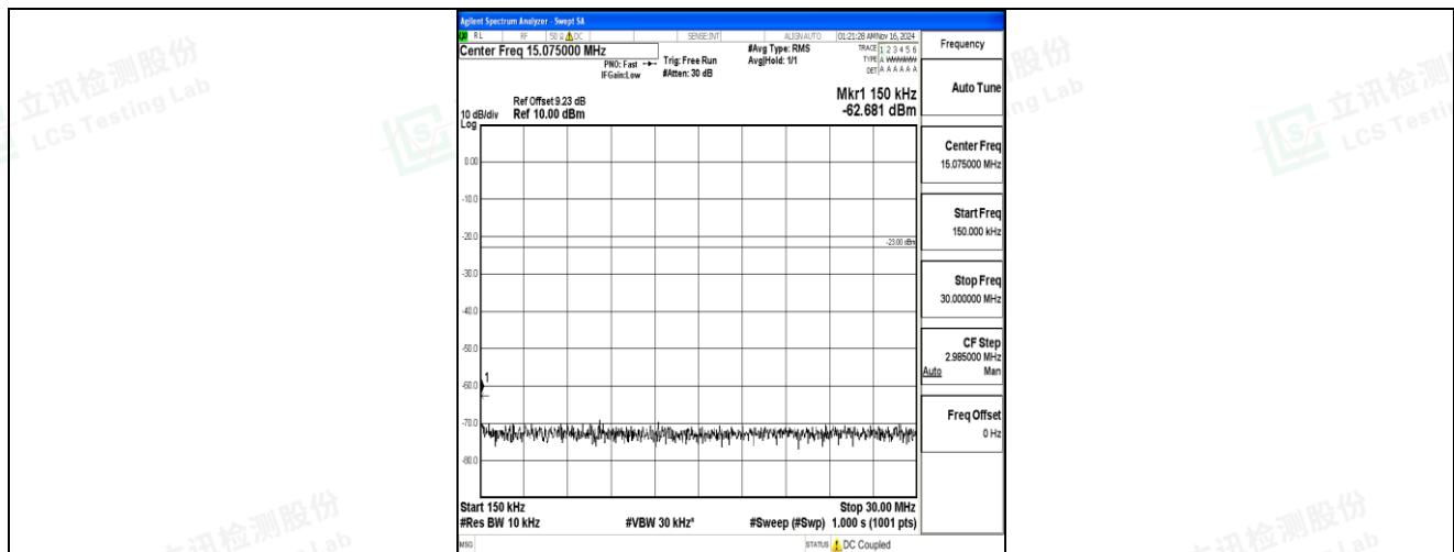
Band5-10MHz-QPSK-20600-1RB#0-0.15~30-PASS
