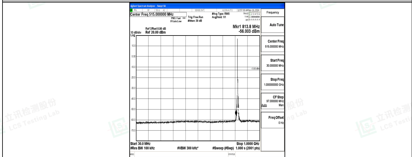
Band5-5MHz-16QAM-20425-1RB#0-30~1000-PASS
