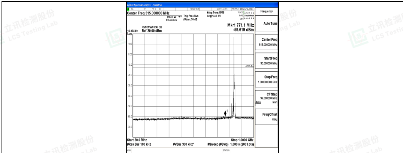
Band5-10MHz-16QAM-20600-1RB#0-30~1000-PASS
