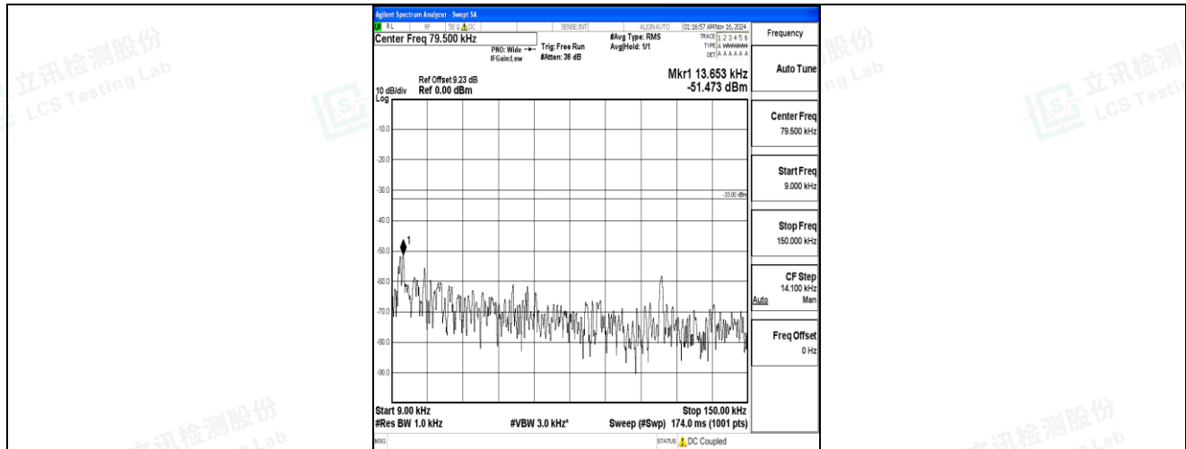
Band5-10MHz-QPSK-20450-1RB#0-0.009~0.15-PASS
