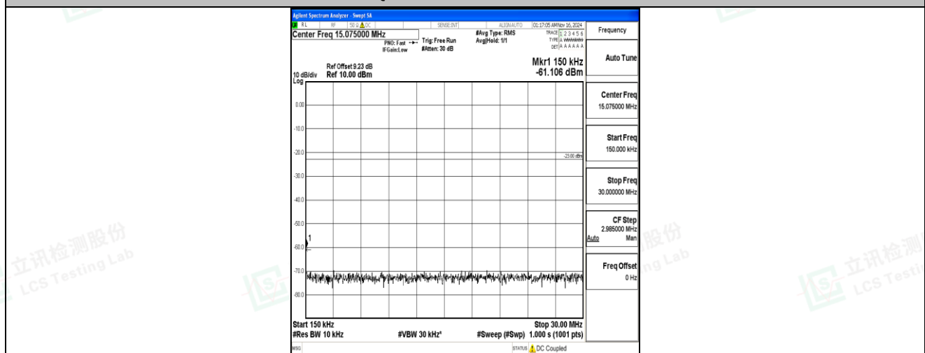
Band5-10MHz-QPSK-20450-1RB#0-0.15~30-PASS
