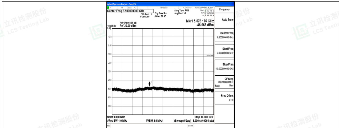
Band5-5MHz-QPSK-20625-1RB#0-3000~10000-PASS
