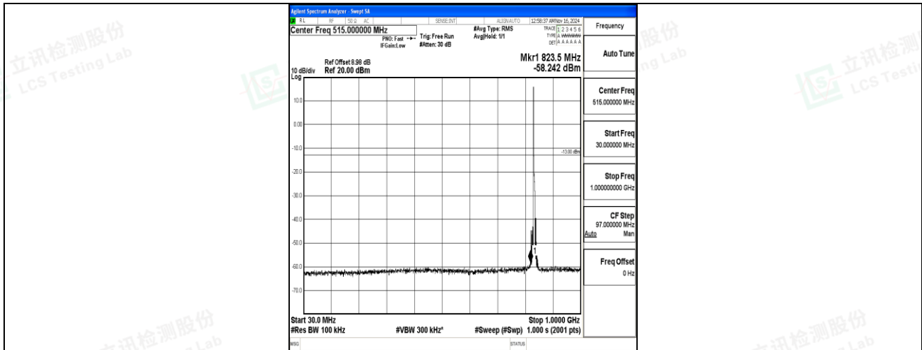
Band5-5MHz-QPSK-20525-1RB#0-30~1000-PASS
