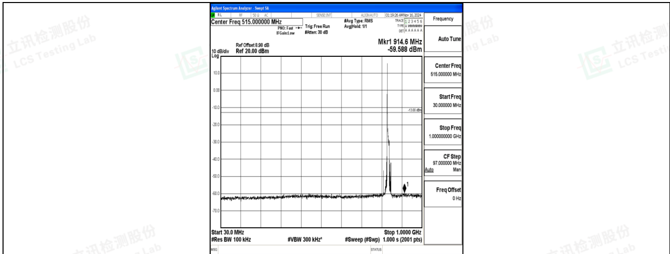
Band5-10MHz-QPSK-20525-1RB#0-30~1000-PASS
