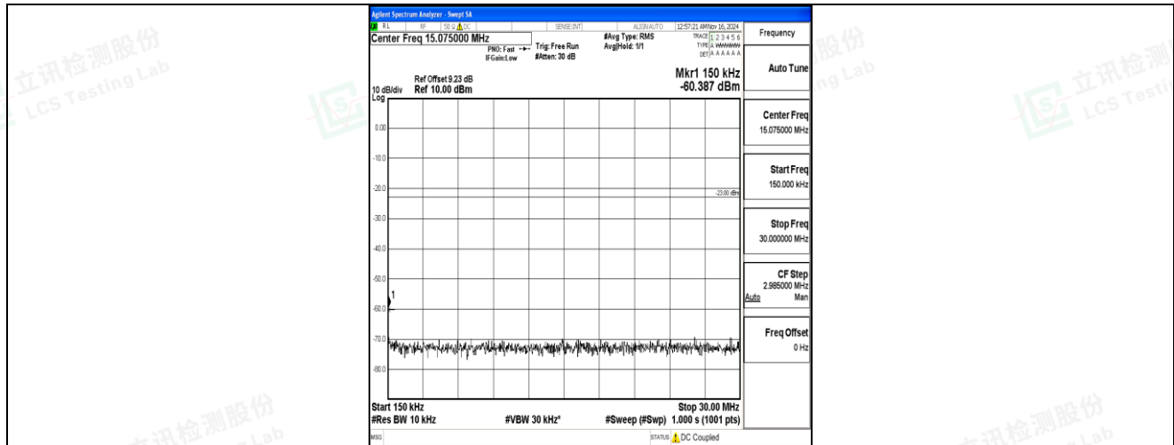
Band5-5MHz-16QAM-20425-1RB#0-0.15~30-PASS
