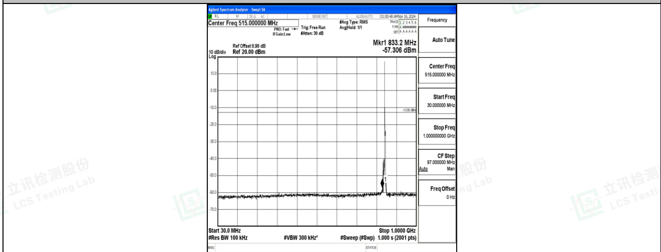
Band5-5MHz-QPSK-20625-1RB#0-30~1000-PASS
