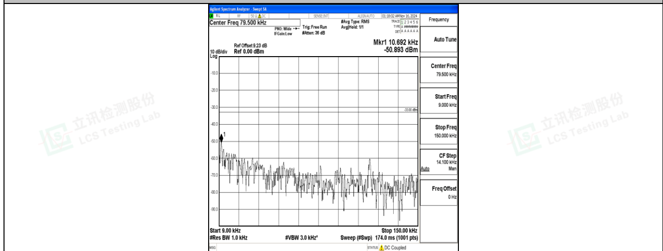
Band5-10MHz-16QAM-20450-1RB#0-0.009~0.15-PASS
