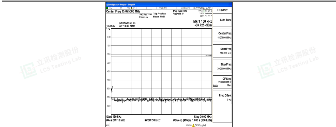
Band5-10MHz-16QAM-20600-1RB#0-0.15~30-PASS
