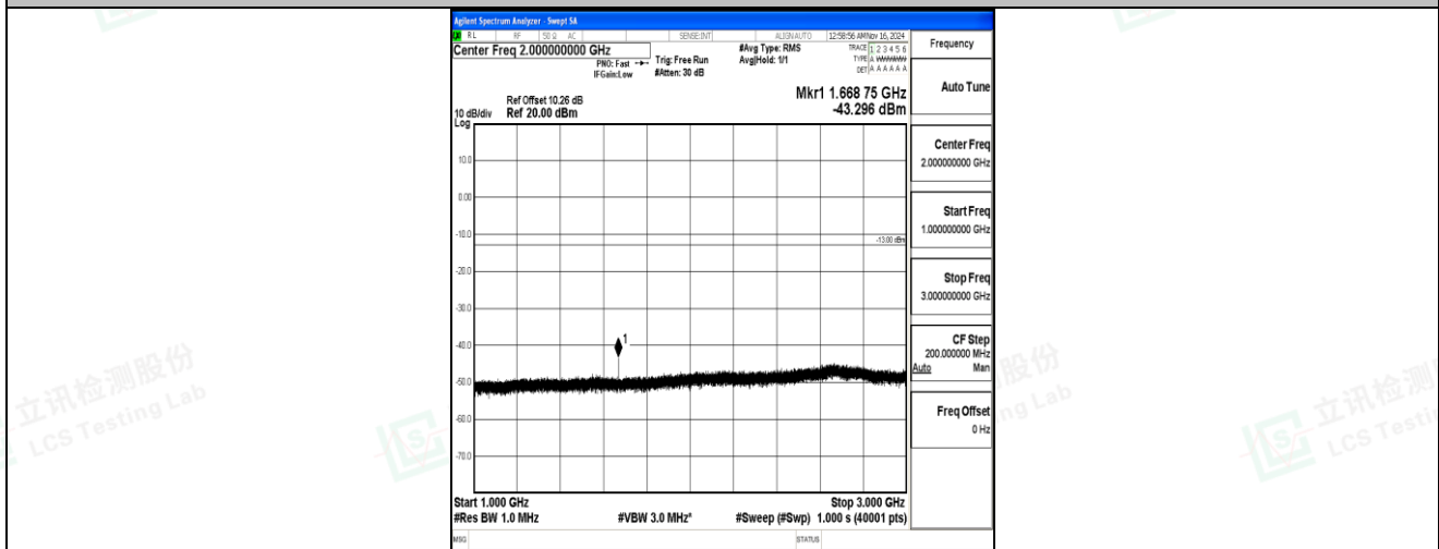
Band5-5MHz-QPSK-20525-1RB#0-1000~3000-PASS
