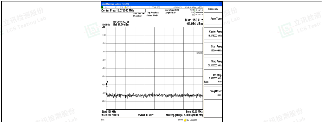
Band5-5MHz-QPSK-20625-1RB#0-0.15~30-PASS
