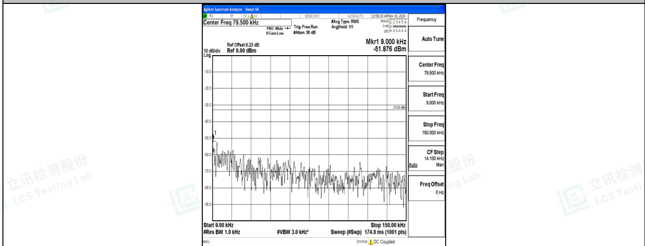
Band5-5MHz-QPSK-20525-1RB#0-0.009~0.15-PASS
