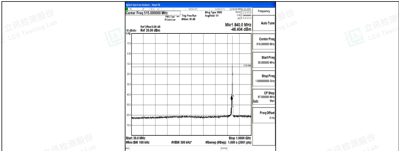
Band5-3MHz-16QAM-20635-1RB#0-30~1000-PASS
