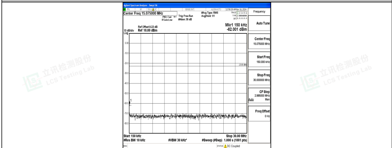
Band5-5MHz-QPSK-20525-1RB#0-0.15~30-PASS
