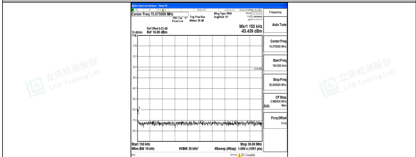
Band5-5MHz-16QAM-20625-1RB#0-0.15~30-PASS
