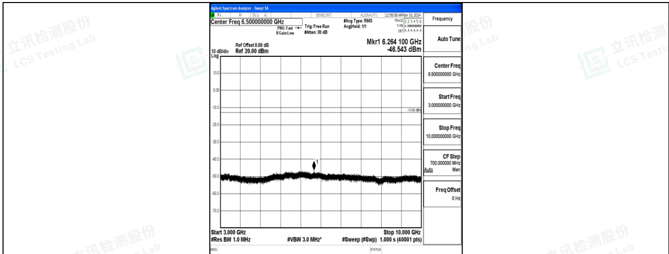
Band5-5MHz-16QAM-20425-1RB#0-3000~10000-PASS
