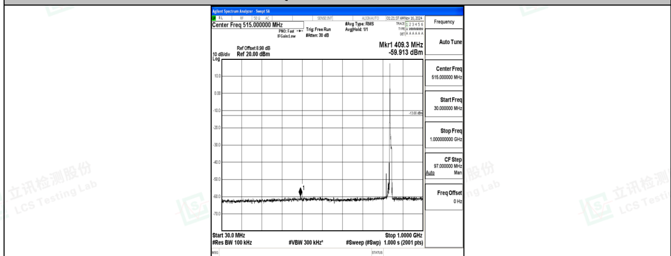
Band5-10MHz-QPSK-20600-1RB#0-30~1000-PASS
