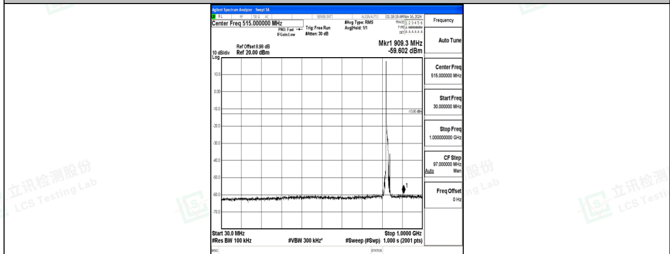
Band5-10MHz-16QAM-20450-1RB#0-30~1000-PASS
