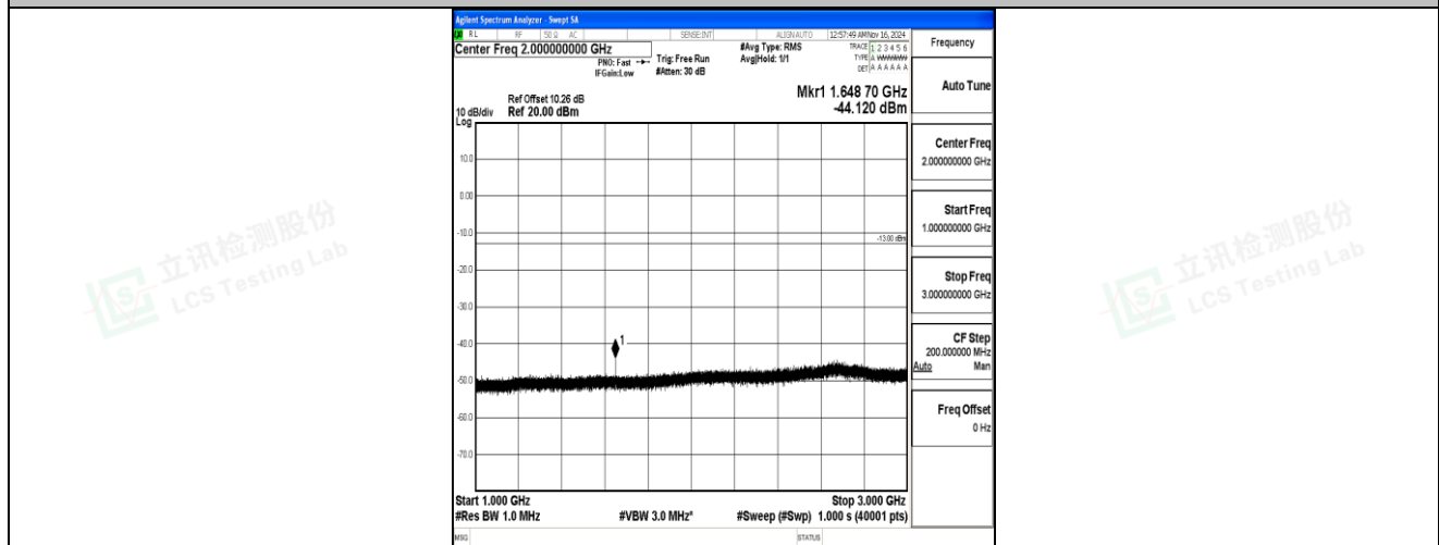
Band5-5MHz-16QAM-20425-1RB#0-1000~3000-PASS
