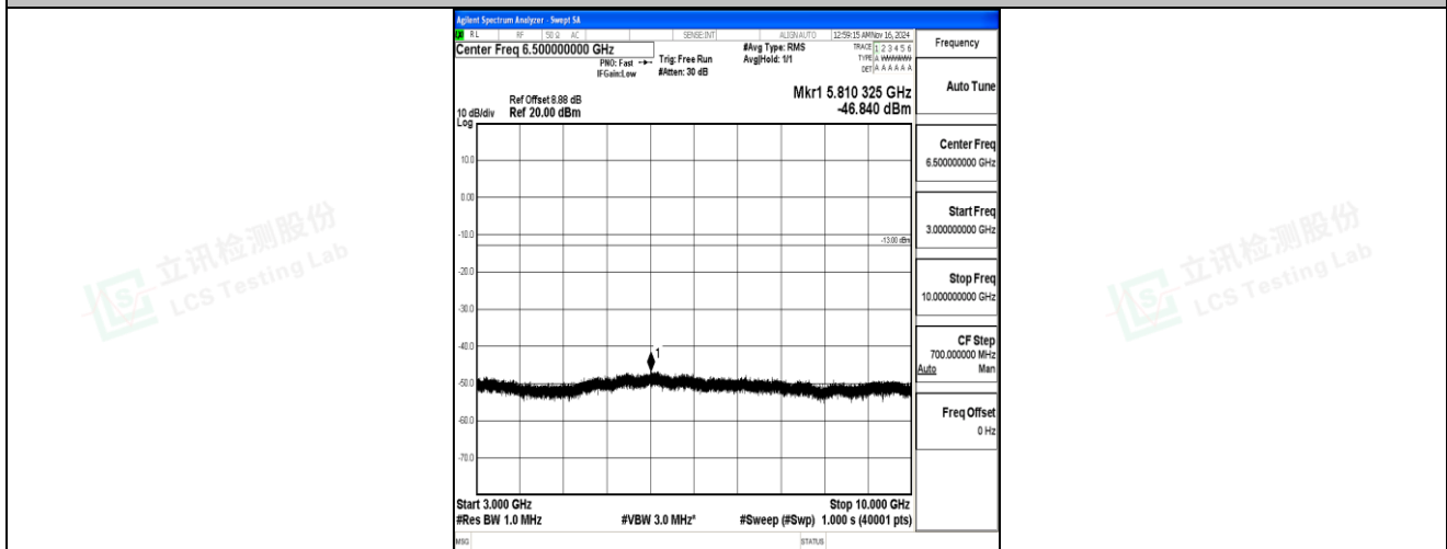
Band5-5MHz-QPSK-20525-1RB#0-3000~10000-PASS
