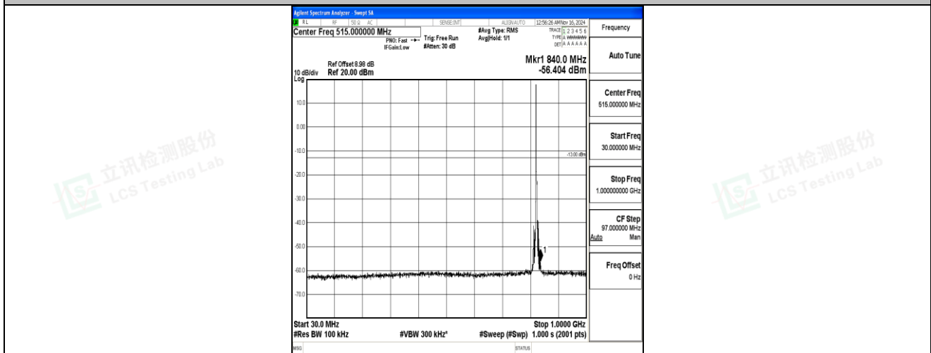
Band5-5MHz-QPSK-20425-1RB#0-30~1000-PASS
