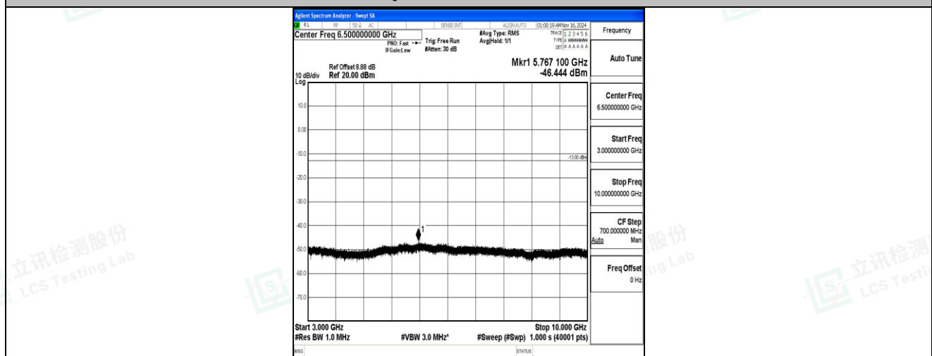
Band5-5MHz-16QAM-20525-1RB#0-3000~10000-PASS
