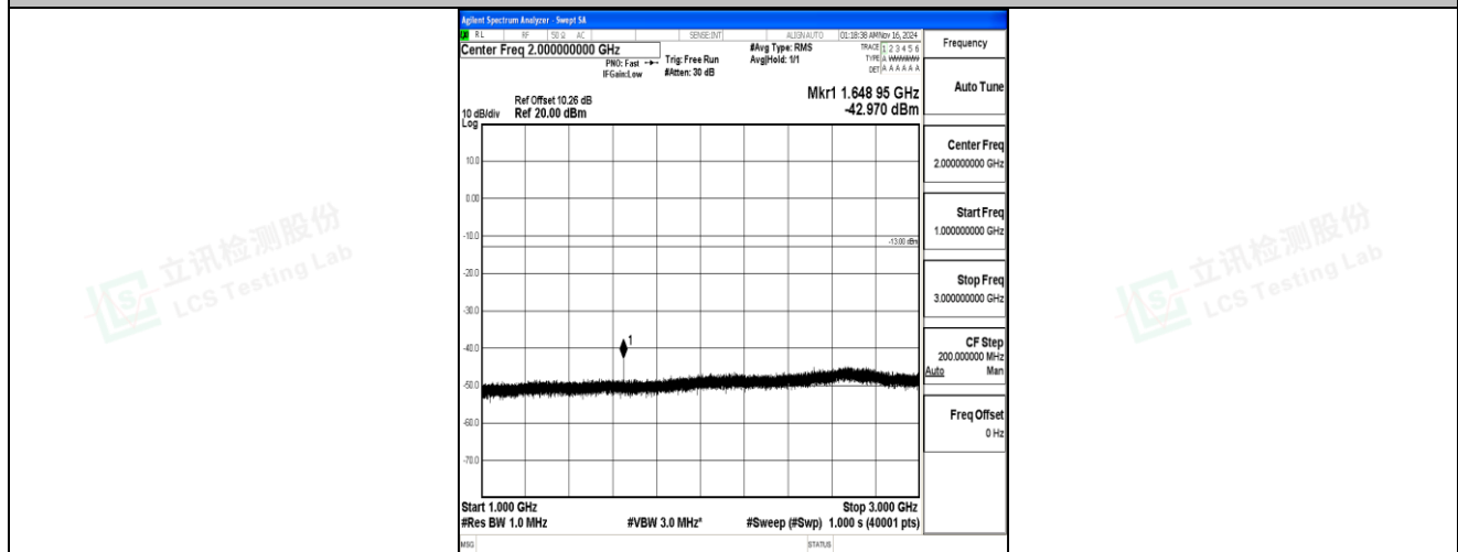
Band5-10MHz-16QAM-20450-1RB#0-1000~3000-PASS
