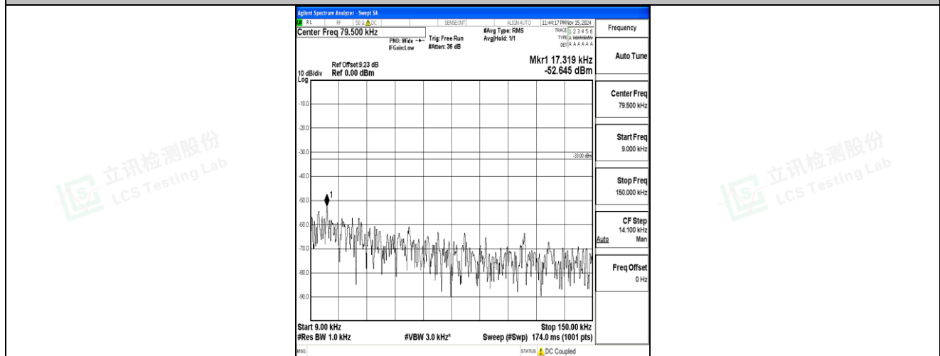
Band5-1.4MHz-16QAM-20407-1RB#0-0.009~0.15-PASS
