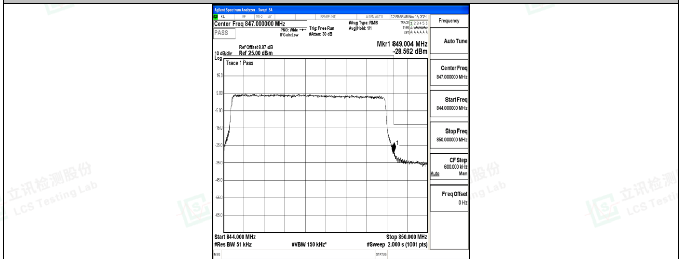
Band5-5MHz-16QAM-20625-25RB#0-PASS
