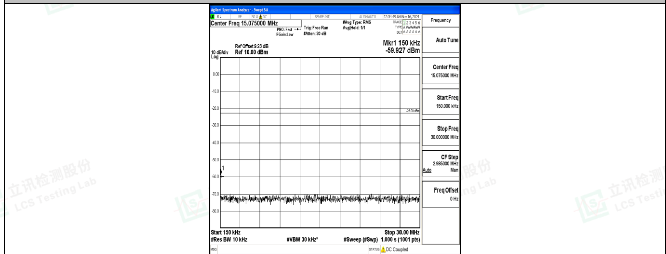
Band5-3MHz-QPSK-20415-1RB#0-0.15~30-PASS
