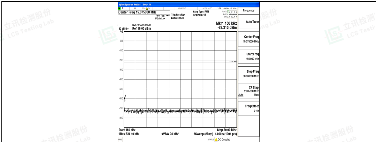
Band5-3MHz-QPSK-20635-1RB#0-0.15~30-PASS
