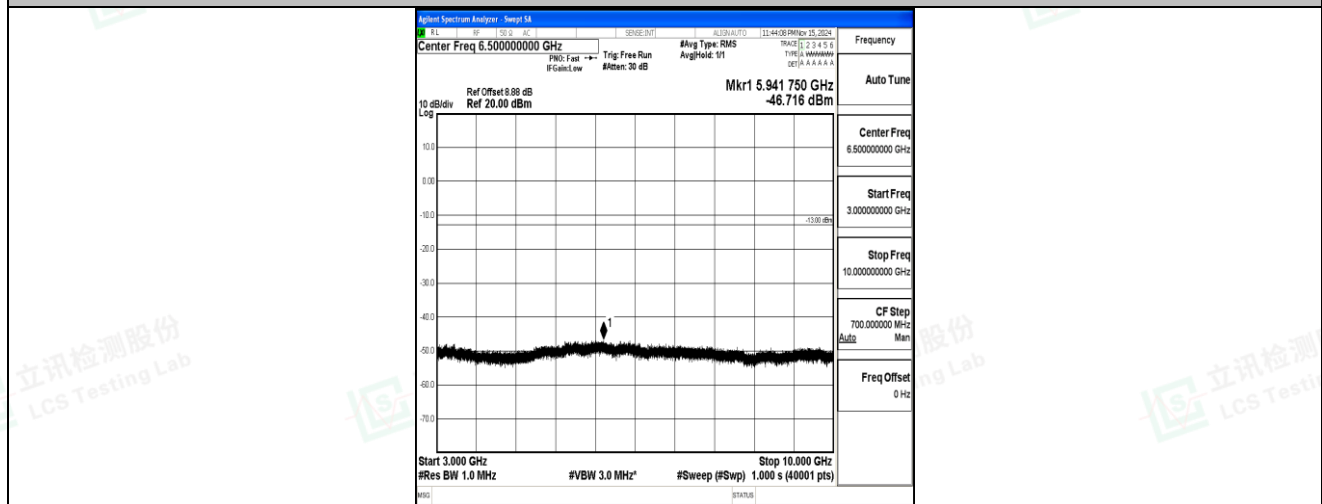
Band5-1.4MHz-QPSK-20407-1RB#0-3000~10000-PASS
