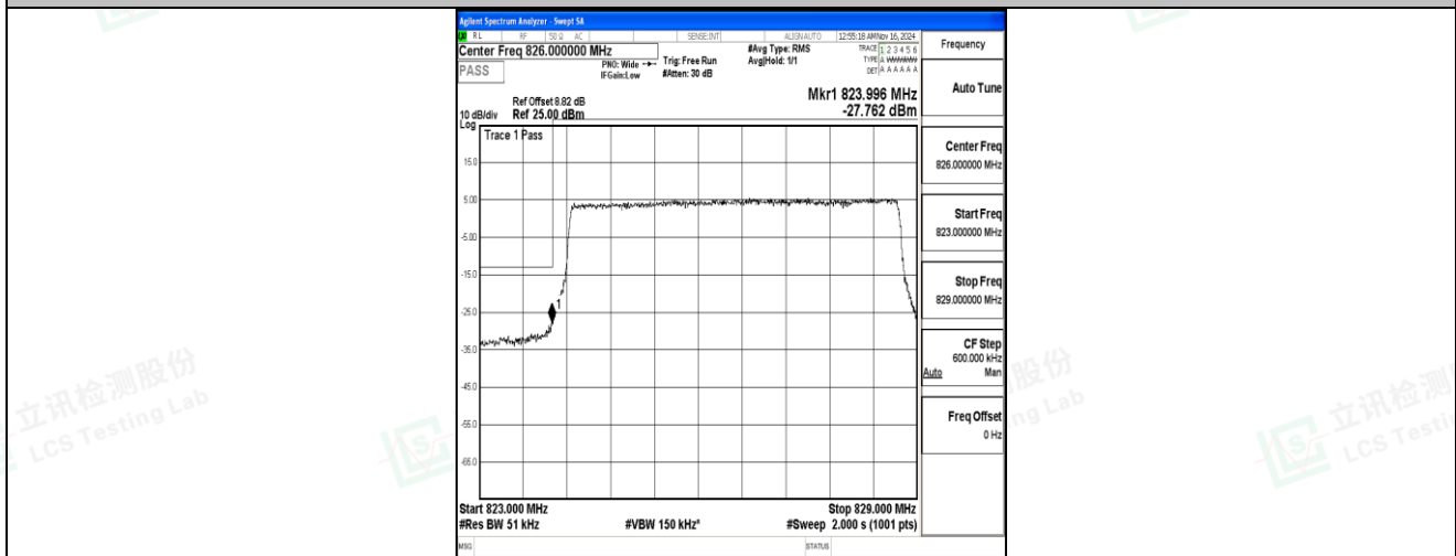
Band5-5MHz-QPSK-20425-25RB#0-PASS
