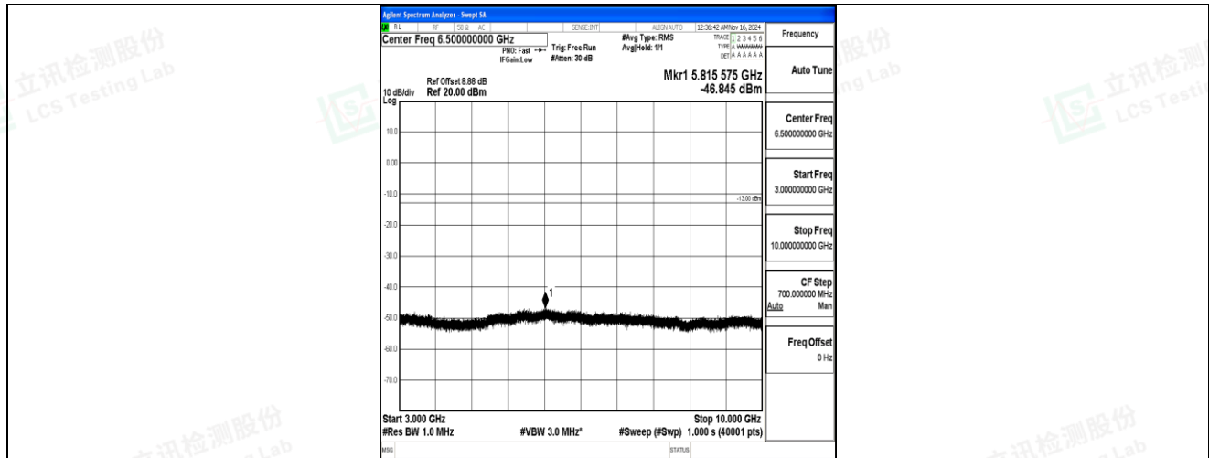
Band5-3MHz-16QAM-20415-1RB#0-3000~10000-PASS
