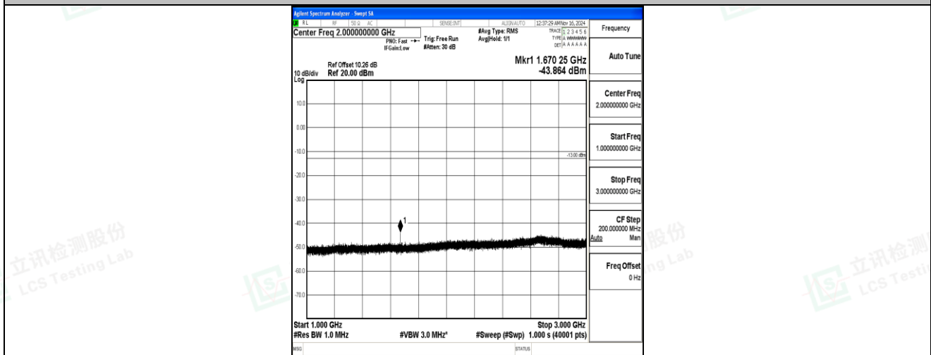
Band5-3MHz-QPSK-20525-1RB#0-1000~3000-PASS
