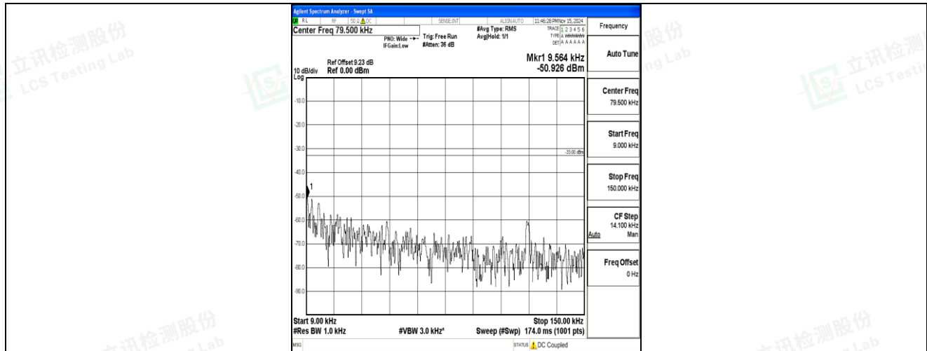
Band5-1.4MHz-16QAM-20525-1RB#0-0.009~0.15-PASS
