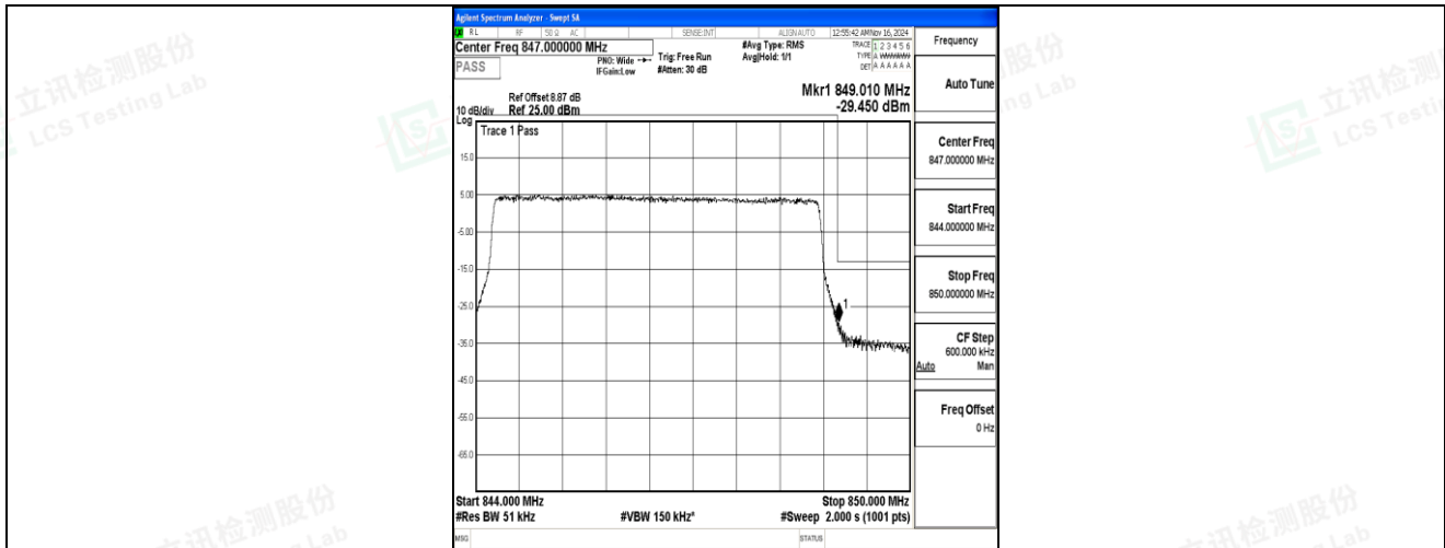
Band5-5MHz-QPSK-20625-25RB#0-PASS
