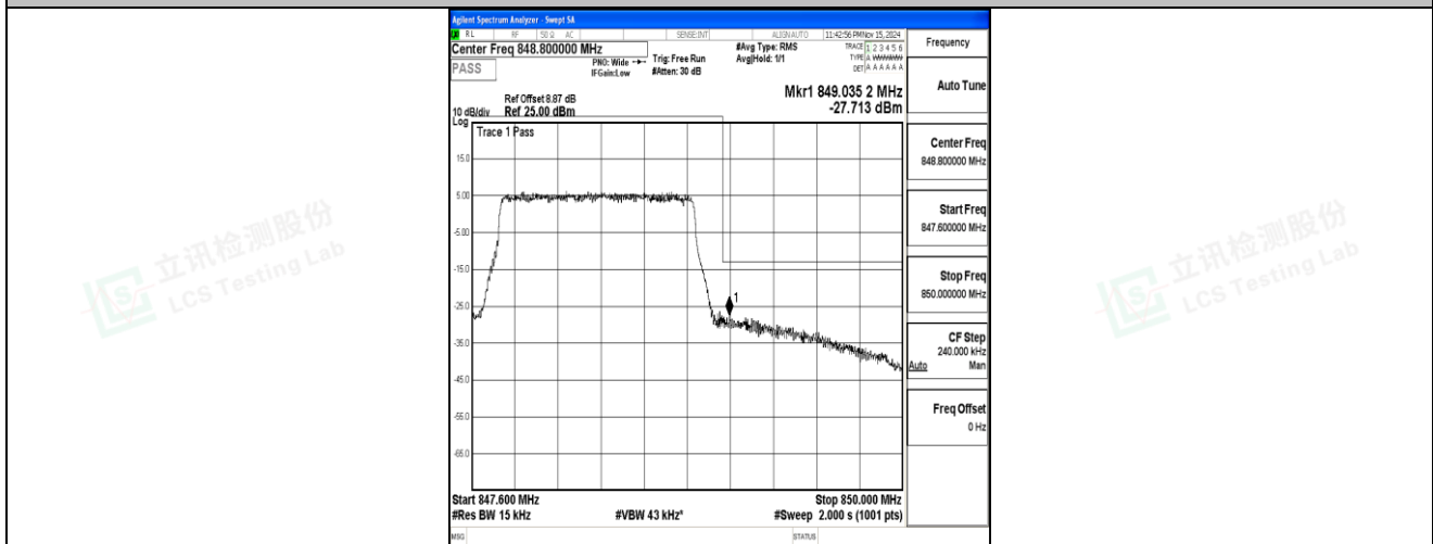
Band5-1.4MHz-16QAM-20643-6RB#0-PASS
