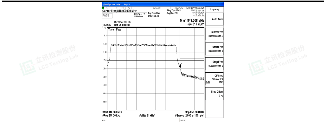
Band5-3MHz-QPSK-20635-15RB#0-PASS
