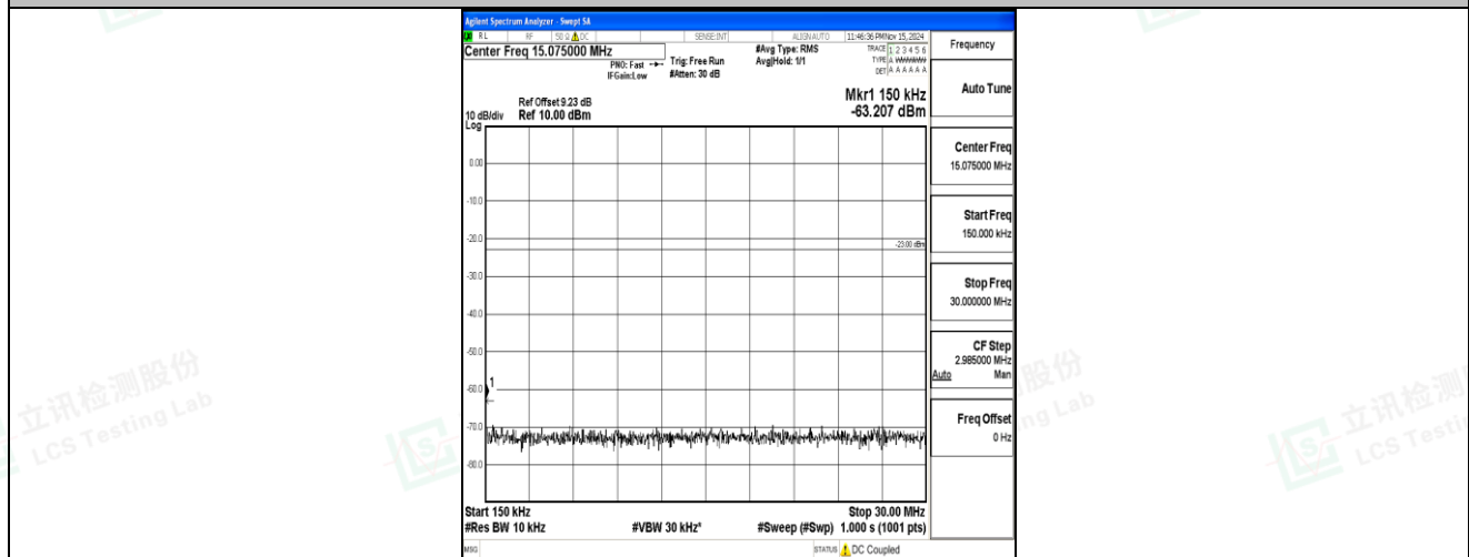
Band5-1.4MHz-16QAM-20525-1RB#0-0.15~30-PASS
