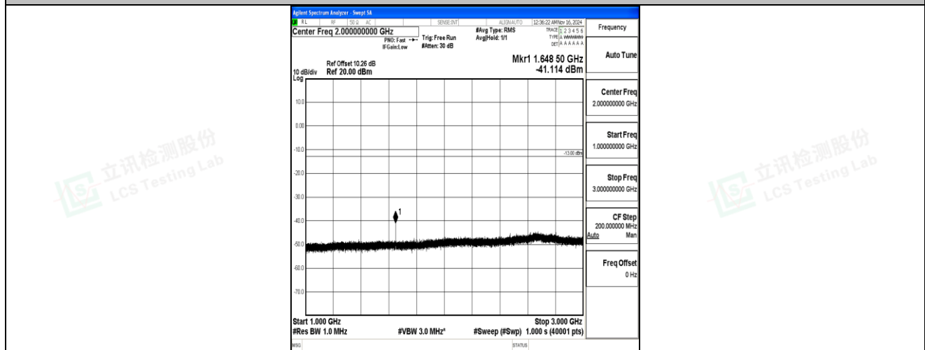
Band5-3MHz-16QAM-20415-1RB#0-1000~3000-PASS
