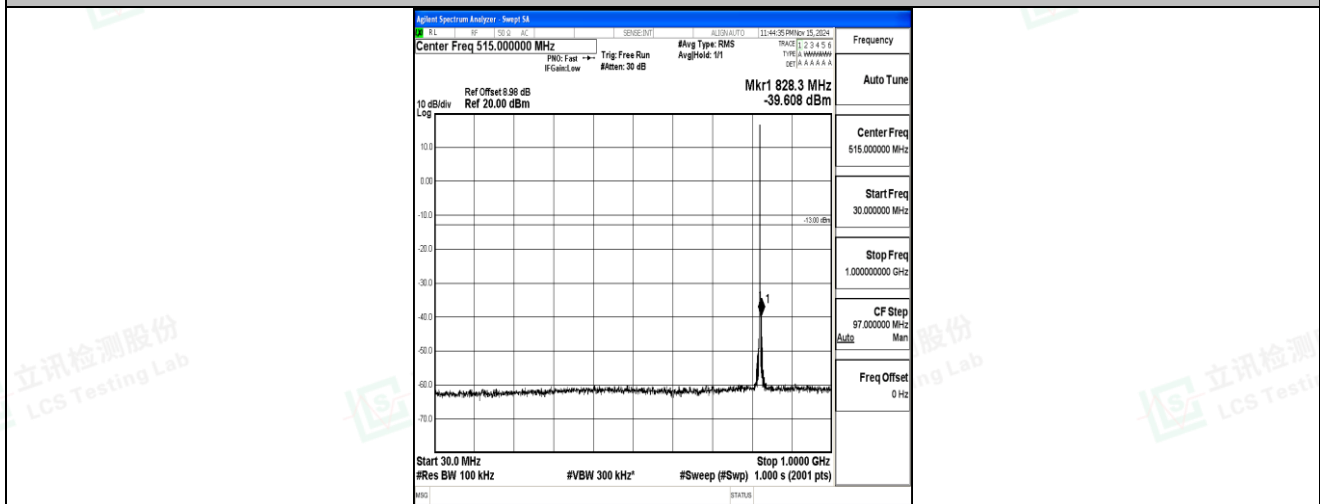
Band5-1.4MHz-16QAM-20407-1RB#0-30~1000-PASS
