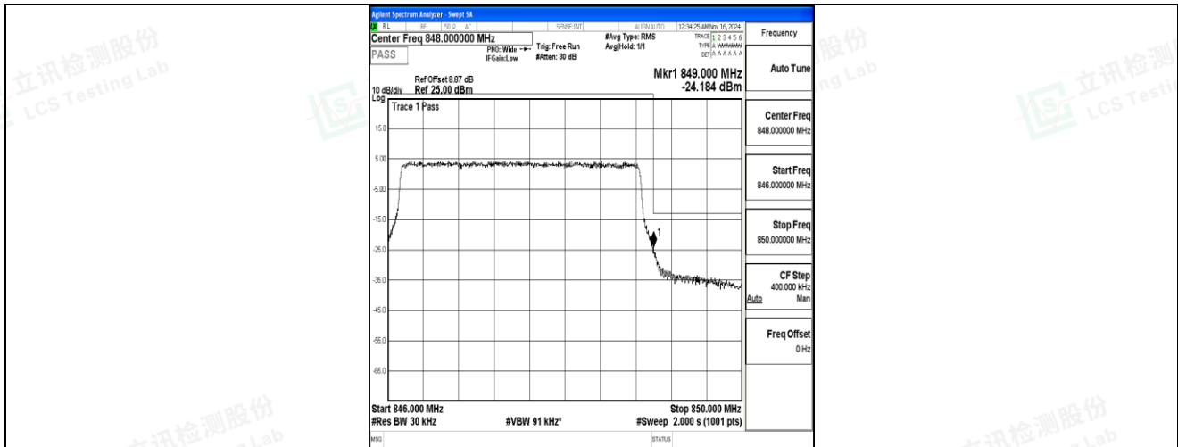
Band5-3MHz-16QAM-20635-15RB#0-PASS
