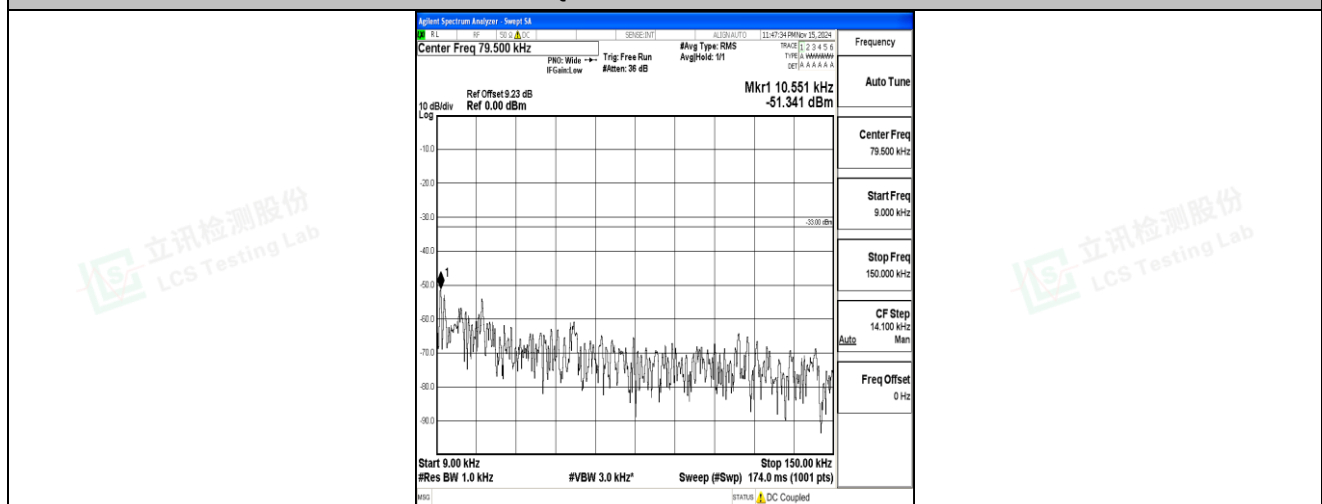
Band5-1.4MHz-QPSK-20643-1RB#0-0.009~0.15-PASS
