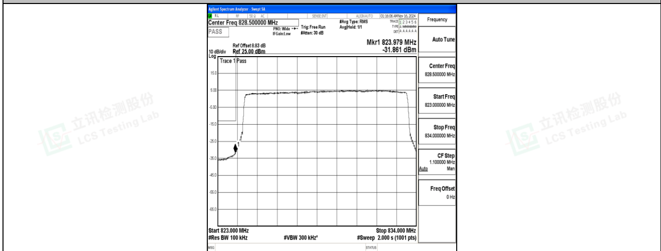
Band5-10MHz-QPSK-20450-50RB#0-PASS
