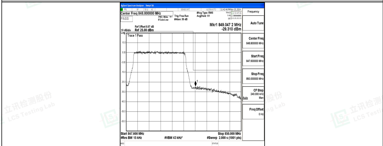
Band5-1.4MHz-QPSK-20643-6RB#0-PASS
