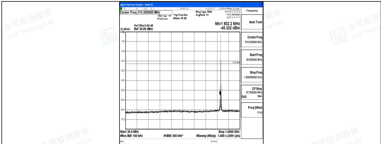
Band5-1.4MHz-QPSK-20525-1RB#0-30~1000-PASS
