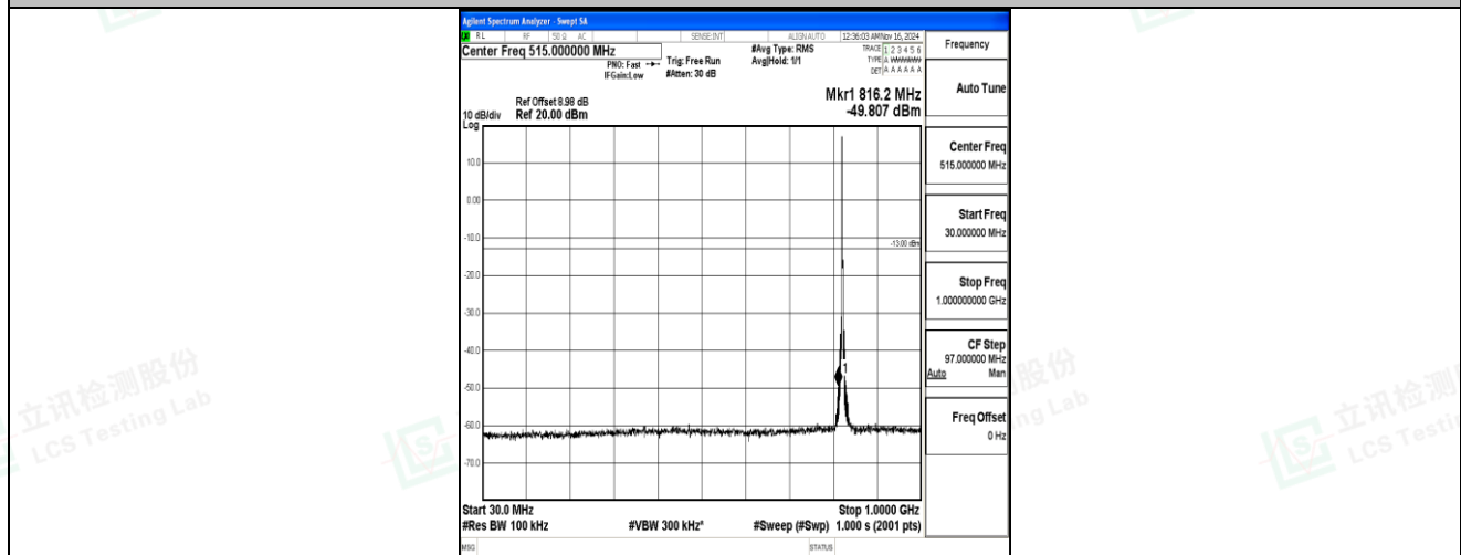
Band5-3MHz-16QAM-20415-1RB#0-30~1000-PASS
