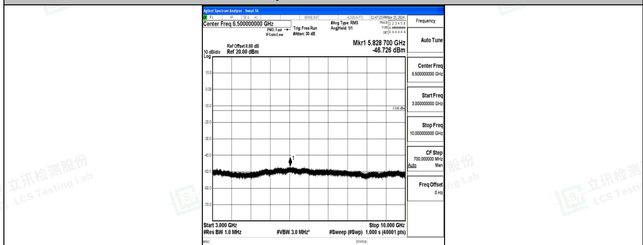
Band5-1.4MHz-16QAM-20525-1RB#0-3000~10000-PASS
