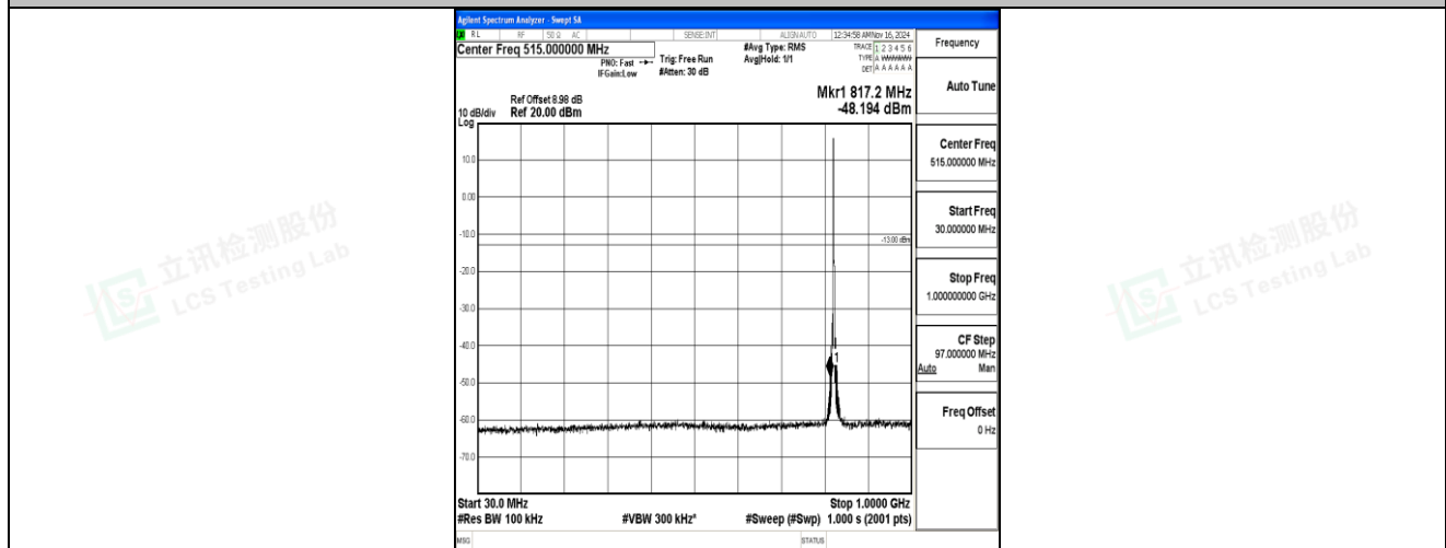
Band5-3MHz-QPSK-20415-1RB#0-30~1000-PASS
