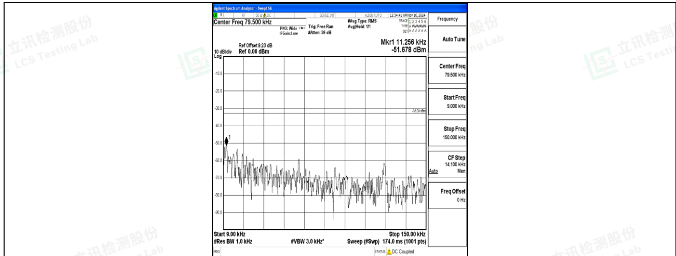
Band5-3MHz-QPSK-20415-1RB#0-0.009~0.15-PASS
