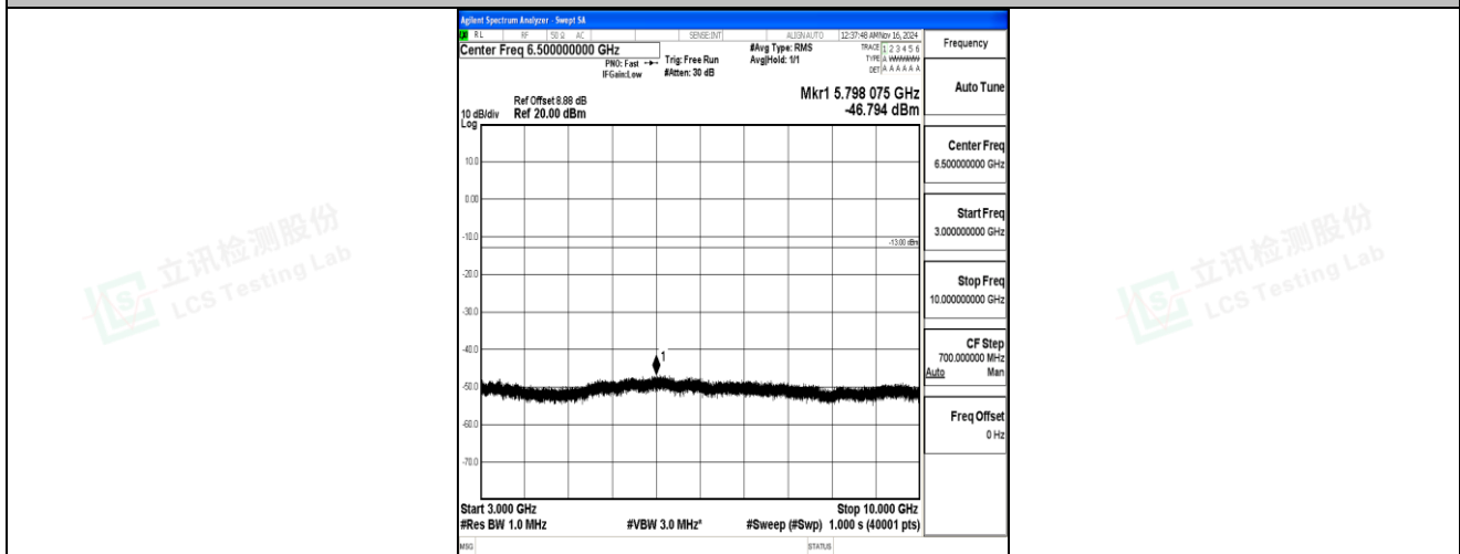
Band5-3MHz-QPSK-20525-1RB#0-3000~10000-PASS
