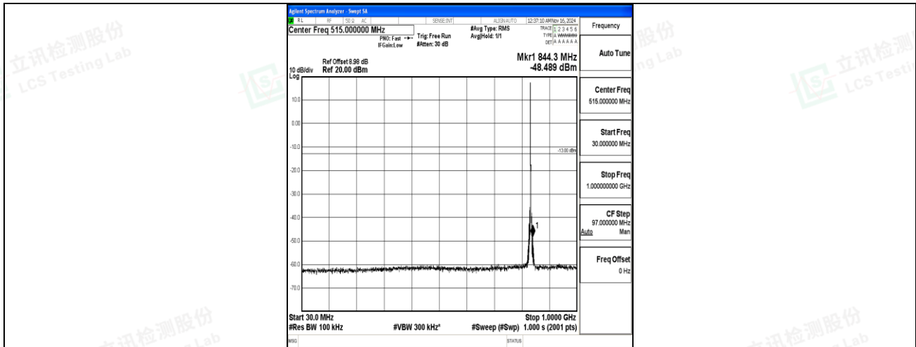
Band5-3MHz-QPSK-20525-1RB#0-30~1000-PASS
