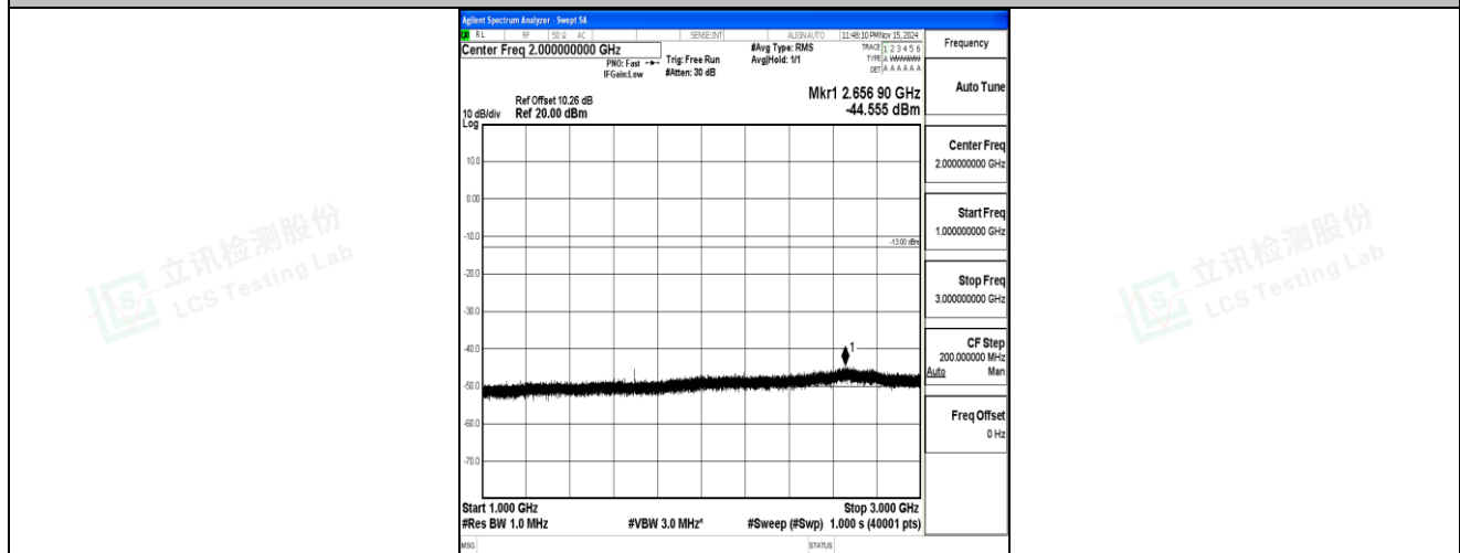
Band5-1.4MHz-QPSK-20643-1RB#0-1000~3000-PASS
