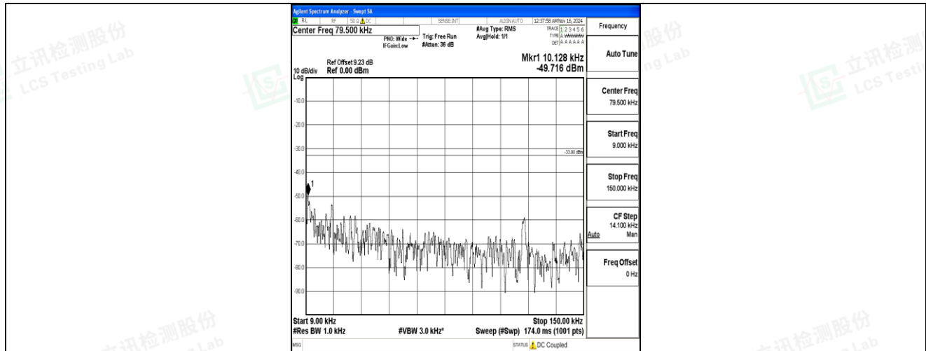
Band5-3MHz-16QAM-20525-1RB#0-0.009~0.15-PASS
