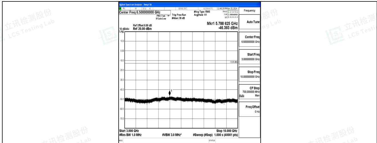
Band5-1.4MHz-QPSK-20643-1RB#0-3000~10000-PASS
