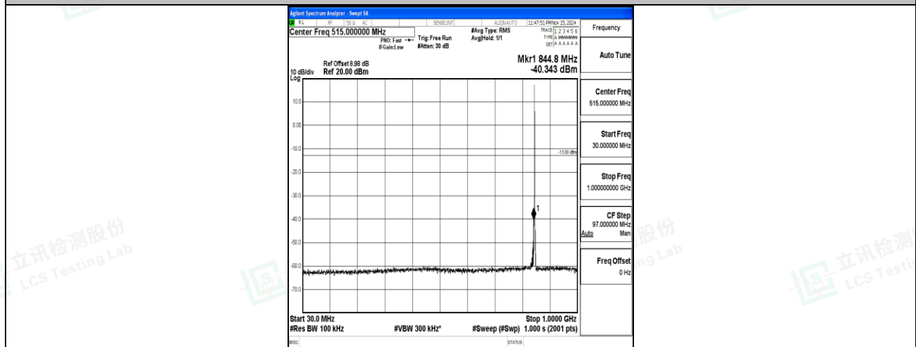
Band5-1.4MHz-QPSK-20643-1RB#0-30~1000-PASS
