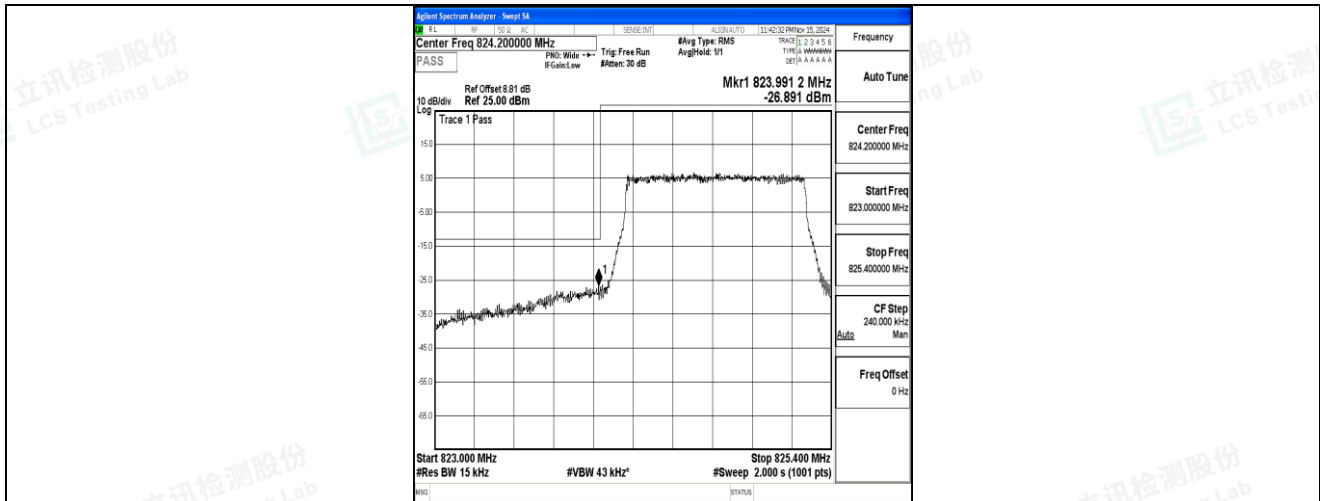
Band5-1.4MHz-16QAM-20407-6RB#0-PASS
