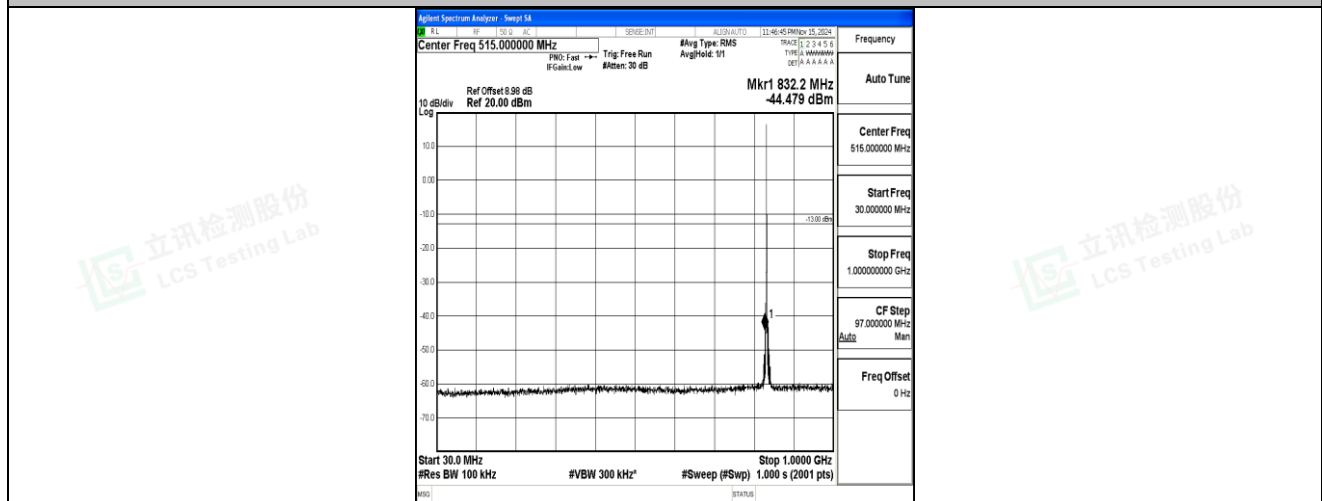
Band5-1.4MHz-16QAM-20525-1RB#0-30~1000-PASS
