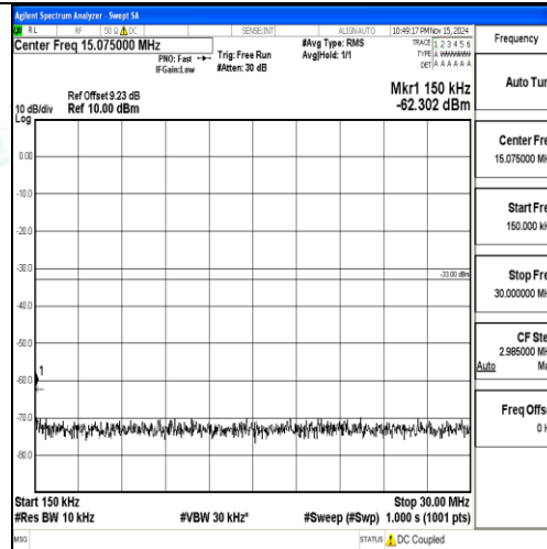
Band2-15MHz-16QAM-19125-1RB#0-0.15~30-PASS
