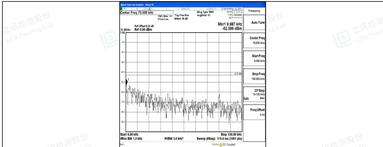
Band2-15MHz-QPSK-19125-1RB#0-0.009~0.15-PASS
