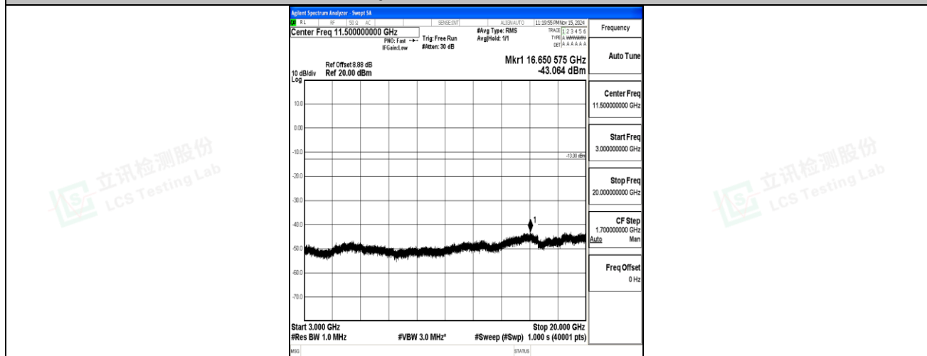
Band2-20MHz-QPSK-18700-1RB#0-3000~20000-PASS
