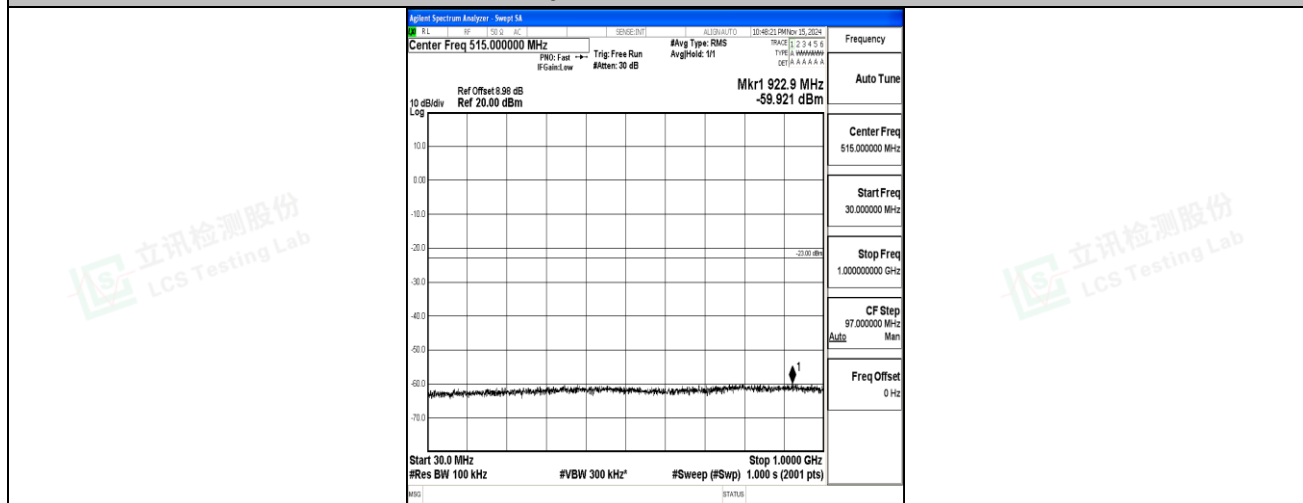
Band2-15MHz-QPSK-19125-1RB#0-30~1000-PASS
