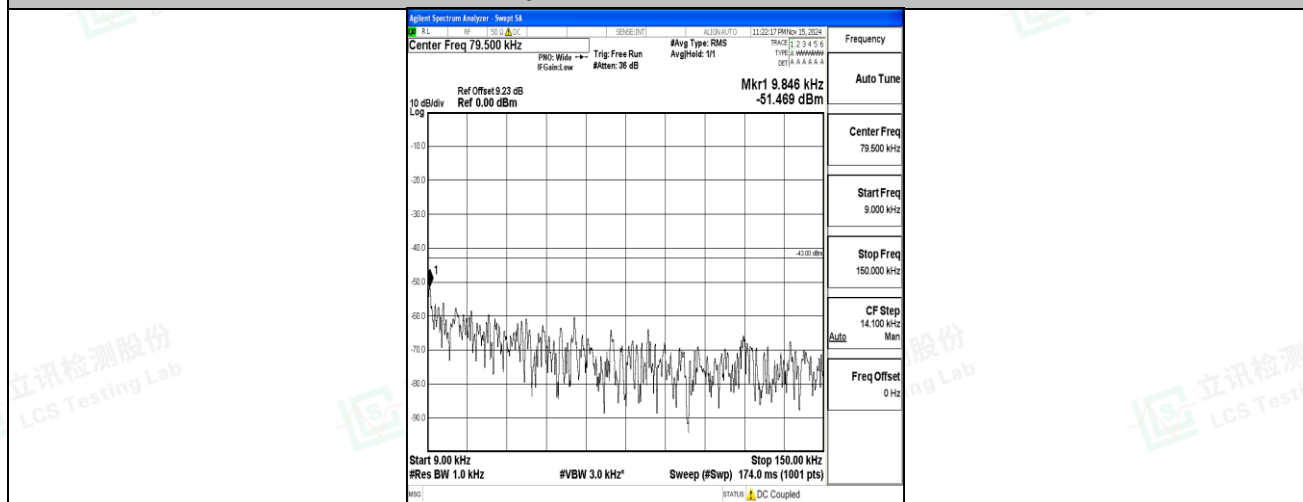
Band2-20MHz-16QAM-18900-1RB#0-0.009~0.15-PASS
