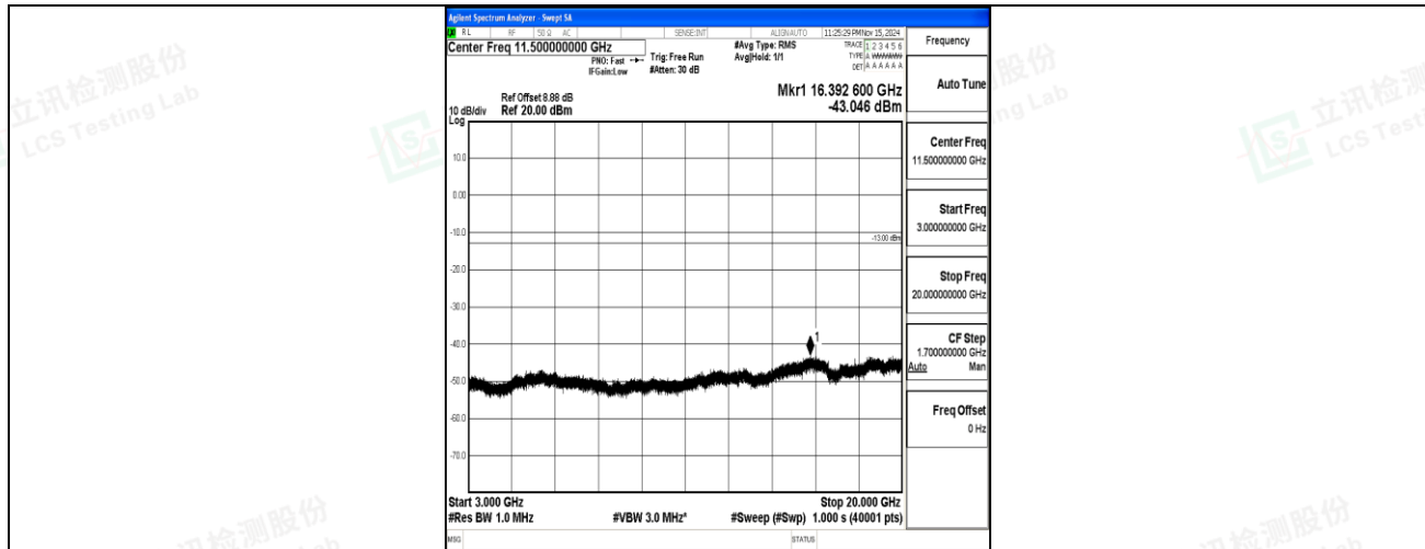
Band2-20MHz-16QAM-19100-1RB#0-3000~20000-PASS
