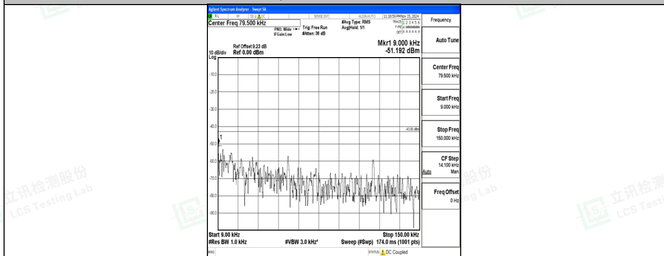
Band2-20MHz-QPSK-18700-1RB#0-0.009~0.15-PASS
