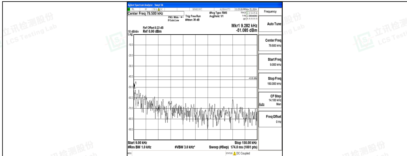
Band2-20MHz-QPSK-19100-1RB#0-0.009~0.15-PASS
