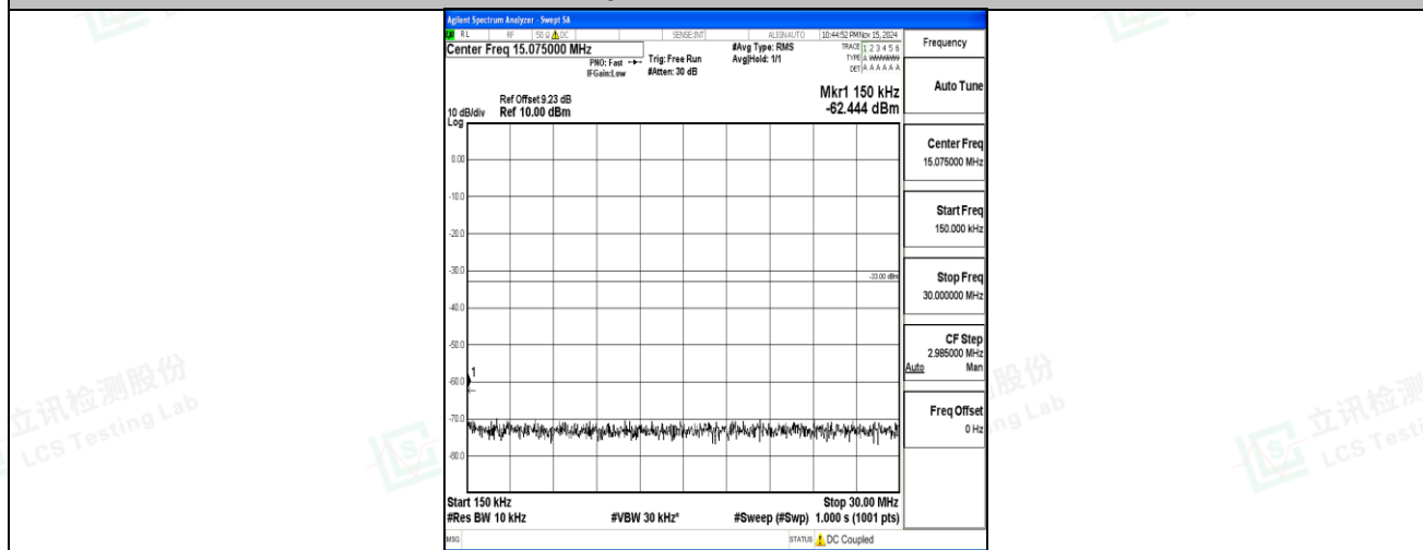
Band2-15MHz-16QAM-18675-1RB#0-0.15~30-PASS
