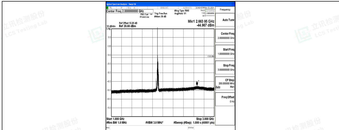
Band2-15MHz-QPSK-19125-1RB#0-1000~3000-PASS
