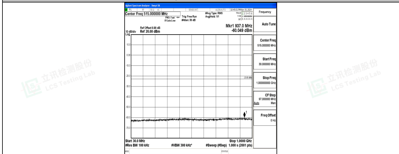
Band2-15MHz-16QAM-18675-1RB#0-30~1000-PASS
