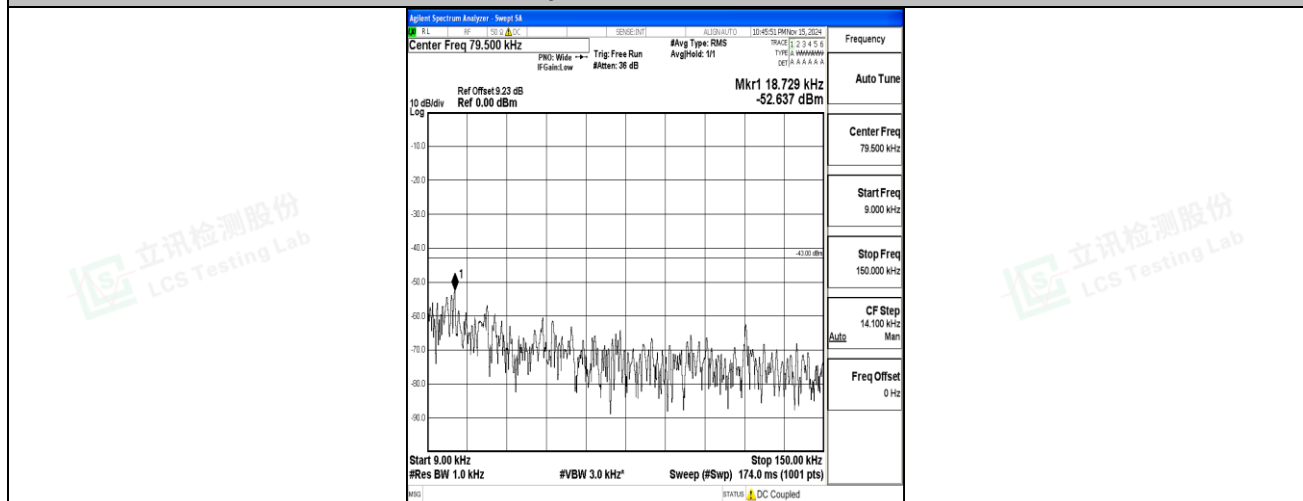
Band2-15MHz-QPSK-18900-1RB#0-0.009~0.15-PASS
