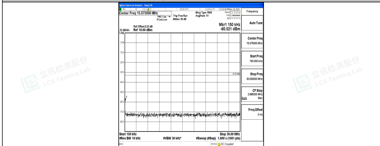
Band2-20MHz-16QAM-18900-1RB#0-0.15~30-PASS
