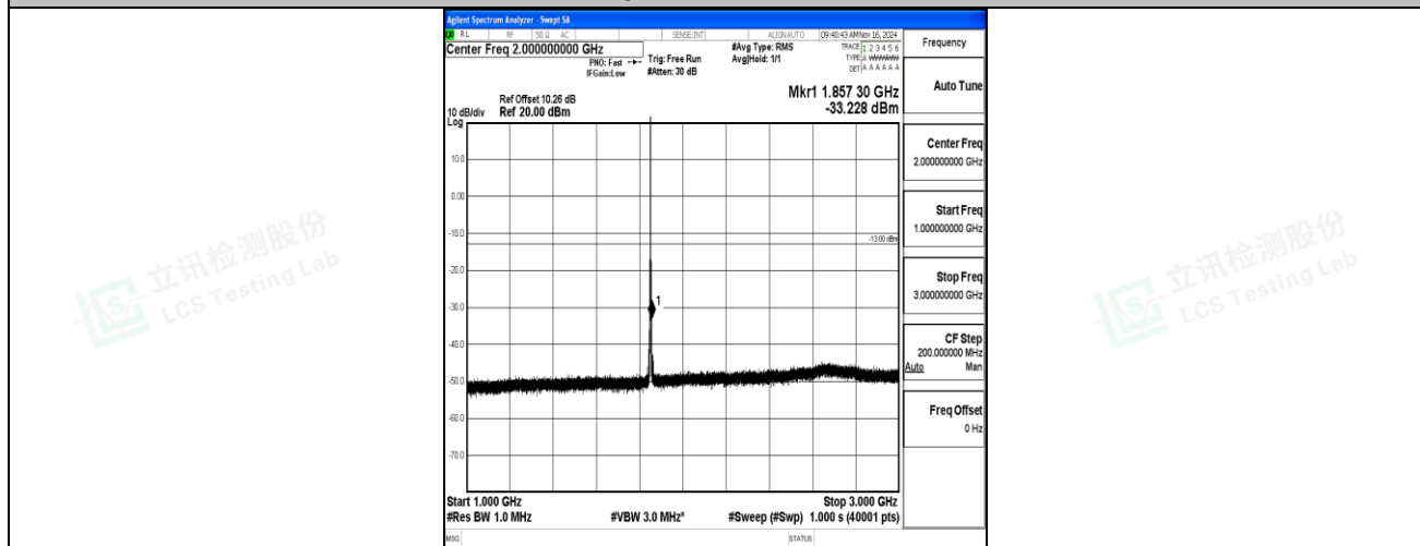
Band2-1.4MHz-16QAM-18607-1RB#0-1000~3000-PASS
