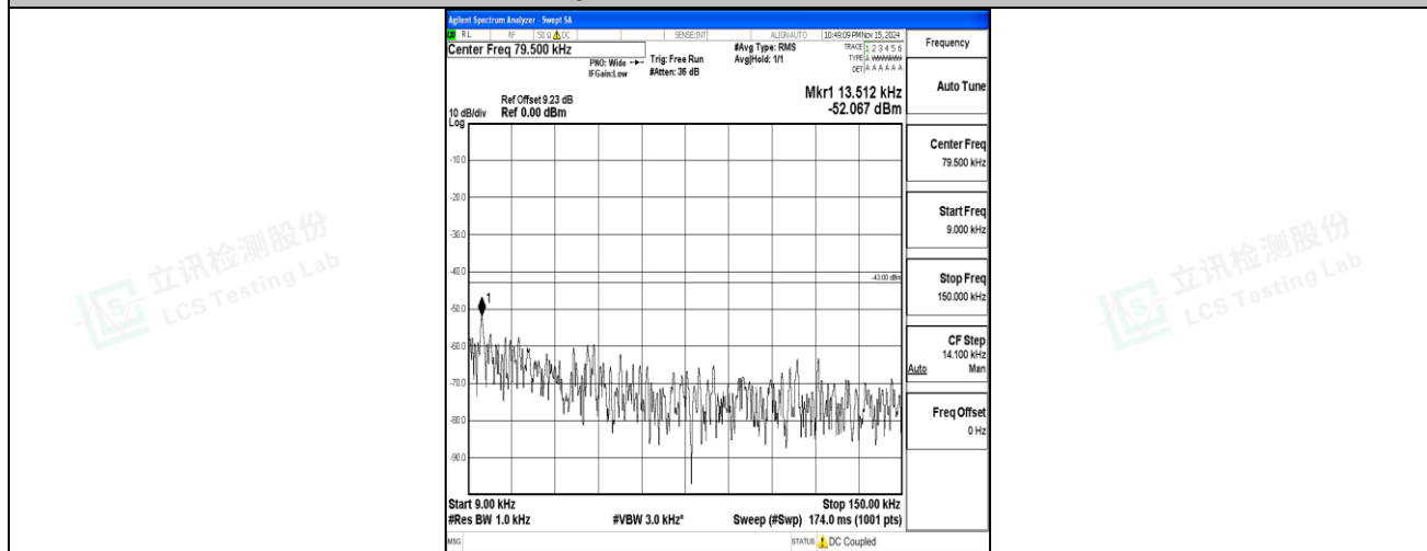
Band2-15MHz-16QAM-19125-1RB#0-0.009~0.15-PASS
