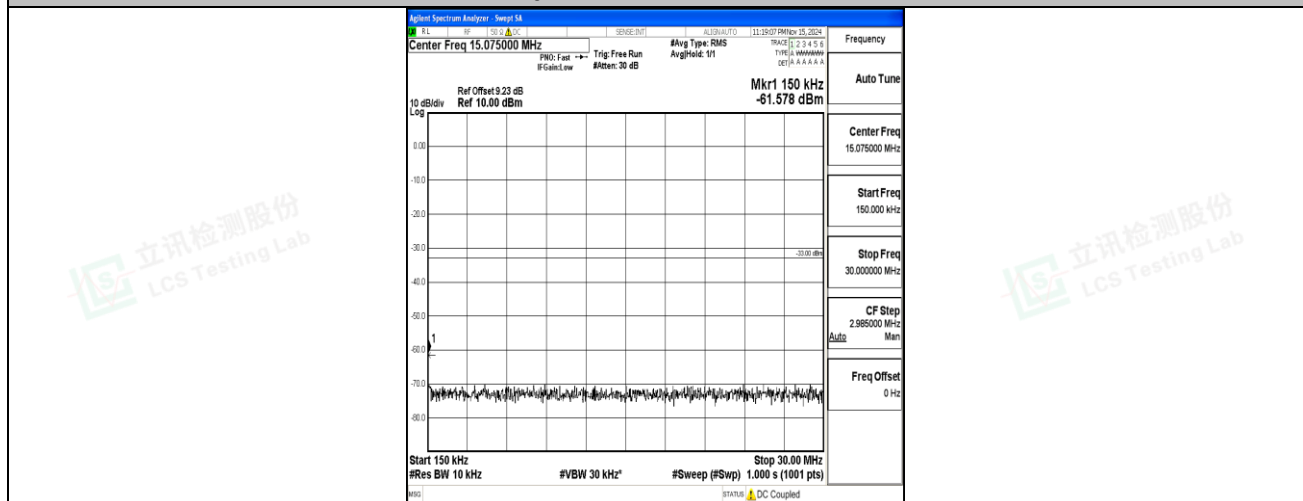
Band2-20MHz-QPSK-18700-1RB#0-0.15~30-PASS
