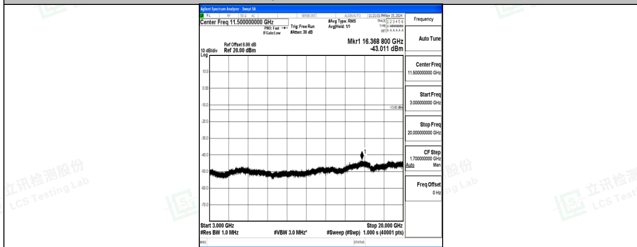
Band2-20MHz-16QAM-18700-1RB#0-3000~20000-PASS
