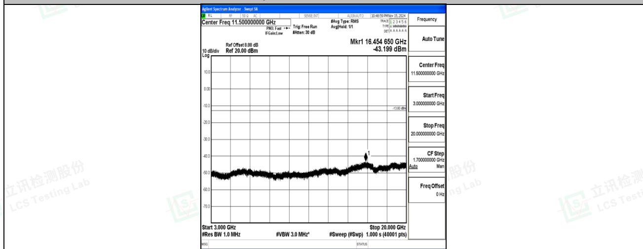
Band2-15MHz-QPSK-19125-1RB#0-3000~20000-PASS
