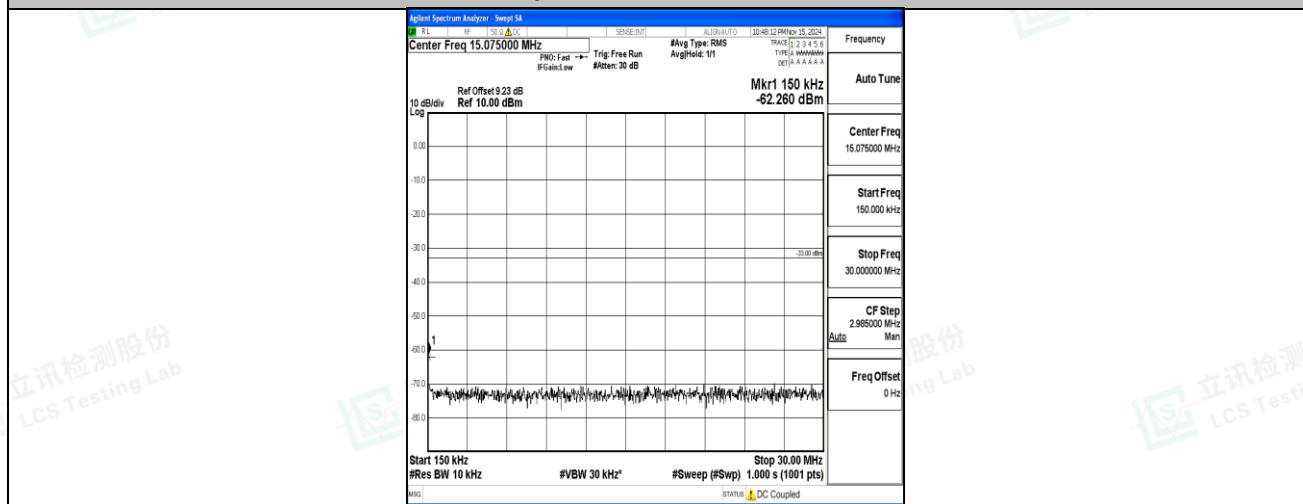
Band2-15MHz-QPSK-19125-1RB#0-0.15~30-PASS
