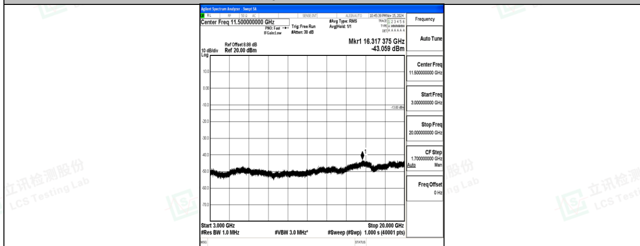
Band2-15MHz-16QAM-18675-1RB#0-3000~20000-PASS
