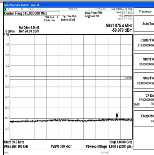
Band2-15MHz-16QAM-19125-1RB#0-0-30~1000-PASS
