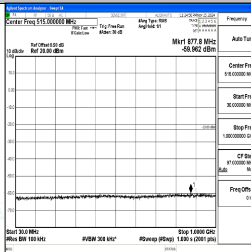
Band2-20MHz-16QAM-19100-1RB#0-0-30~1000-PASS
