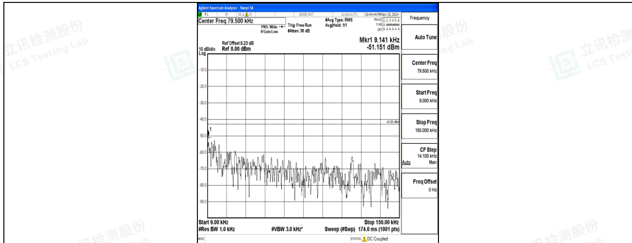
Band2-15MHz-16QAM-18675-1RB#0-0.009~0.15-PASS
