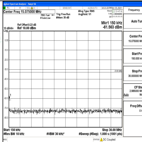
Band2-10MHz-16QAM-19150-1RB#0-0.15~30-PASS
