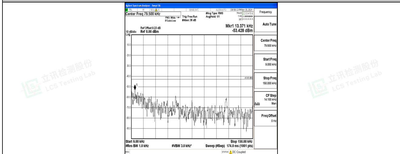
Band2-5MHz-16QAM-19175-1RB#0-0.009~0.15-PASS
