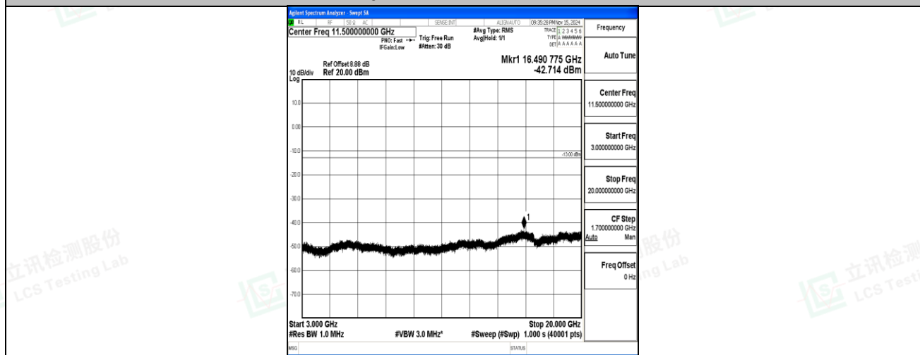
Band2-3MHz-QPSK-19185-1RB#0-3000~20000-PASS
