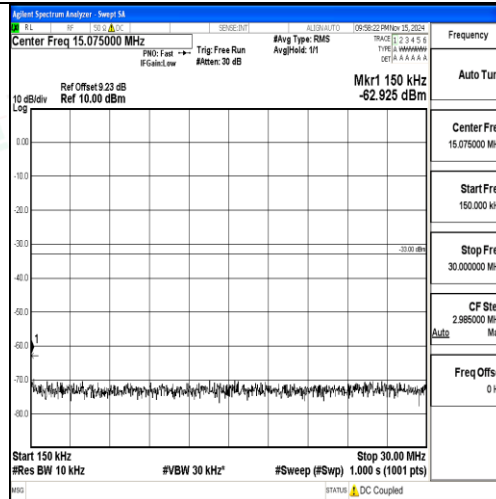
Band2-5MHz-16QAM-19175-1RB#0-0.15~30-PASS
