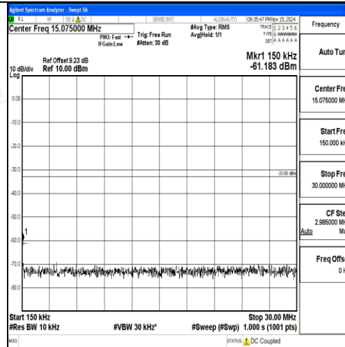
Band2-3MHz-16QAM-19185-1RB#0-0.15~30-PASS
