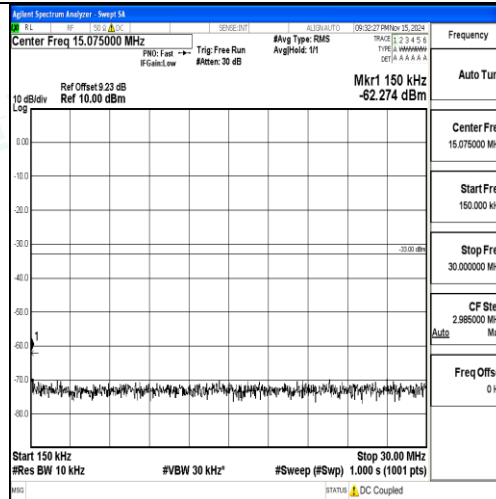
Band2-3MHz-QPSK-18900-1RB#0-0.15~30-PASS
