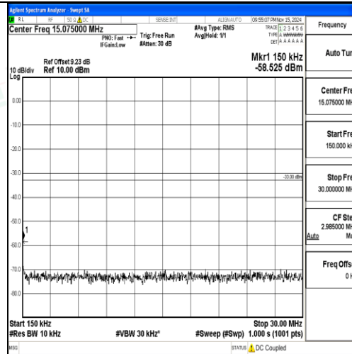
Band2-5MHz-QPSK-18900-1RB#0-0.15~30-PASS
