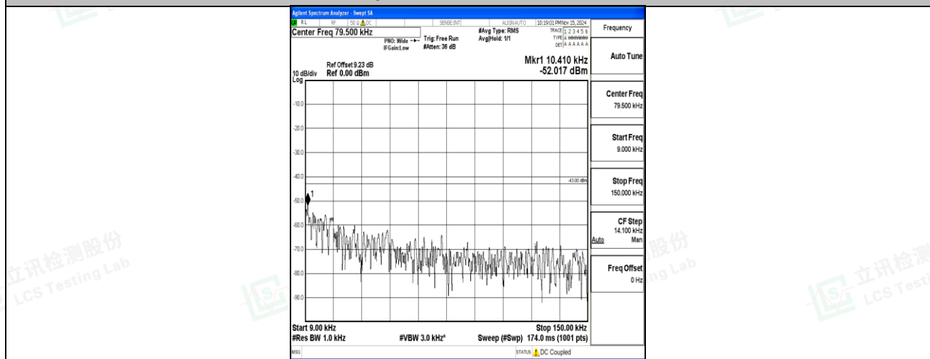
Band2-10MHz-16QAM-18900-1RB#0-0.009~0.15-PASS
