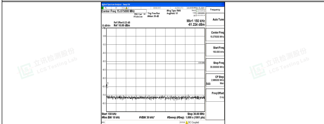
Band2-10MHz-QPSK-18650-1RB#0-0.15~30-PASS
