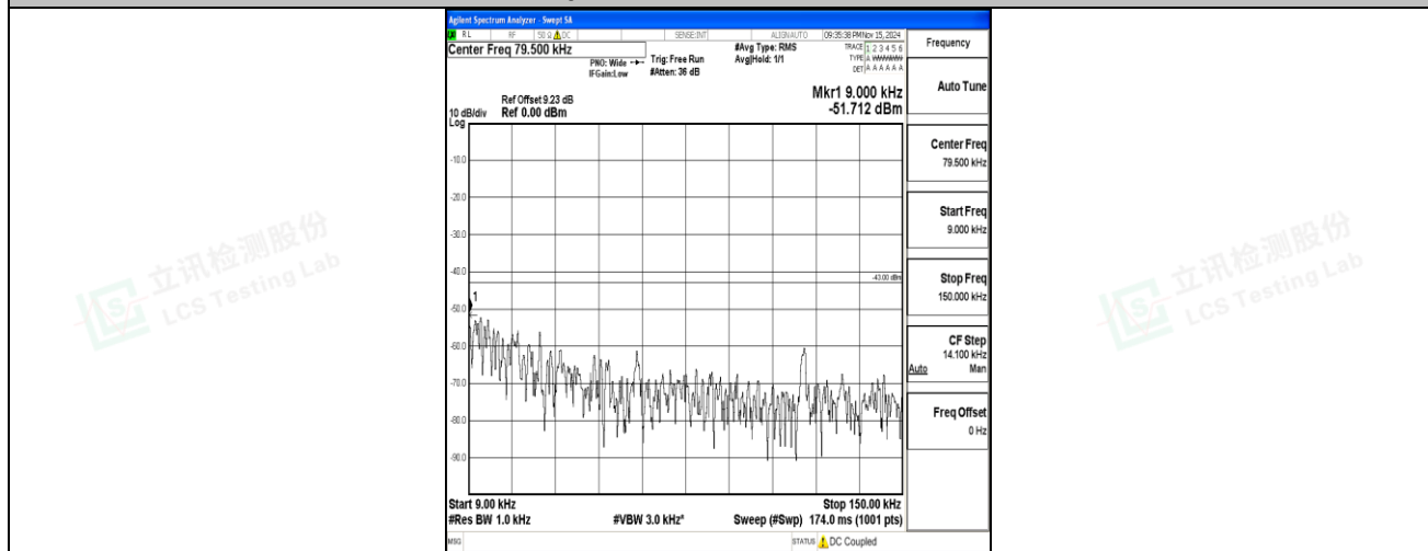
Band2-3MHz-16QAM-19185-1RB#0-0.009~0.15-PASS
