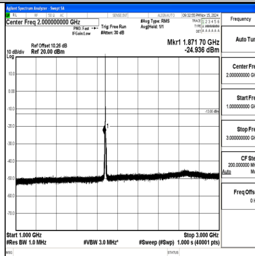
Band2-3MHz-QPSK-18900-1RB#0-1000~3000-PASS
