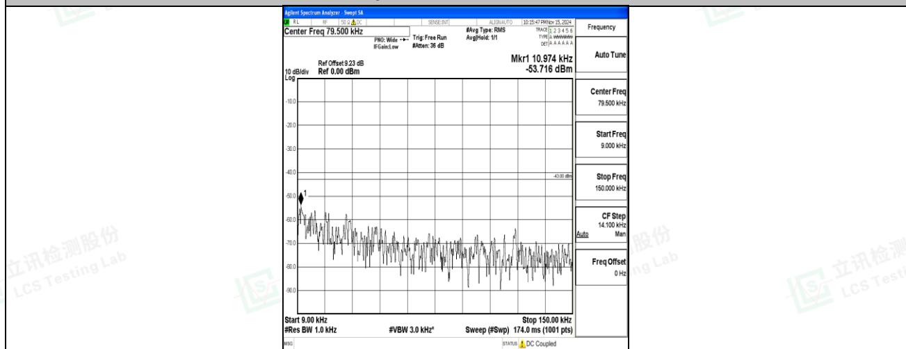
Band2-10MHz-QPSK-18650-1RB#0-0.009~0.15-PASS
