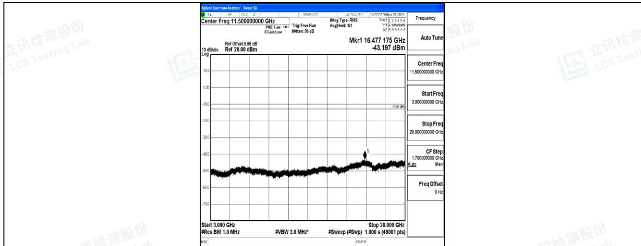
Band2-10MHz-16QAM-19150-1RB#0-3000~20000-PASS
