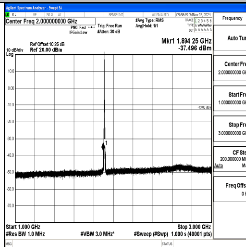
Band2-5MHz-16QAM-19175-1RB#0-1000~3000-PASS
