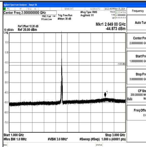
Band2-10MHz-16QAM-19150-1RB#0-0-1000~3000-PASS
