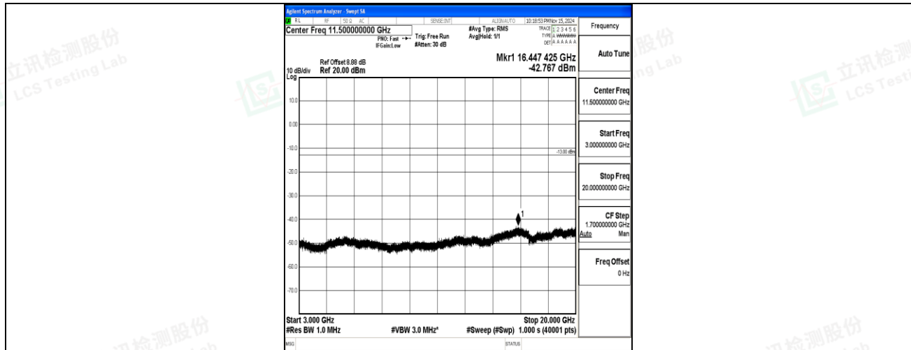
Band2-10MHz-QPSK-18900-1RB#0-3000~20000-PASS
