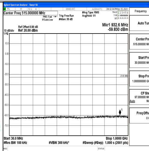
Band2-3MHz-QPSK-18900-1RB#0-30~1000-PASS
