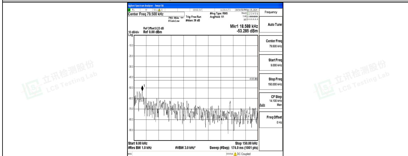
Band2-5MHz-QPSK-18900-1RB#0-0.009~0.15-PASS
