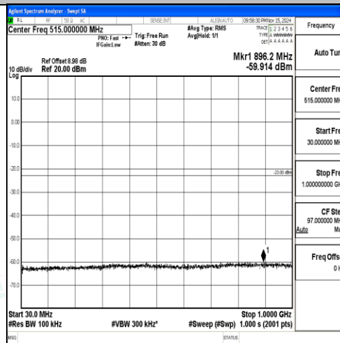
Band2-5MHz-16QAM-19175-1RB#0-30~1000-PASS
