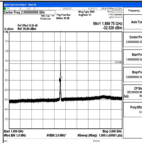
Band2-3MHz-16QAM-19185-1RB#0-1000~3000-PASS
