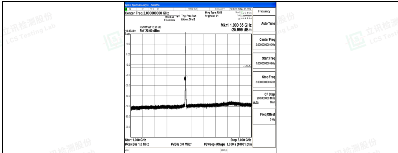
Band2-3MHz-QPSK-19185-1RB#0-1000~3000-PASS
