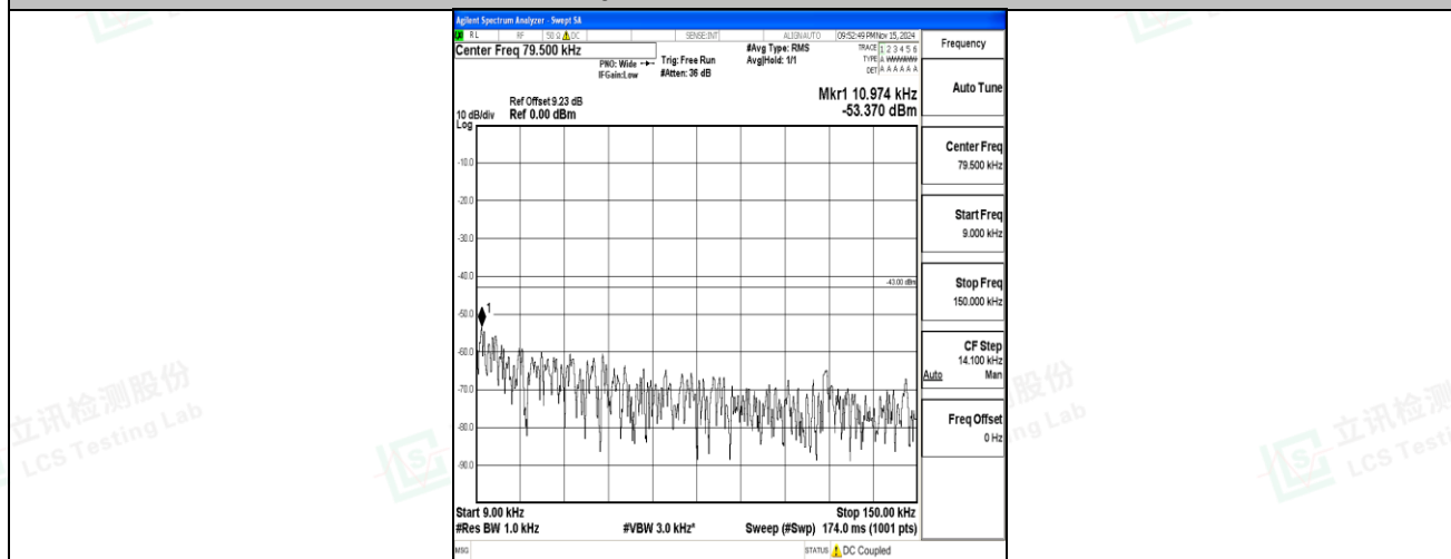
Band2-5MHz-QPSK-18625-1RB#0-0.009~0.15-PASS
