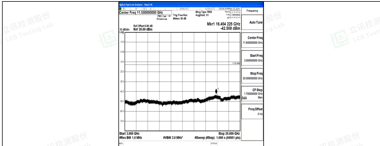
Band2-3MHz-16QAM-19185-1RB#0-3000~20000-PASS
