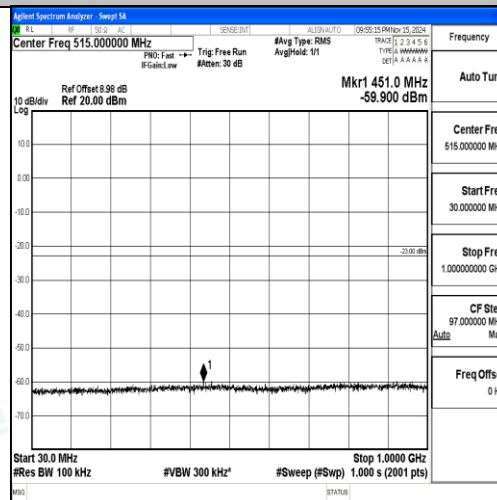
Band2-5MHz-QPSK-18900-1RB#0-30~1000-PASS
