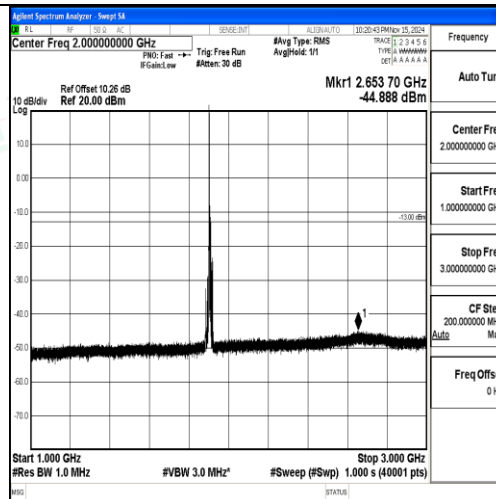
Band2-10MHz-QPSK-19150-1RB#0-1000~3000-PASS
