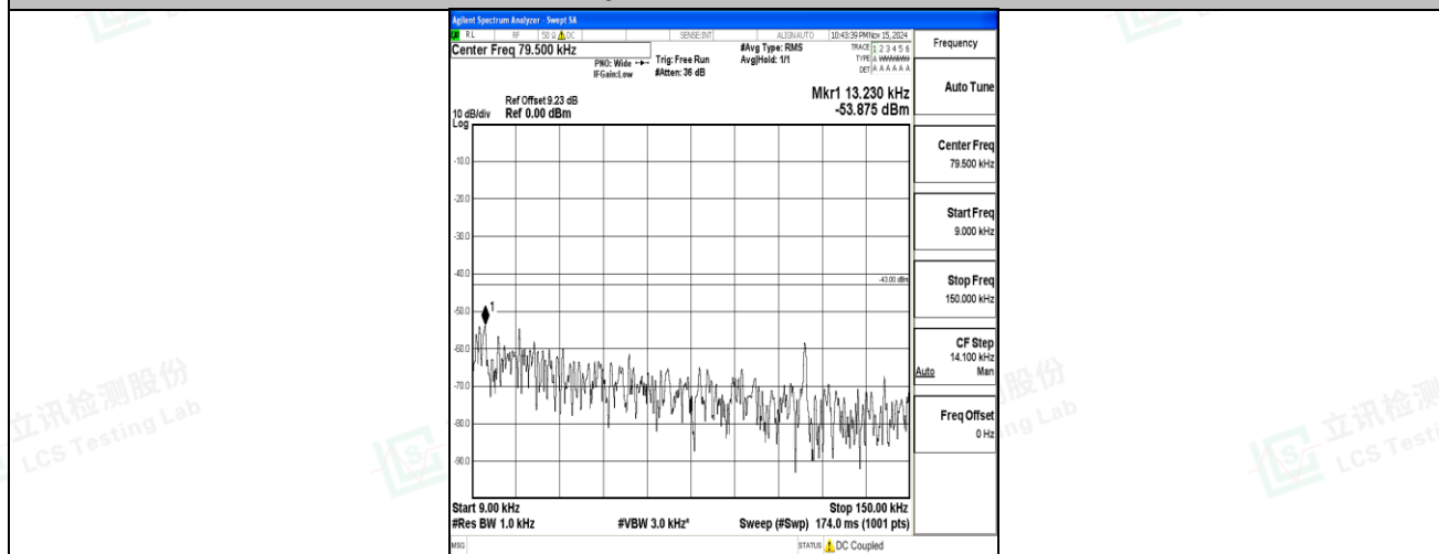
Band2-15MHz-QPSK-18675-1RB#0-0.009~0.15-PASS
