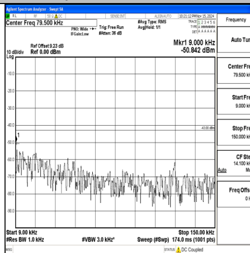
Band2-10MHz-16QAM-19150-1RB#0-0.009~0.15-PASS
