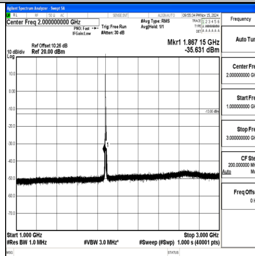
Band2-5MHz-QPSK-18900-1RB#0-1000~3000-PASS
