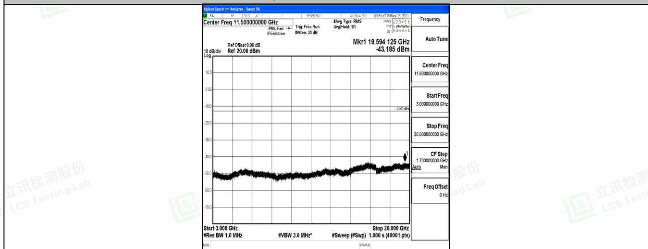
Band2-5MHz-16QAM-18625-1RB#0-3000~20000-PASS
