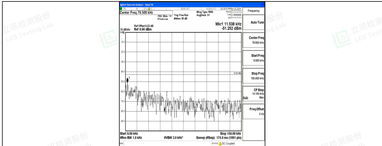
Band2-10MHz-16QAM-18650-1RB#0-0.009~0.15-PASS
