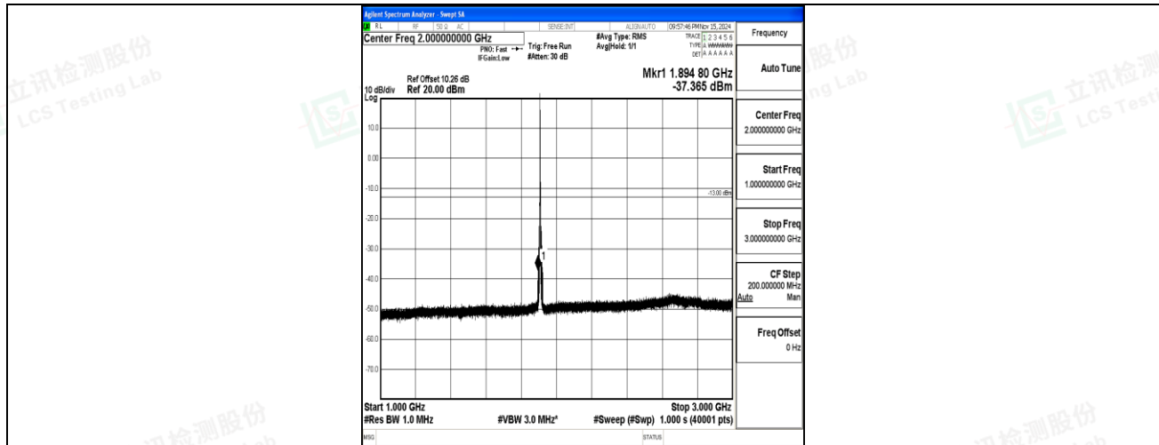
Band2-5MHz-QPSK-19175-1RB#0-1000~3000-PASS
