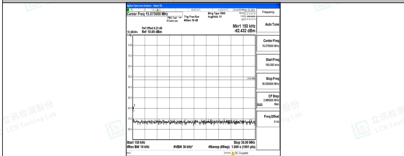
Band2-10MHz-16QAM-18650-1RB#0-0.15~30-PASS
