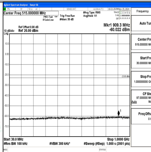
Band2-10MHz-16QAM-19150-1RB#0-0-30~1000-PASS
