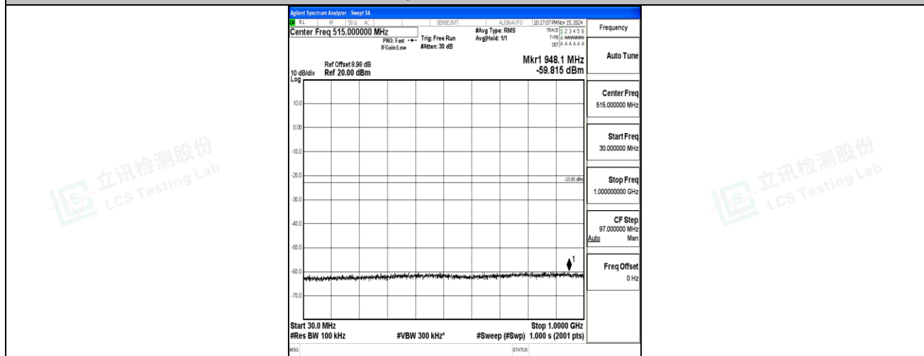
Band2-10MHz-16QAM-18650-1RB#0-30~1000-PASS
