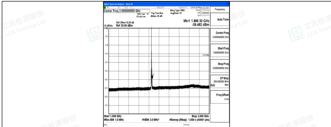
Band2-5MHz-16QAM-18625-1RB#0-1000~3000-PASS
