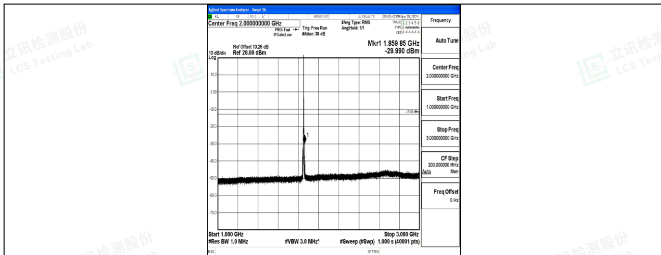
Band2-3MHz-16QAM-18615-1RB#0-1000~3000-PASS
