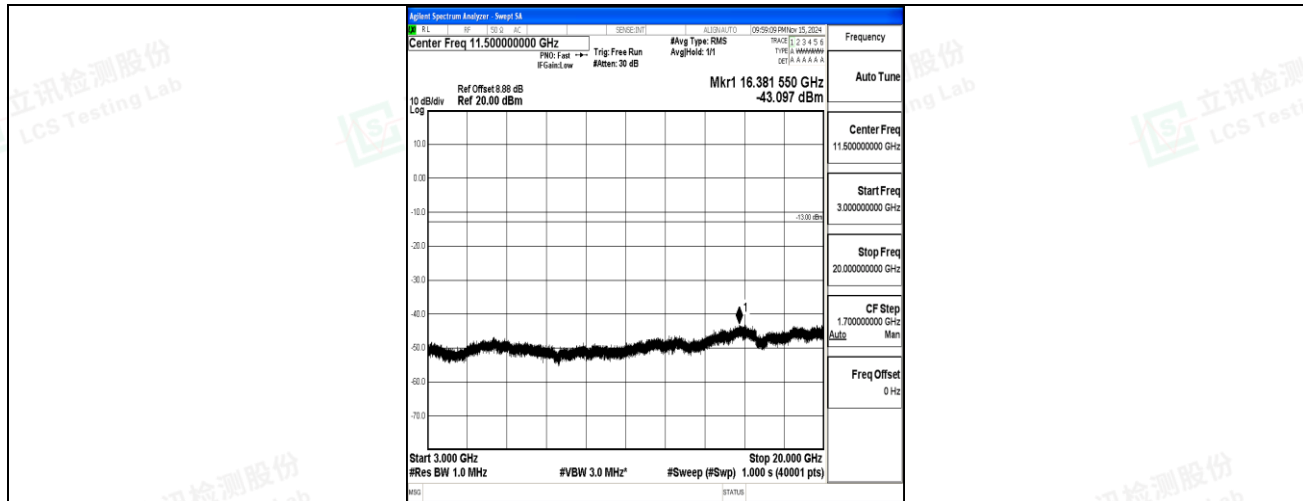
Band2-5MHz-16QAM-19175-1RB#0-3000~20000-PASS
