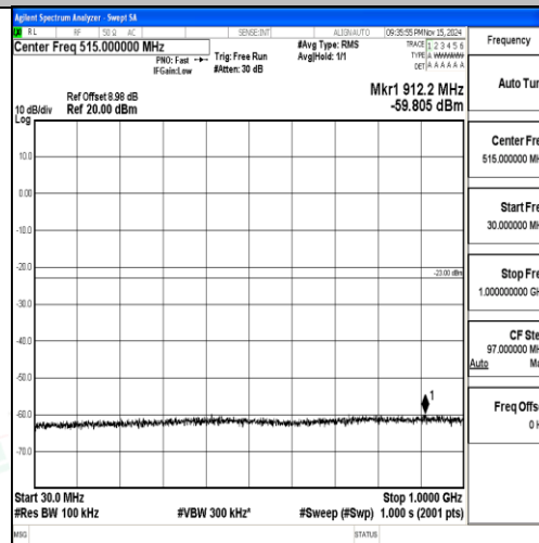
Band2-3MHz-16QAM-19185-1RB#0-30~1000-PASS
