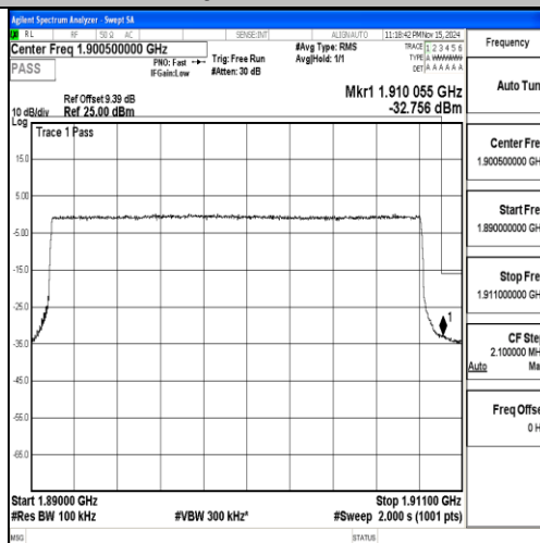
Band2-20MHz-16QAM-19100-100RB#0-PASS
