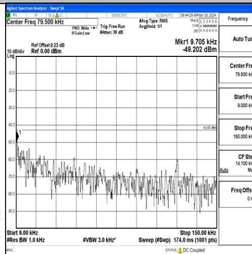
Band2-1.4MHz-16QAM-19193-1RB#0-0.009~0.15-PASS
