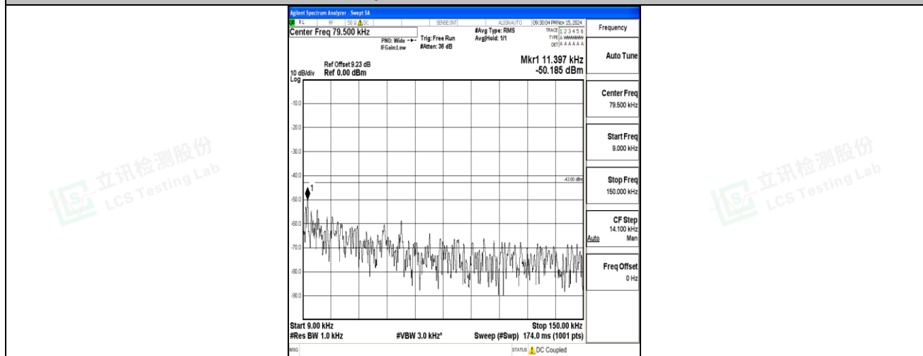
Band2-3MHz-QPSK-18615-1RB#0-0.009~0.15-PASS
