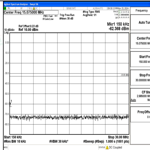
Band2-3MHz-QPSK-18615-1RB#0-0.15~30-PASS
