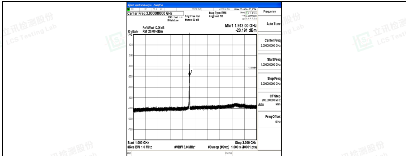
Band2-1.4MHz-QPSK-19193-1RB#0-1000~3000-PASS
