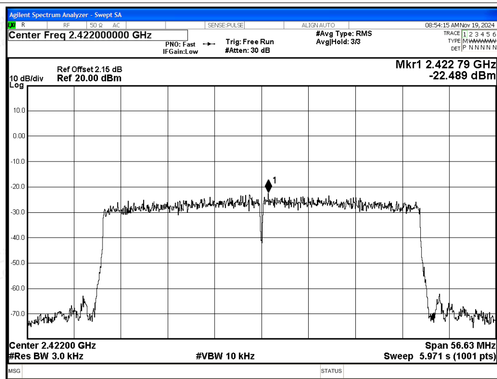
PSD NVNT ax40 2422MHz Ant7
