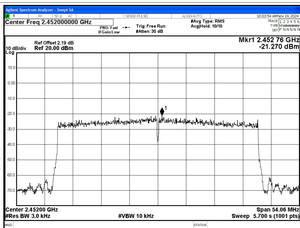
PSD NVNT ax40 2452MHz Ant7
