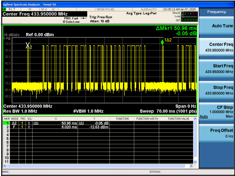
(Transmit cycle 50.96ms)
