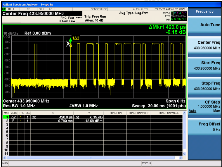
(Time per burst: 0.42ms*16pcs)
