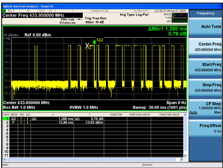
(Time per burst: 1.26 ms*9pcs)
