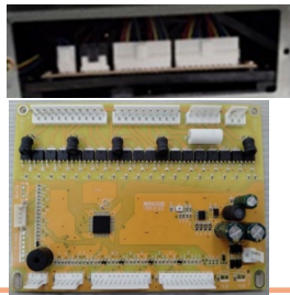
Main board (inside the north field operation BOX)
