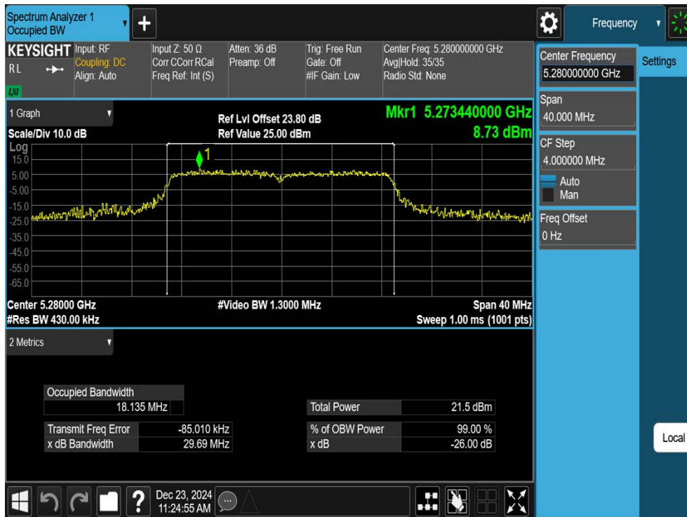
11N20SISO-Ant1-5280
