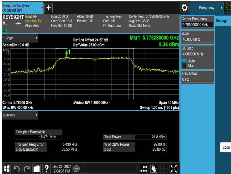
11N20SISO-Ant1-5785
