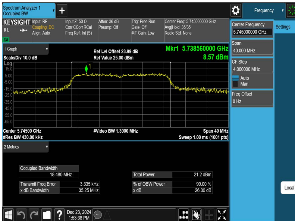
11N20SISO-Ant1-5745
