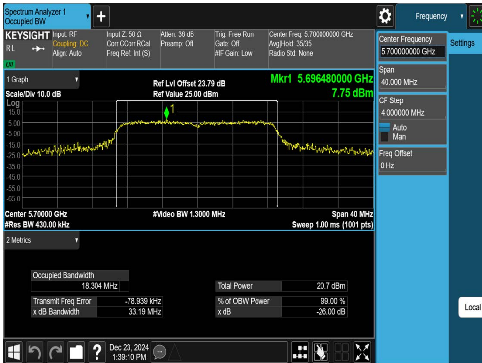
11N20SISO-Ant1-5700
