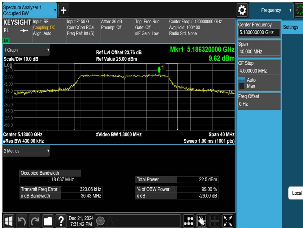
11A-Ant1-5180
