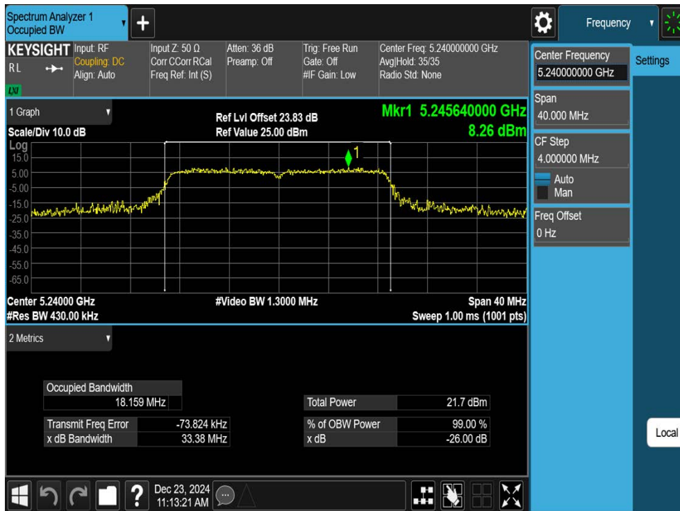
11N20SISO-Ant1-5240
