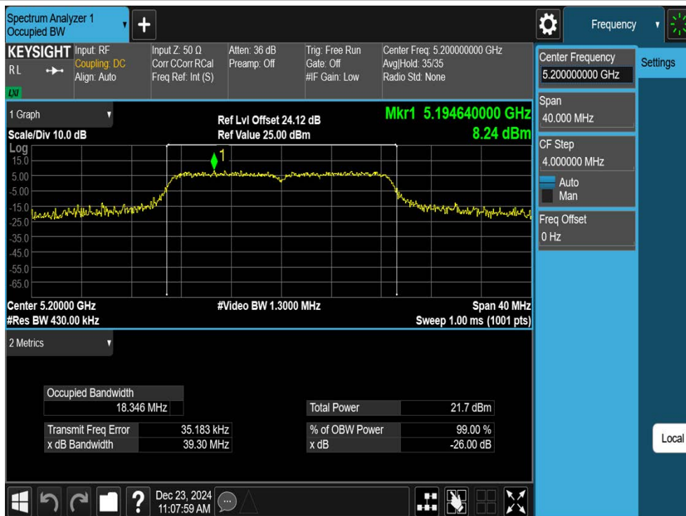
11N20SISO-Ant1-5200
