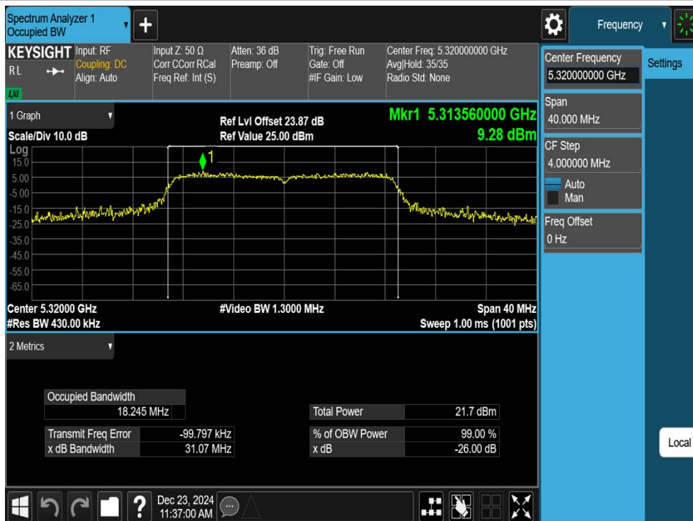
11N20SISO-Ant1-5320
