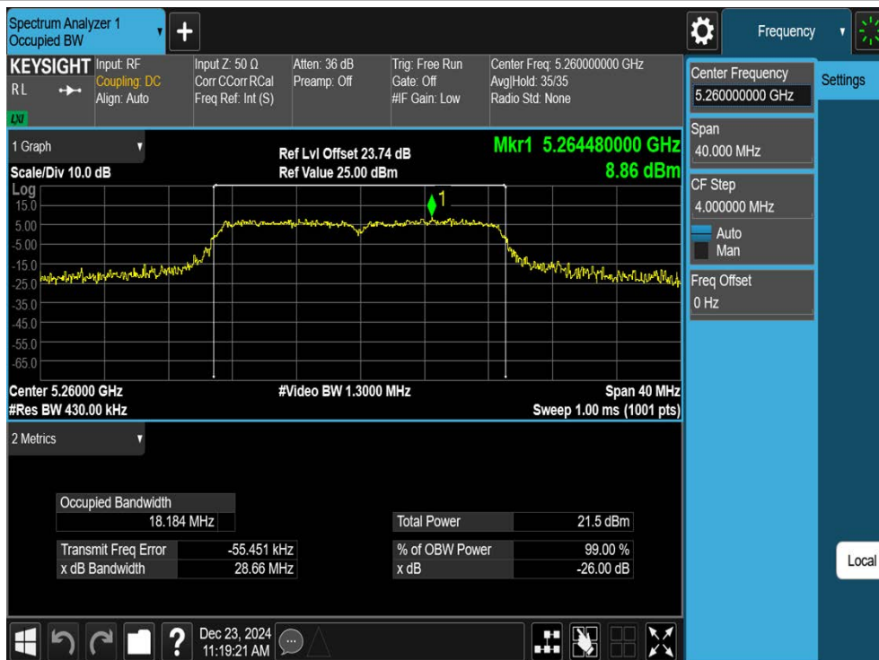
11N20SISO-Ant1-5260
