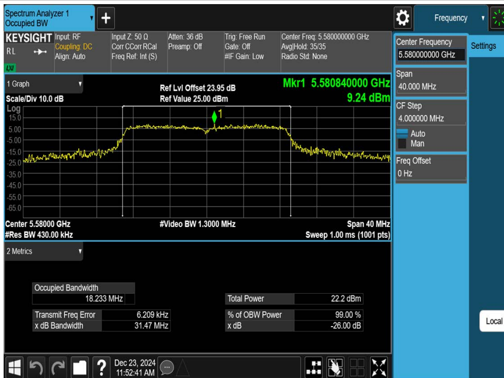
11N20SISO-Ant1-5580
