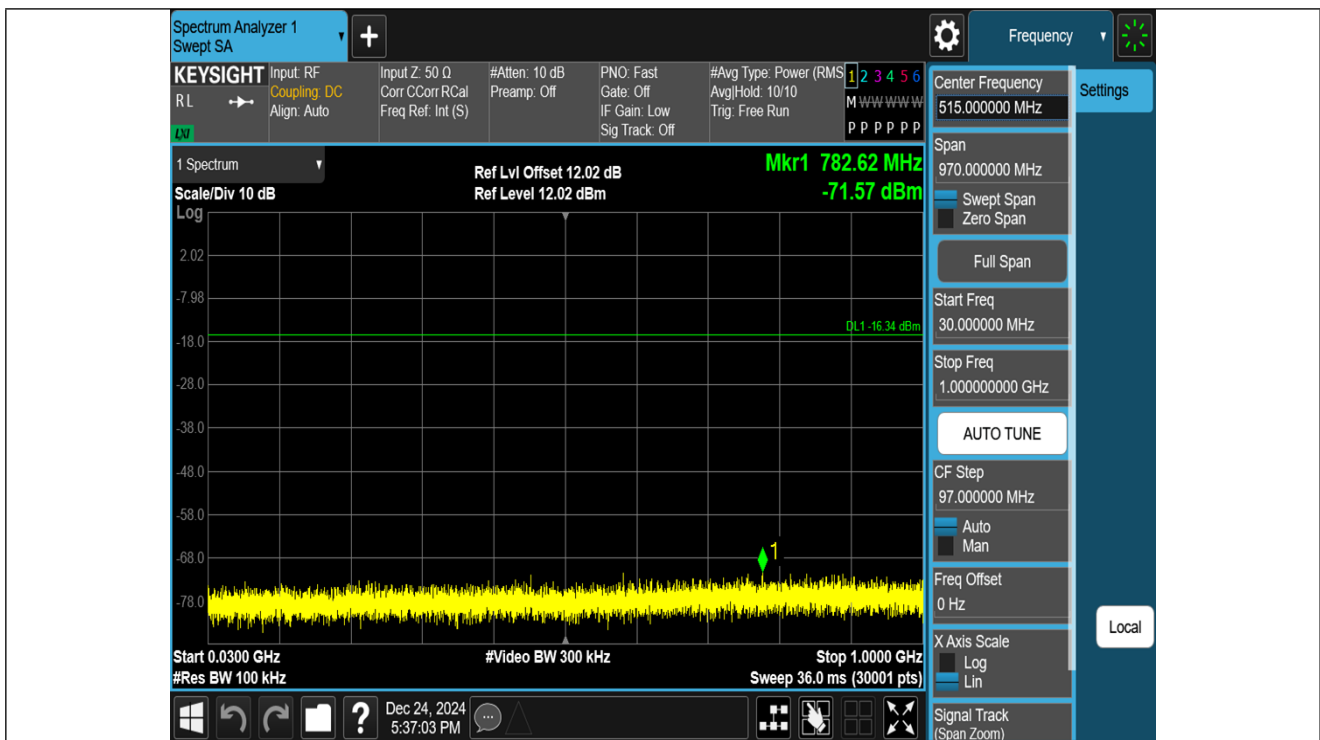
BLE_1M-Ant1-2440-30~1000-PASS
