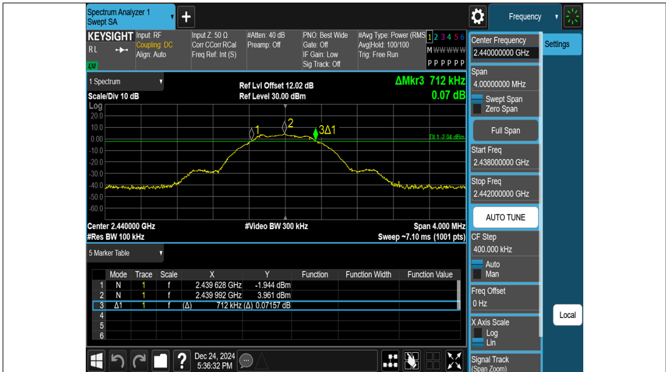
BLE_1M-Ant1-2440-PASS
