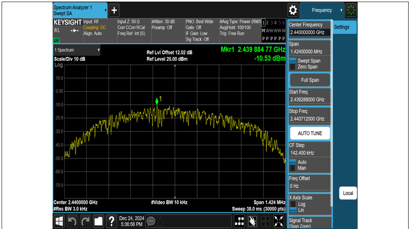
BLE_1M-Ant1-2440-PASS
