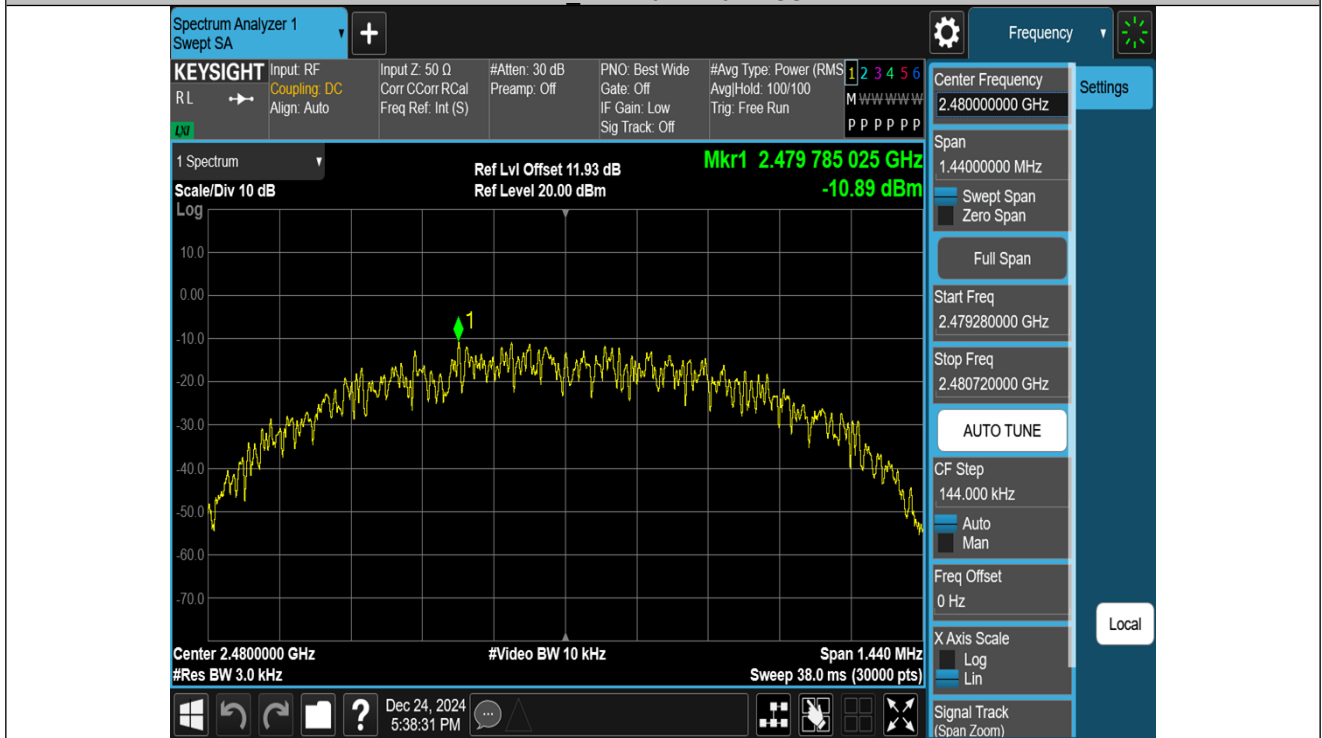
BLE_1M-Ant1-2480-PASS
