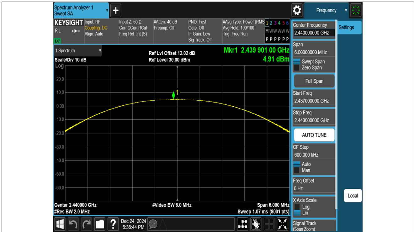
BLE_1M-Ant1-2440-PASS
