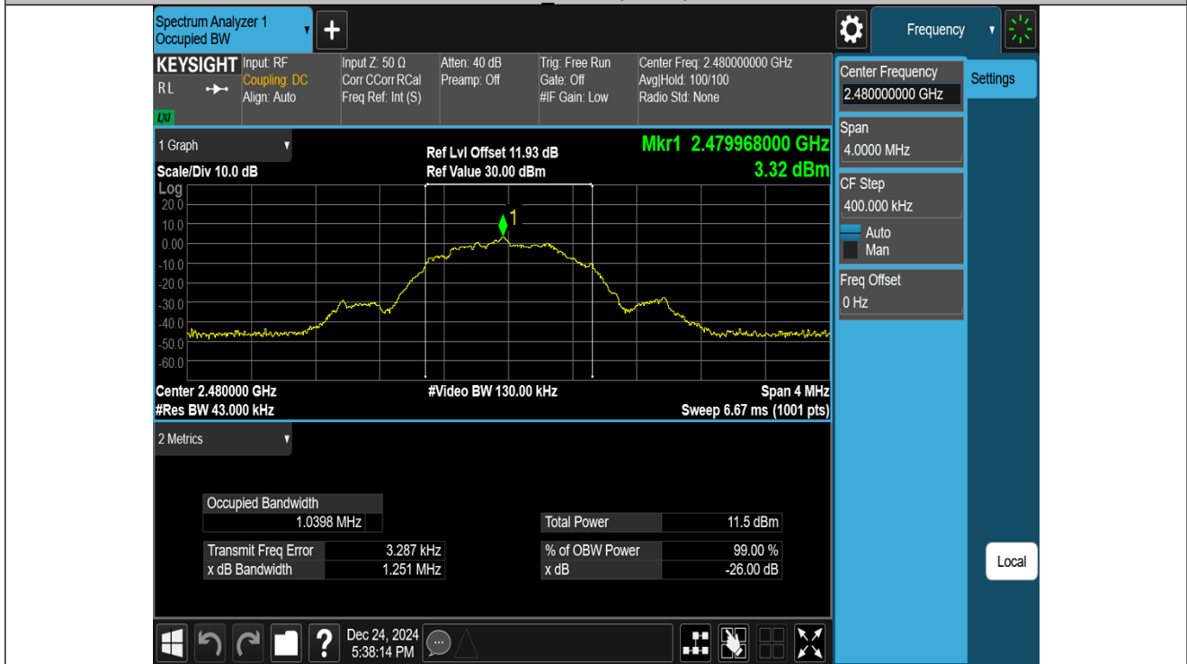
BLE_1M-Ant1-2480
