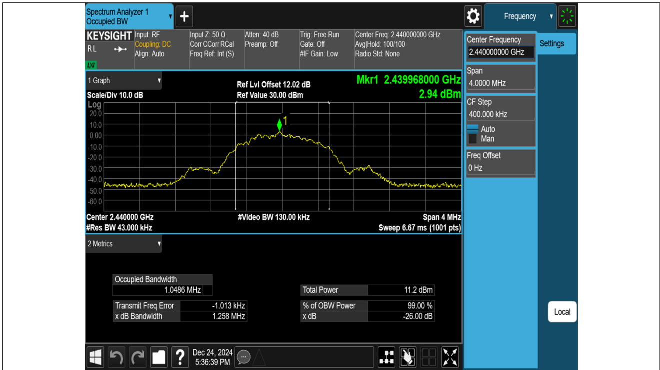
BLE_1M-Ant1-2440
