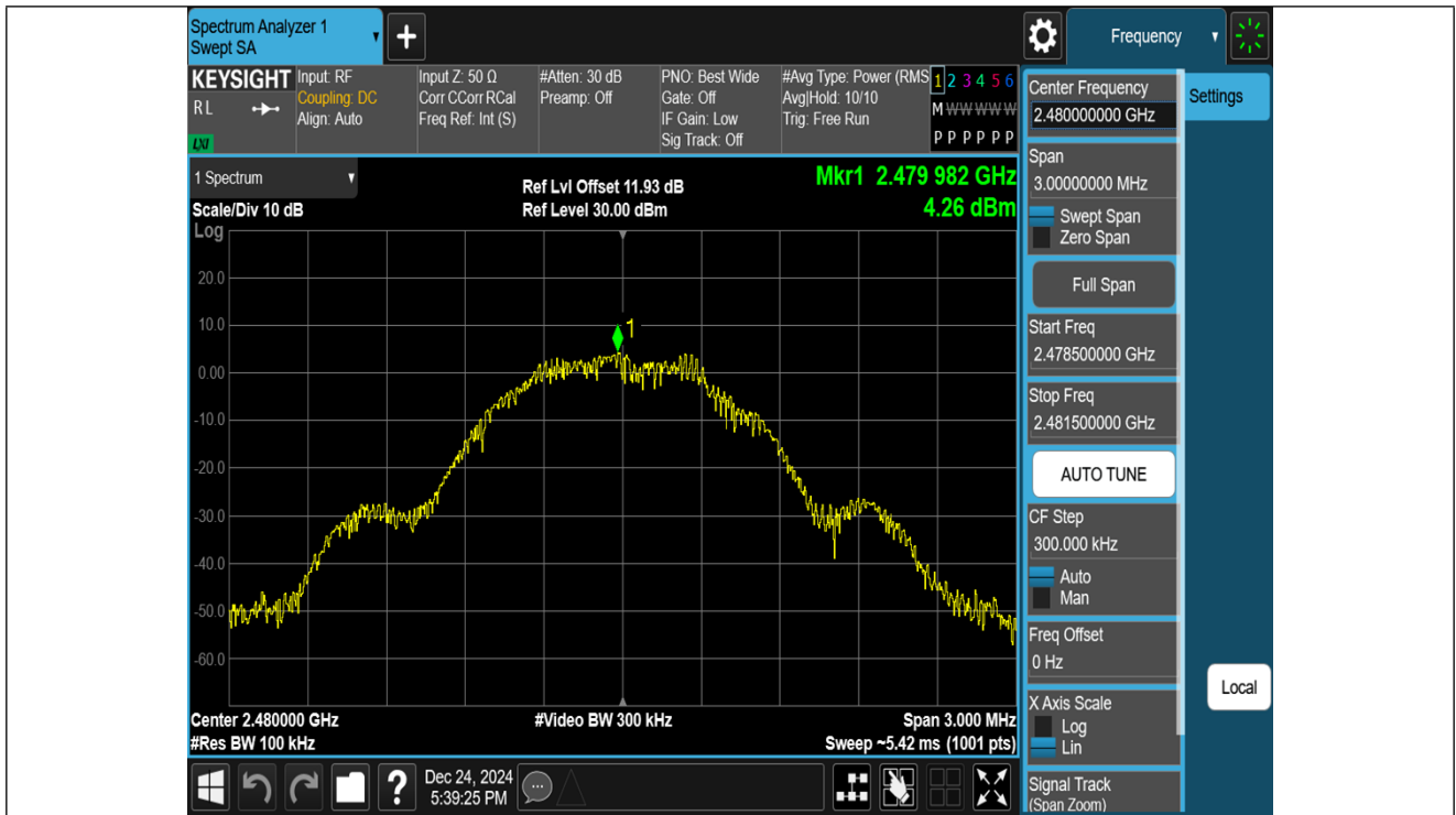
BLE_1M-Ant1-2480-0~Reference-PASS
