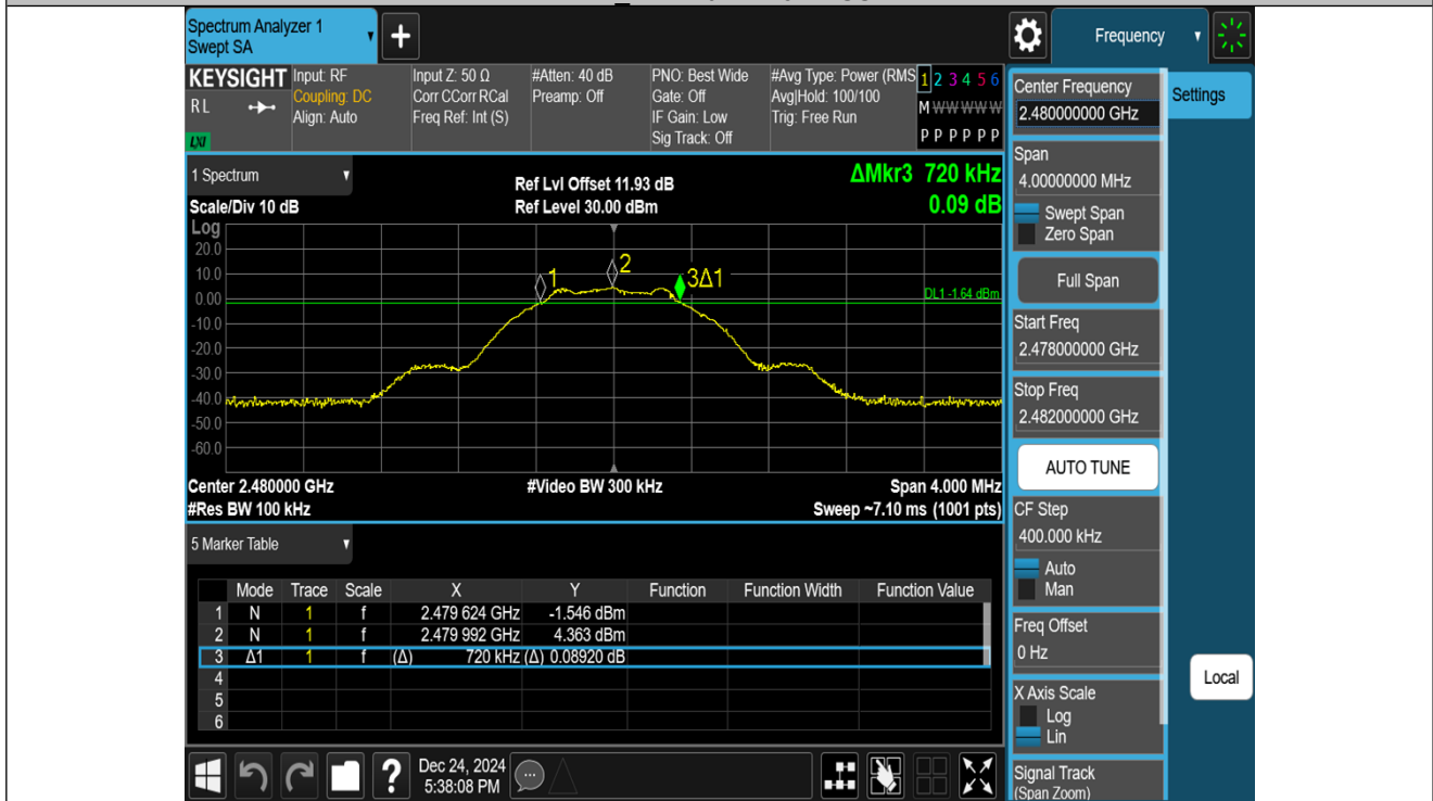
BLE_1M-Ant1-2480-PASS
