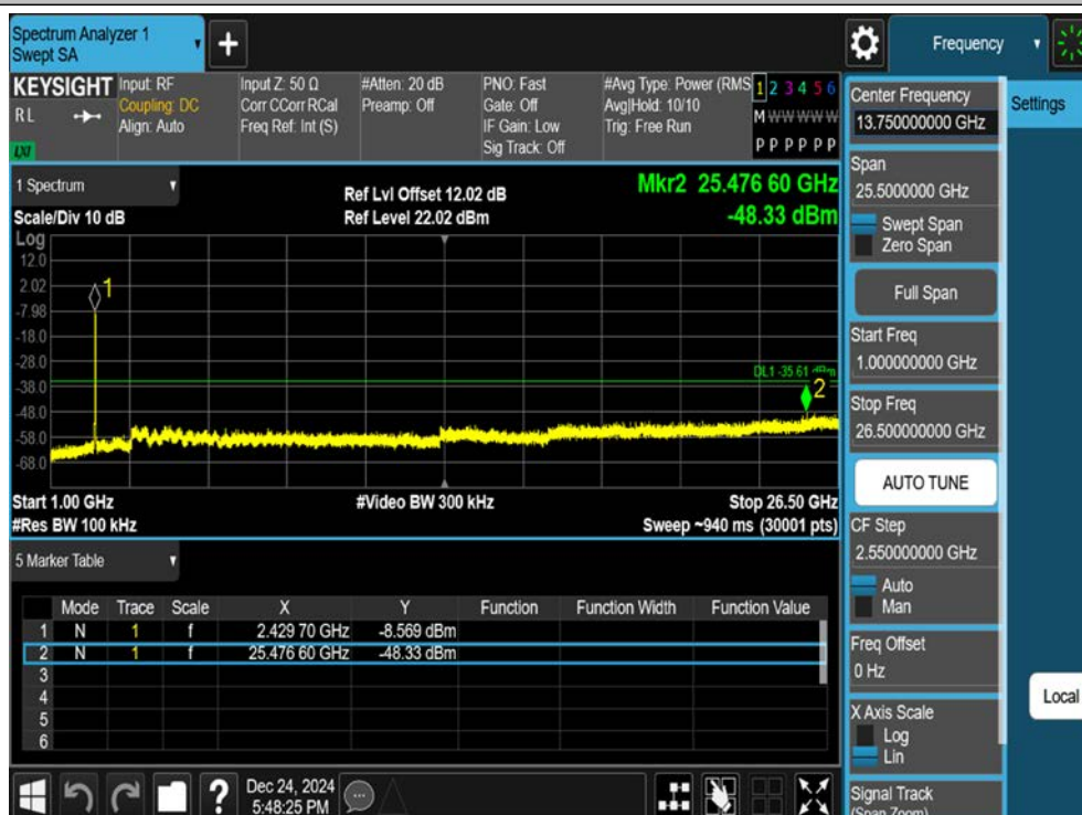
11N20SISO-Ant1-2437-1000~26500-PASS
