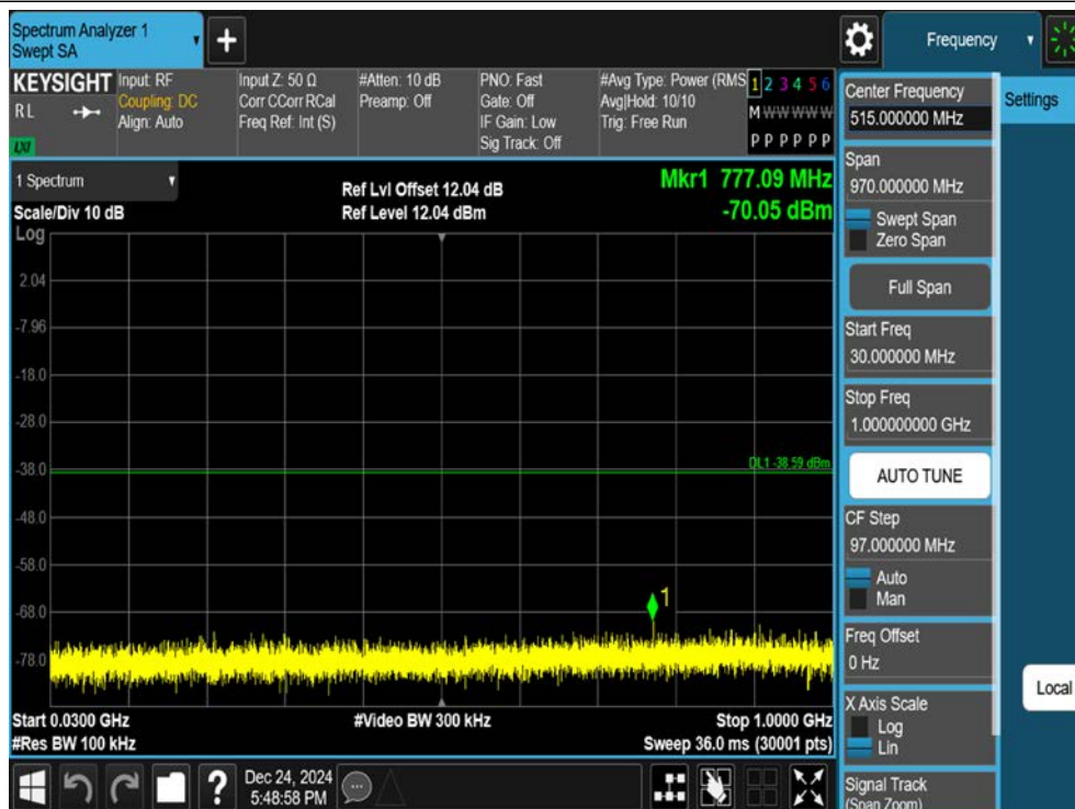
11N40SISO-Ant1-2422-30~1000-PASS
