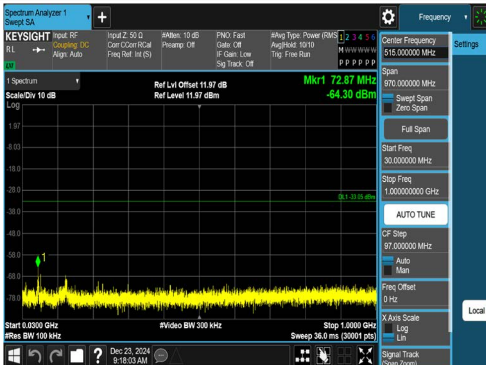
11N20SISO-Ant1-2462-30~1000-PASS
