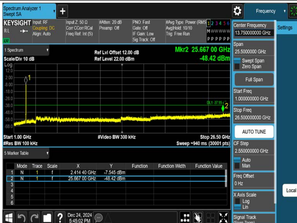
11G-Ant1-2412-1000~26500-PASS
