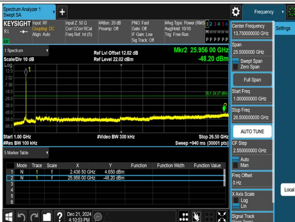
11B-Ant1-2437-1000~26500-PASS
