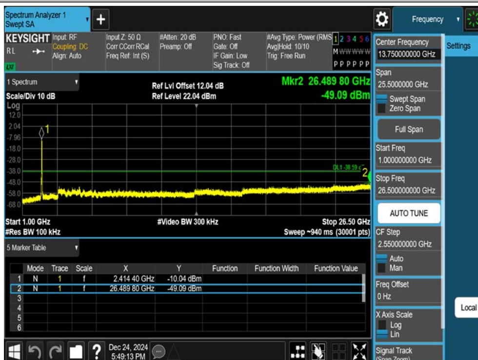
11N40SISO-Ant1-2422-1000~26500-PASS
