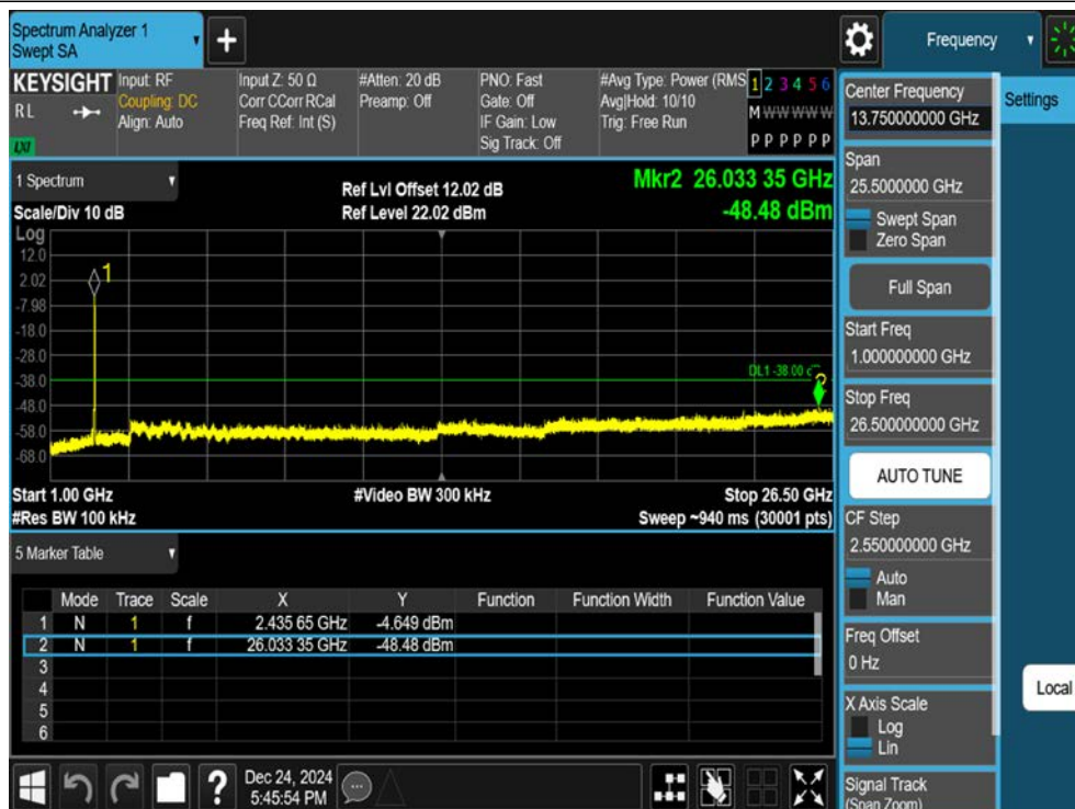
11G-Ant1-2437-1000~26500-PASS
