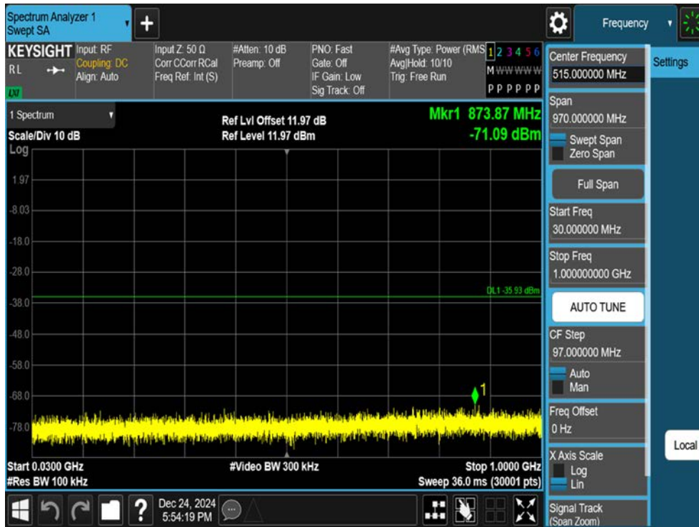
11N20SISO-Ant1-2462-0~Reference-PASS
