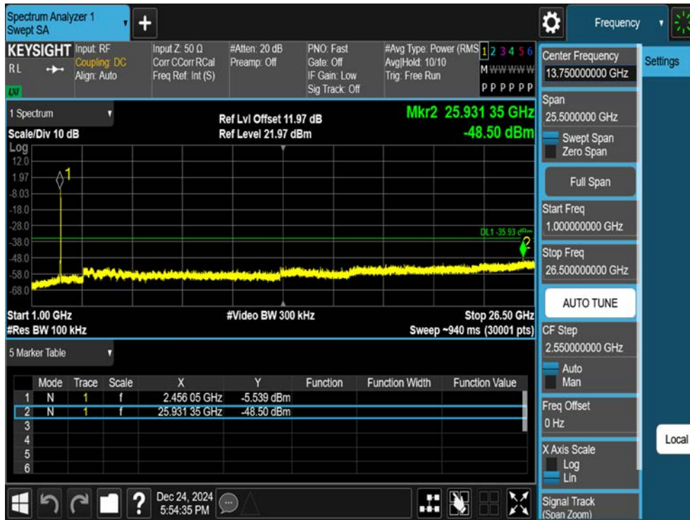
11N20SISO-Ant1-2462-1000~26500-PASS
