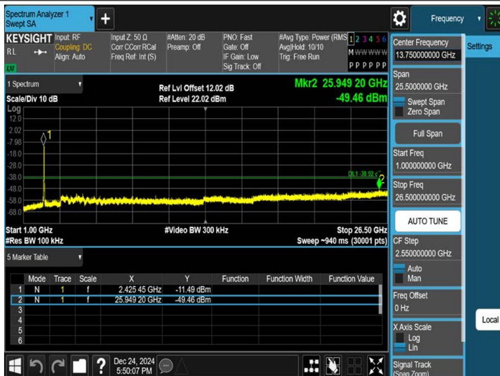
11N40SISO-Ant1-2437-1000~26500-PASS
