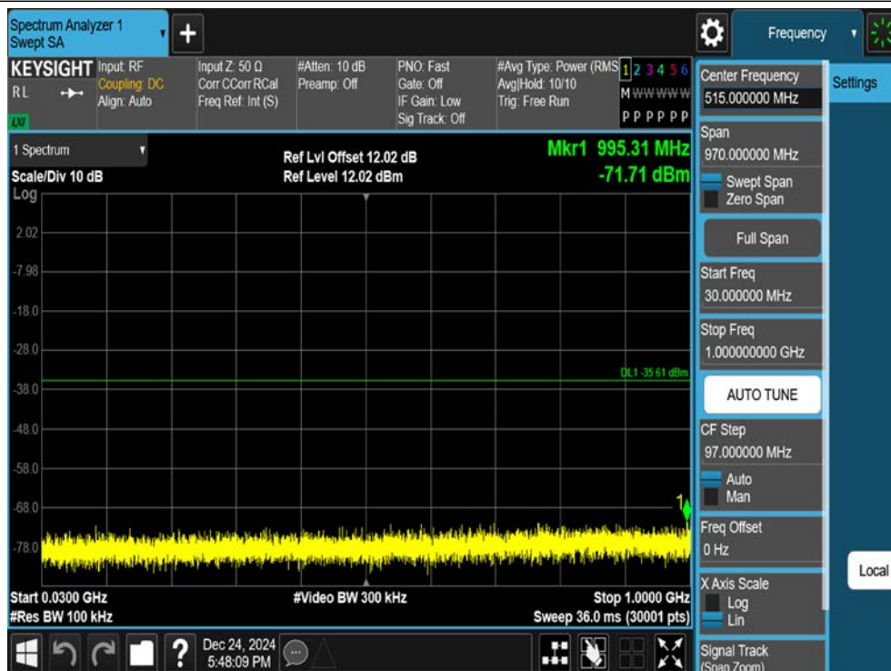
11N20SISO-Ant1-2437-30~1000-PASS
