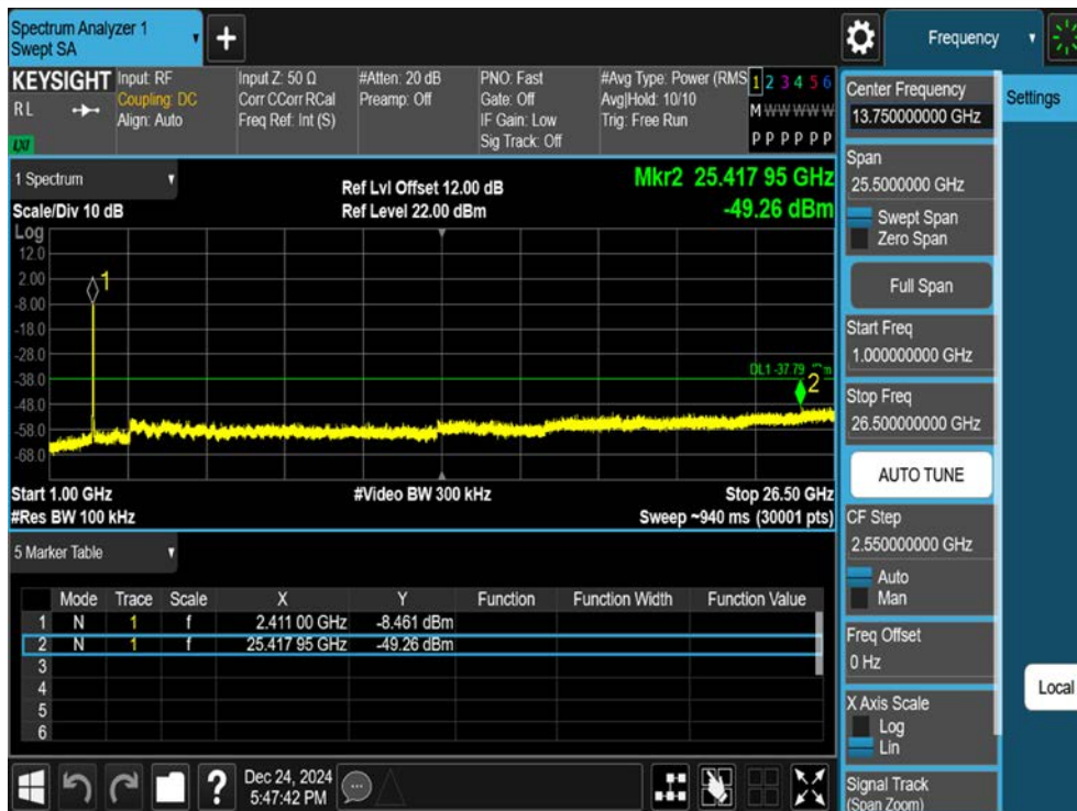
11N20SISO-Ant1-2412-1000~26500-PASS
