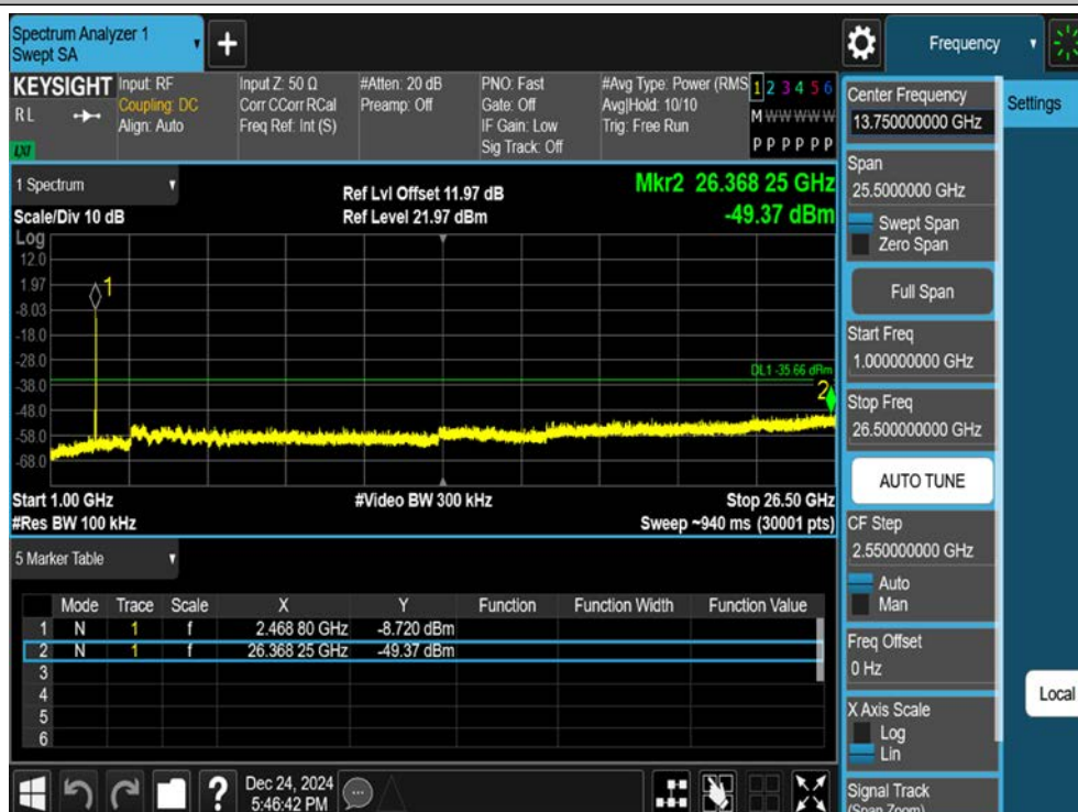
11G-Ant1-2462-1000~26500-PASS
