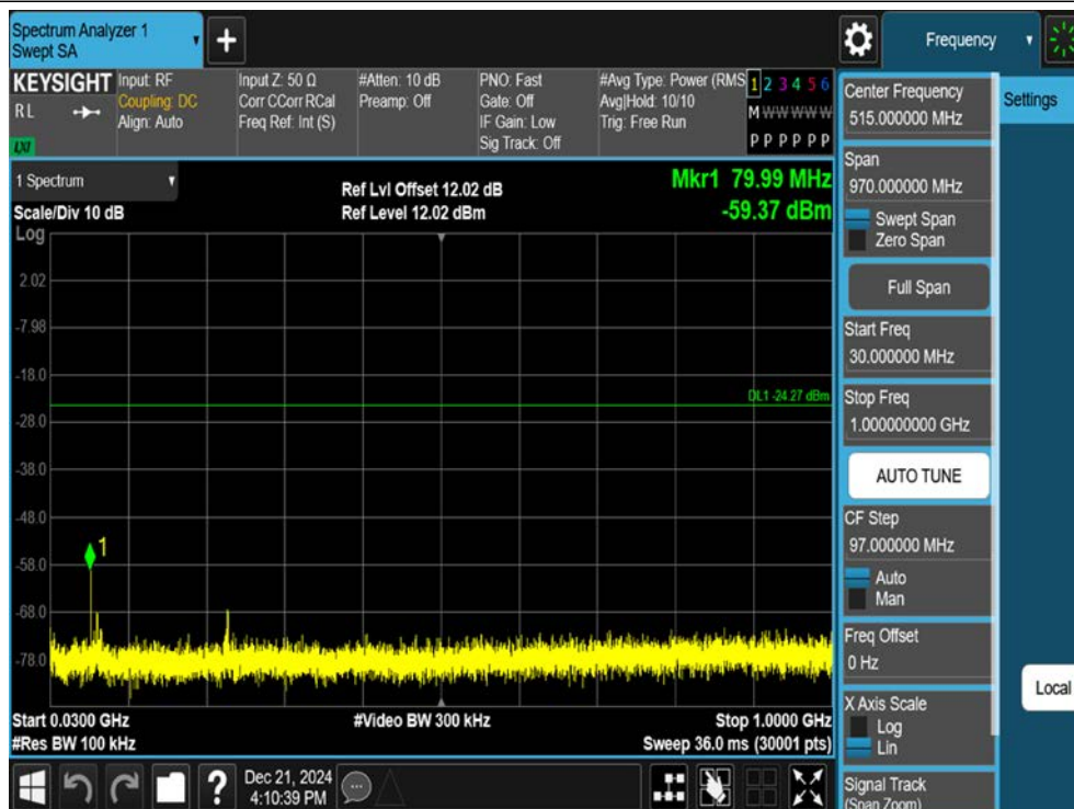
11B-Ant1-2437-30~1000-PASS
