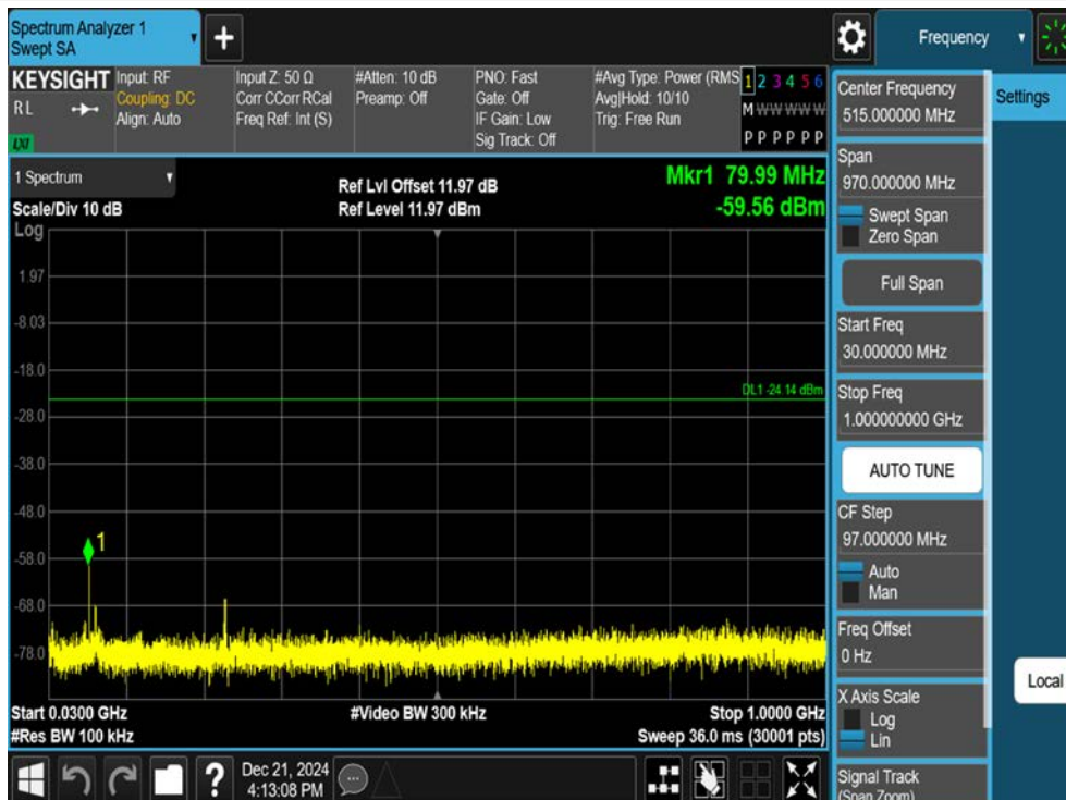
11B-Ant1-2462-30~1000-PASS
