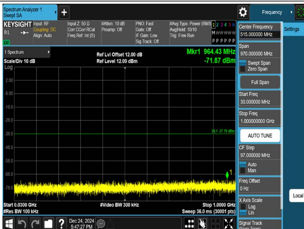
11N20SISO-Ant1-2412-30~1000-PASS
