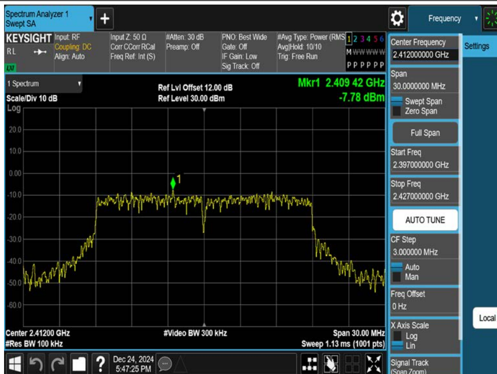
11N20SISO-Ant1-2412-0~Reference-PASS
