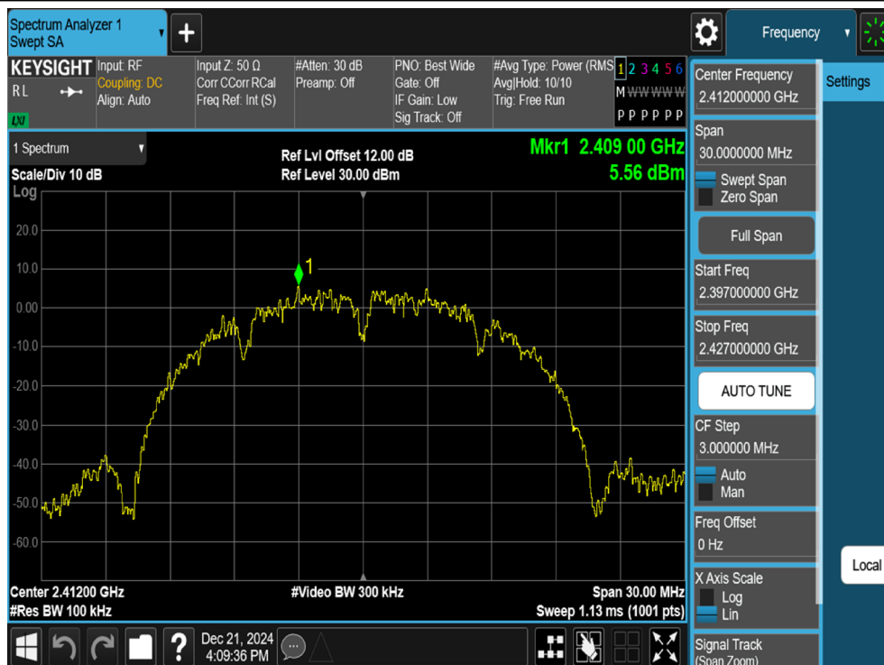
11B-Ant1-2412-0~Reference-PASS
