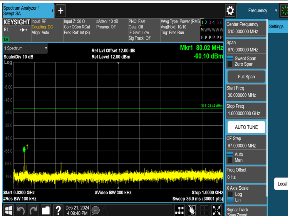
11B-Ant1-2412-30~1000-PASS
