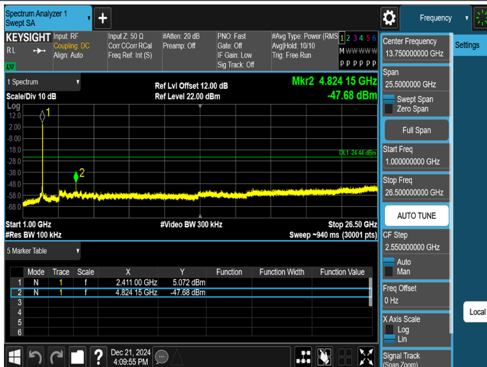
11B-Ant1-2412-1000~26500-PASS
