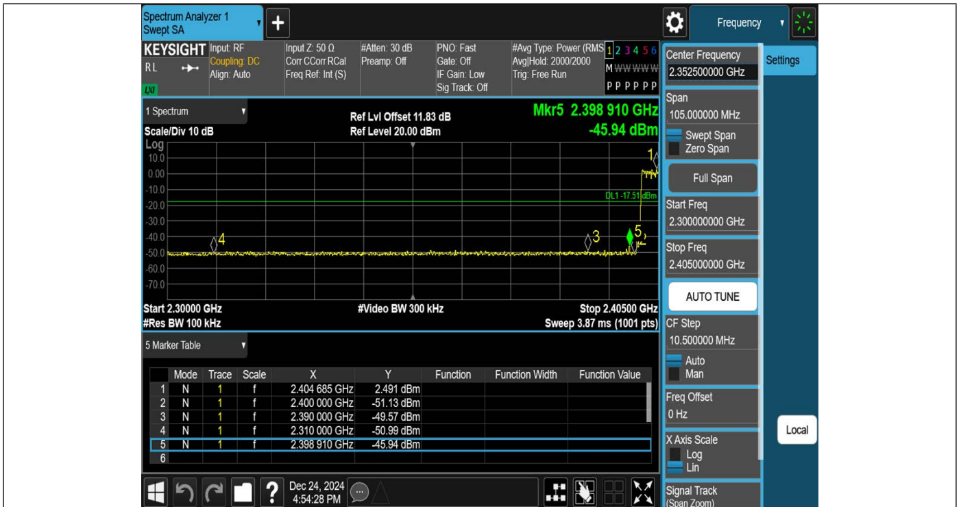
3DH5-Ant1-Hop_2402-PASS
