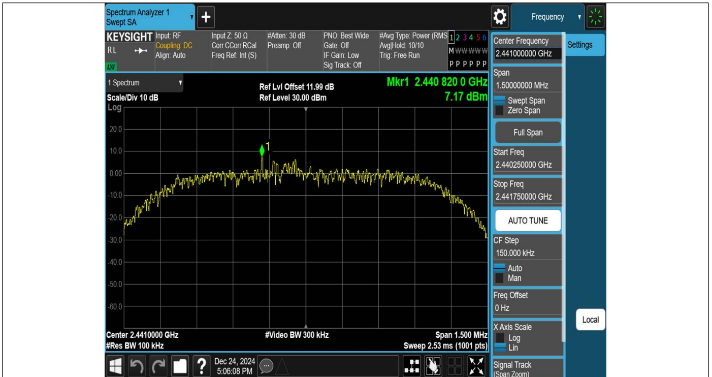
2DH5-Ant1-2441-0~Reference-PASS
