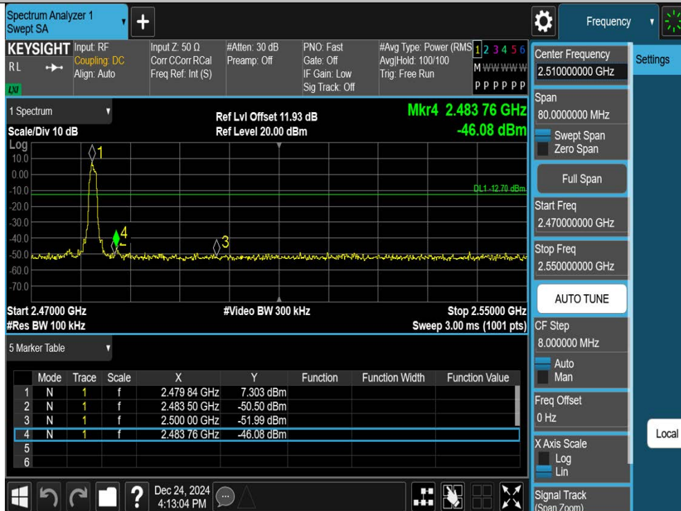
3DH5-Ant1-2480-PASS
