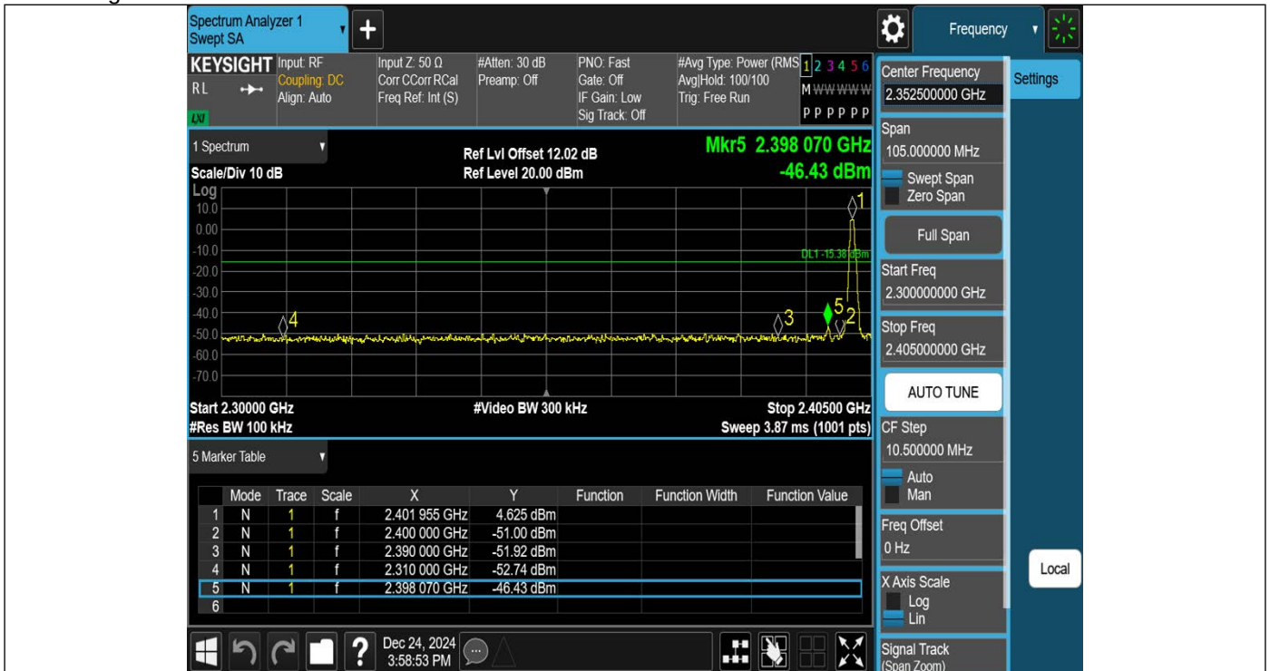
DH5-Ant1-2402-PASS
