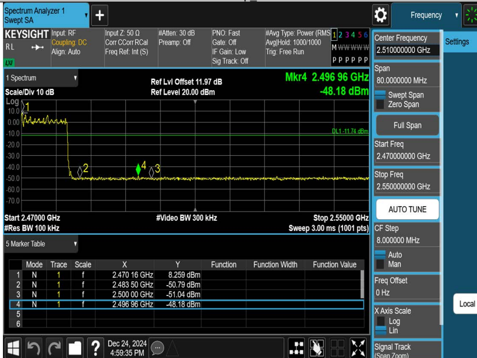
2DH5-Ant1-Hop_2480-PASS
