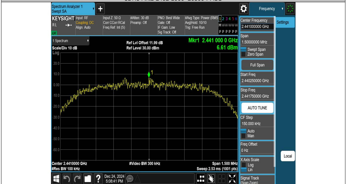
3DH5-Ant1-2441-0~Reference-PASS
