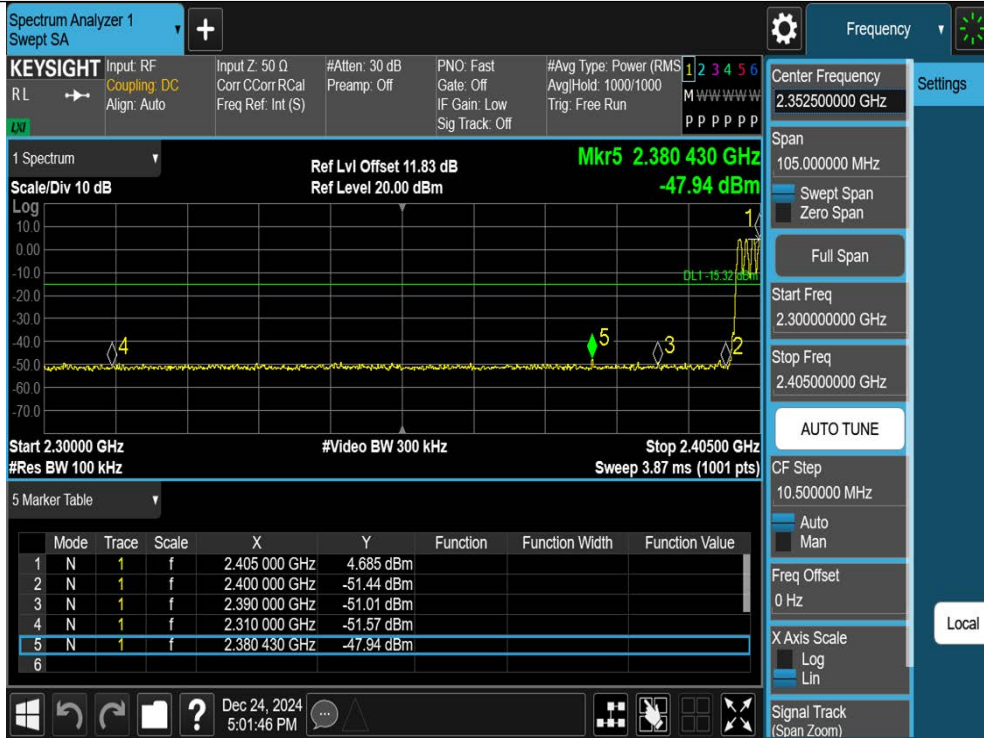
DH5-Ant1-Hop_2402-PASS
