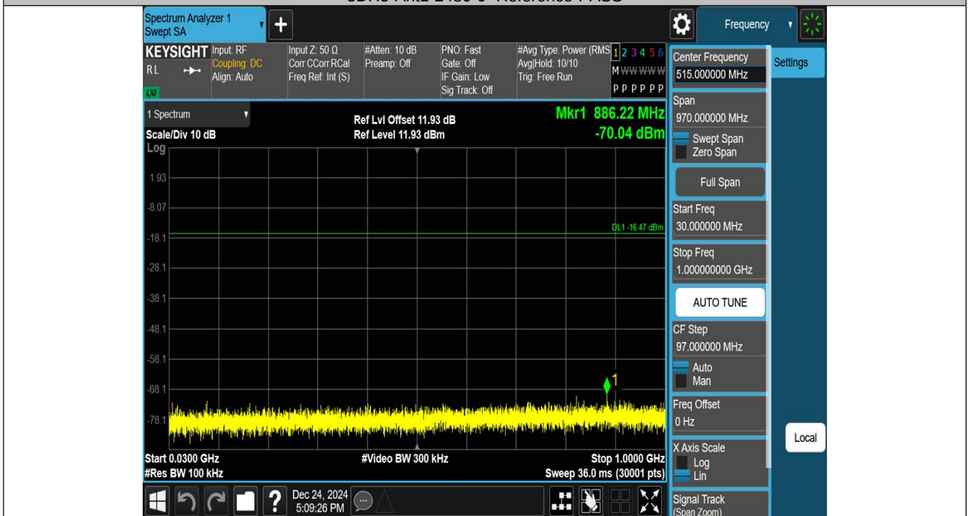
3DH5-Ant1-2480-30~1000-PASS
