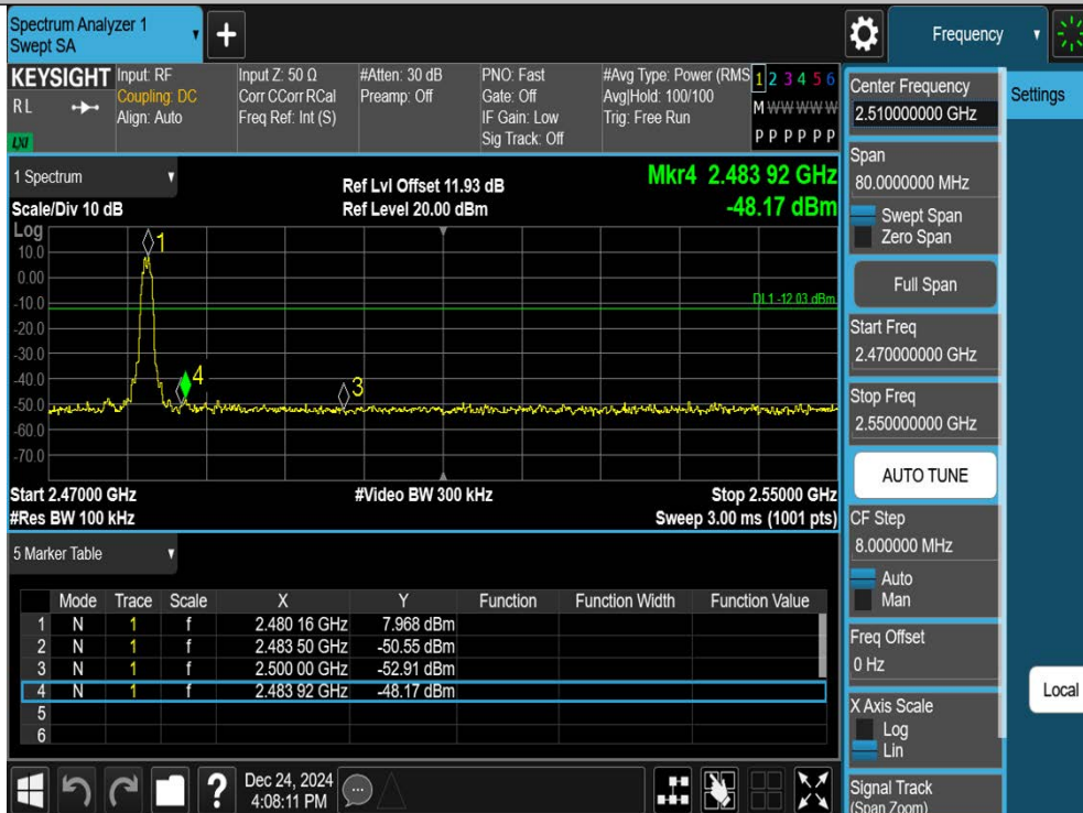
2DH5-Ant1-2480-PASS
