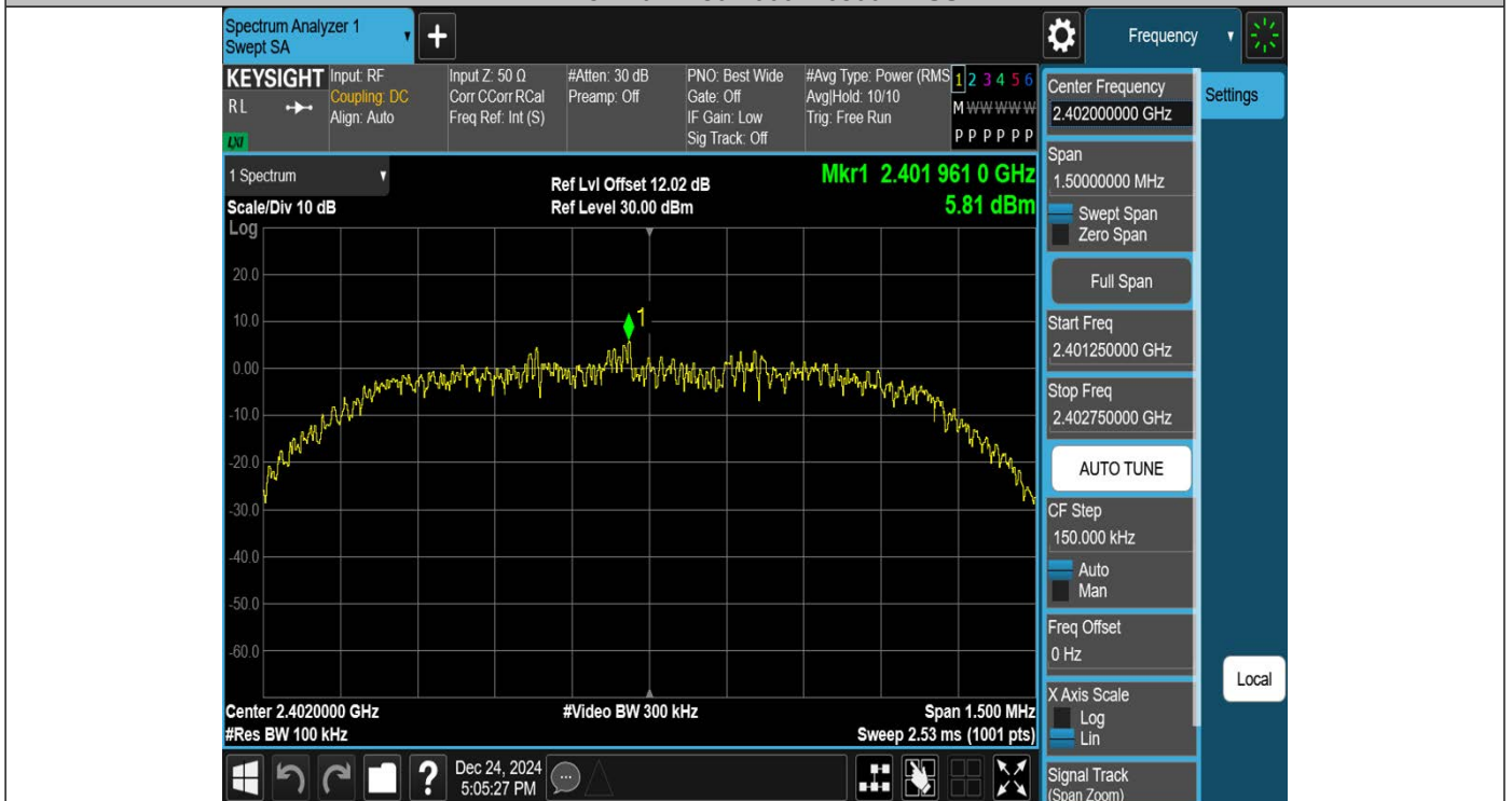
2DH5-Ant1-2402-0~Reference-PASS
