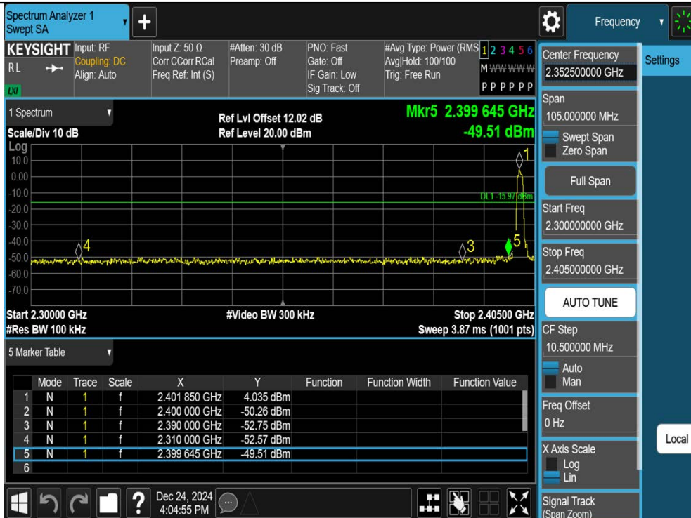
2DH5-Ant1-2402-PASS
