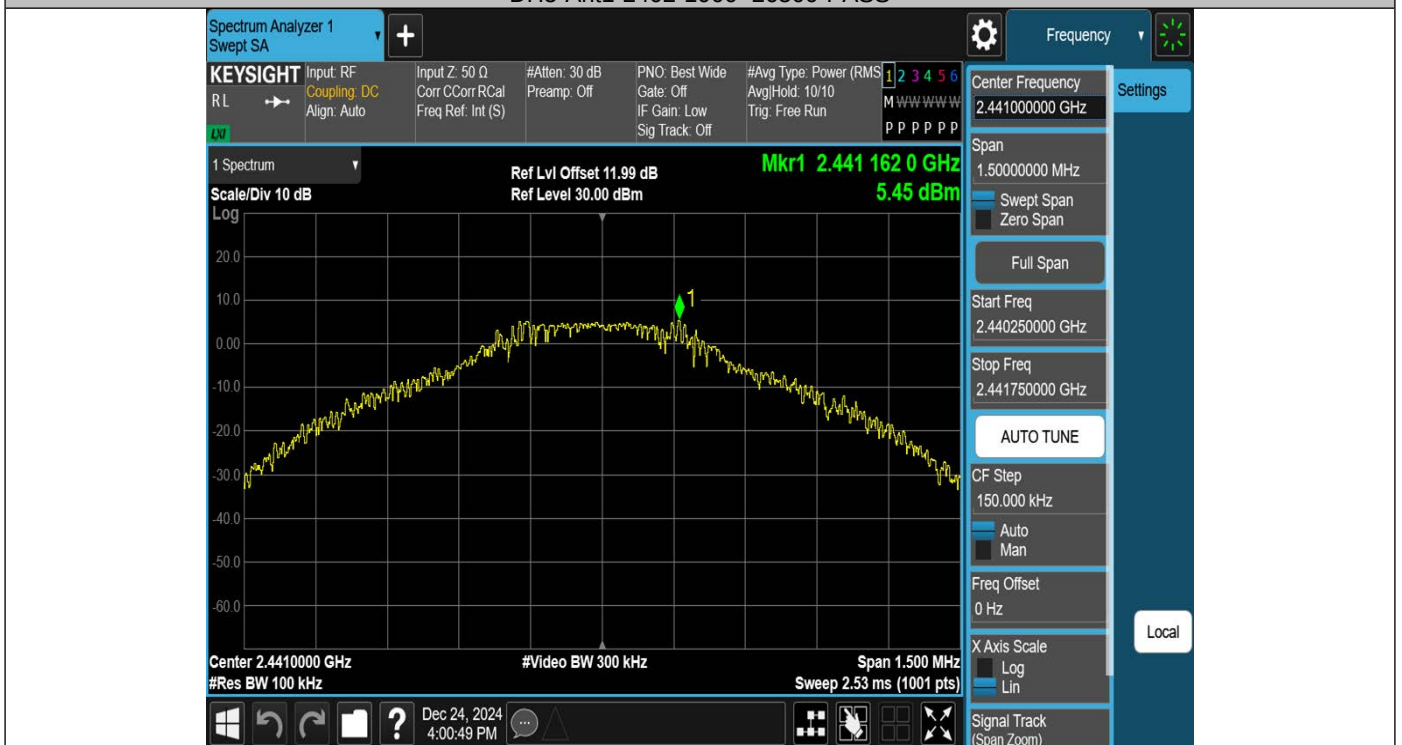
DH5-Ant1-2441-0~Reference-PASS
