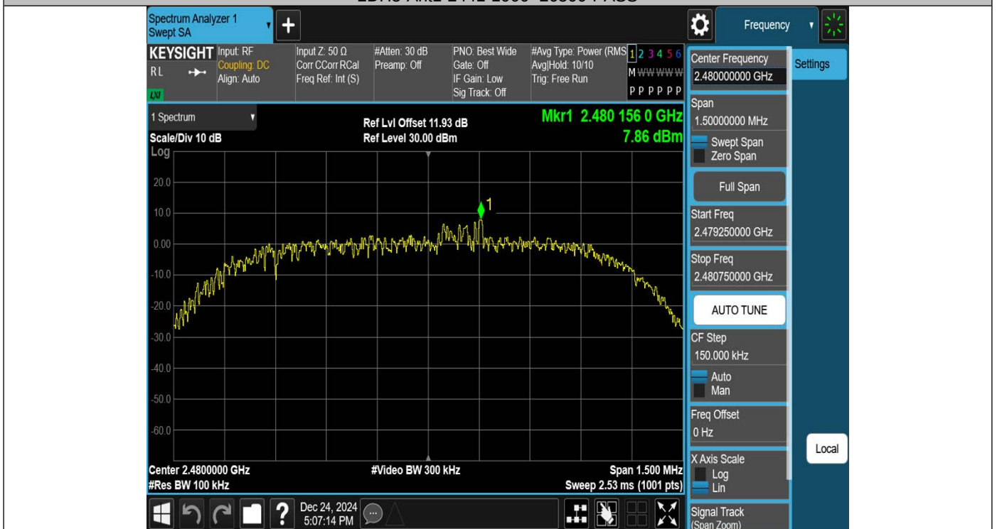
2DH5-Ant1-2480-0~Reference-PASS
