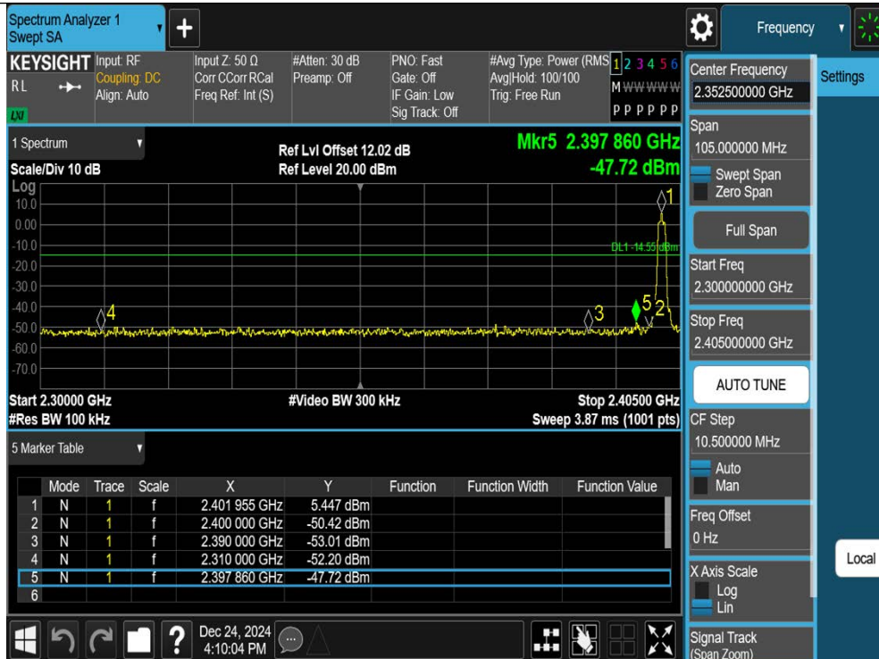
3DH5-Ant1-2402-PASS
