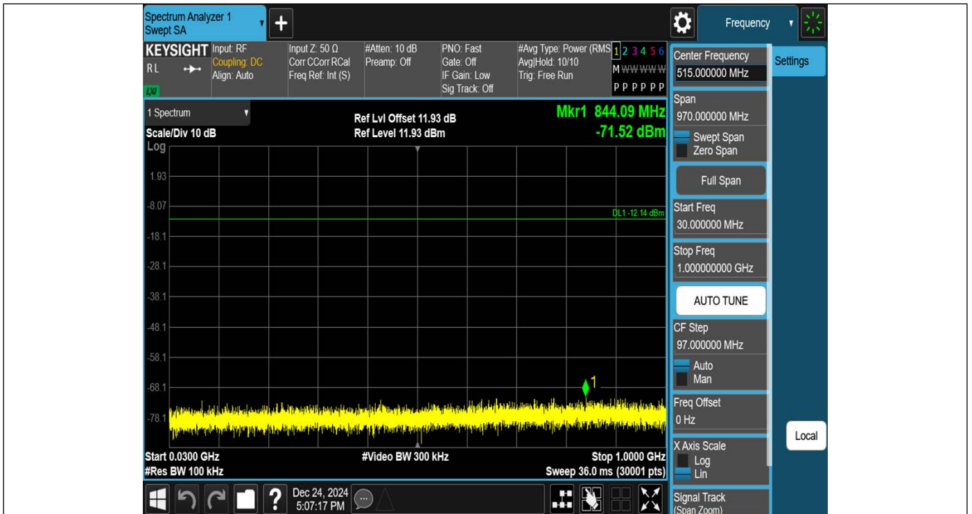
2DH5-Ant1-2480-30~1000-PASS
