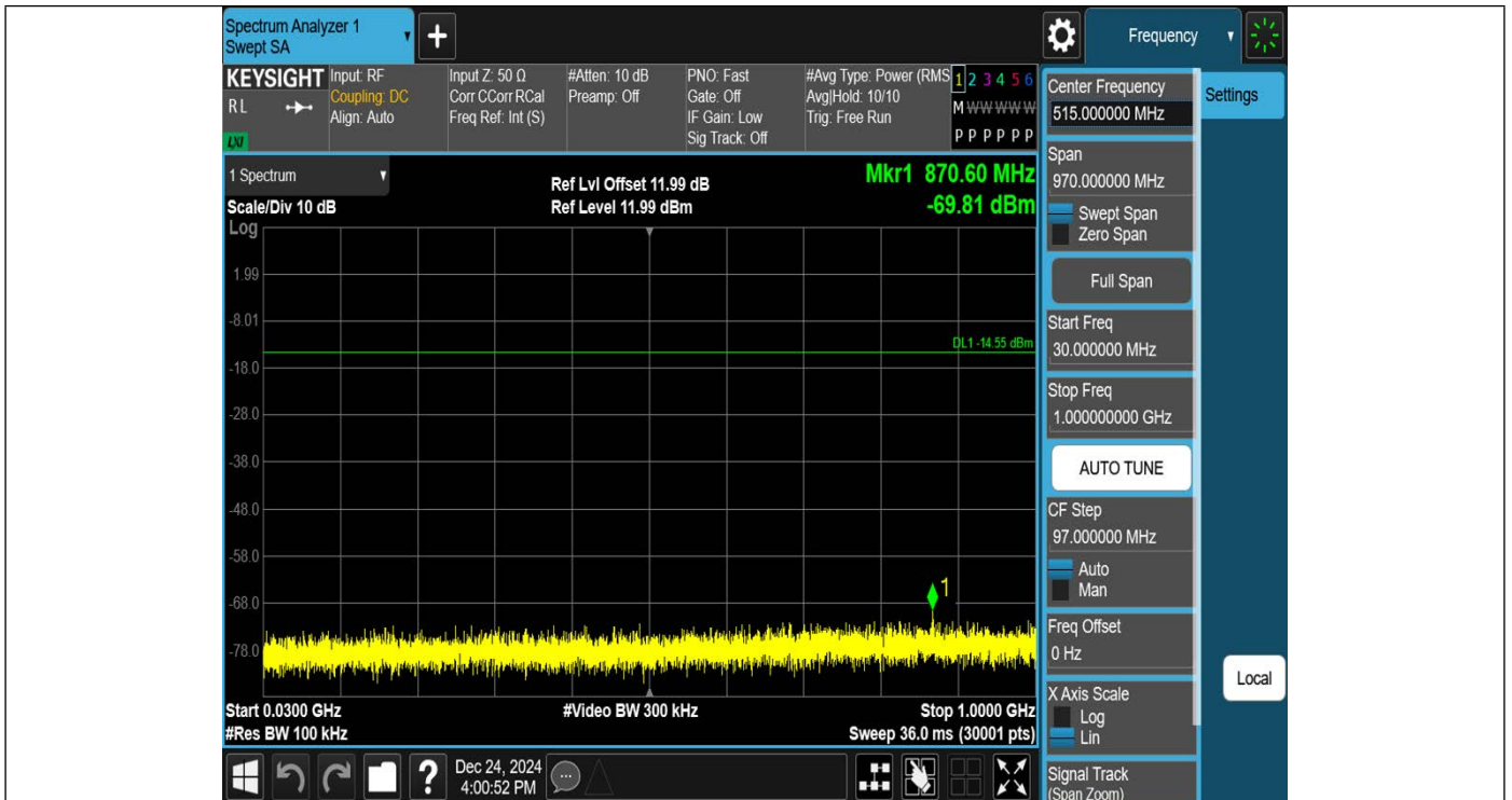
DH5-Ant1-2441-30~1000-PASS
