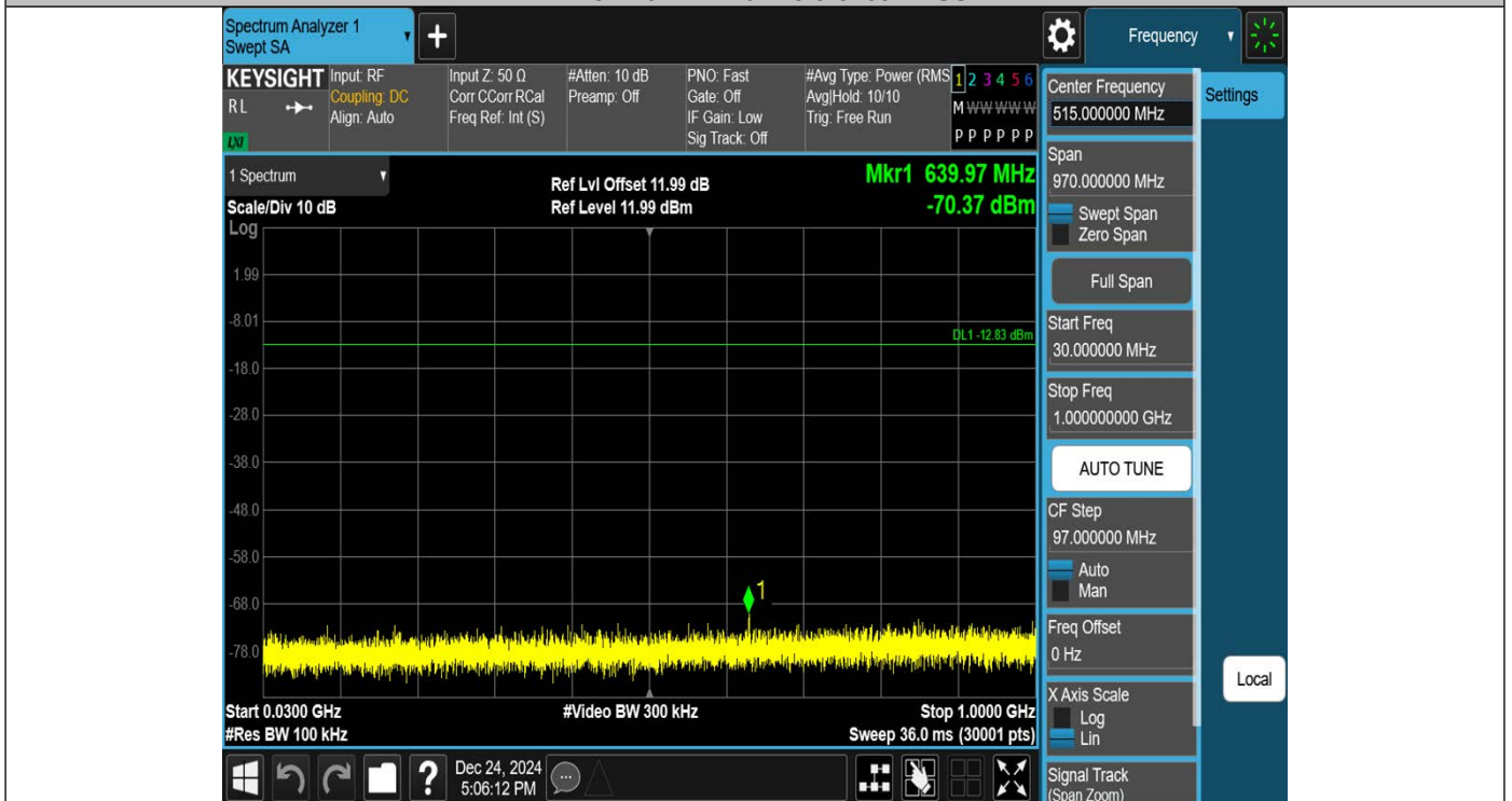
2DH5-Ant1-2441-30~1000-PASS
