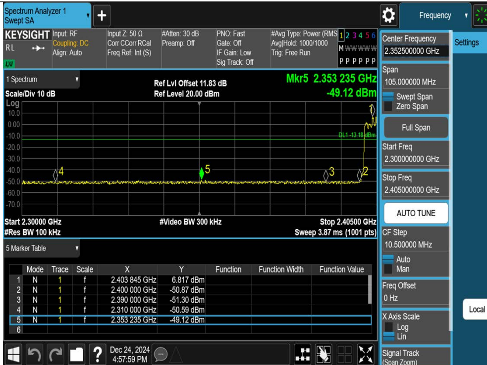
2DH5-Ant1-Hop_2402-PASS
