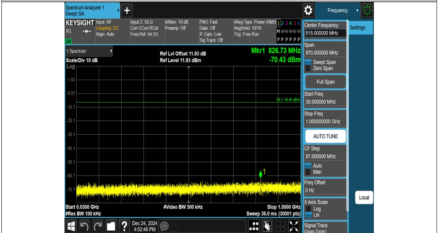
DH5-Ant1-2480-30-1000-PASS
