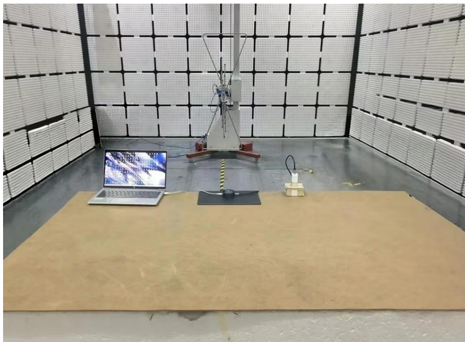
Radiated spurious emission Test Setup-1(Below 1GHz)
