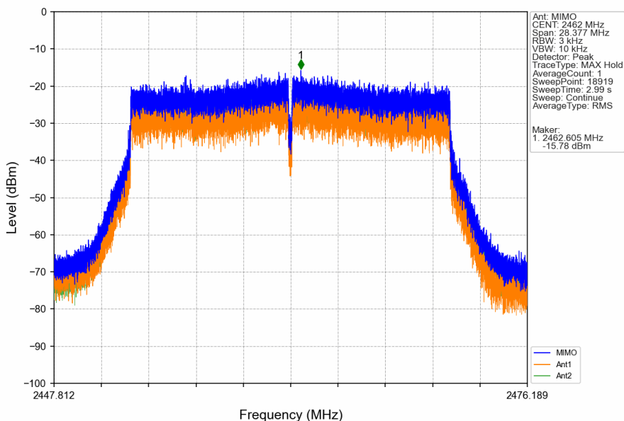
802.11ax(HEW20)_HCH_2462MHz_RU242_Left_MIMO_NTNV
