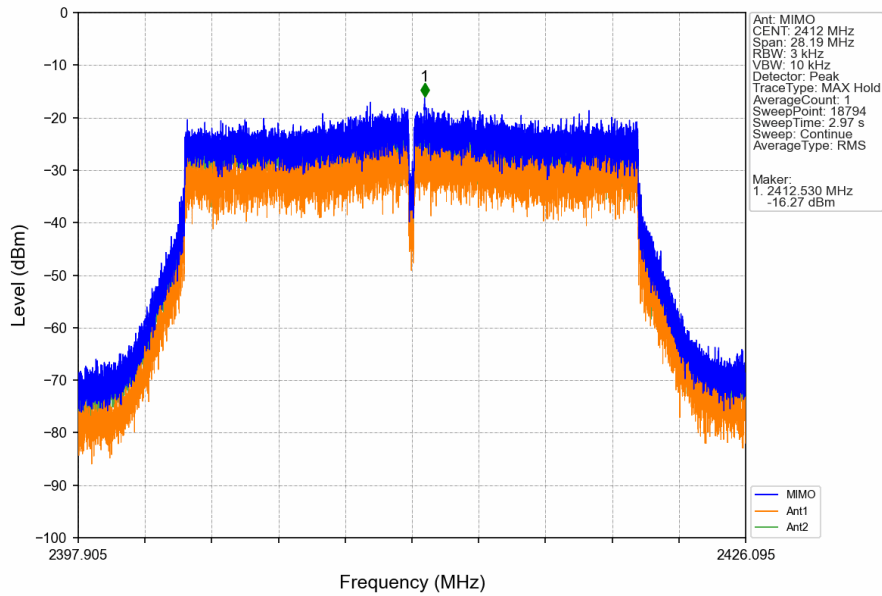
802.11ax(HEW20)_LCH_2412MHz_RU242_Left_MIMO_NTNV
