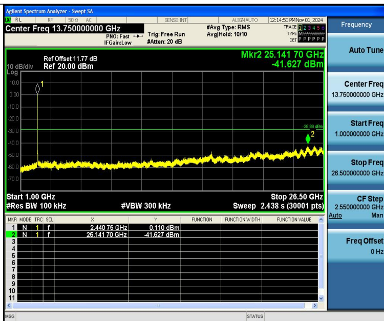
11G-Ant1-2437-1000~26500-PASS
