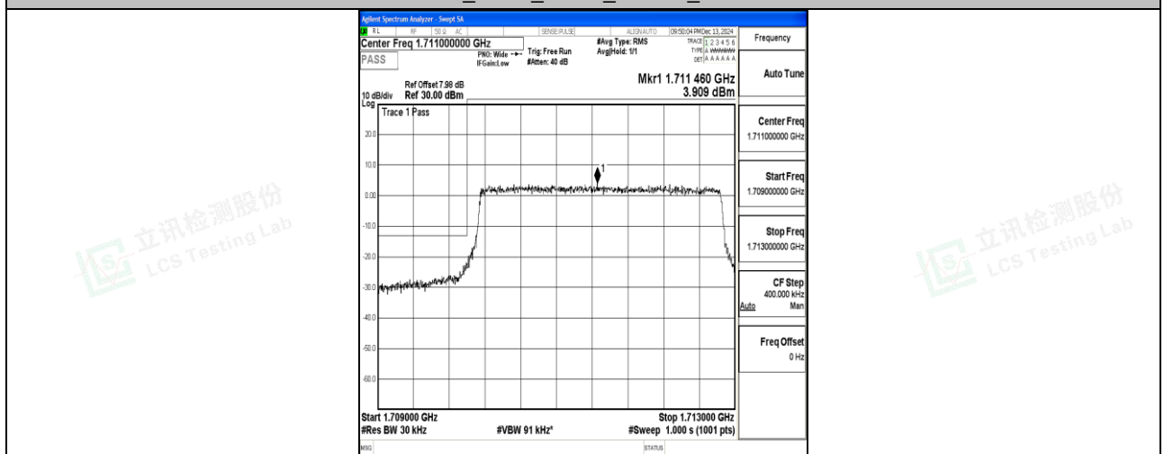
Band66_3MHz_16QAM_131987_15RB#0
