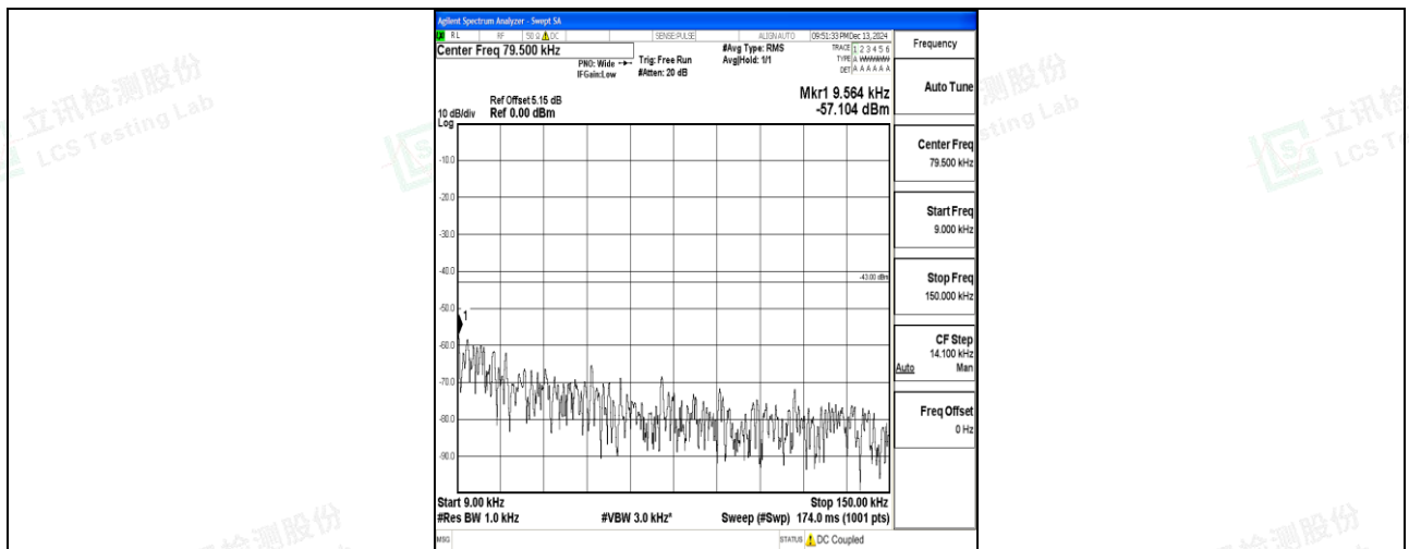
Band66_3MHz_QPSK_132322_1RB#0_0.009~0.15_0.009~0.15
