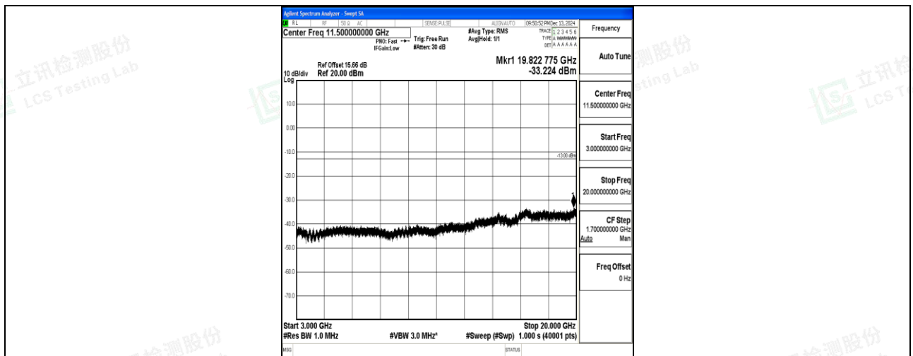
Band66_3MHz_QPSK_131987_1RB#0_3000~20000_3000~20000
