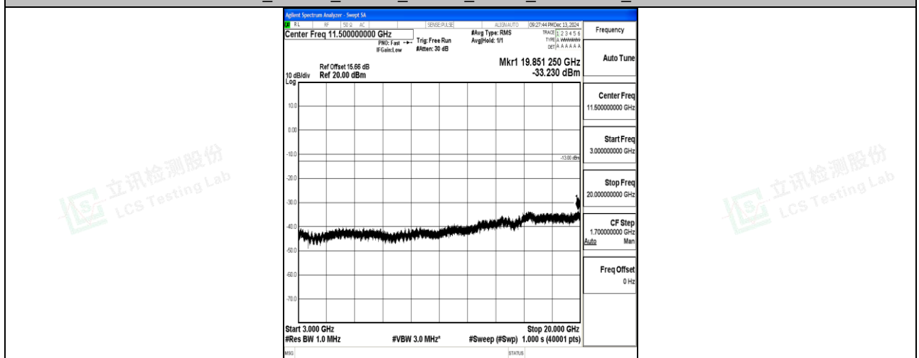
Band66_1.4MHz_16QAM_131979_1RB#0_3000~20000_3000~20000
