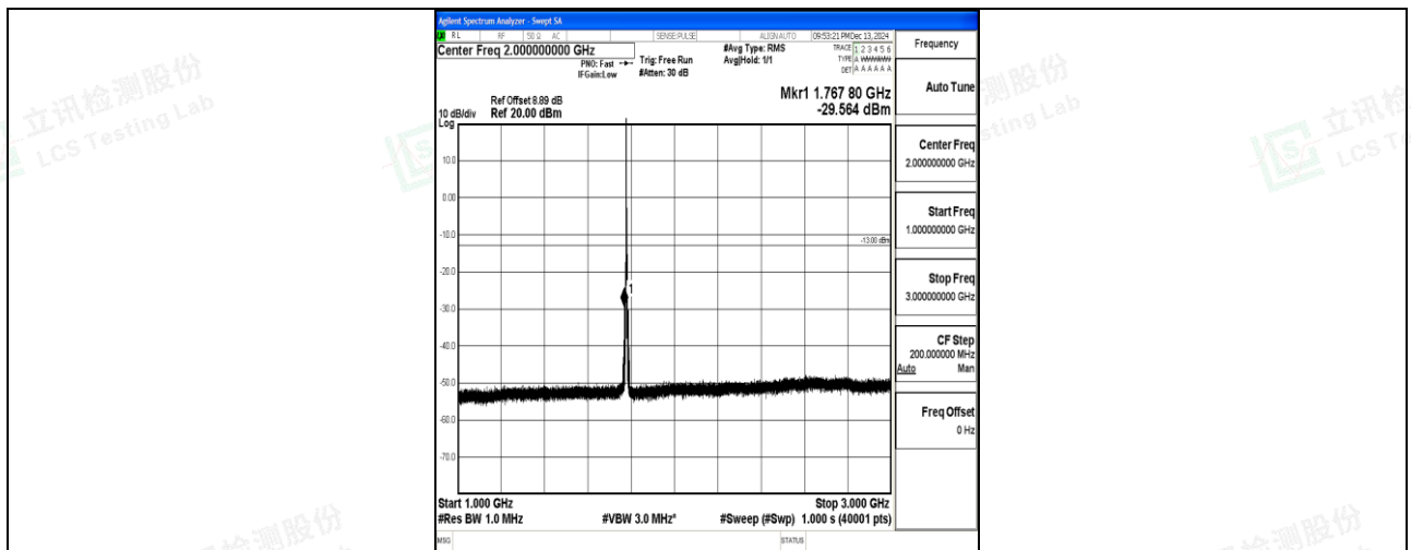
Band66_3MHz_16QAM_132657_1RB#0_1000~3000_1000~3000
