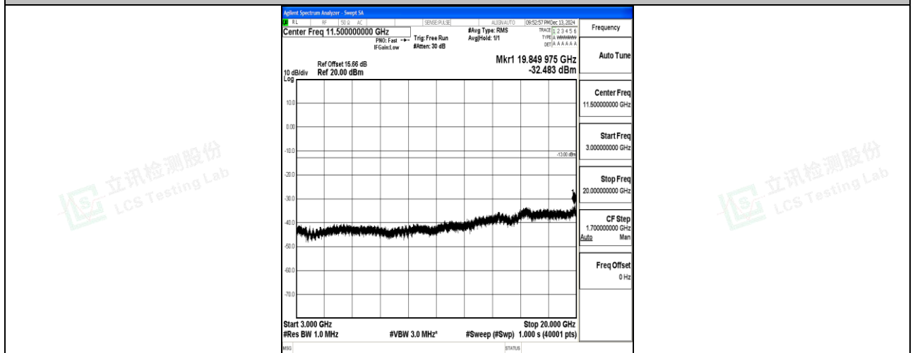
Band66_3MHz_QPSK_132657_1RB#0_3000~20000_3000~20000
