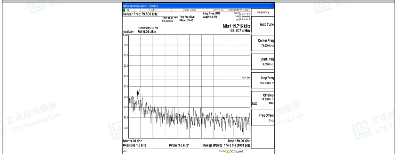
Band66_5MHz_16QAM_131997_1RB#0_0.009~0.15_0.009~0.15
