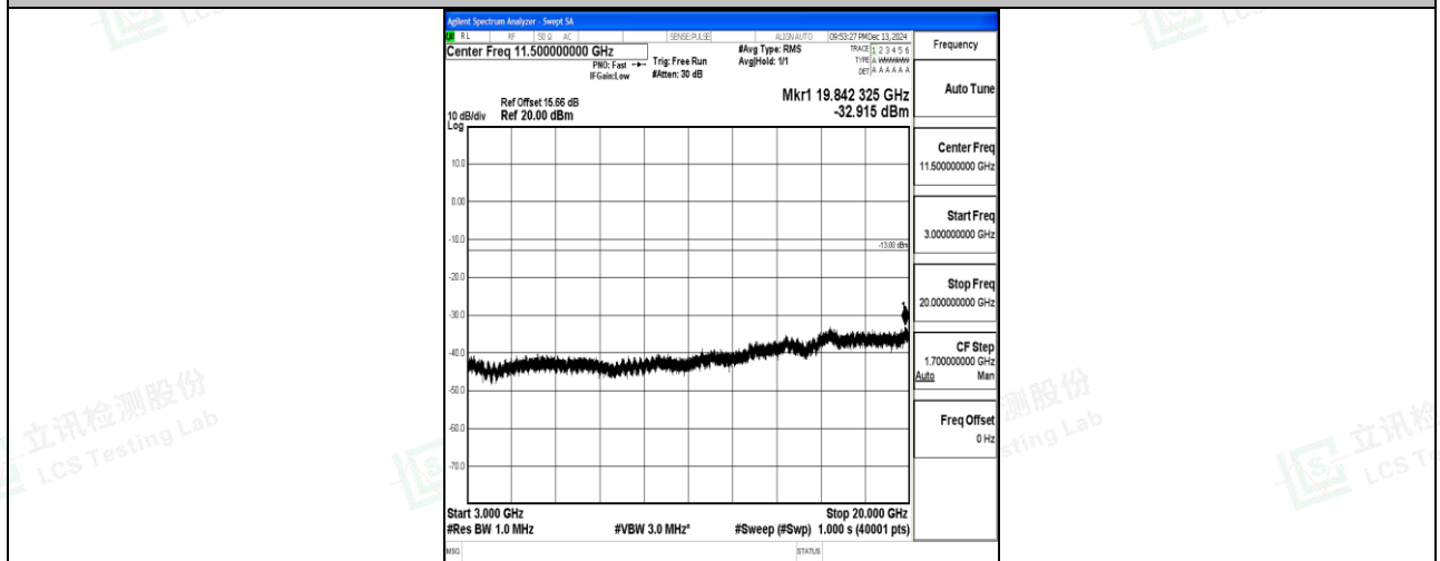
Band66_3MHz_16QAM_132657_1RB#0_3000~20000_3000~20000
