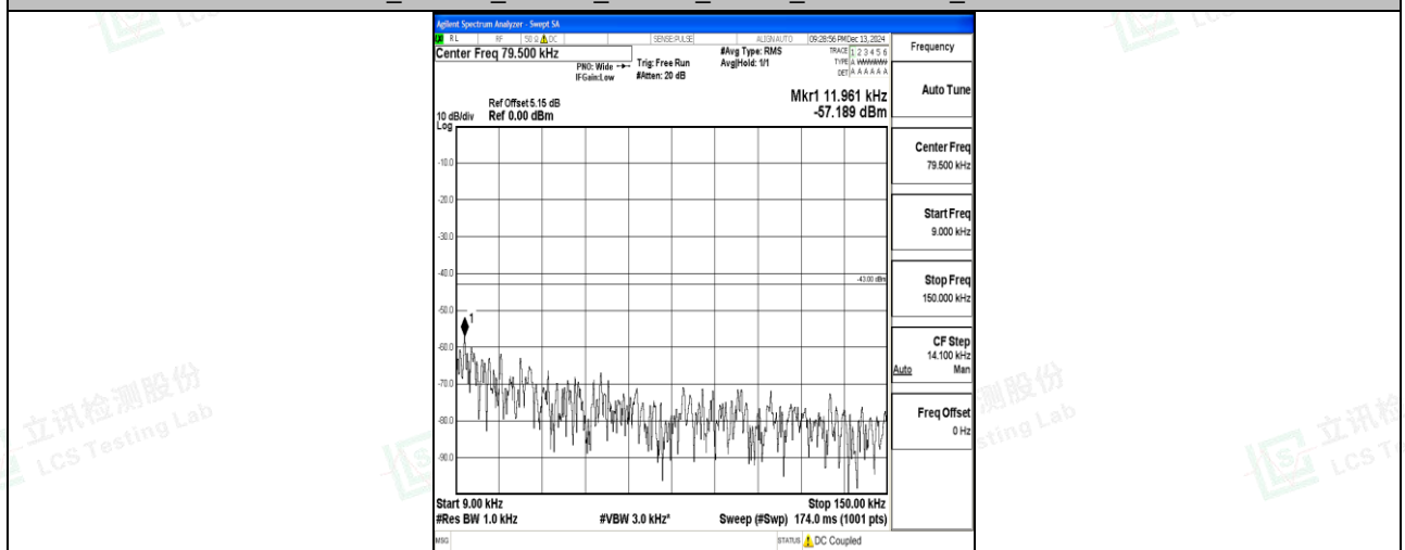
Band66_1.4MHz_QPSK_132665_1RB#0_0.009~0.15_0.009~0.15
