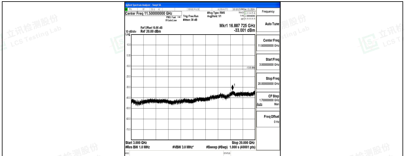
Band66_5MHz_QPSK_131997_1RB#0_3000~20000_3000~20000
