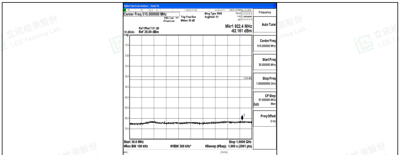
Band66_3MHz_16QAM_131987_1RB#0_30~1000_30~1000
