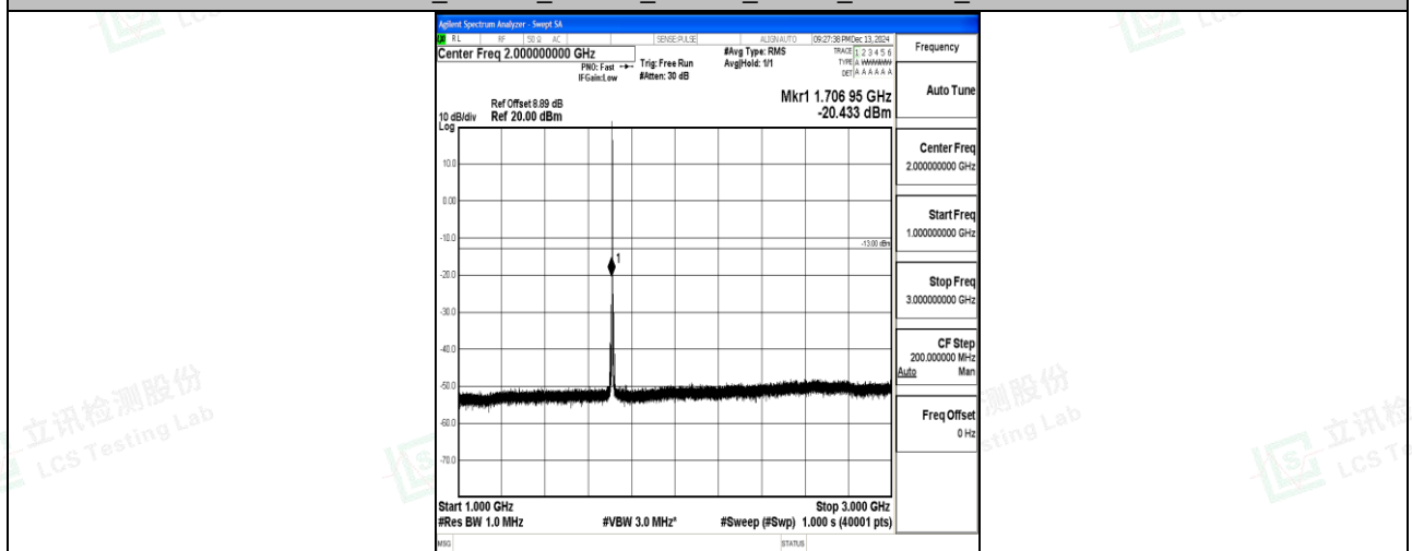
Band66_1.4MHz_16QAM_131979_1RB#0_1000~3000_1000~3000
