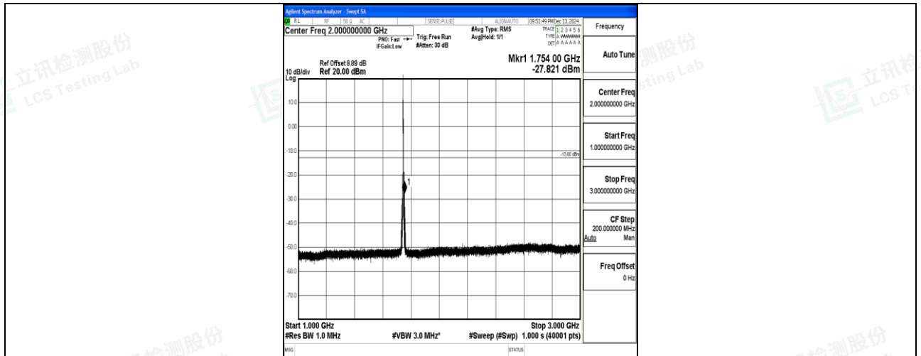
Band66_3MHz_QPSK_132322_1RB#0_1000~3000_1000~3000
