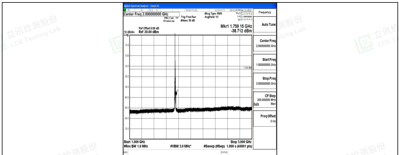
Band66_5MHz_QPSK_132322_1RB#0_1000~3000_1000~3000
