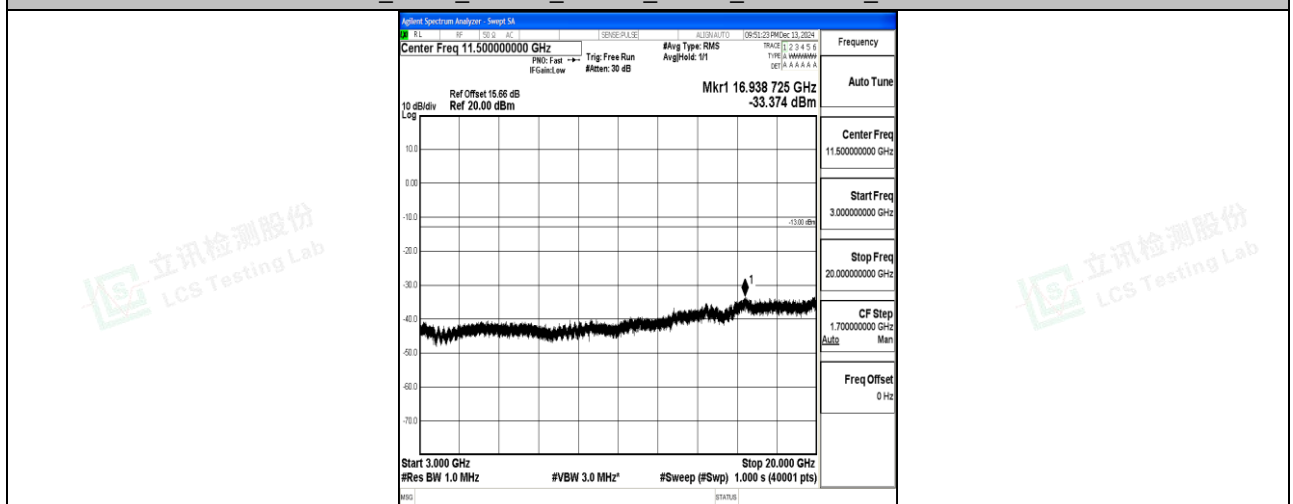
Band66_3MHz_16QAM_131987_1RB#0_3000~20000_3000~20000
