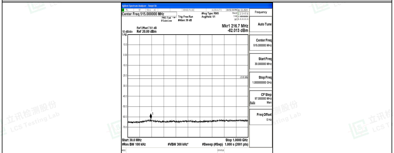
Band66_3MHz_QPSK_131987_1RB#0_30~1000_30~1000
