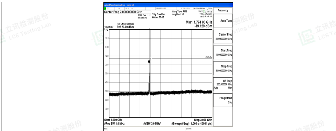
Band66_1.4MHz_16QAM_132665_1RB#0_1000~3000_1000~3000
