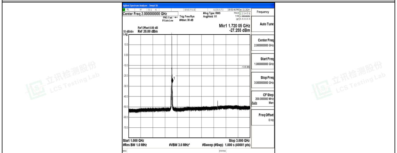
Band66_3MHz_QPSK_131987_1RB#0_1000~3000_1000~3000
