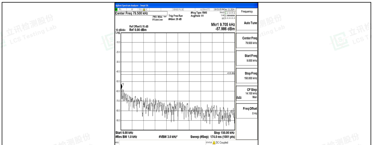
Band66_3MHz_16QAM_132657_1RB#0_0.009~0.15_0.009~0.15
