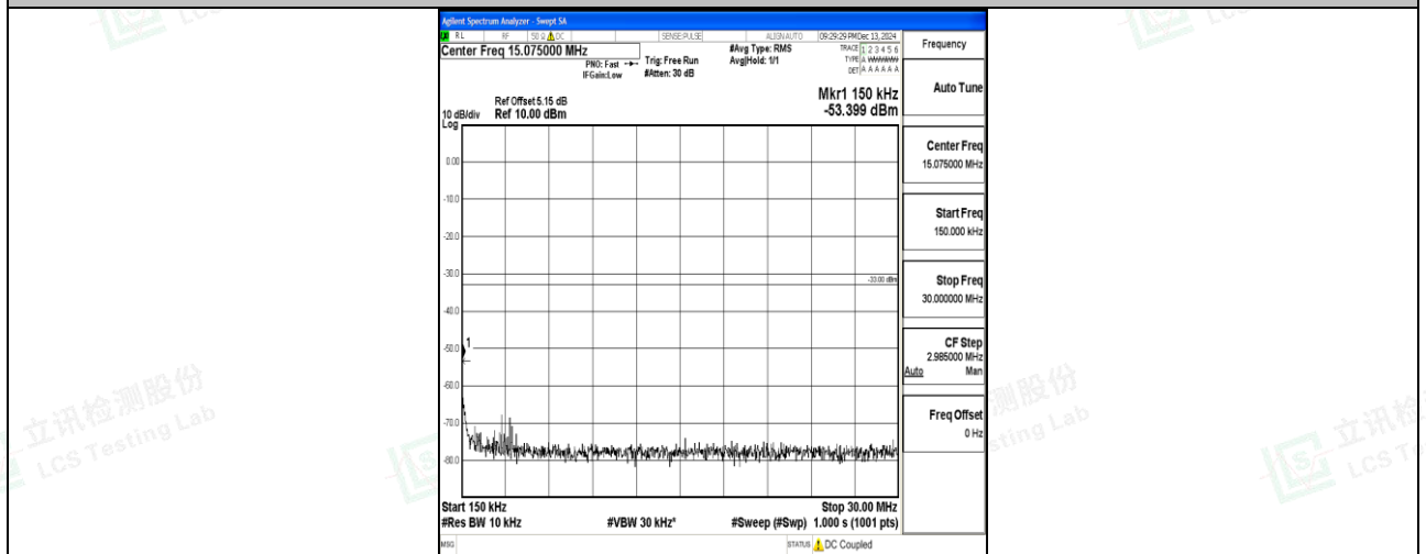
Band66_1.4MHz_16QAM_132665_1RB#0_0.15~30_0.15~30
