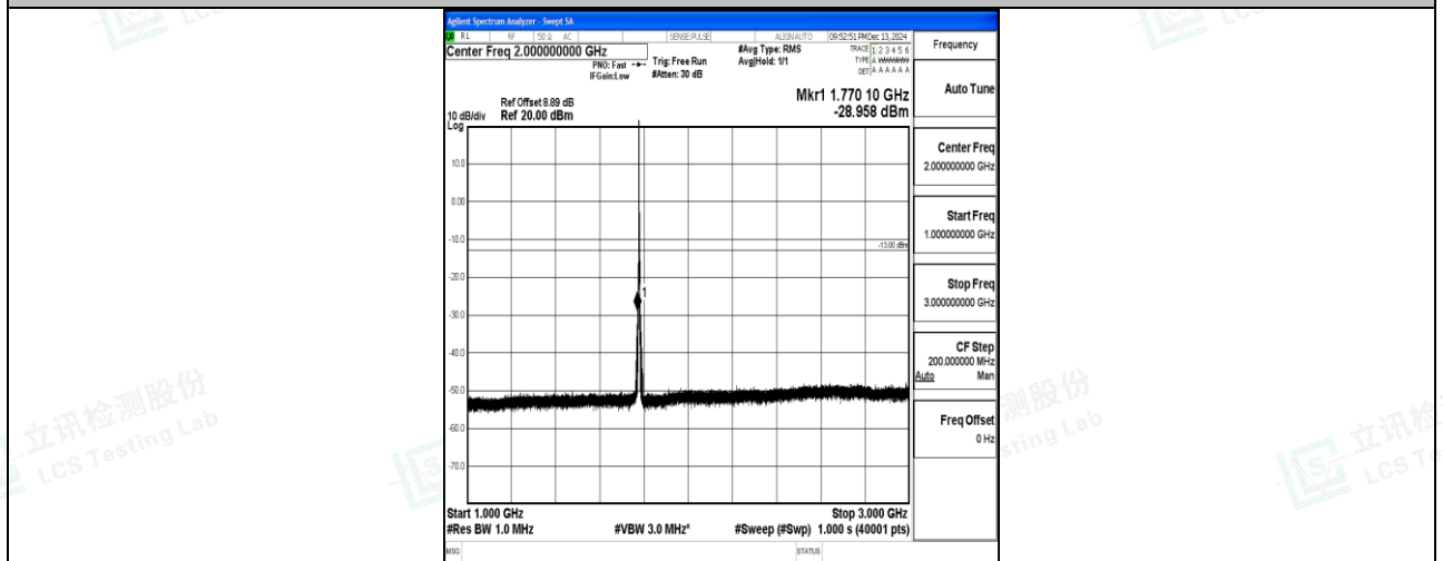
Band66_3MHz_QPSK_132657_1RB#0_1000~3000_1000~3000
