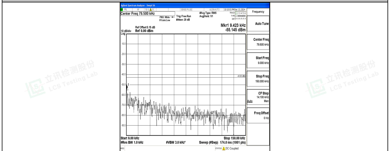
Band66_5MHz_QPSK_131997_1RB#0_0.009~0.15_0.009~0.15
