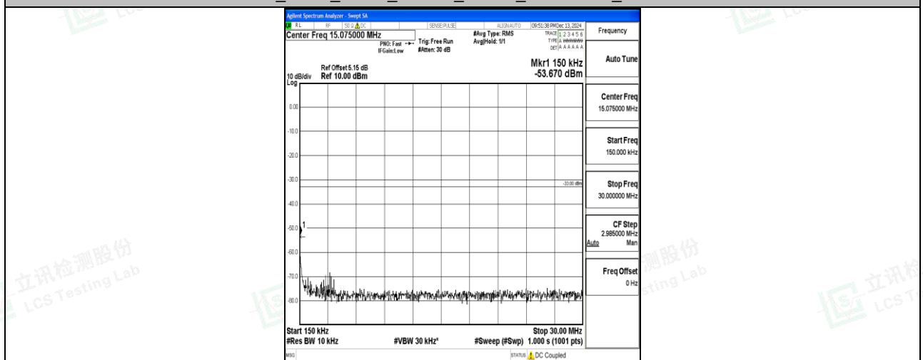
Band66_3MHz_QPSK_132322_1RB#0_0.15~30_0.15~30
