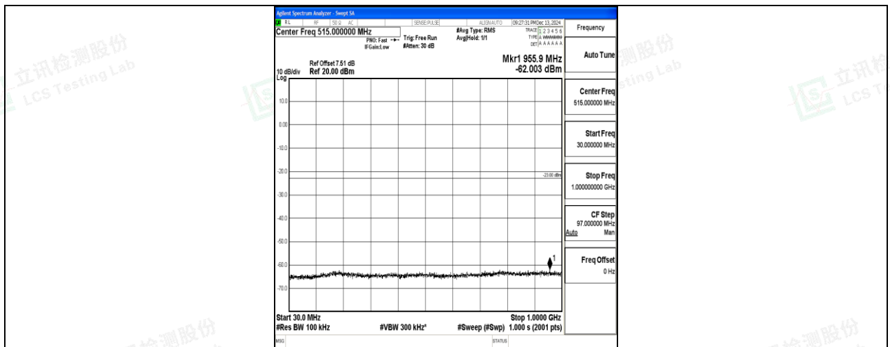
Band66_1.4MHz_16QAM_131979_1RB#0_30~1000_30~1000
