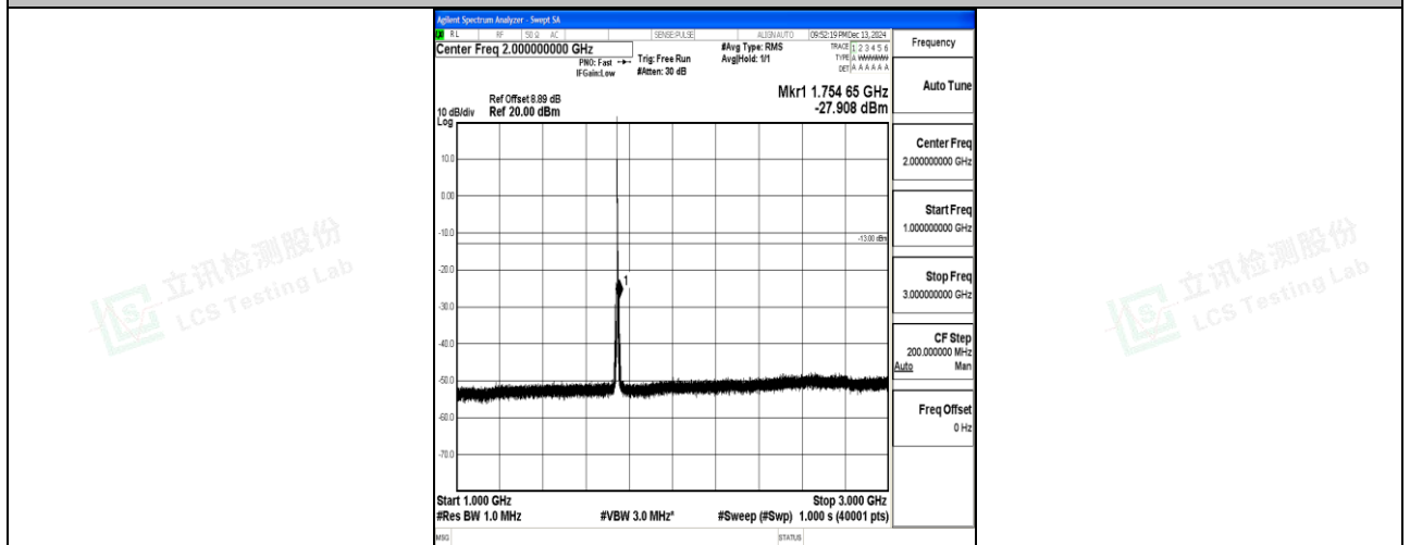
Band66_3MHz_16QAM_132322_1RB#0_1000~3000_1000~3000
