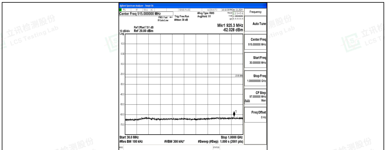
Band66_5MHz_16QAM_131997_1RB#0_30~1000_30~1000
