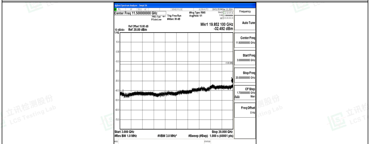
Band66_3MHz_QPSK_132322_1RB#0_3000~20000_3000~20000
