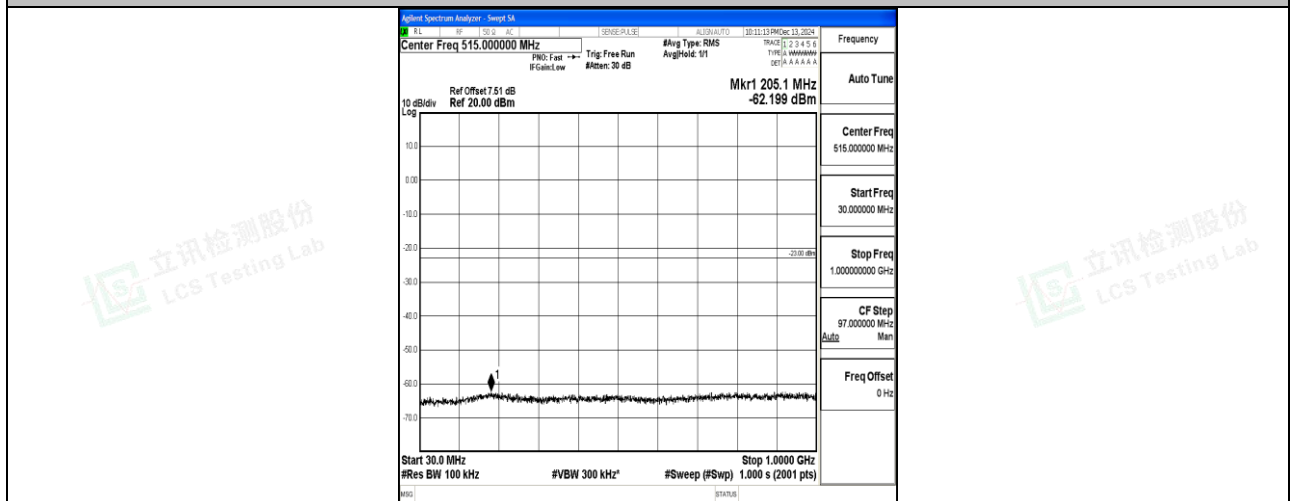
Band66_5MHz_QPSK_132322_1RB#0_30~1000_30~1000
