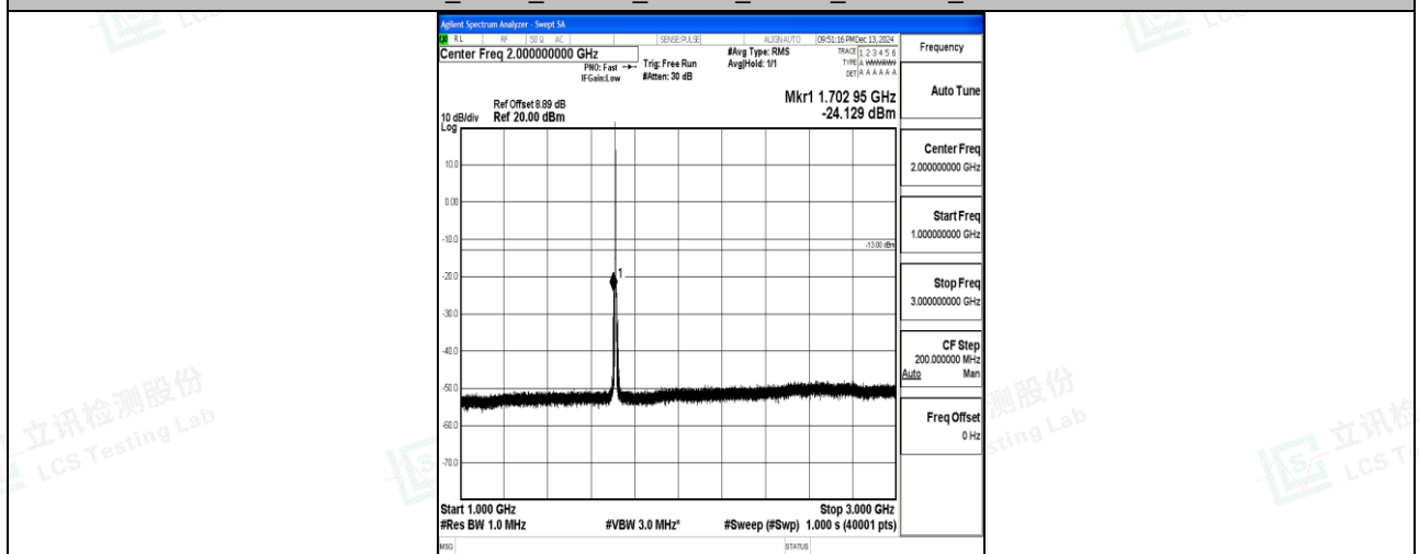
Band66_3MHz_16QAM_131987_1RB#0_1000~3000_1000~3000
