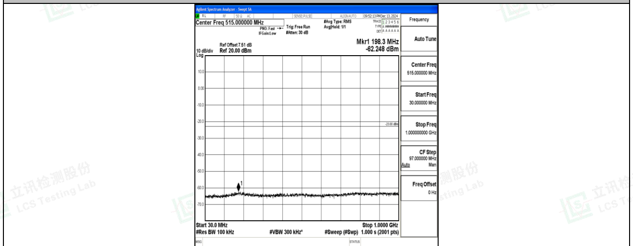
Band66_3MHz_16QAM_132322_1RB#0_30~1000_30~1000
