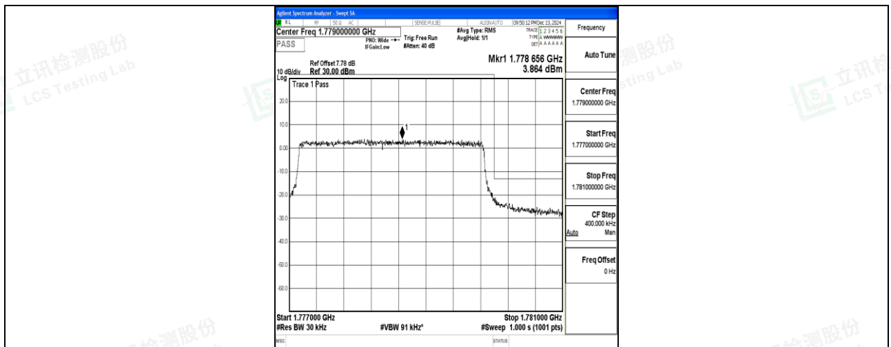
Band66_3MHz_QPSK_132657_15RB#0
