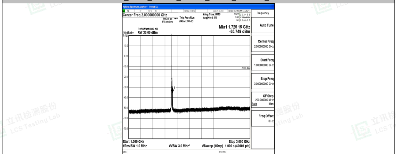
Band66_5MHz_16QAM_131997_1RB#0_1000~3000_1000~3000
