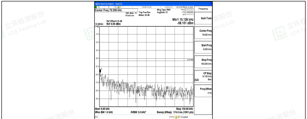
Band66_5MHz_QPSK_132322_1RB#0_0.009~0.15_0.009~0.15
