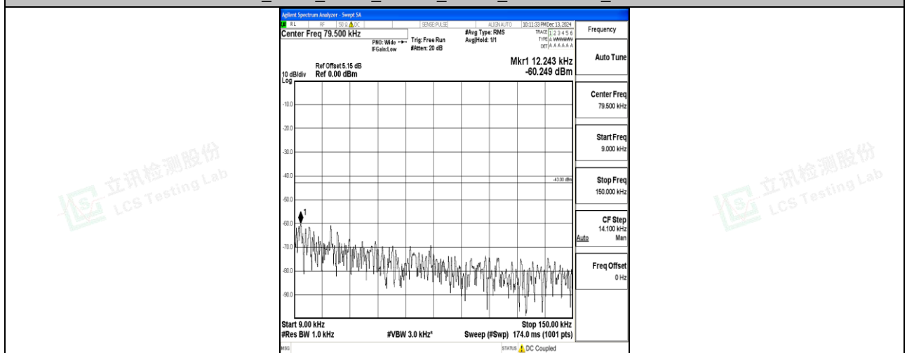
Band66_5MHz_16QAM_132322_1RB#0_0.009~0.15_0.009~0.15
