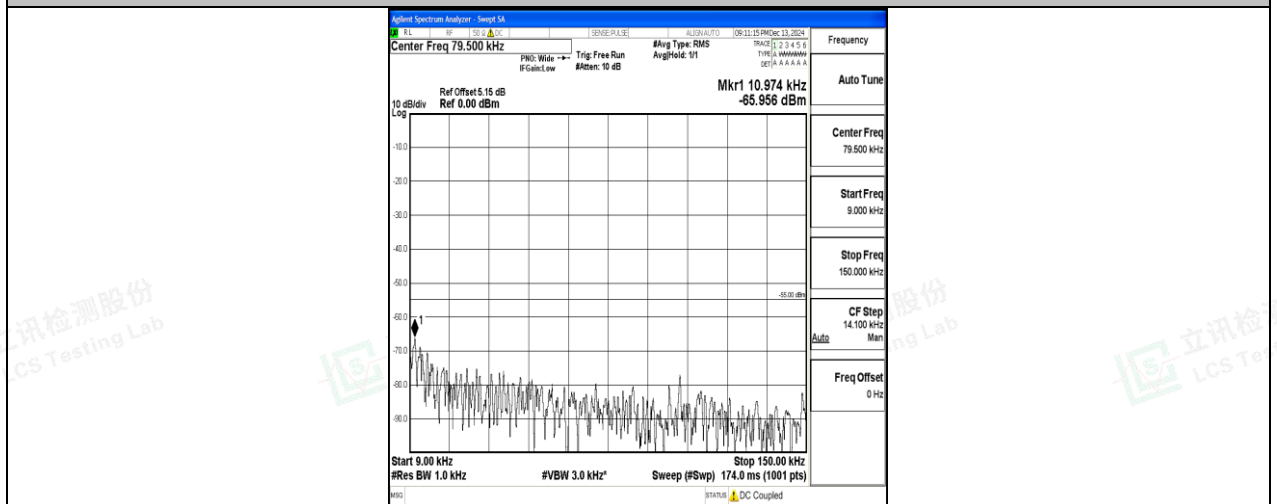
Band7_20MHz_QPSK_20850_1RB#0_0.009~0.15_0.009~0.15
