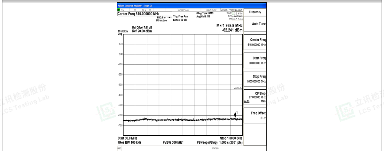
Band7_20MHz_16QAM_21350_1RB#0_30~1000_30~1000
