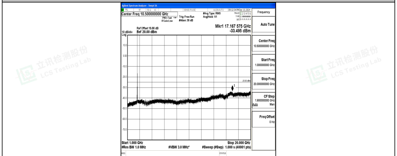
Band7_20MHz_QPSK_21100_1RB#0_1000~20000_1000~20000
