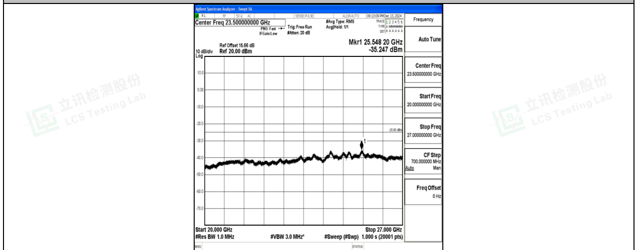
Band7_20MHz_16QAM_21100_1RB#0_20000~27000_20000~27000
