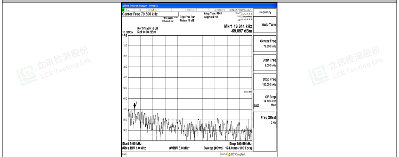
Band7_15MHz_QPSK_21100_1RB#0_0.009~0.15_0.009~0.15
