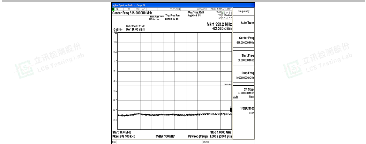
Band7_15MHz_16QAM_20825_1RB#0_30~1000_30~1000
