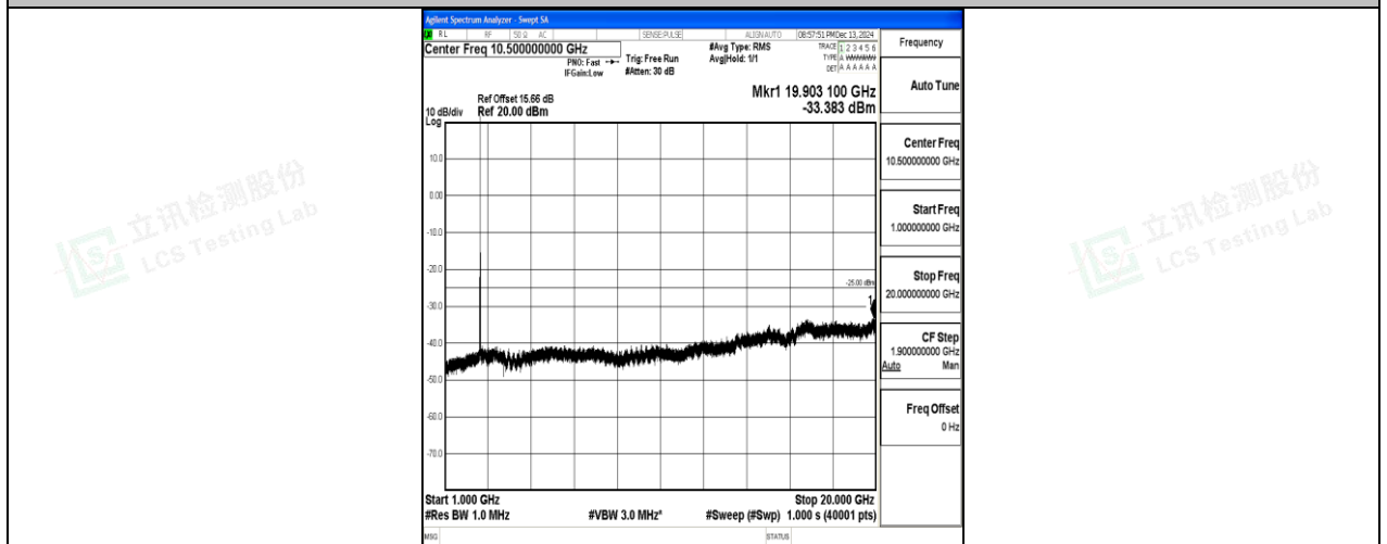
Band7_15MHz_16QAM_21375_1RB#0_1000~20000_1000~20000
