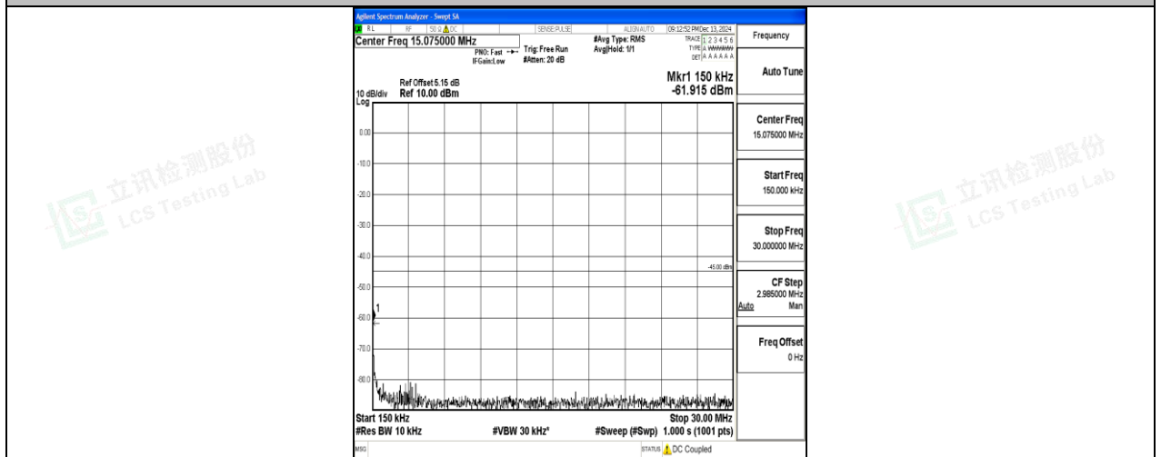
Band7_20MHz_16QAM_21100_1RB#0_0.15~30_0.15~30
