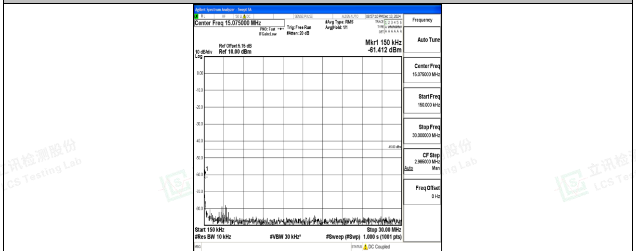
Band7_15MHz_QPSK_21375_1RB#0_0.15~30_0.15~30
