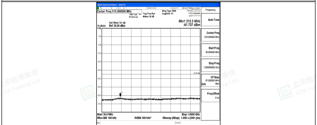
Band7_20MHz_QPSK_21100_1RB#0_30~1000_30~1000
