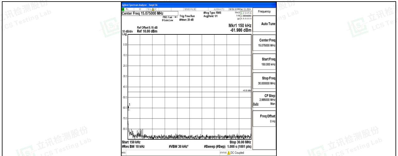
Band7_15MHz_QPSK_21100_1RB#0_0.15~30_0.15~30
