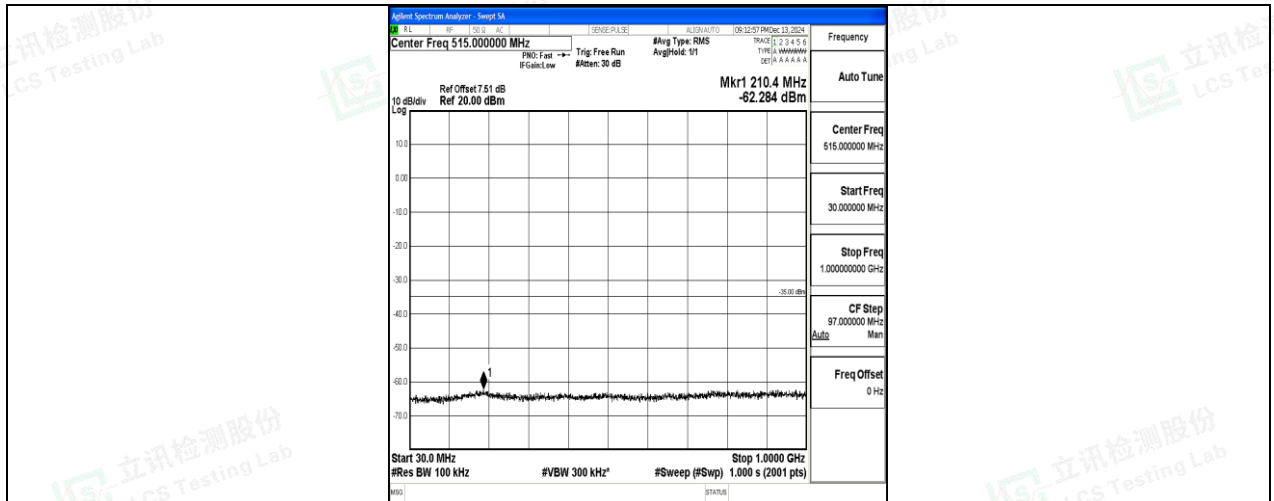
Band7_20MHz_16QAM_21100_1RB#0_30~1000_30~1000
