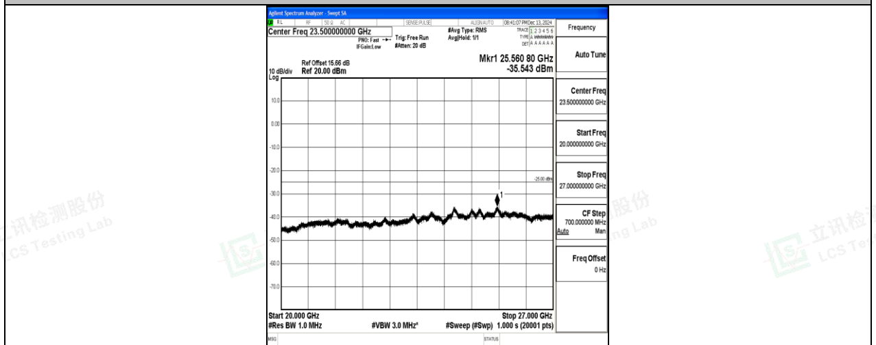
Band7_10MHz_QPSK_21400_1RB#0_20000~27000_20000~27000
