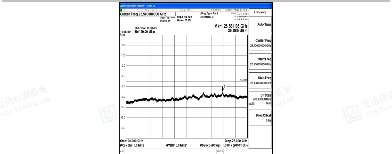
Band7_15MHz_16QAM_20825_1RB#0_20000~27000_20000~27000
