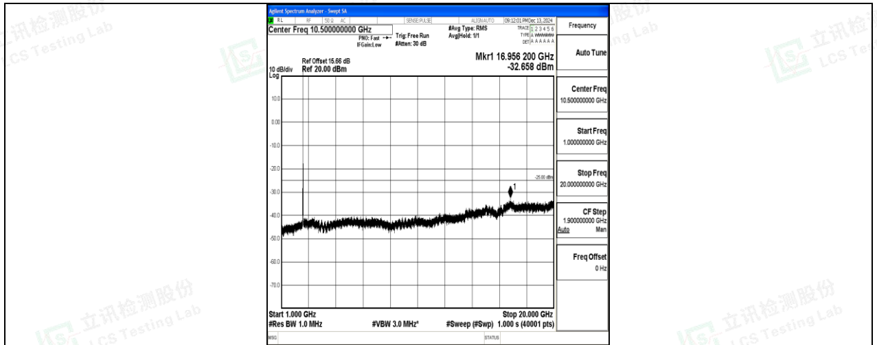
Band7_20MHz_16QAM_20850_1RB#0_1000~20000_1000~20000
