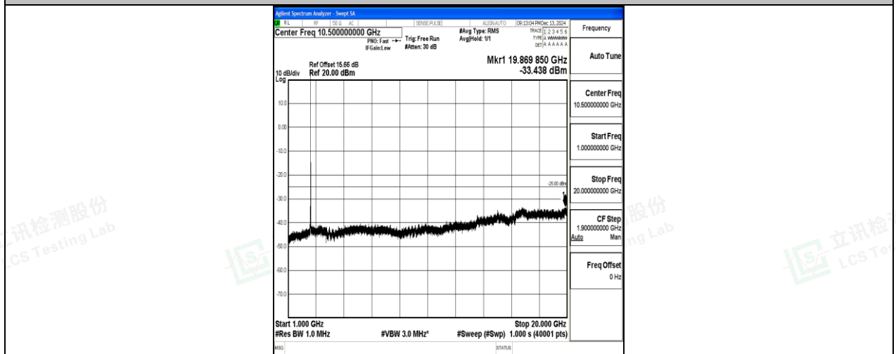
Band7_20MHz_16QAM_21100_1RB#0_1000~20000_1000~20000
