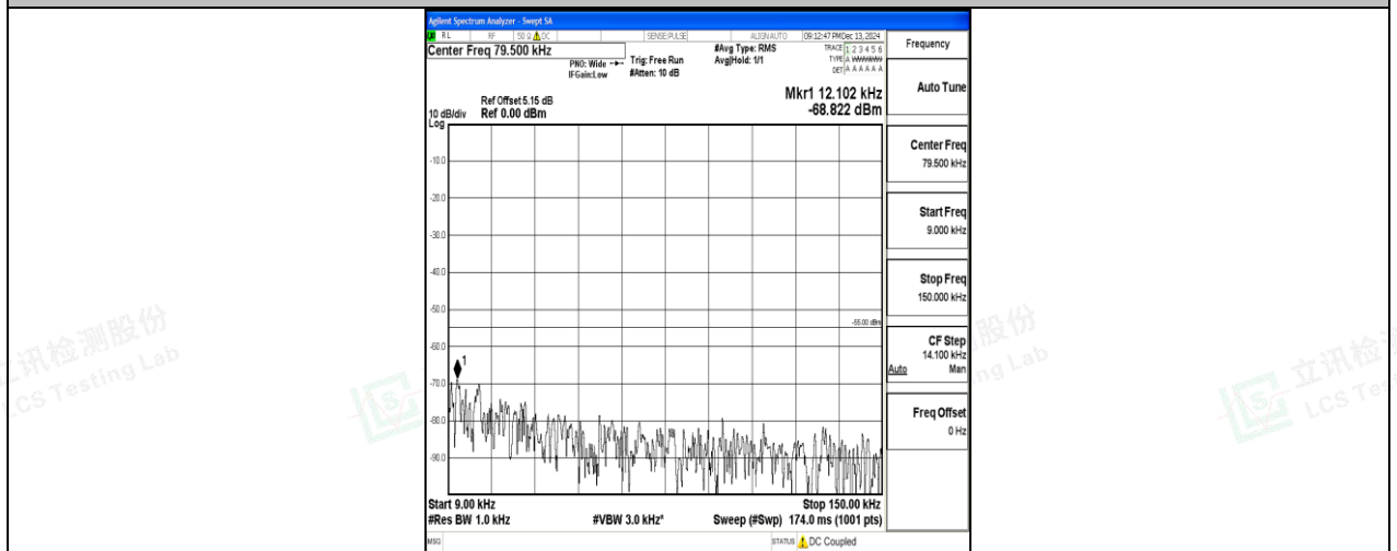
Band7_20MHz_16QAM_21100_1RB#0_0.009~0.15_0.009~0.15
