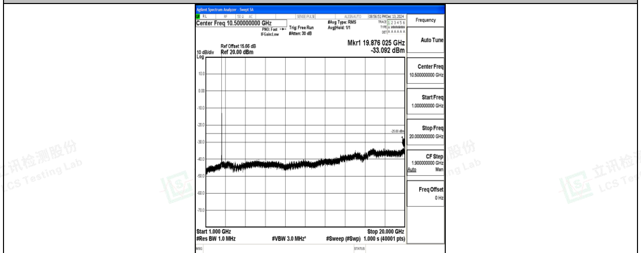
Band7_15MHz_16QAM_21100_1RB#0_1000~20000_1000~20000
