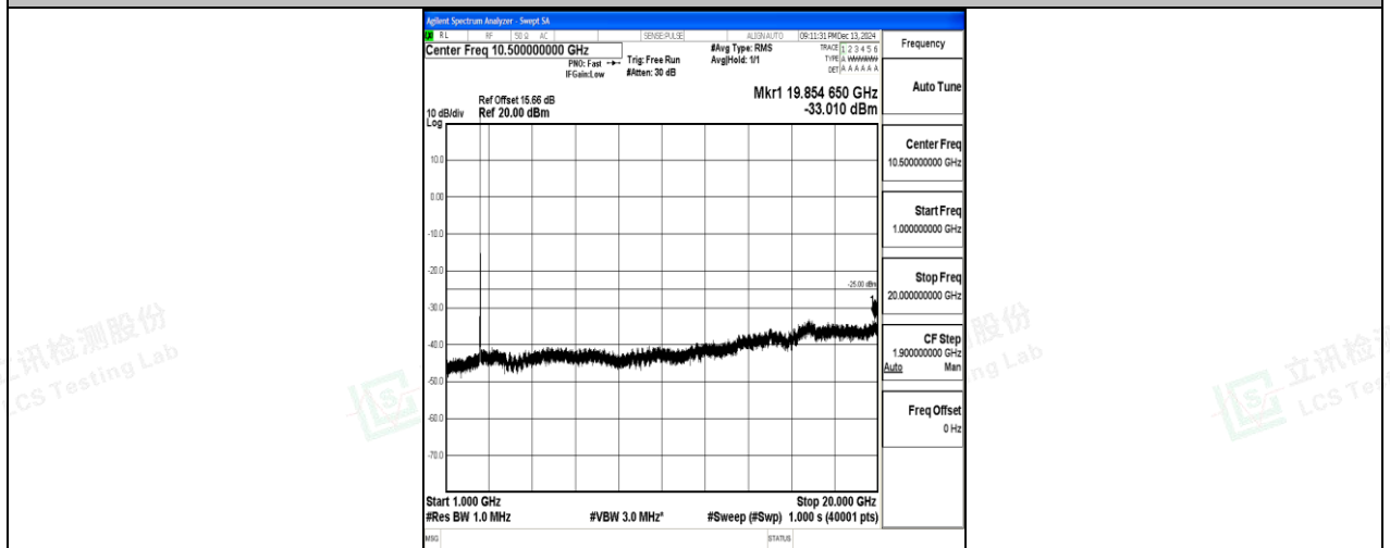
Band7_20MHz_QPSK_20850_1RB#0_1000~20000_1000~20000
