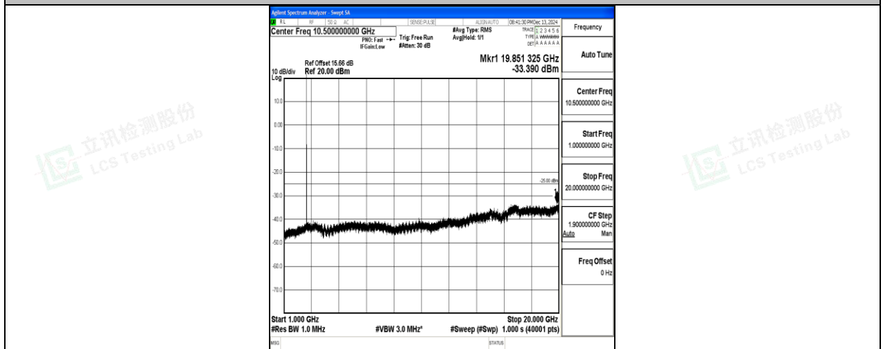
Band7_10MHz_16QAM_21400_1RB#0_1000~20000_1000~20000
