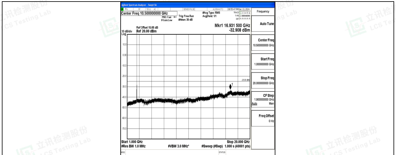
Band7_15MHz_16QAM_20825_1RB#0_1000~20000_1000~20000
