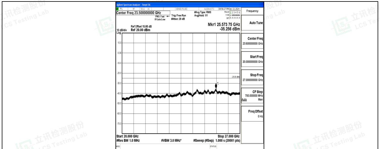
Band7_15MHz_QPSK_21100_1RB#0_20000~27000_20000~27000
