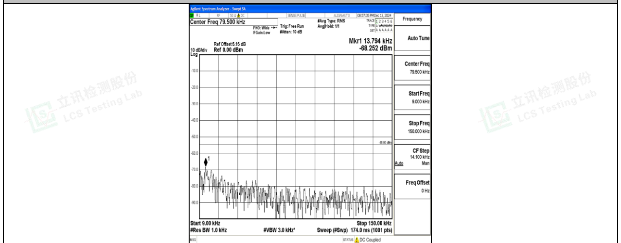
Band7_15MHz_16QAM_21375_1RB#0_0.009~0.15_0.009~0.15
