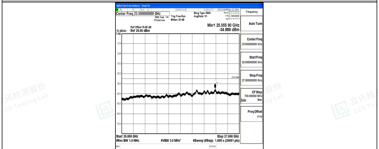
Band7_20MHz_16QAM_20850_1RB#0_20000~27000_20000~27000
