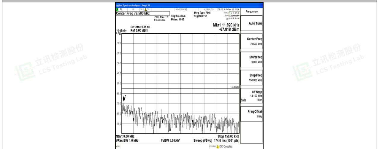
Band7_20MHz_QPSK_21100_1RB#0_0.009~0.15_0.009~0.15
