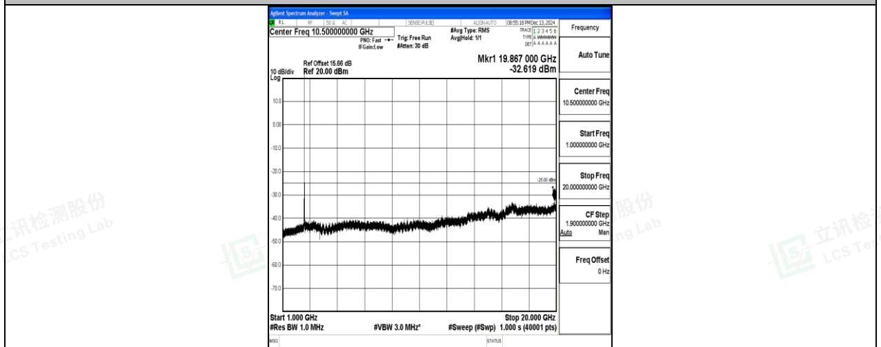
Band7_15MHz_QPSK_20825_1RB#0_1000~20000_1000~20000
