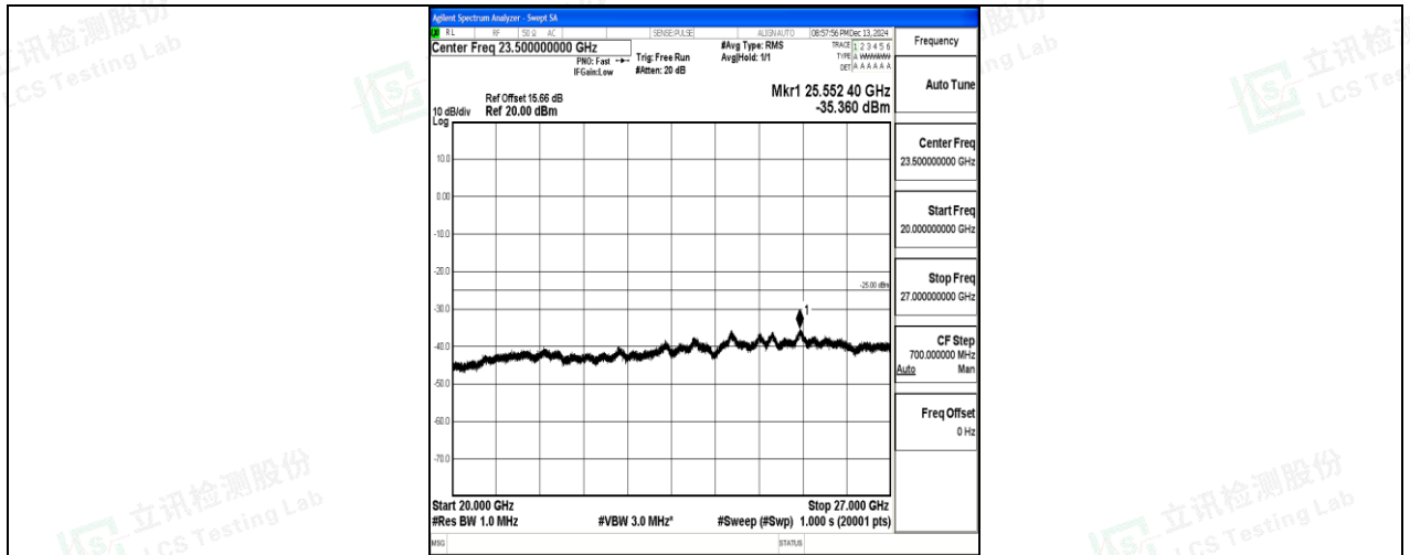
Band7_15MHz_16QAM_21375_1RB#0_20000~27000_20000~27000
