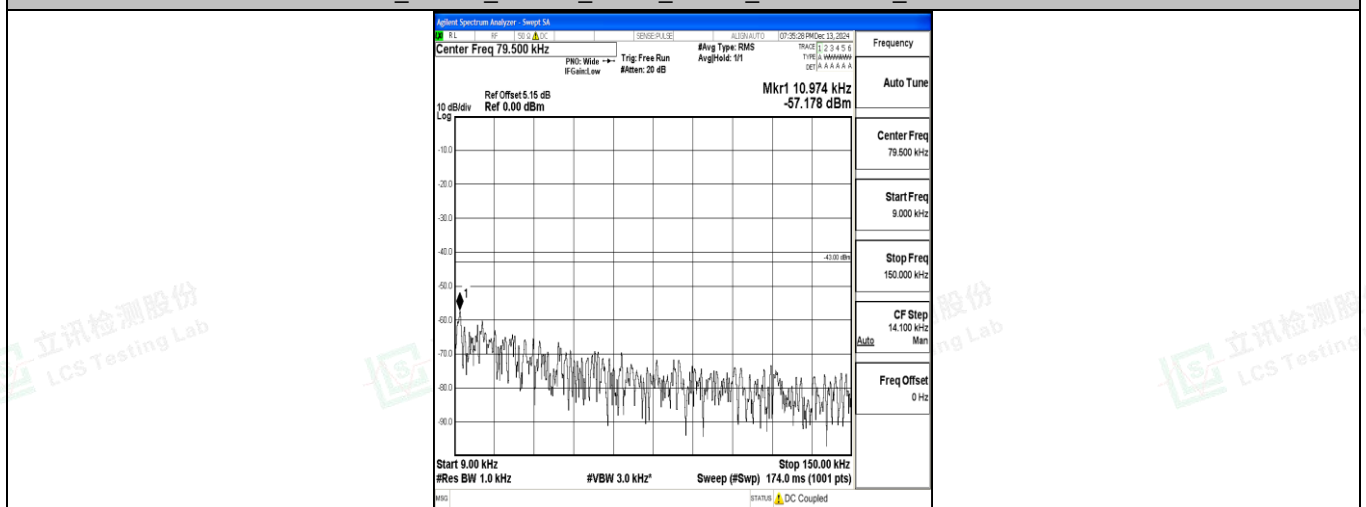
Band4_10MHz_QPSK_20350_1RB#0_0.009~0.15_0.009~0.15
