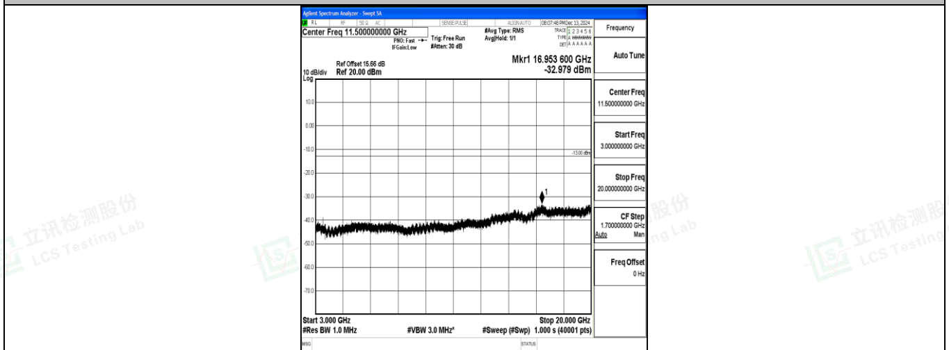
Band4_20MHz_16QAM_20300_1RB#0_3000~20000_3000~20000
