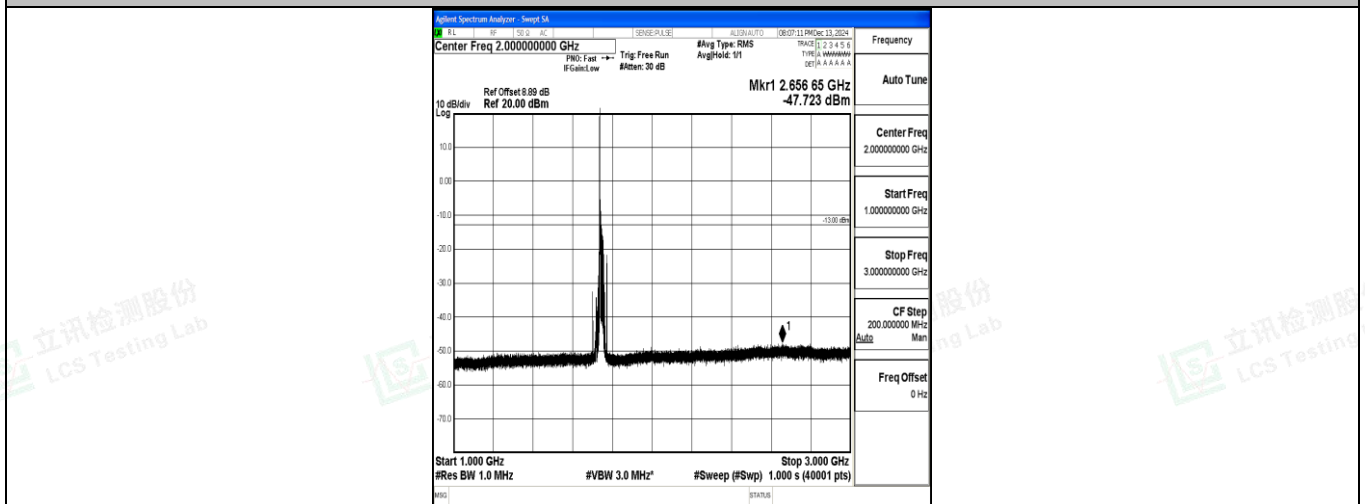
Band4_20MHz_QPSK_20300_1RB#0_1000~3000_1000~3000
