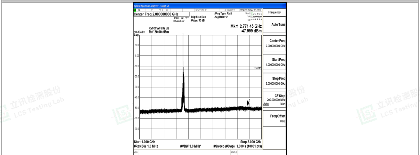
Band4_15MHz_16QAM_20025_1RB#0_1000~3000_1000~3000
