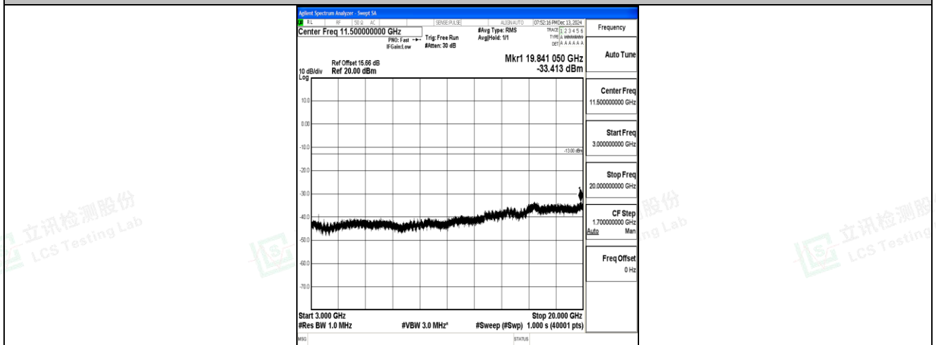
Band4_15MHz_16QAM_20325_1RB#0_3000~20000_3000~20000
