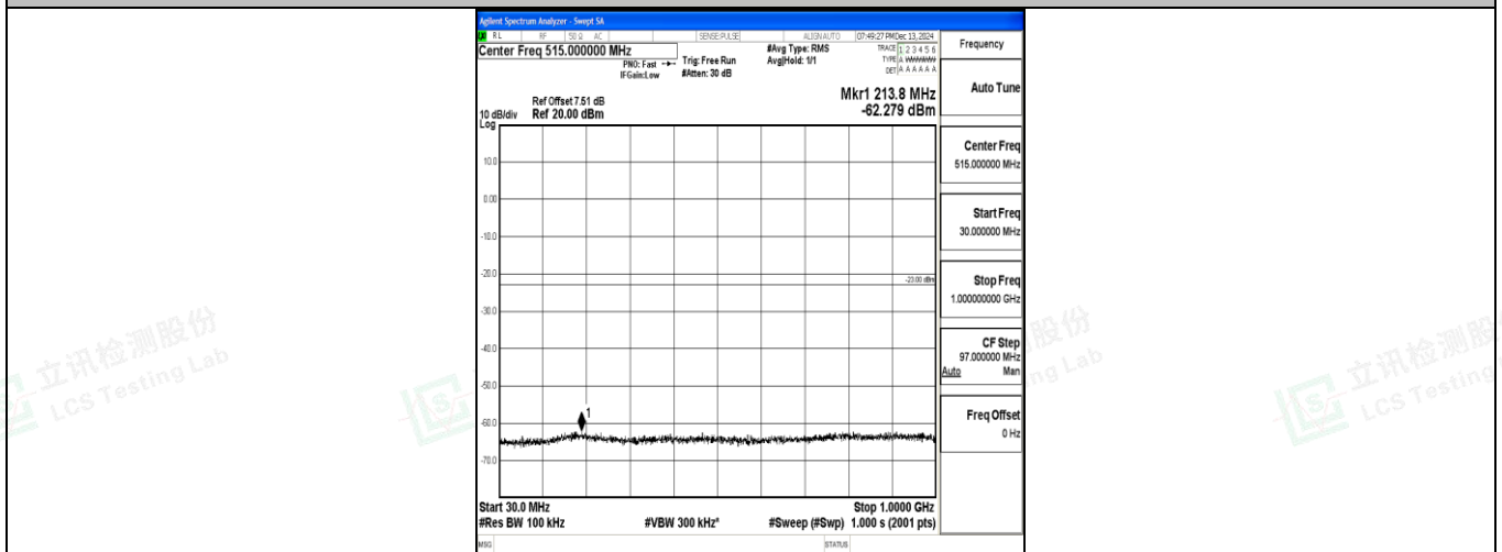
Band4_15MHz_QPSK_20025_1RB#0_30~1000_30~1000
