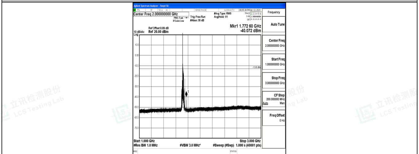
Band4_20MHz_16QAM_20050_1RB#0_1000~3000_1000~3000
