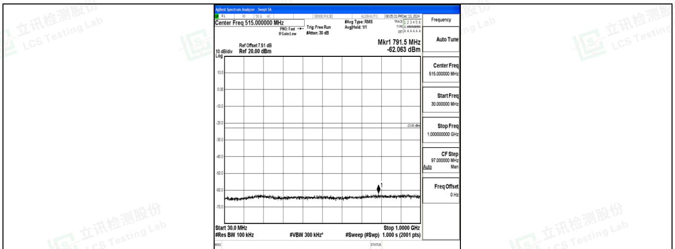
Band4_20MHz_16QAM_20050_1RB#0_30~1000_30~1000
