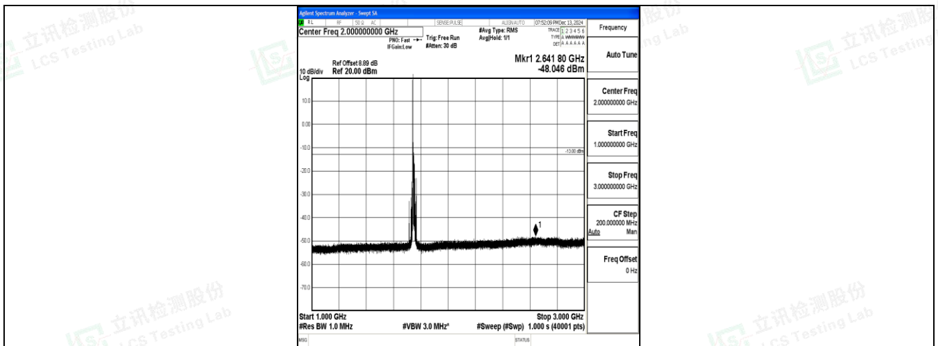
Band4_15MHz_16QAM_20325_1RB#0_1000~3000_1000~3000
