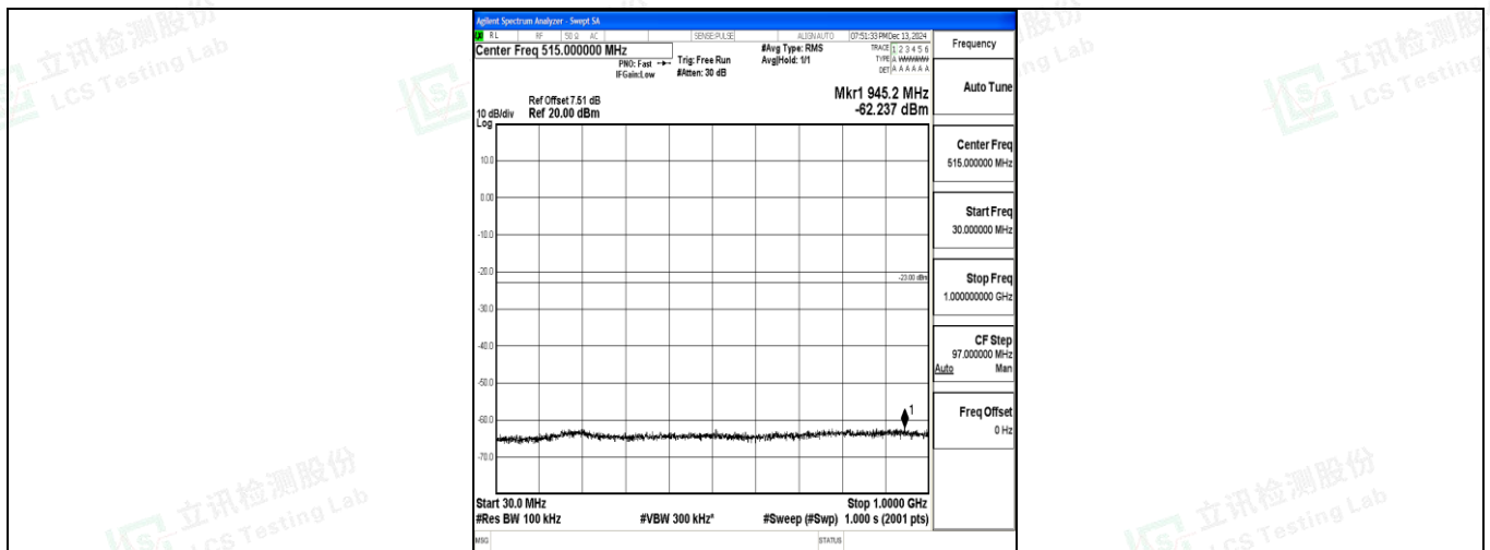
Band4_15MHz_QPSK_20325_1RB#0_30~1000_30~1000
