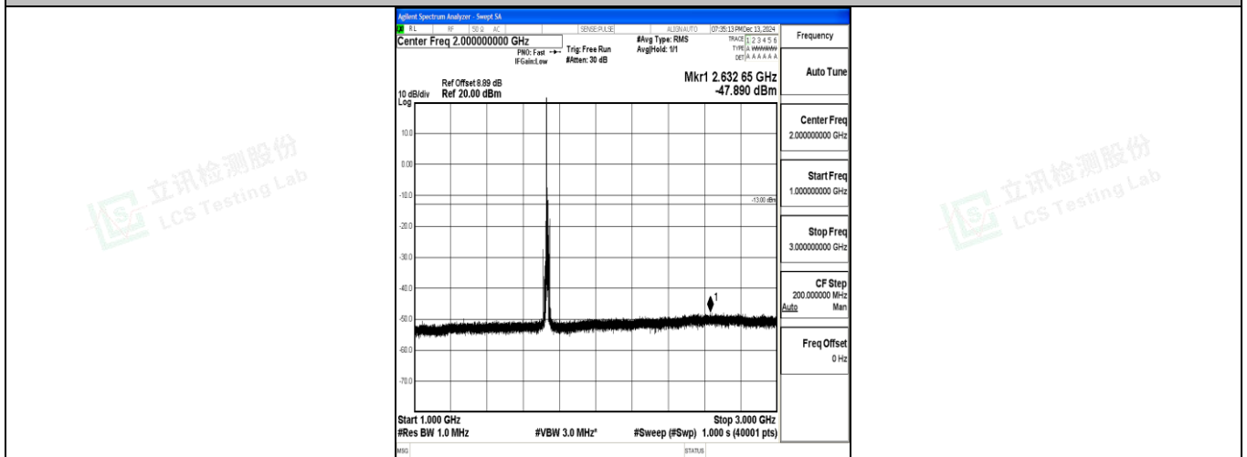
Band4_10MHz_16QAM_20175_1RB#0_1000~3000_1000~3000
