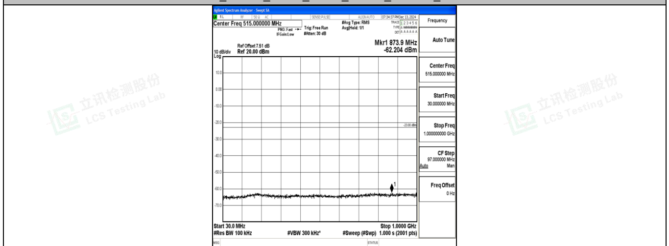
Band4_10MHz_QPSK_20175_1RB#0_30~1000_30~1000
