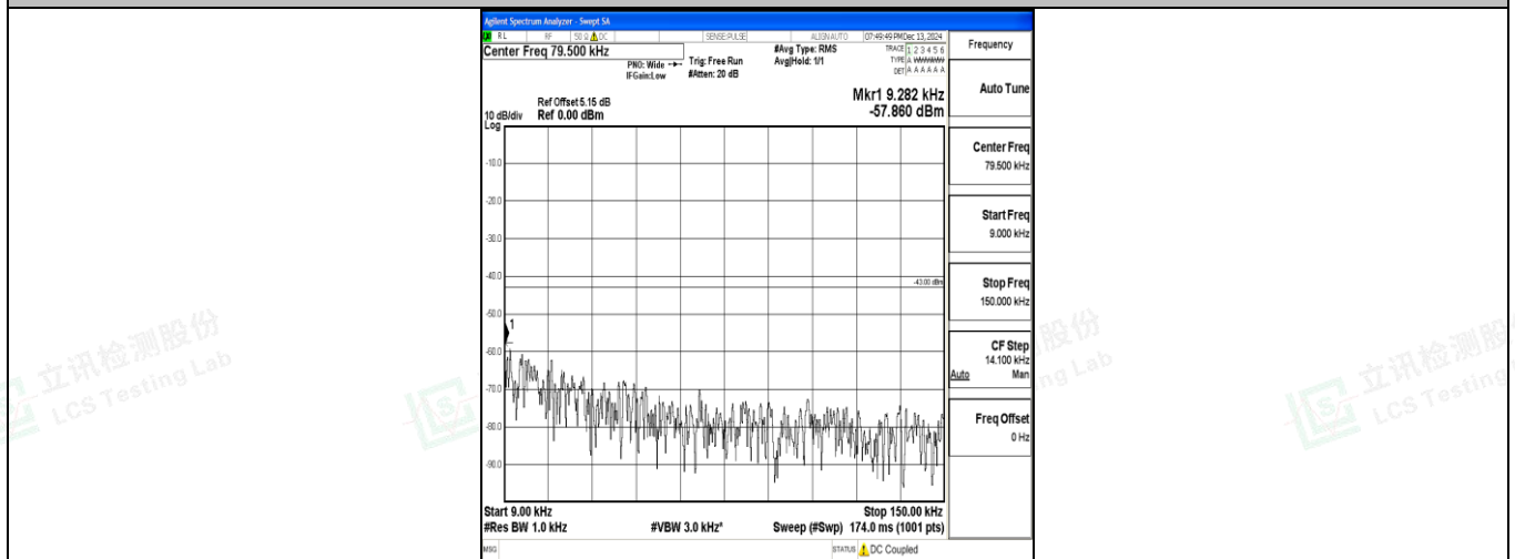
Band4_15MHz_16QAM_20025_1RB#0_0.009~0.15_0.009~0.15
