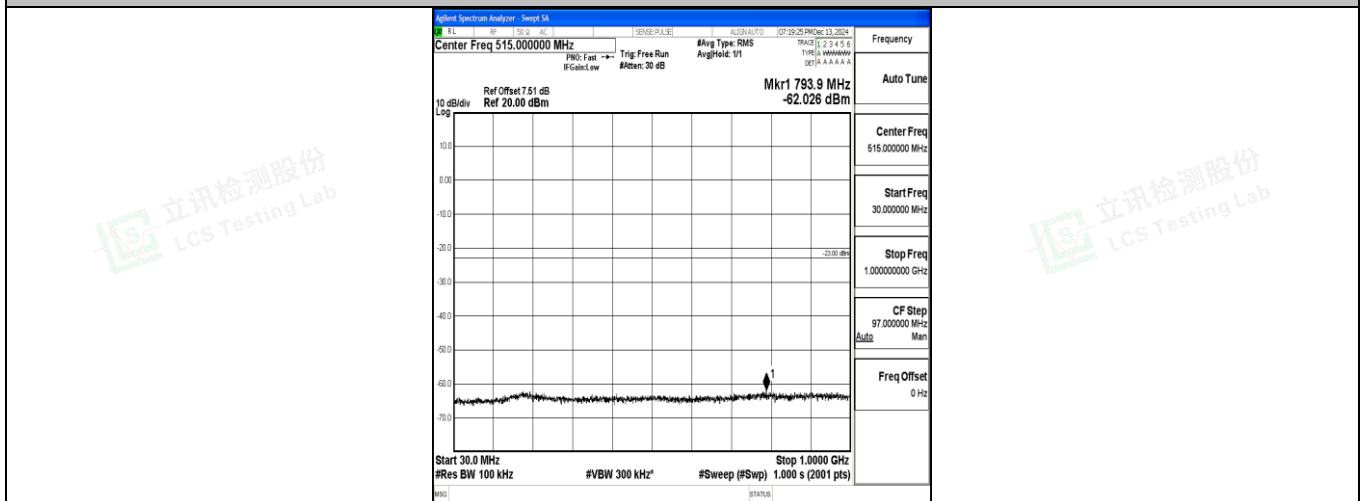
Band4_5MHz_16QAM_20375_1RB#0_30~1000_30~1000
