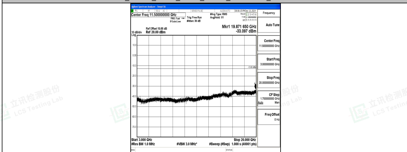
Band4_20MHz_QPSK_20175_1RB#0_3000~20000_3000~20000
