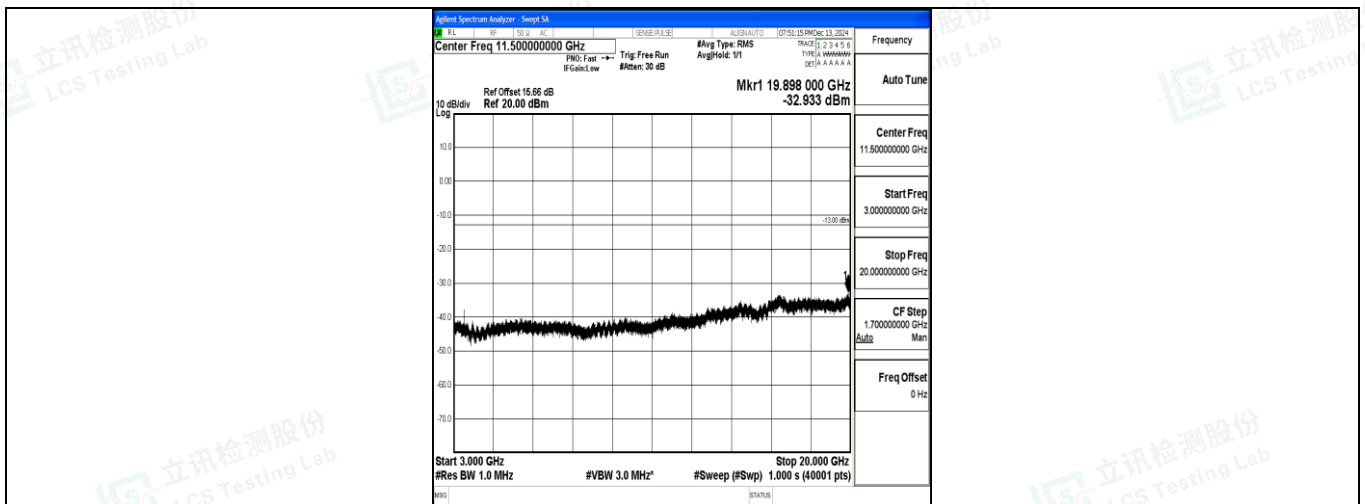
Band4_15MHz_16QAM_20175_1RB#0_3000~20000_3000~20000
