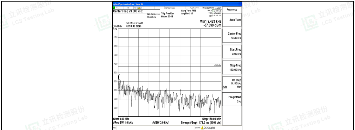
Band4_20MHz_QPSK_20175_1RB#0_0.009~0.15_0.009~0.15
