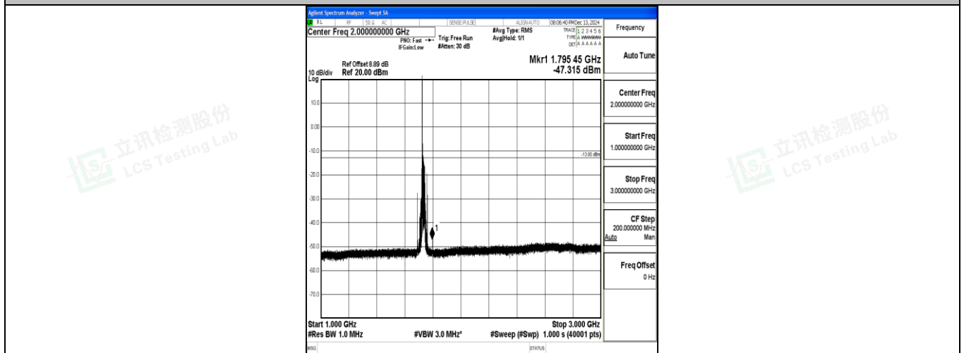
Band4_20MHz_16QAM_20175_1RB#0_1000~3000_1000~3000
