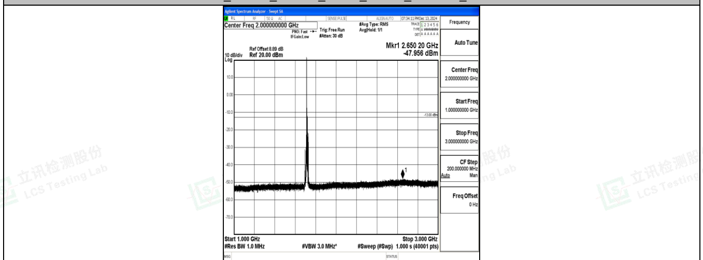
Band4_10MHz_16QAM_20000_1RB#0_1000~3000_1000~3000
