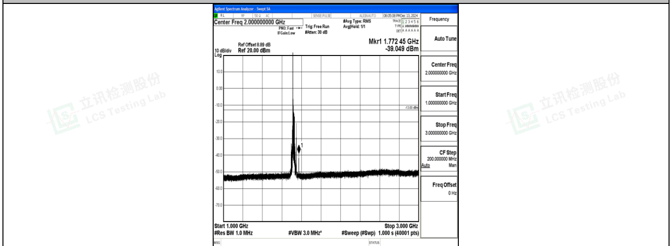
Band4_20MHz_QPSK_20050_1RB#0_1000~3000_1000~3000
