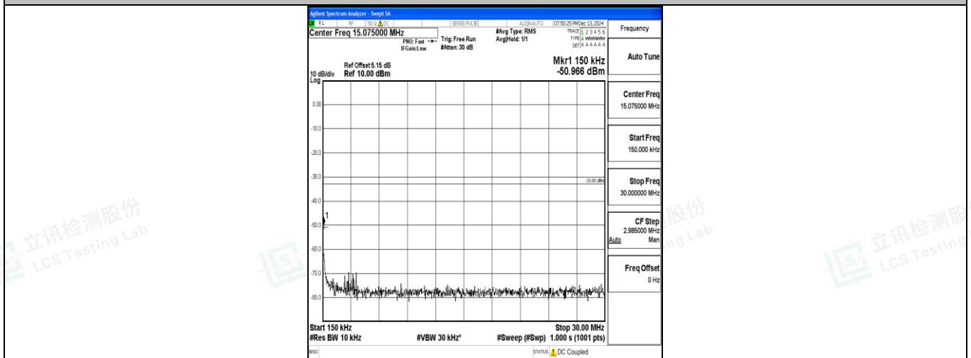
Band4_15MHz_QPSK_20175_1RB#0_0.15~30_0.15~30
