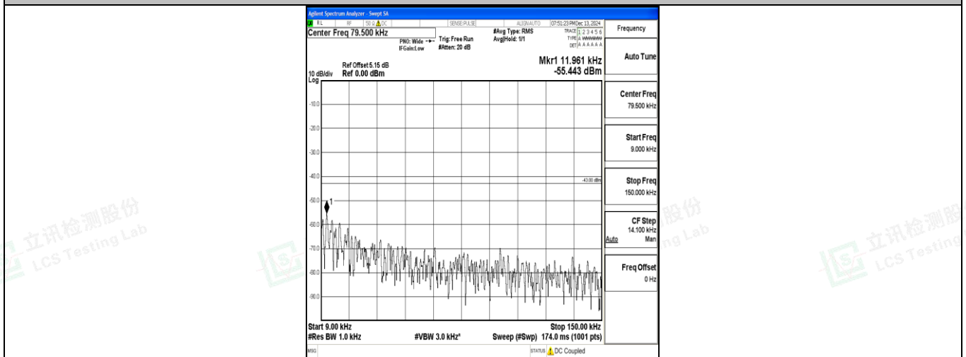
Band4_15MHz_QPSK_20325_1RB#0_0.009~0.15_0.009~0.15
