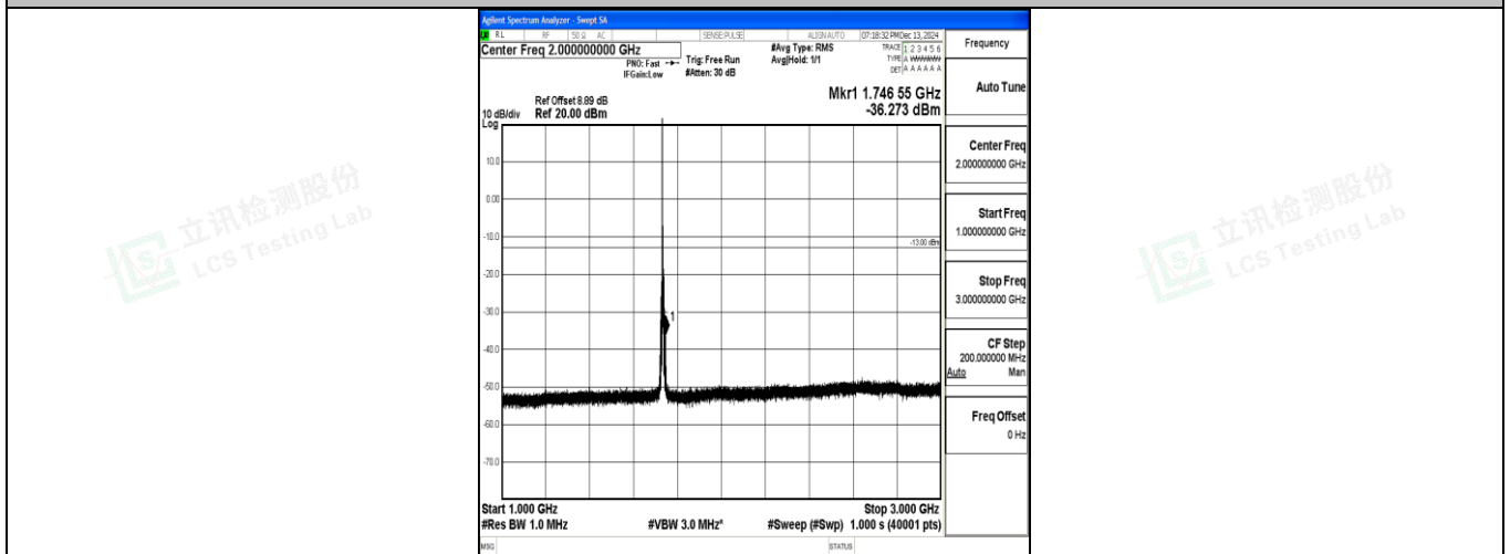
Band4_5MHz_16QAM_20175_1RB#0_1000~3000_1000~3000
