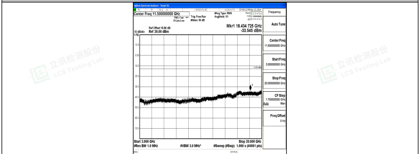
Band4_15MHz_16QAM_20025_1RB#0_3000~20000_3000~20000
