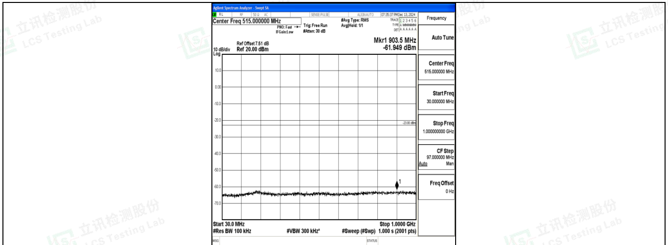
Band4_10MHz_QPSK_20350_1RB#0_30~1000_30~1000
