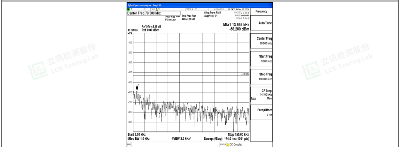
Band4_20MHz_QPSK_20050_1RB#0_0.009~0.15_0.009~0.15
