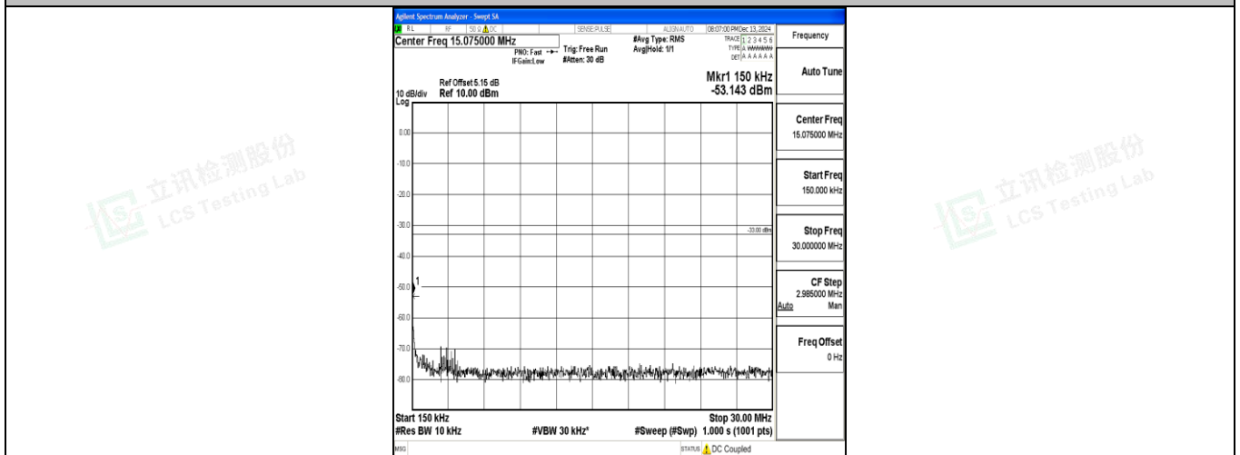
Band4_20MHz_QPSK_20300_1RB#0_0.15~30_0.15~30
