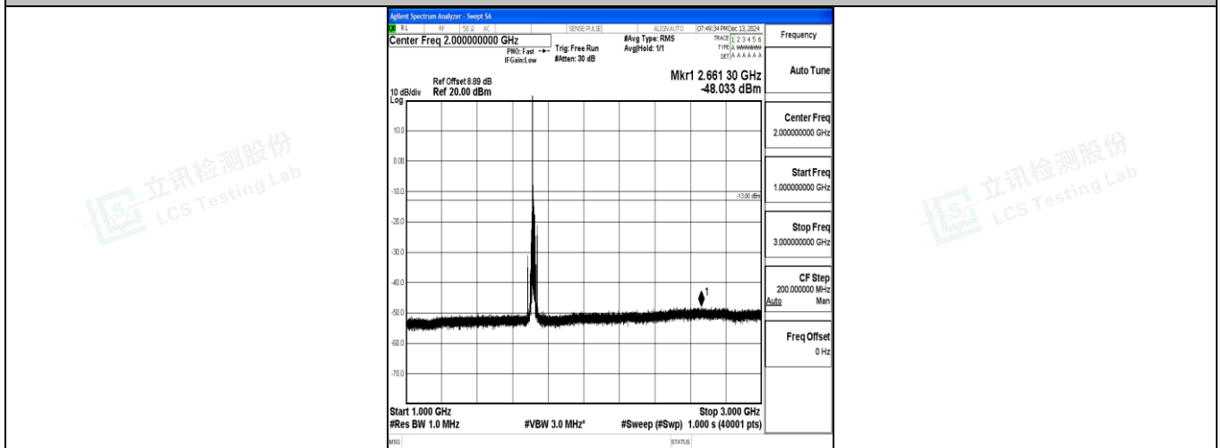
Band4_15MHz_QPSK_20025_1RB#0_1000~3000_1000~3000
