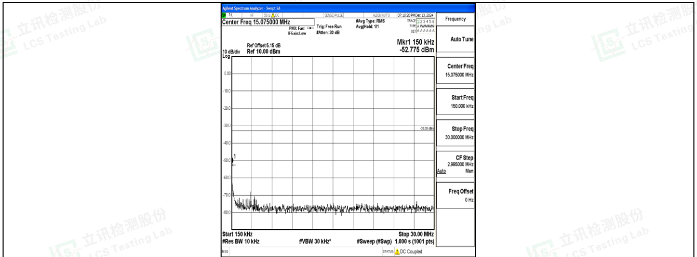
Band4_5MHz_16QAM_20175_1RB#0_0.15~30_0.15~30
