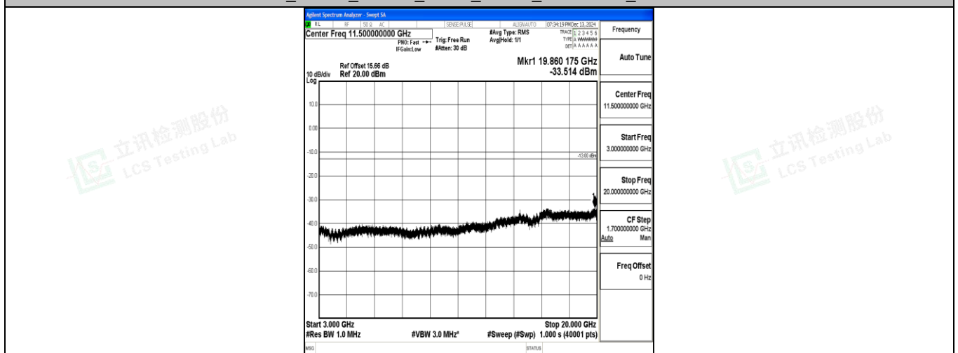
Band4_10MHz_16QAM_20000_1RB#0_3000~20000_3000~20000
