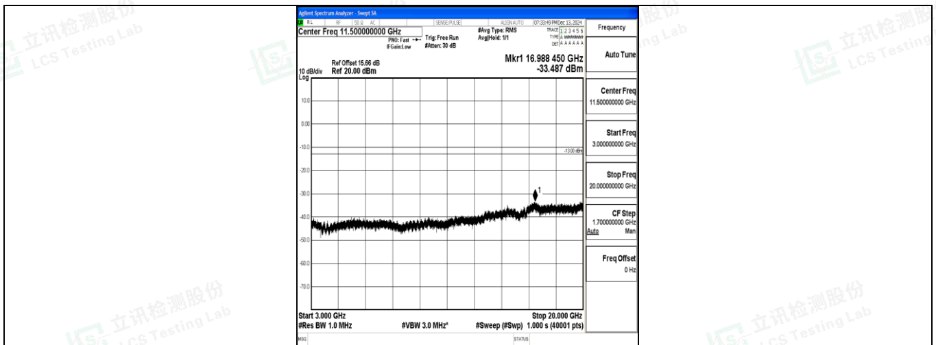
Band4_10MHz_QPSK_20000_1RB#0_3000~20000_3000~20000
