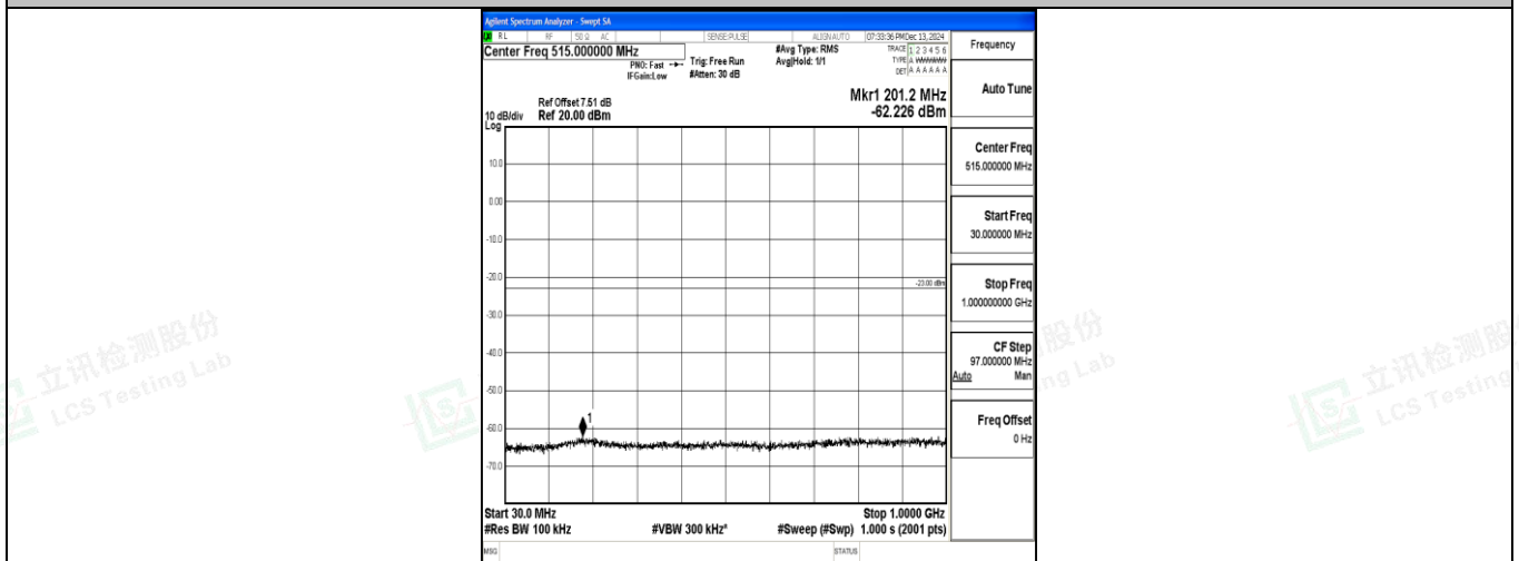
Band4_10MHz_QPSK_20000_1RB#0_30~1000_30~1000
