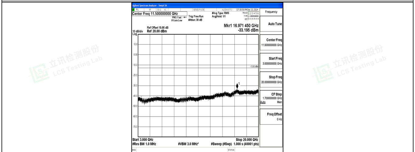
Band4_10MHz_QPSK_20350_1RB#0_3000~20000_3000~20000
