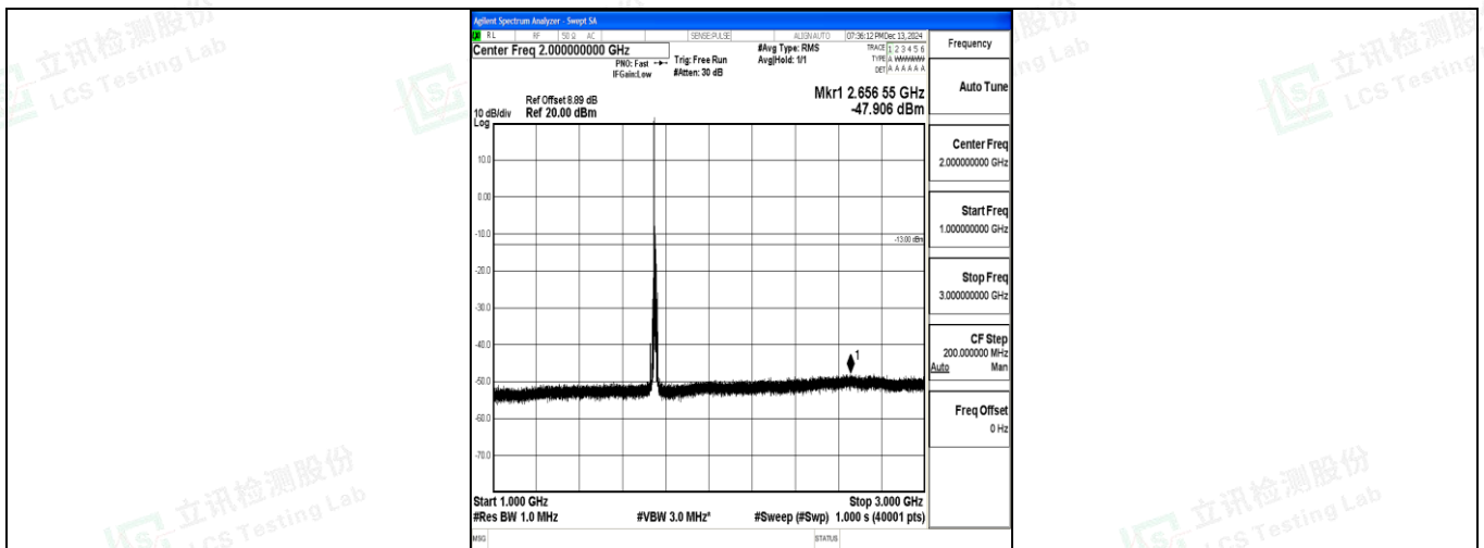
Band4_10MHz_16QAM_20350_1RB#0_1000~3000_1000~3000
