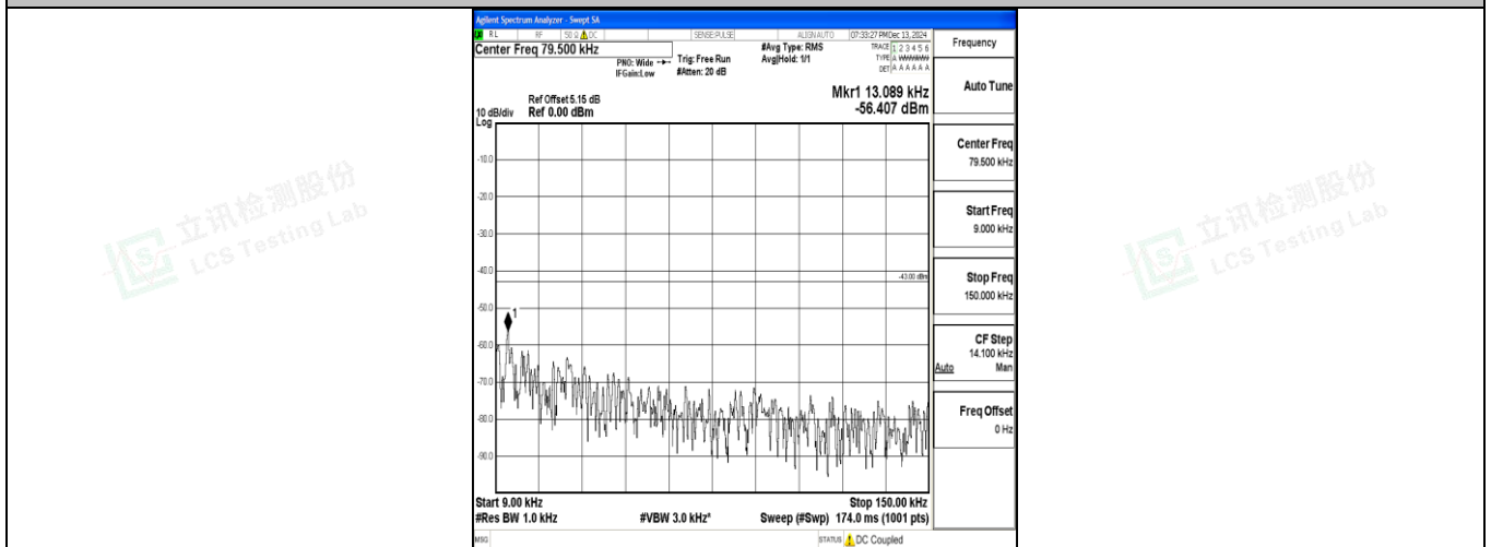
Band4_10MHz_QPSK_20000_1RB#0_0.009~0.15_0.009~0.15
