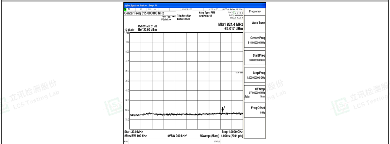
Band4_20MHz_QPSK_20050_1RB#0_30~1000_30~1000
