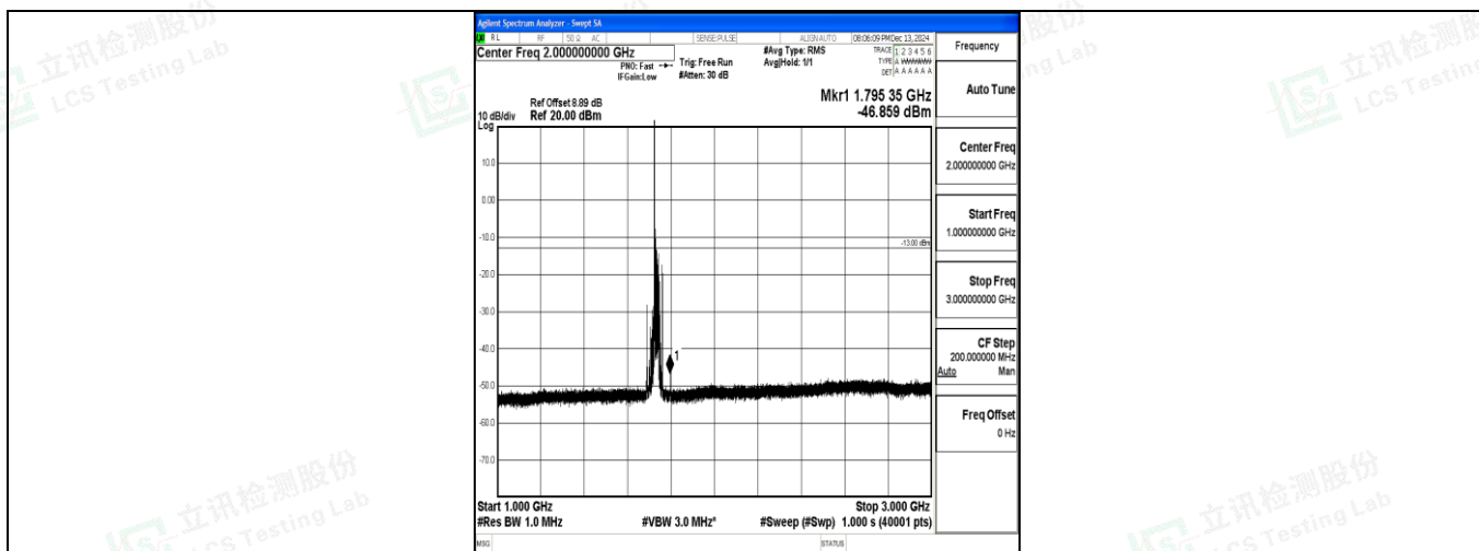
Band4_20MHz_QPSK_20175_1RB#0_1000~3000_1000~3000
