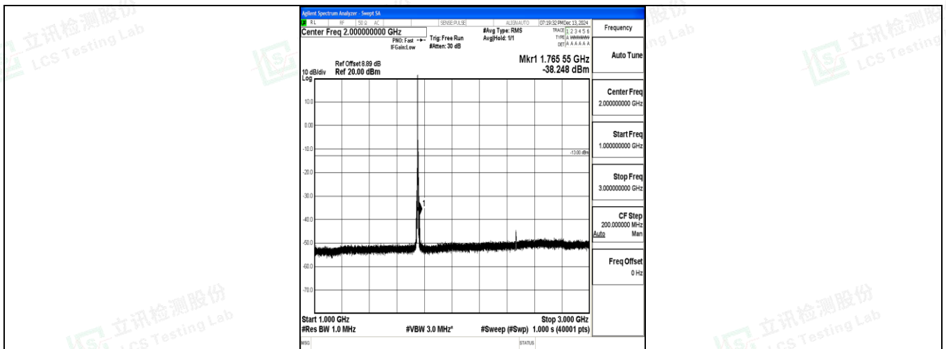
Band4_5MHz_16QAM_20375_1RB#0_1000~3000_1000~3000
