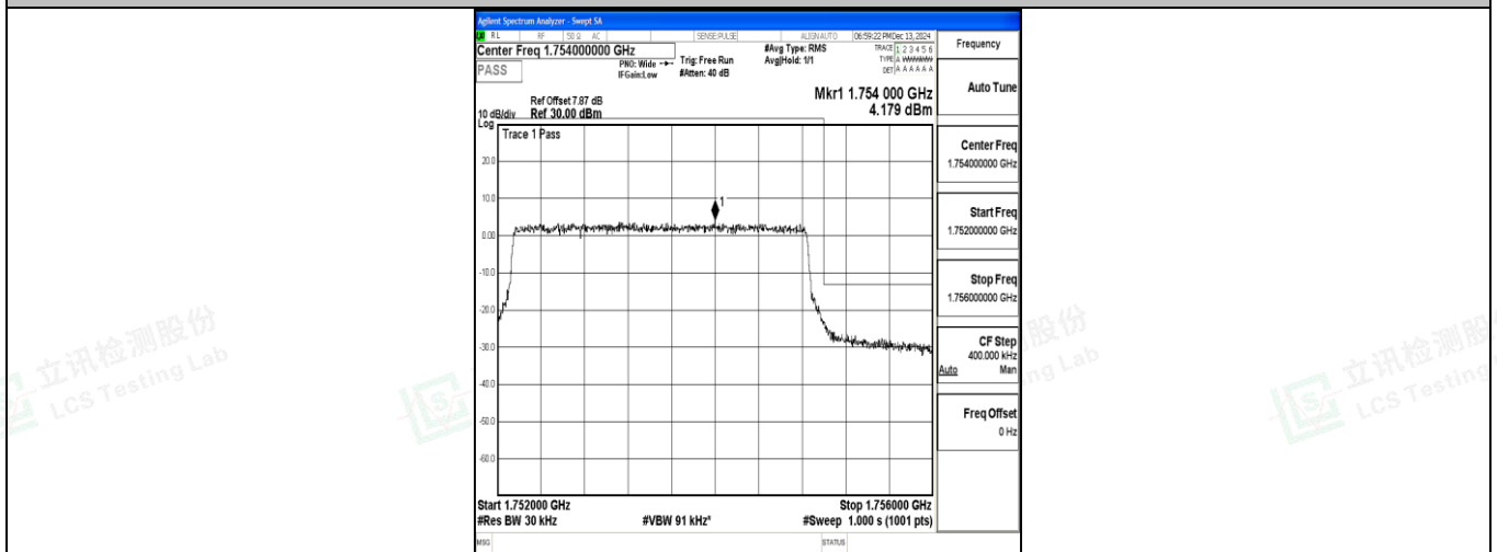
Band4_3MHz_16QAM_20385_15RB#0
