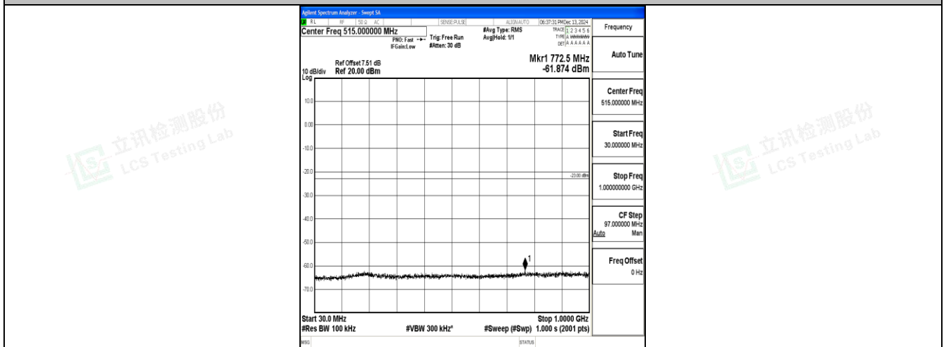
Band4_1.4MHz_QPSK_20175_1RB#0_30~1000_30~1000
