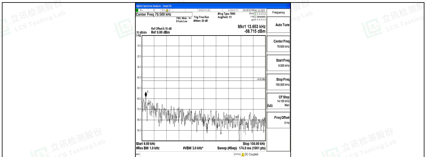
Band4_1.4MHz_16QAM_20393_1RB#0_0.009~0.15_0.009~0.15
