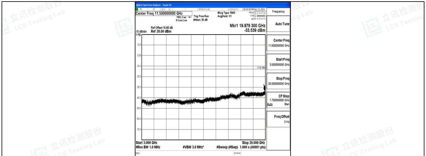
Band4_3MHz_QPSK_19965_1RB#0_3000~20000_3000~20000
