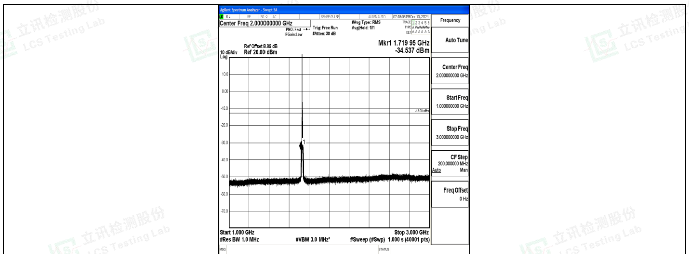
Band4_5MHz_QPSK_20175_1RB#0_1000~3000_1000~3000
