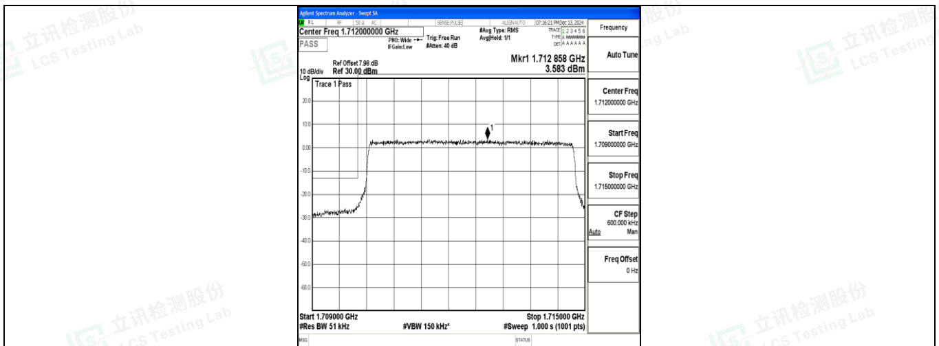
Band4_5MHz_16QAM_19975_25RB#0
