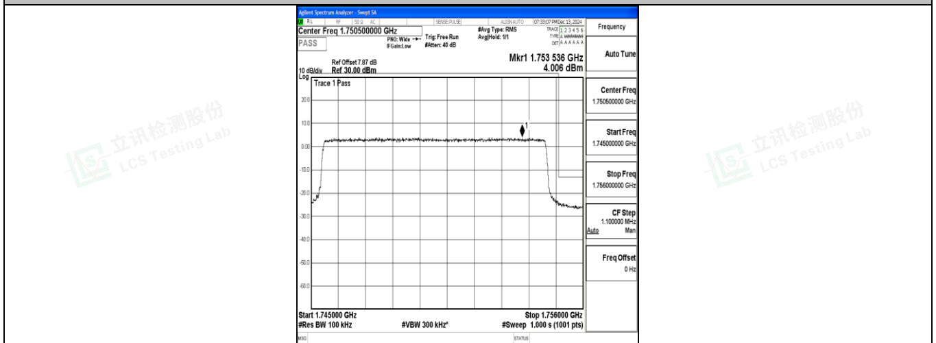
Band4_10MHz_QPSK_20350_50RB#0
