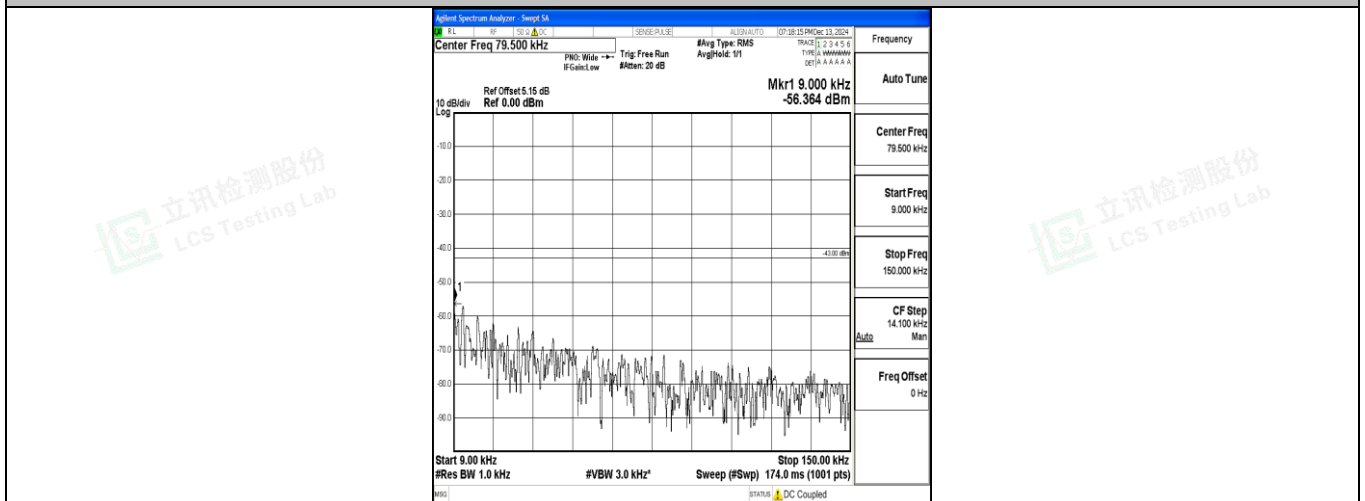
Band4_5MHz_16QAM_20175_1RB#0_0.009~0.15_0.009~0.15
