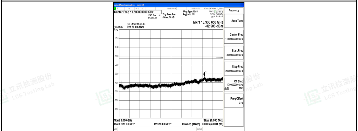
Band4_3MHz_QPSK_20175_1RB#0_3000~20000_3000~20000
