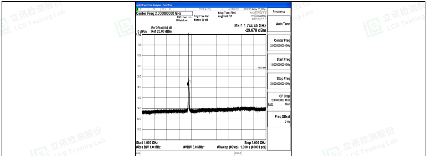
Band4_3MHz_16QAM_20385_1RB#0_1000~3000_1000~3000
