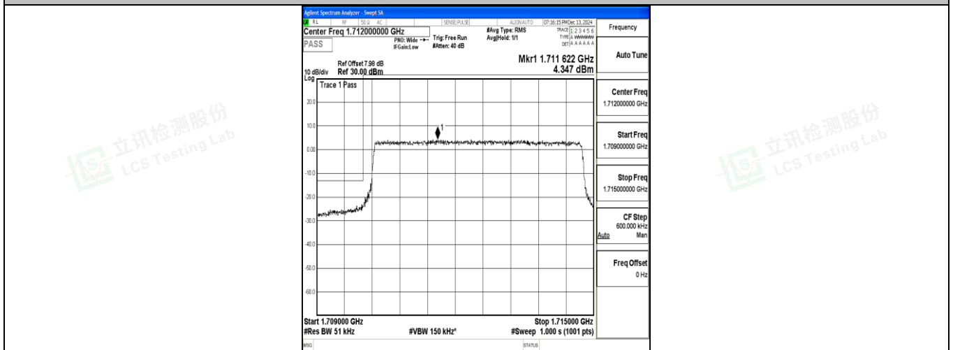
Band4_5MHz_QPSK_19975_25RB#0
