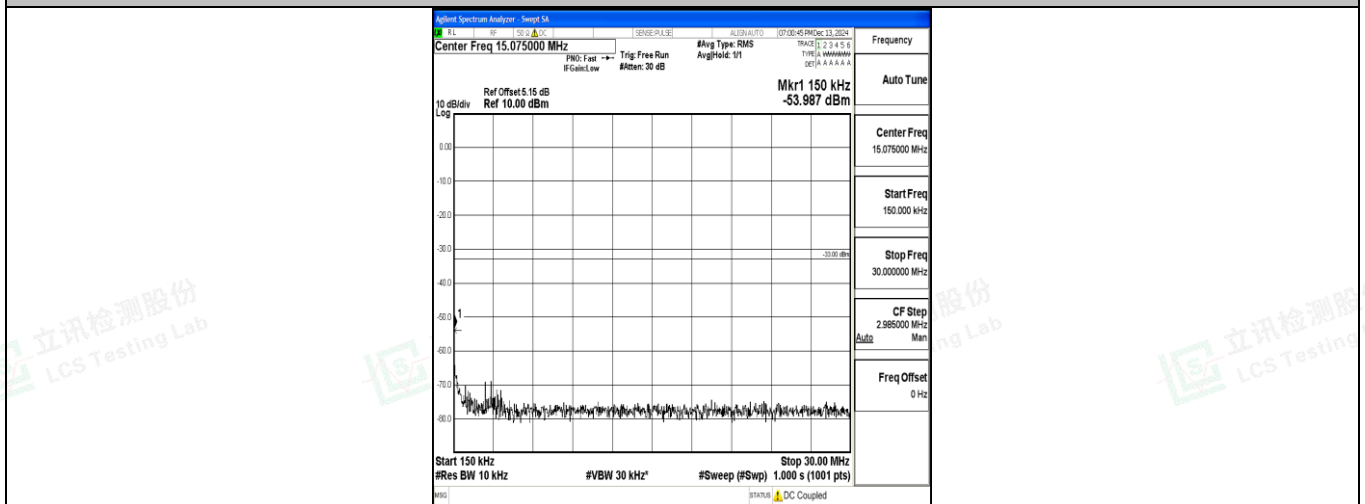
Band4_3MHz_QPSK_20175_1RB#0_0.15~30_0.15~30
