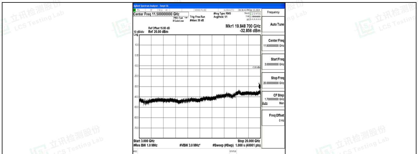
Band4_1.4MHz_QPSK_19957_1RB#0_3000~20000_3000~20000
