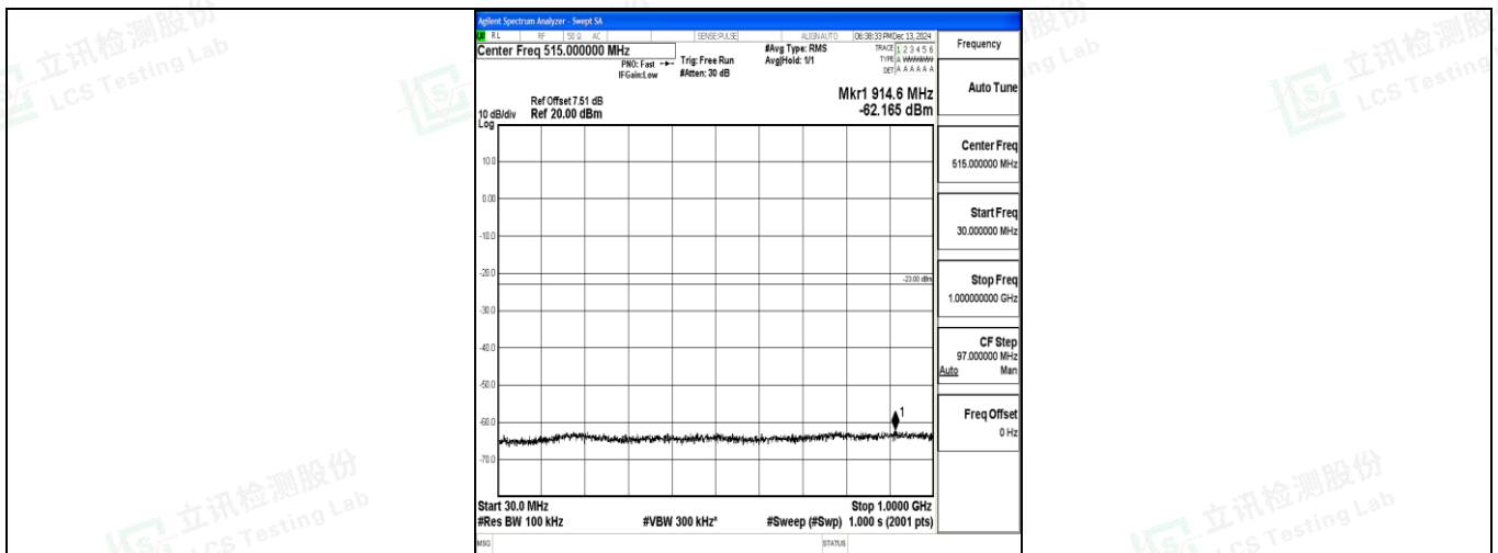
Band4_1.4MHz_QPSK_20393_1RB#0_30~1000_30~1000
