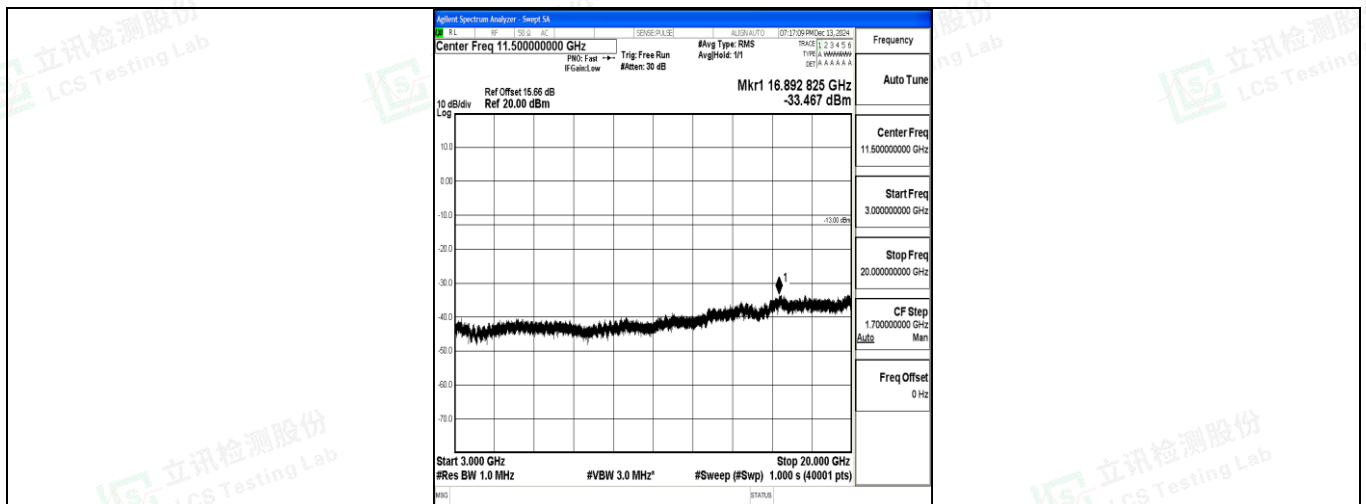
Band4_5MHz_QPSK_19975_1RB#0_3000~20000_3000~20000
