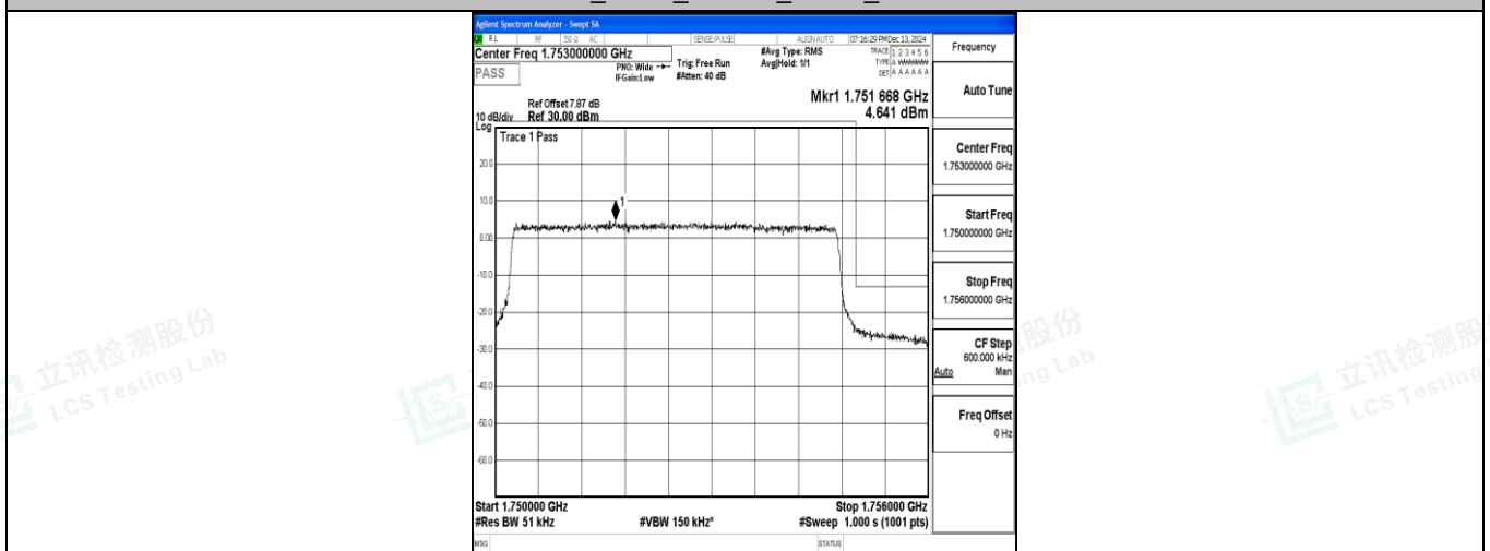
Band4_5MHz_QPSK_20375_25RB#0
