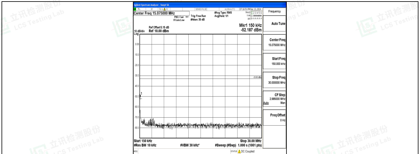
Band4_5MHz_QPSK_19975_1RB#0_0.15~30_0.15~30
