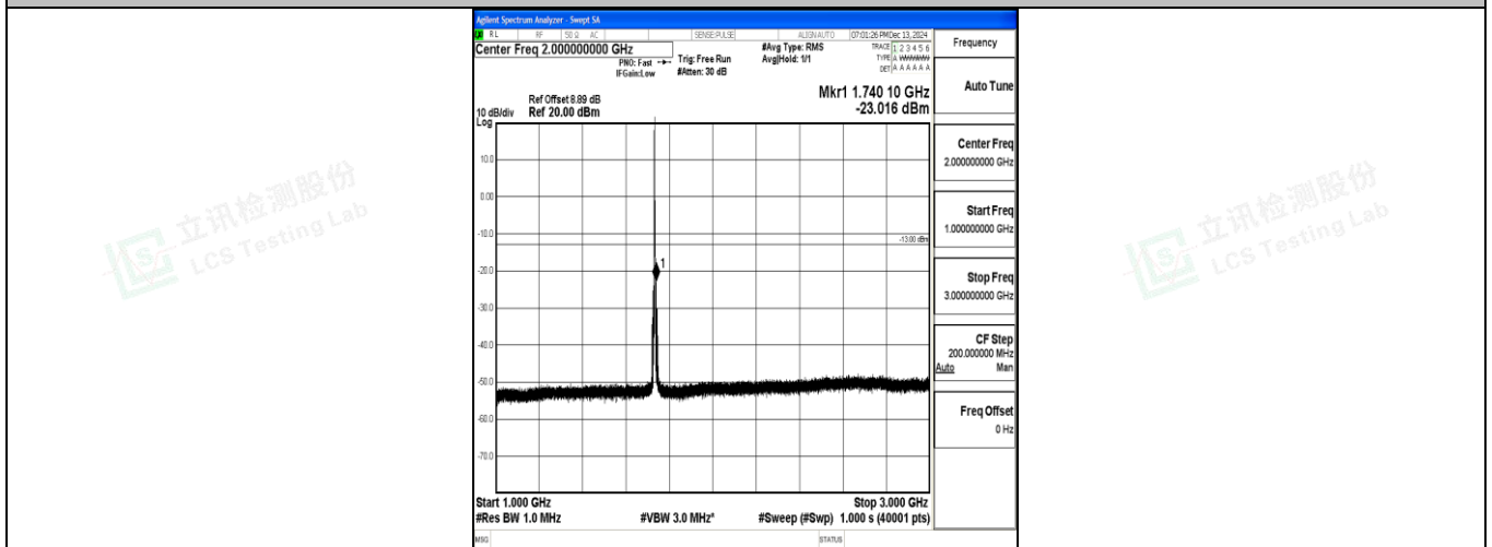
Band4_3MHz_16QAM_20175_1RB#0_1000~3000_1000~3000
