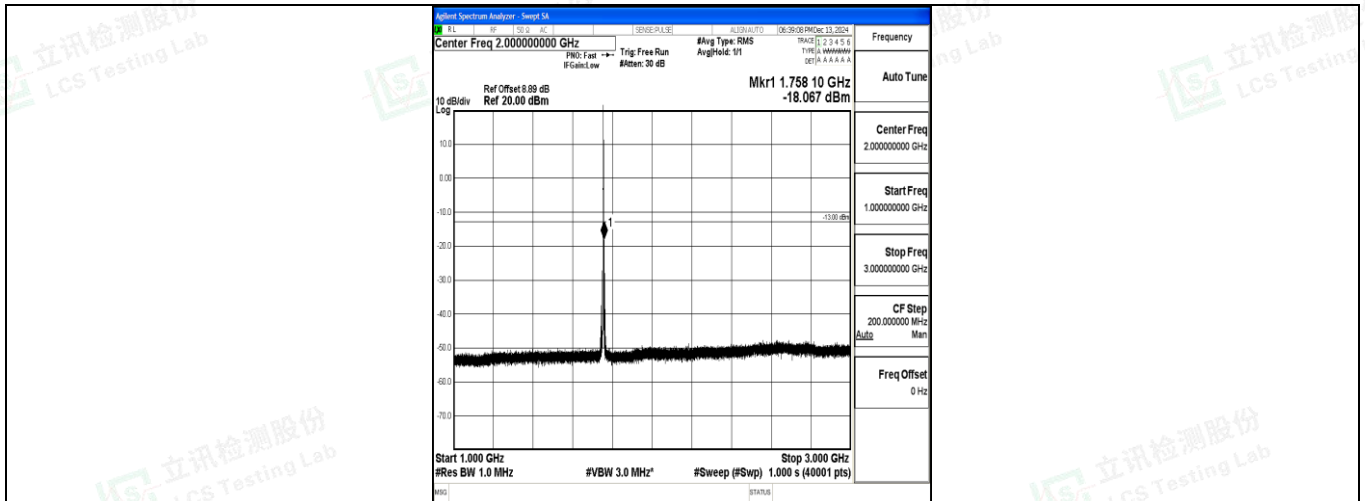
Band4_1.4MHz_16QAM_20393_1RB#0_1000~3000_1000~3000
