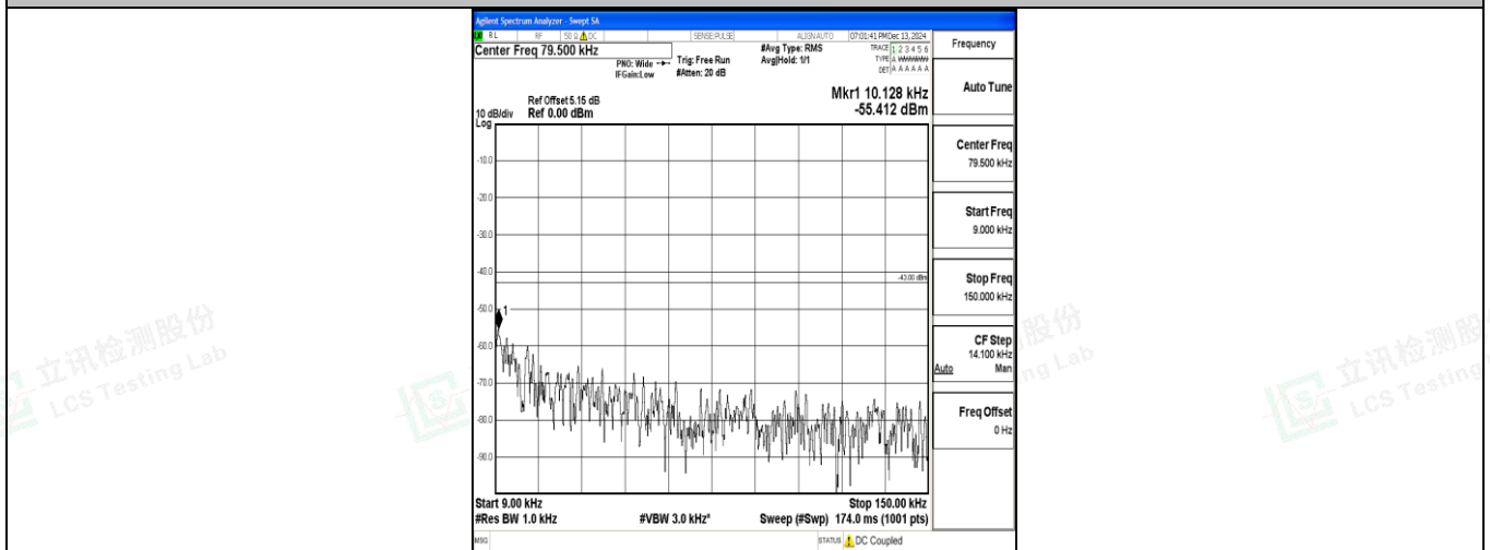
Band4_3MHz_QPSK_20385_1RB#0_0.009~0.15_0.009~0.15
