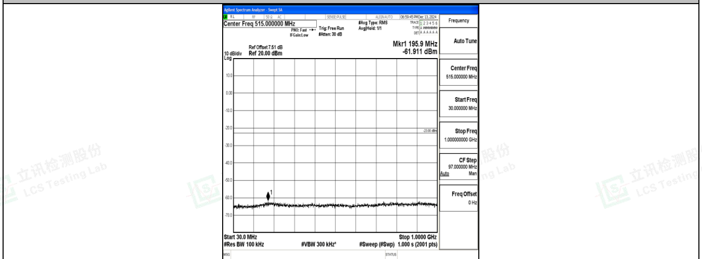
Band4_3MHz_QPSK_19965_1RB#0_30~1000_30~1000
