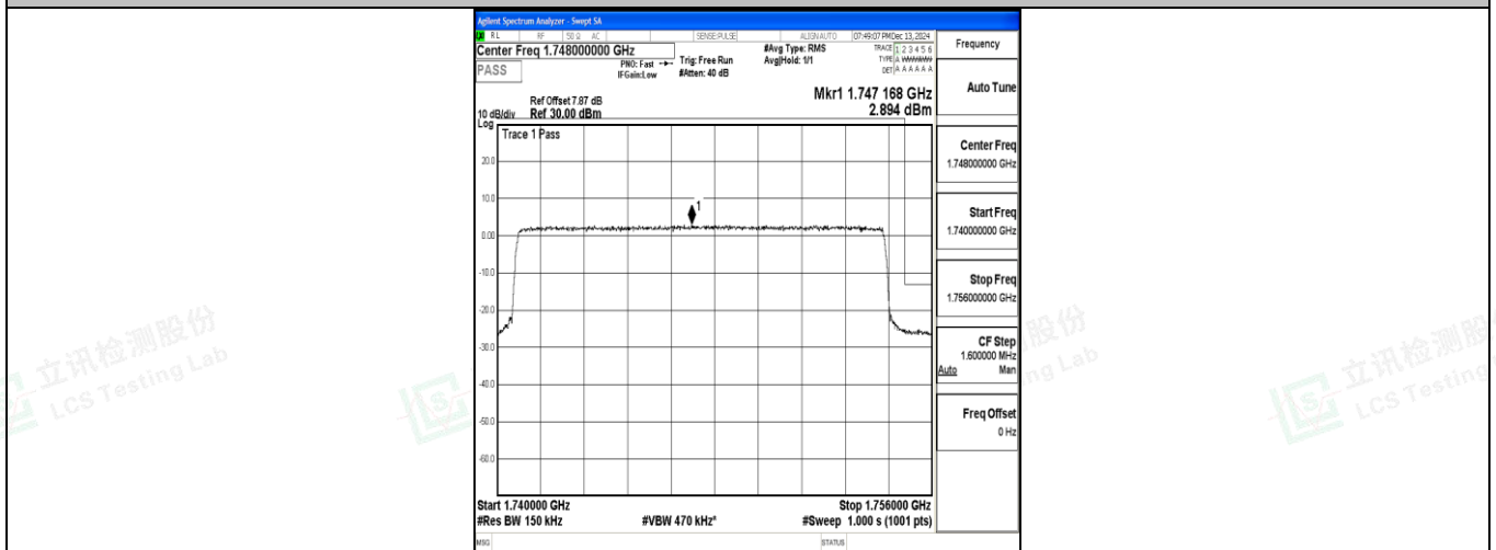
Band4_15MHz_16QAM_20325_75RB#0
