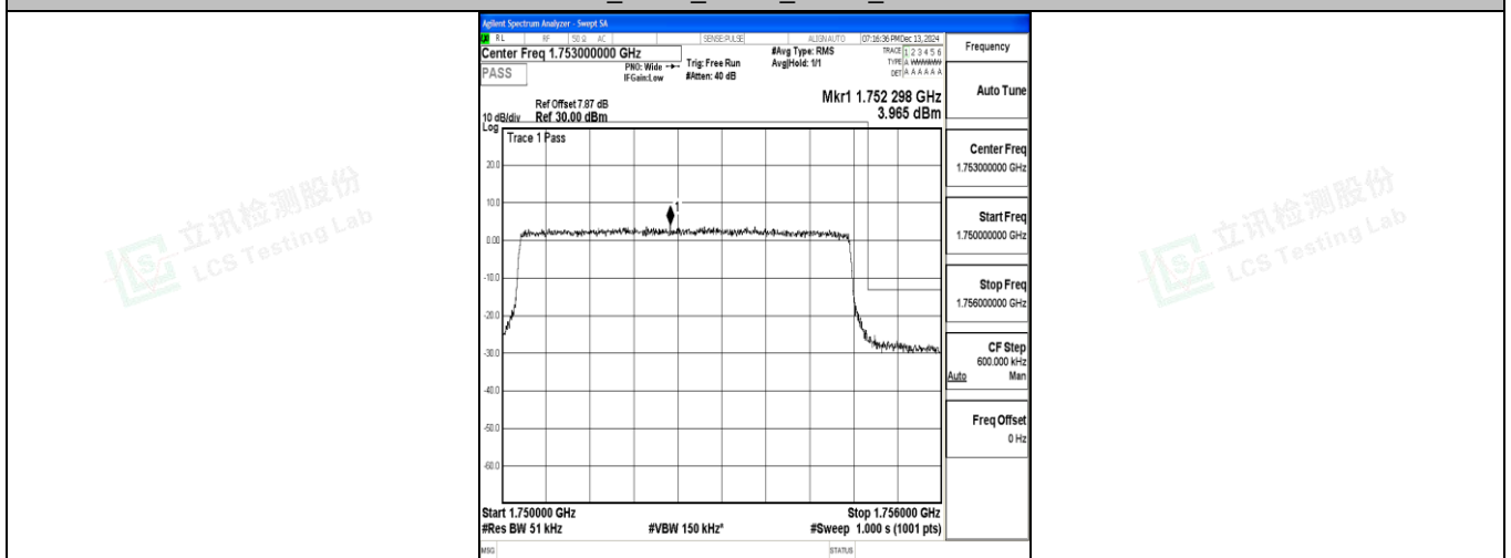
Band4_5MHz_16QAM_20375_25RB#0
