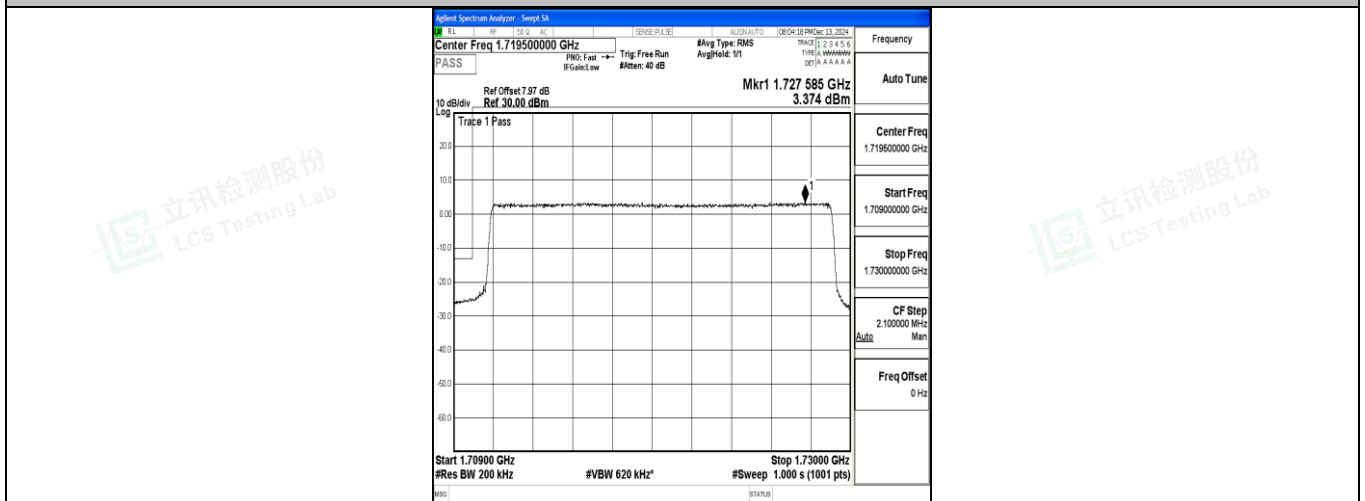
Band4_20MHz_QPSK_20050_100RB#0
