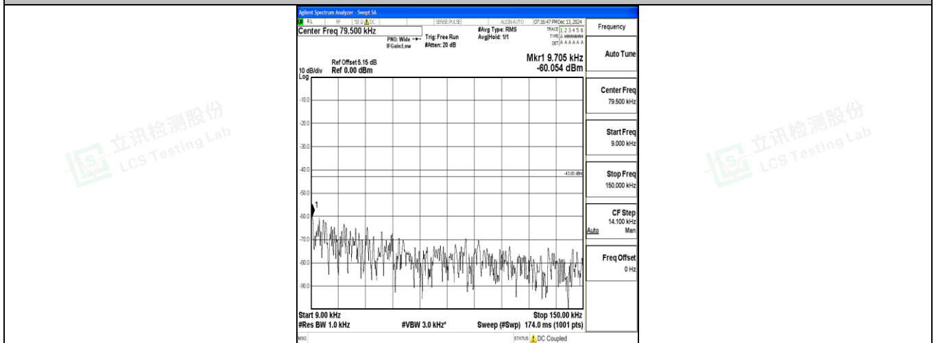
Band4_5MHz_QPSK_19975_1RB#0_0.009~0.15_0.009~0.15
