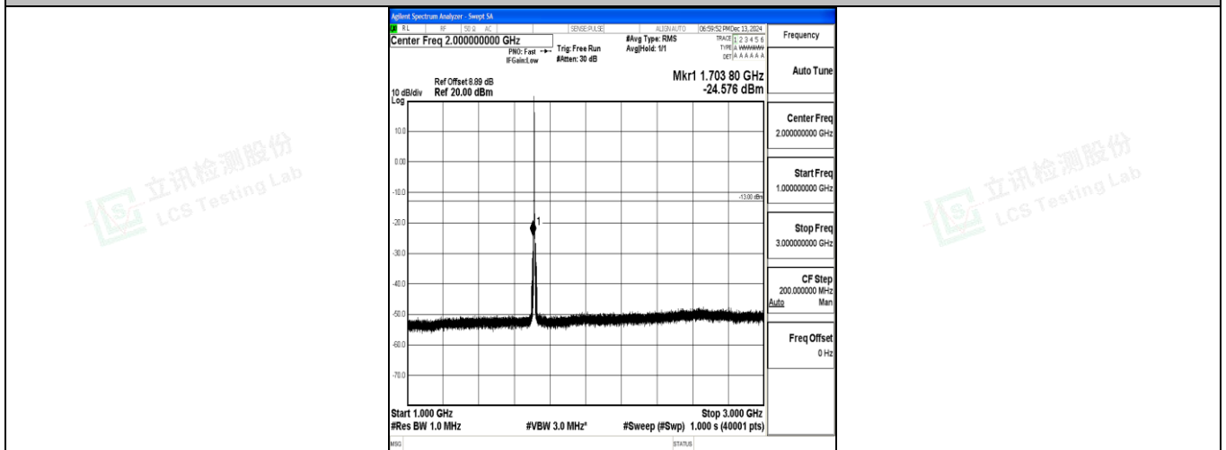
Band4_3MHz_QPSK_19965_1RB#0_1000~3000_1000~3000
