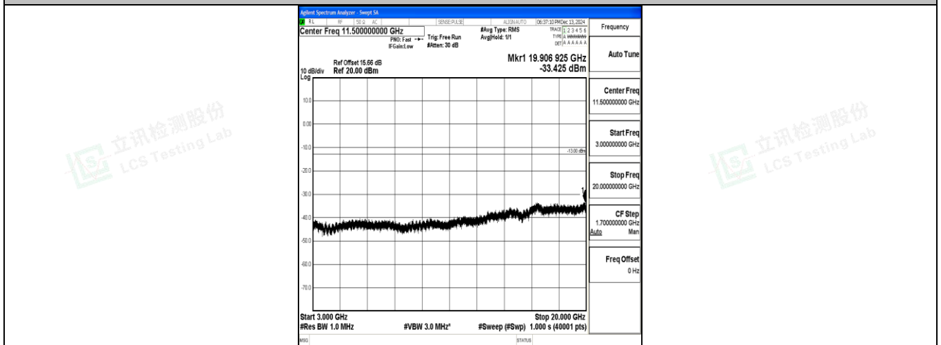
Band4_1.4MHz_16QAM_19957_1RB#0_3000~20000_3000~20000
