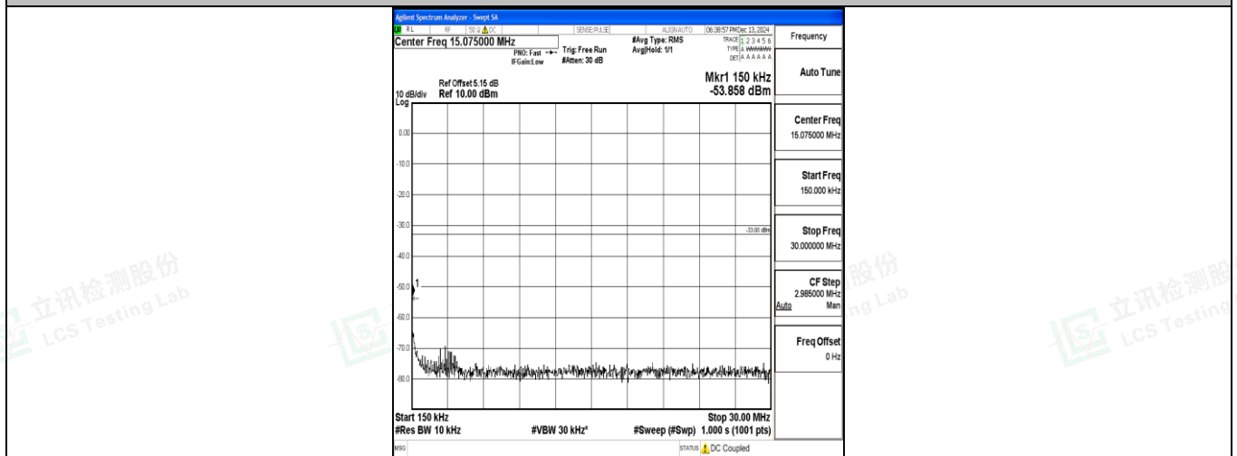
Band4_1.4MHz_16QAM_20393_1RB#0_0.15~30_0.15~30
