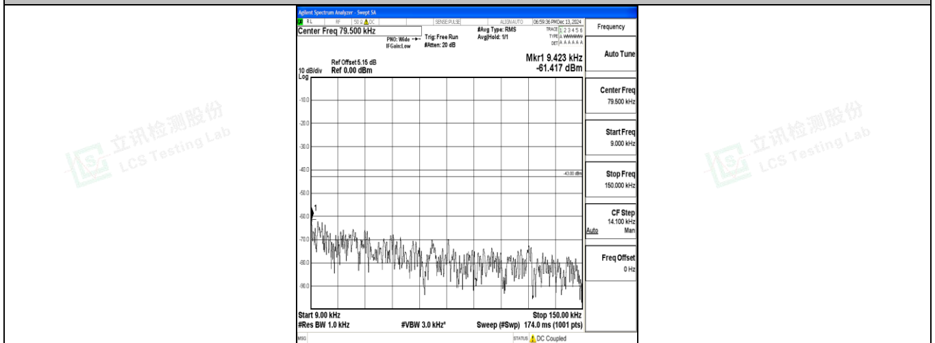
Band4_3MHz_QPSK_19965_1RB#0_0.009~0.15_0.009~0.15
