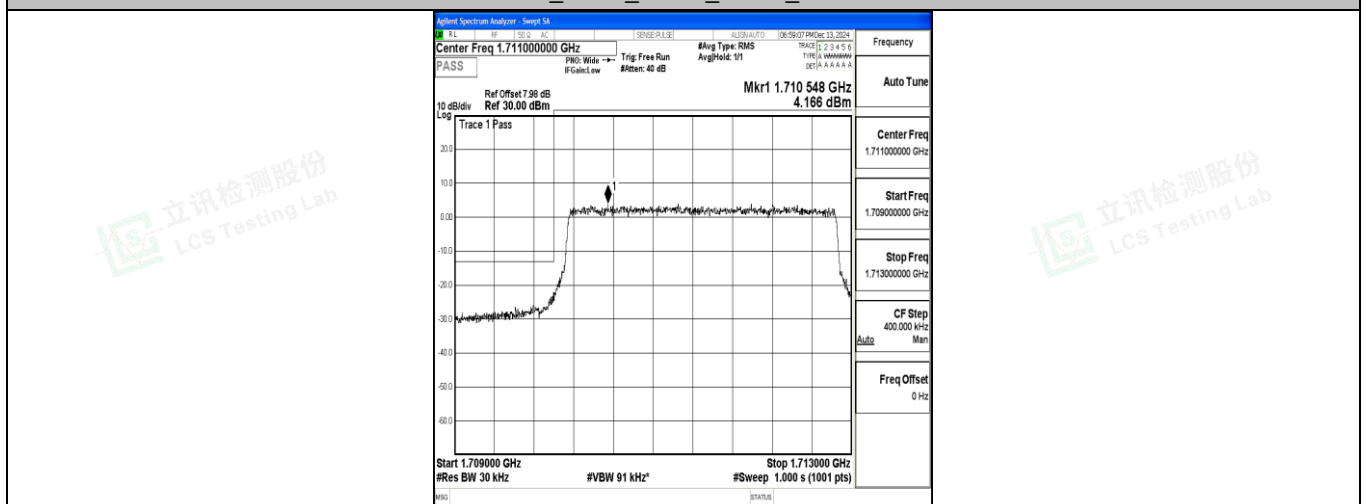
Band4_3MHz_16QAM_19965_15RB#0
