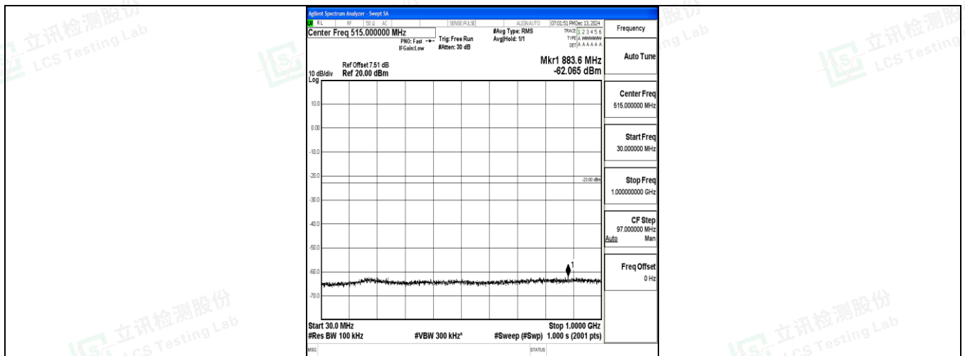
Band4_3MHz_QPSK_20385_1RB#0_30~1000_30~1000
