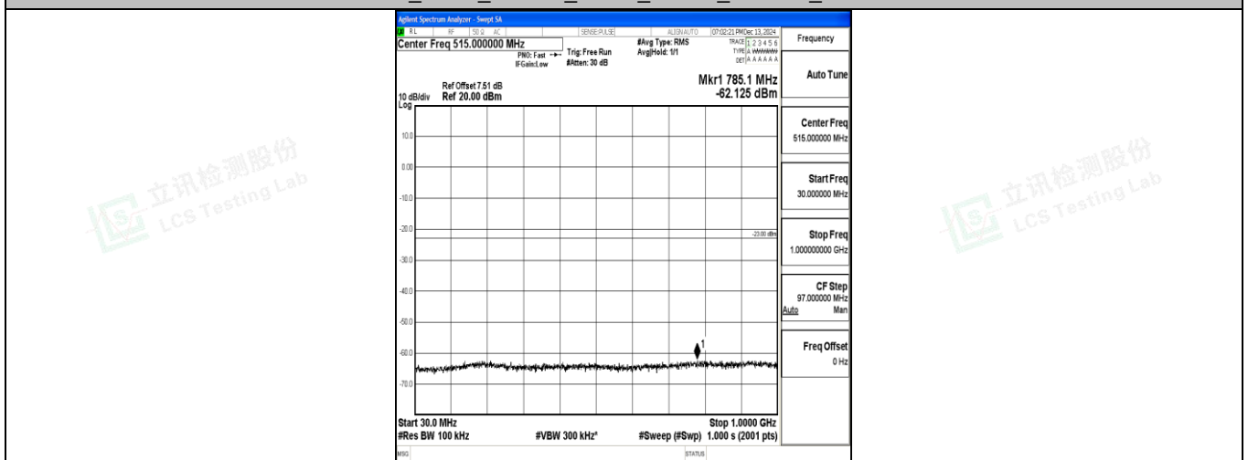
Band4_3MHz_16QAM_20385_1RB#0_30~1000_30~1000
