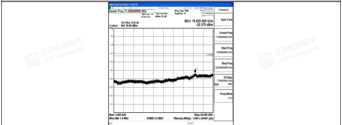
Band4_5MHz_16QAM_19975_1RB#0_3000~20000_3000~20000
