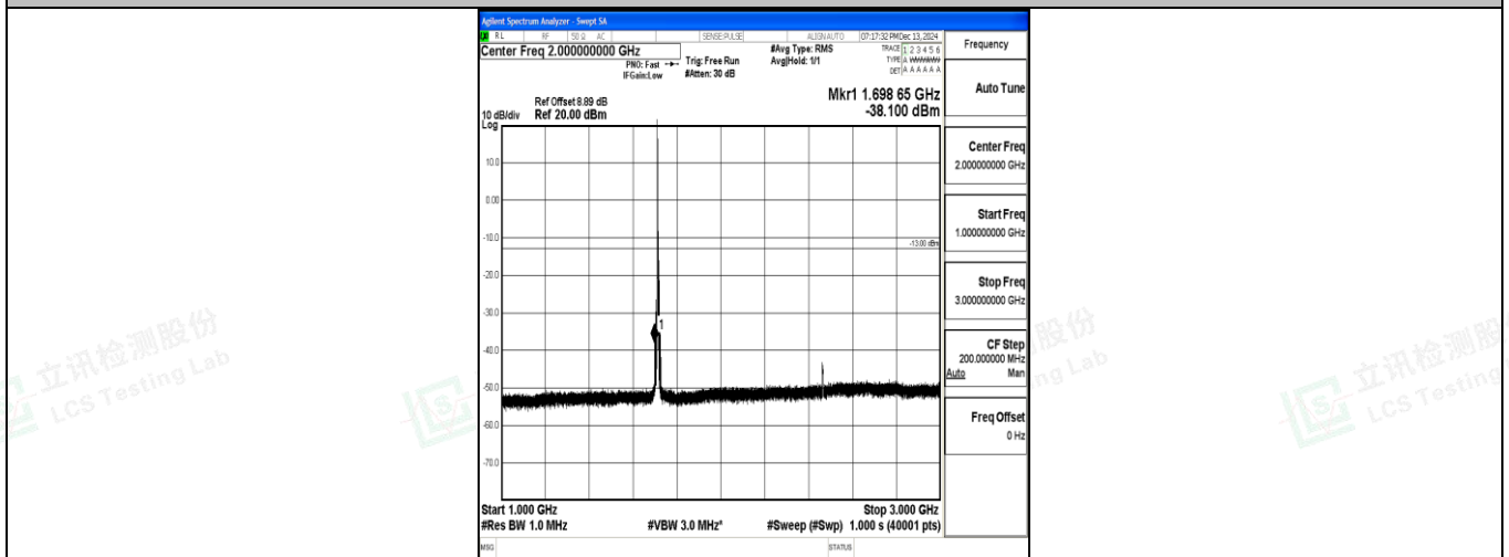
Band4_5MHz_16QAM_19975_1RB#0_1000~3000_1000~3000
