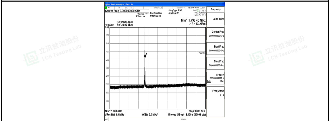
Band4_1.4MHz_16QAM_20175_1RB#0_1000~3000_1000~3000
