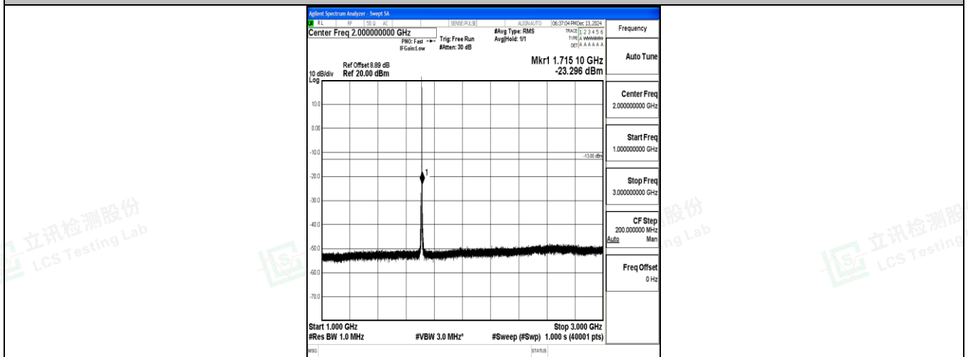
Band4_1.4MHz_16QAM_19957_1RB#0_1000~3000_1000~3000
