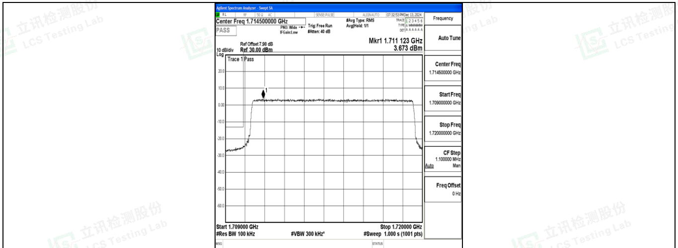
Band4_10MHz_QPSK_20000_50RB#0
