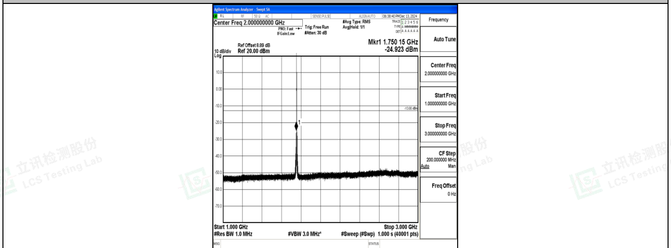
Band4_1.4MHz_QPSK_20393_1RB#0_1000~3000_1000~3000
