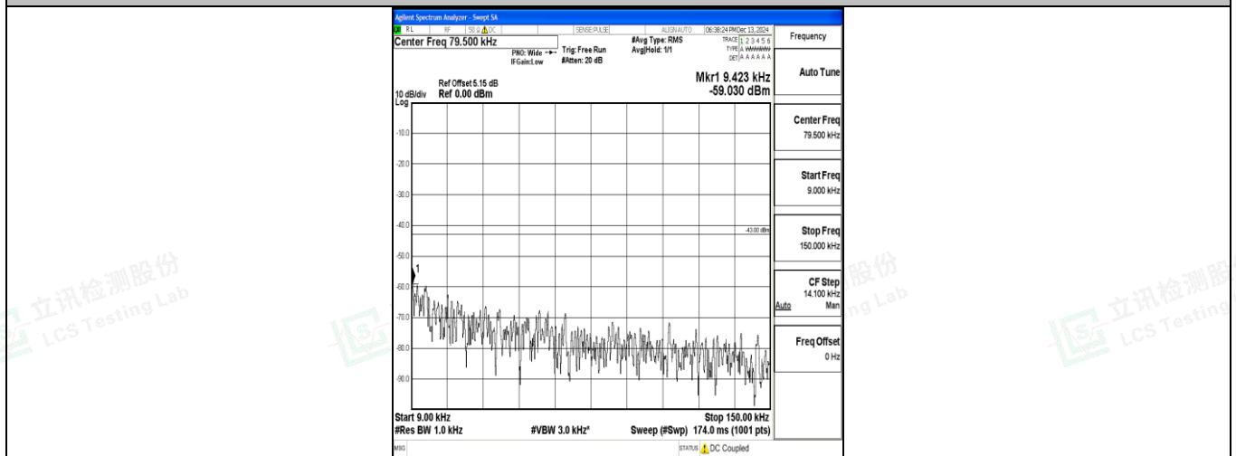
Band4_1.4MHz_QPSK_20393_1RB#0_0.009~0.15_0.009~0.15
