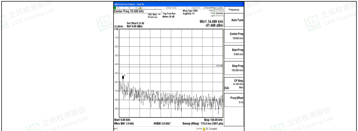
Band4_3MHz_QPSK_20175_1RB#0_0.009~0.15_0.009~0.15
