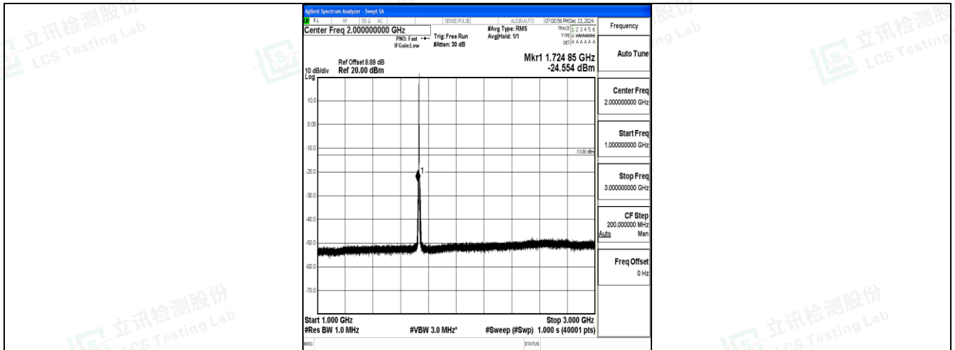
Band4_3MHz_QPSK_20175_1RB#0_1000~3000_1000~3000
