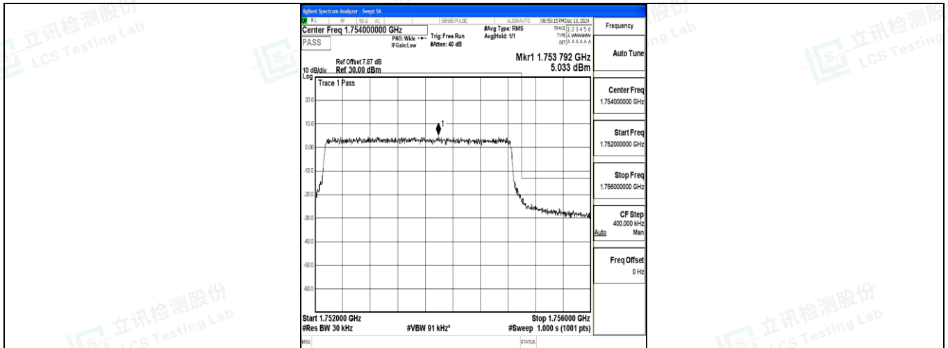
Band4_3MHz_QPSK_20385_15RB#0
