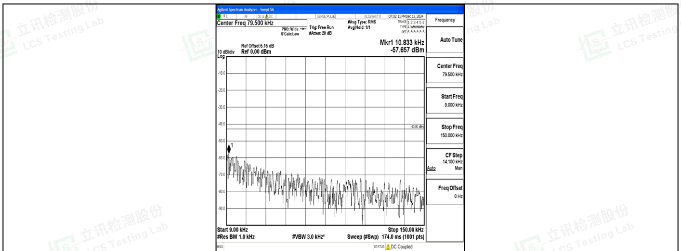
Band4_3MHz_16QAM_20385_1RB#0_0.009~0.15_0.009~0.15
