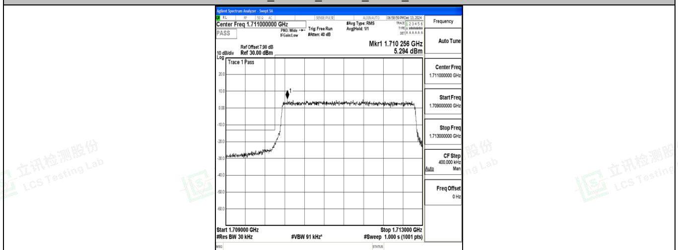
Band4_3MHz_QPSK_19965_15RB#0
