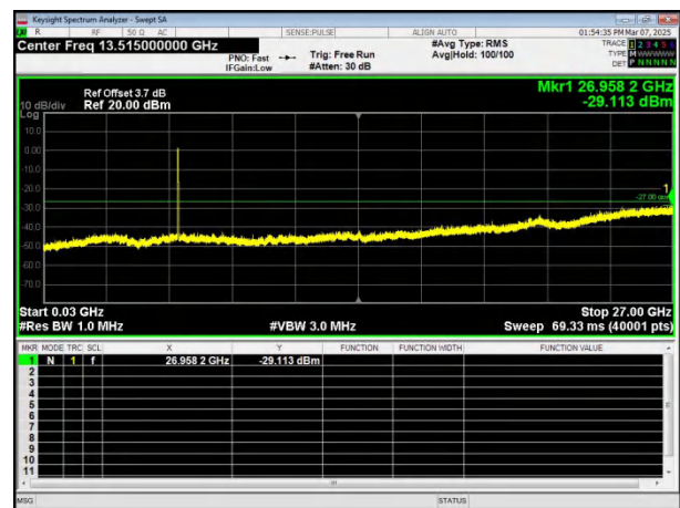
802.11ac40 on channel 163
