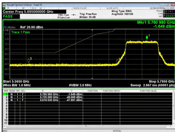
(802.11ax40) Band Edge, Left Side
