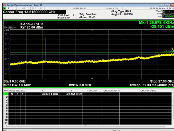
802.11ax20 on channel 165
