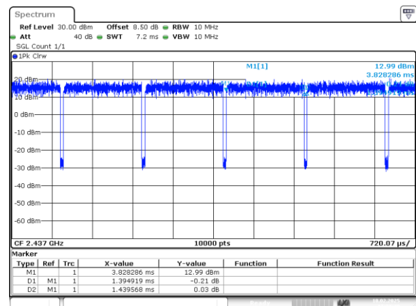
802.11g_2437MHz_Chain 1
