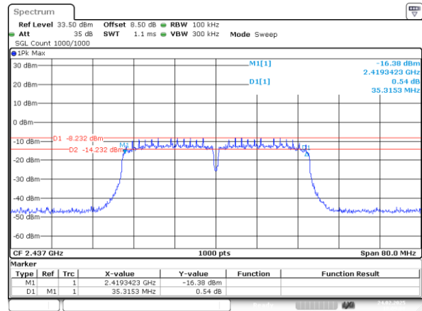
802.11n40_2437MHz_Chain 1
