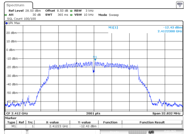
802.11g_2412MHz_Chain 1
