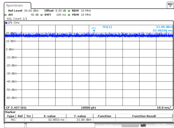
802.11g_2437MHz_Chain 0
