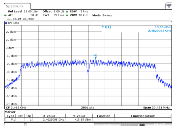
802.11g_2462MHz_Chain 0
